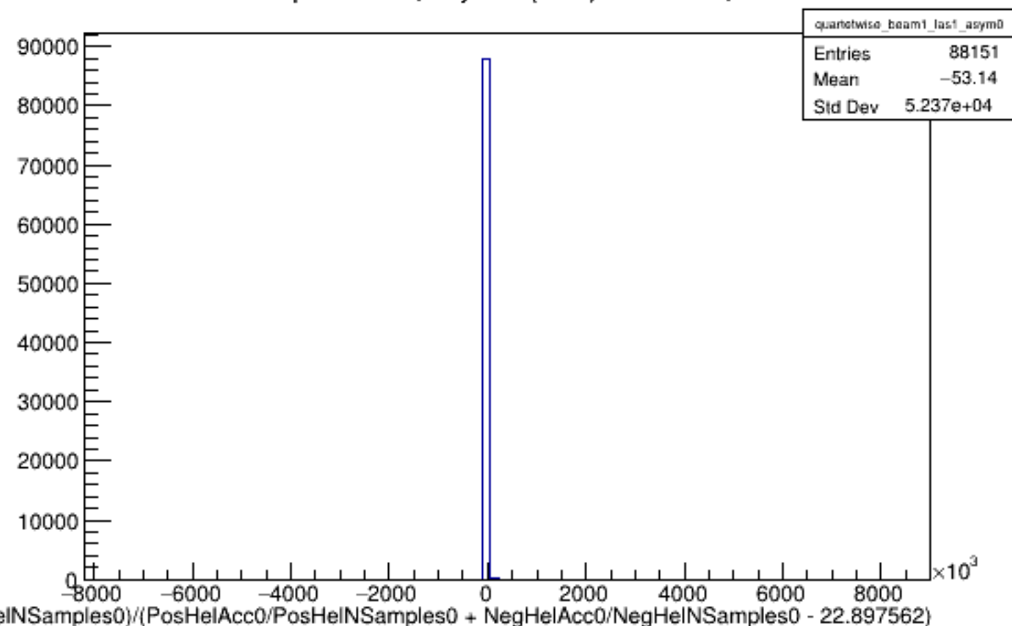
Run 4438 quartetwise, Asyms0 (Raw): Beam ON, Laser ON
