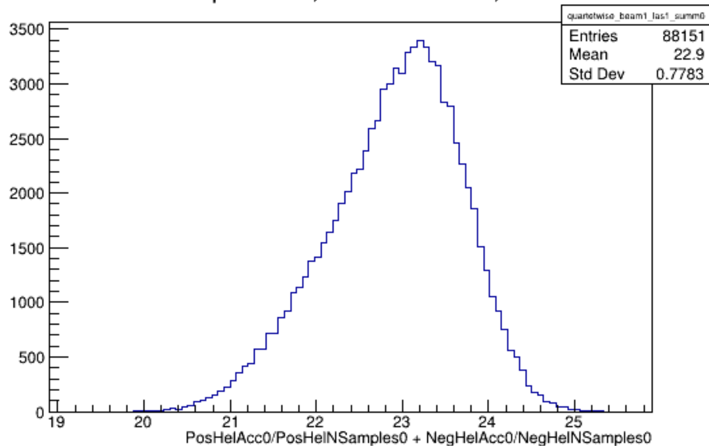
Run 4438 quartetwise, Sums0: Beam ON, Laser ON
