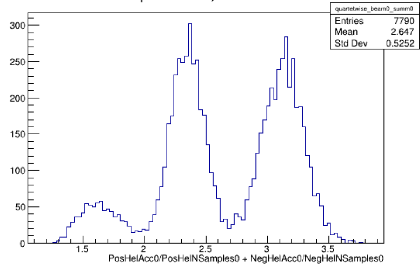
Run 4438 quartetwise, Sums0: Beam OFF
