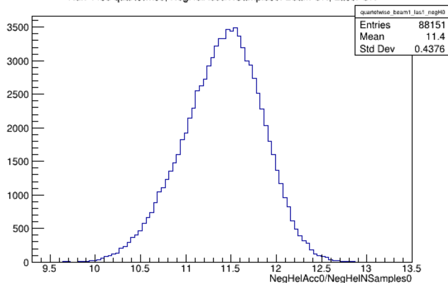
Run 4438 quartetwise, NegHelAcc0/NSamples0: Beam ON, Laser ON
