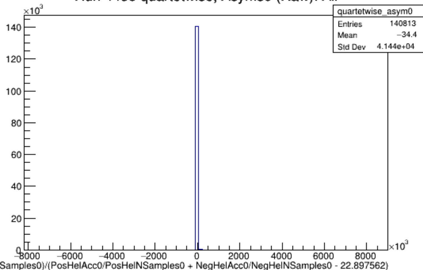
Run 4438 quartetwise, Asyms0 (Raw): All
