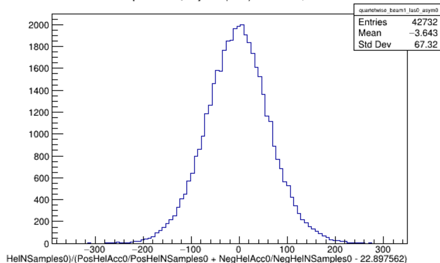
Run 4438 quartetwise, Asyms0 (Raw): Beam ON, Laser OFF
