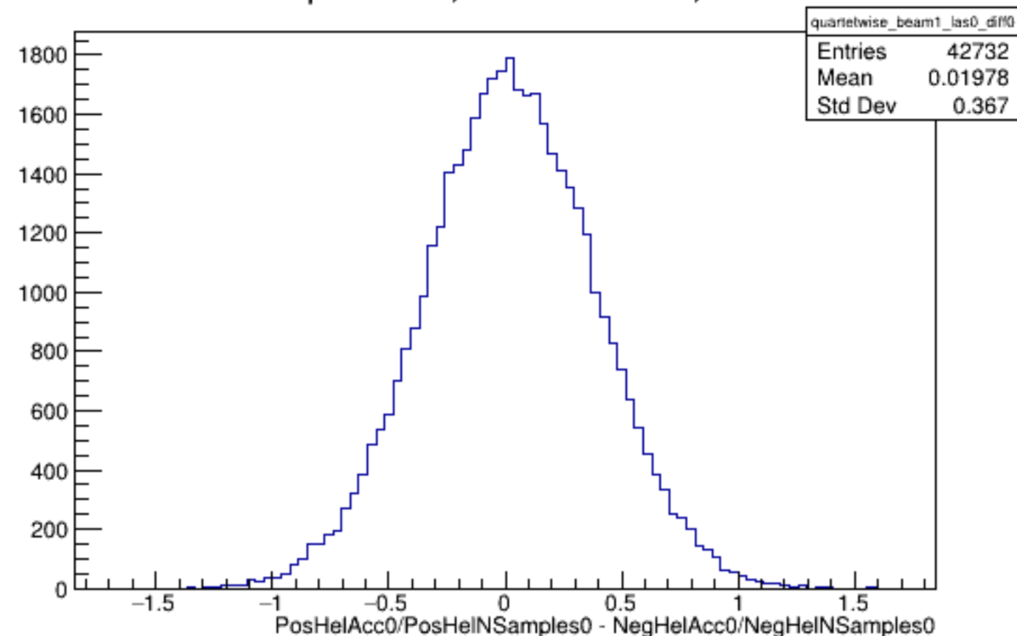
Run 4438 quartetwise, Diffs0: Beam ON, Laser OFF
