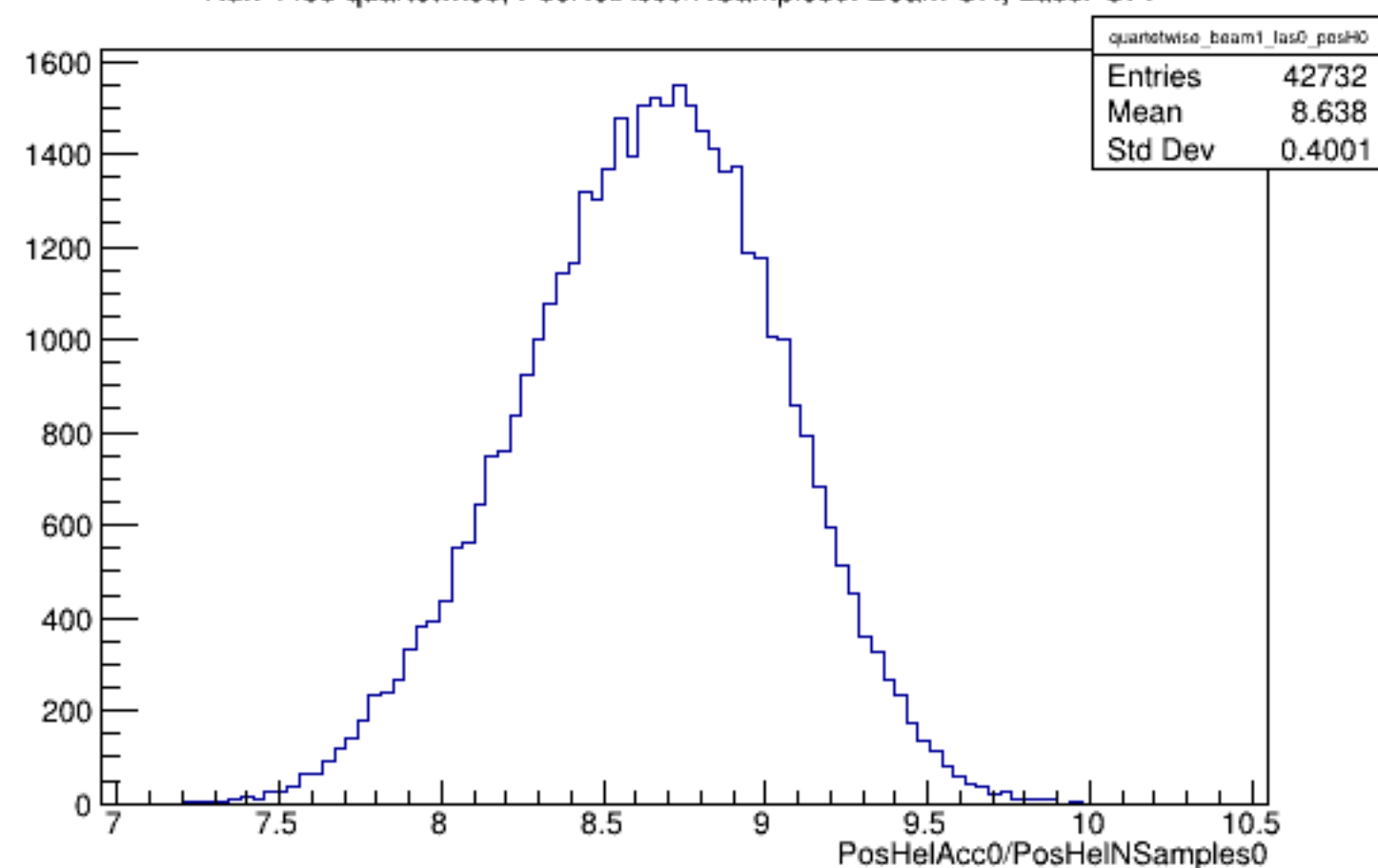
Run 4438 quartetwise, PosHelAcc0/NSamples0: Beam ON, Laser OFF
