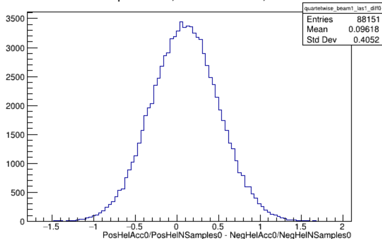
Run 4438 quartetwise, Diffs0: Beam ON, Laser ON
