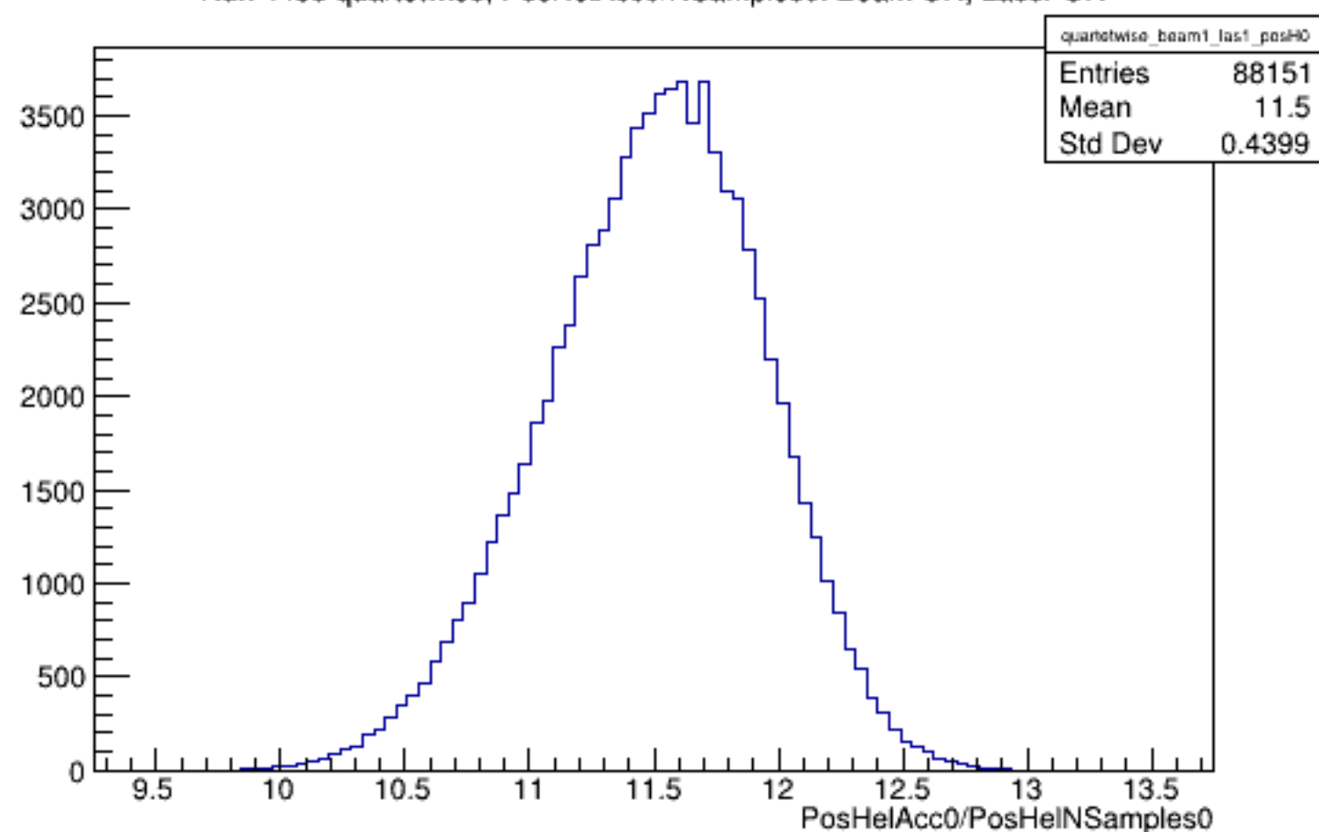
Run 4438 quartetwise, PosHelAcc0/NSamples0: Beam ON, Laser ON
