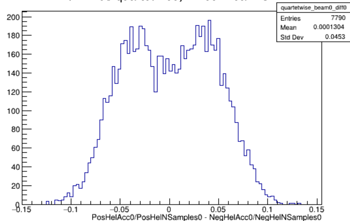
Run 4438 quartetwise, Diffs0: Beam OFF
