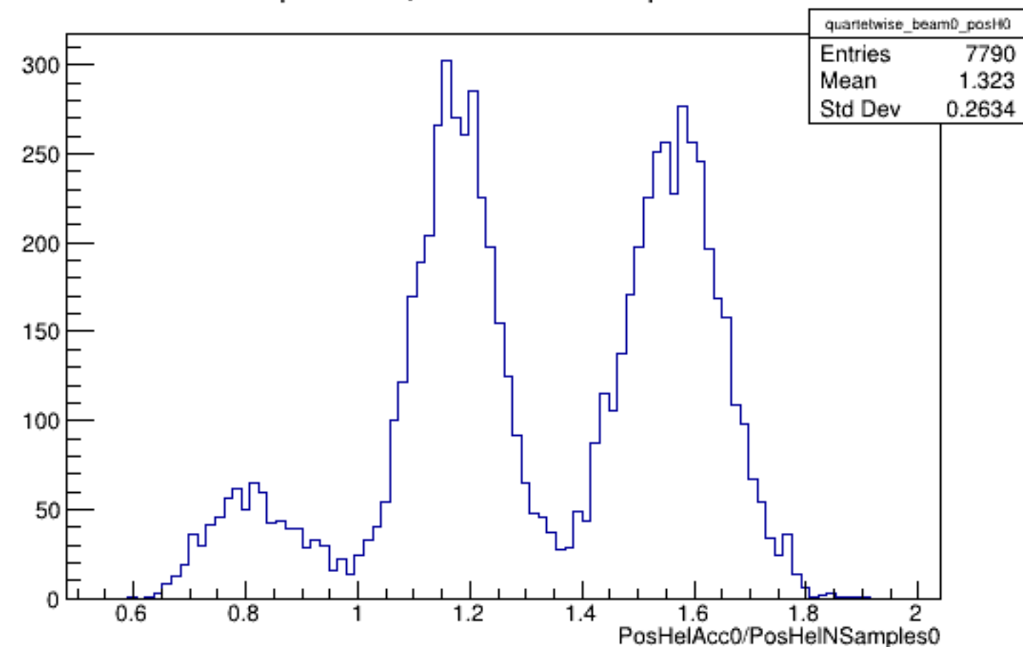
Run 4438 quartetwise, PosHelAcc0/NSamples0: Beam OFF
