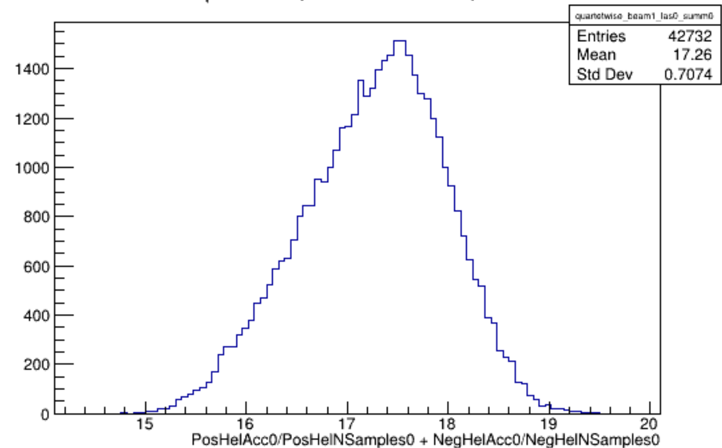
Run 4438 quartetwise, Sums0: Beam ON, Laser OFF
