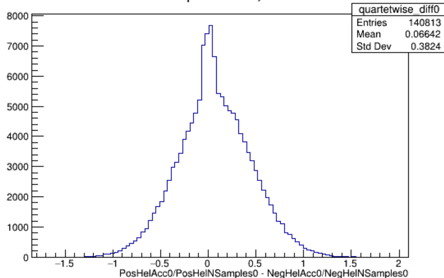
Run 4438 quartetwise, Diffs0: All
