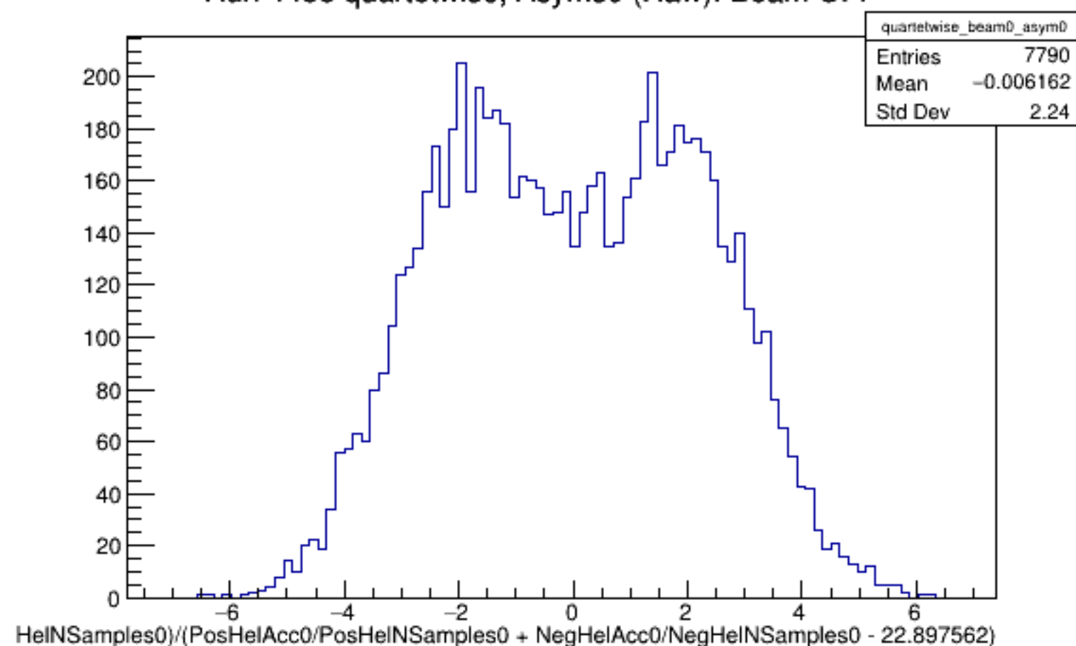
Run 4438 quartetwise, Asyms0 (Raw): Beam OFF
