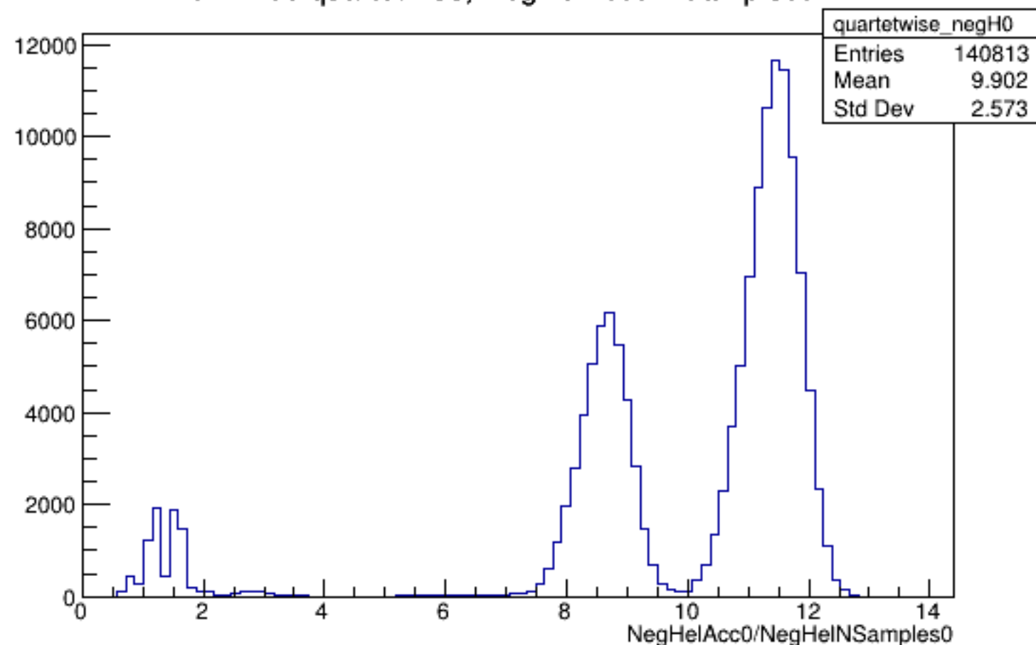
Run 4438 quartetwise, NegHelAcc0/NSamples0: All
