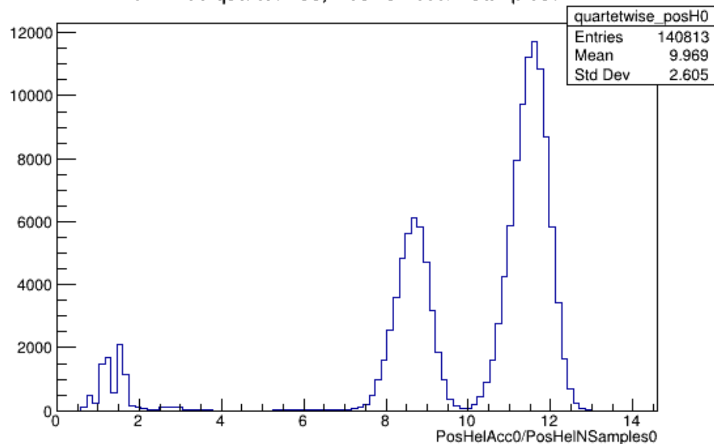
Run 4438 quartetwise, PosHelAcc0/NSamples0: All
