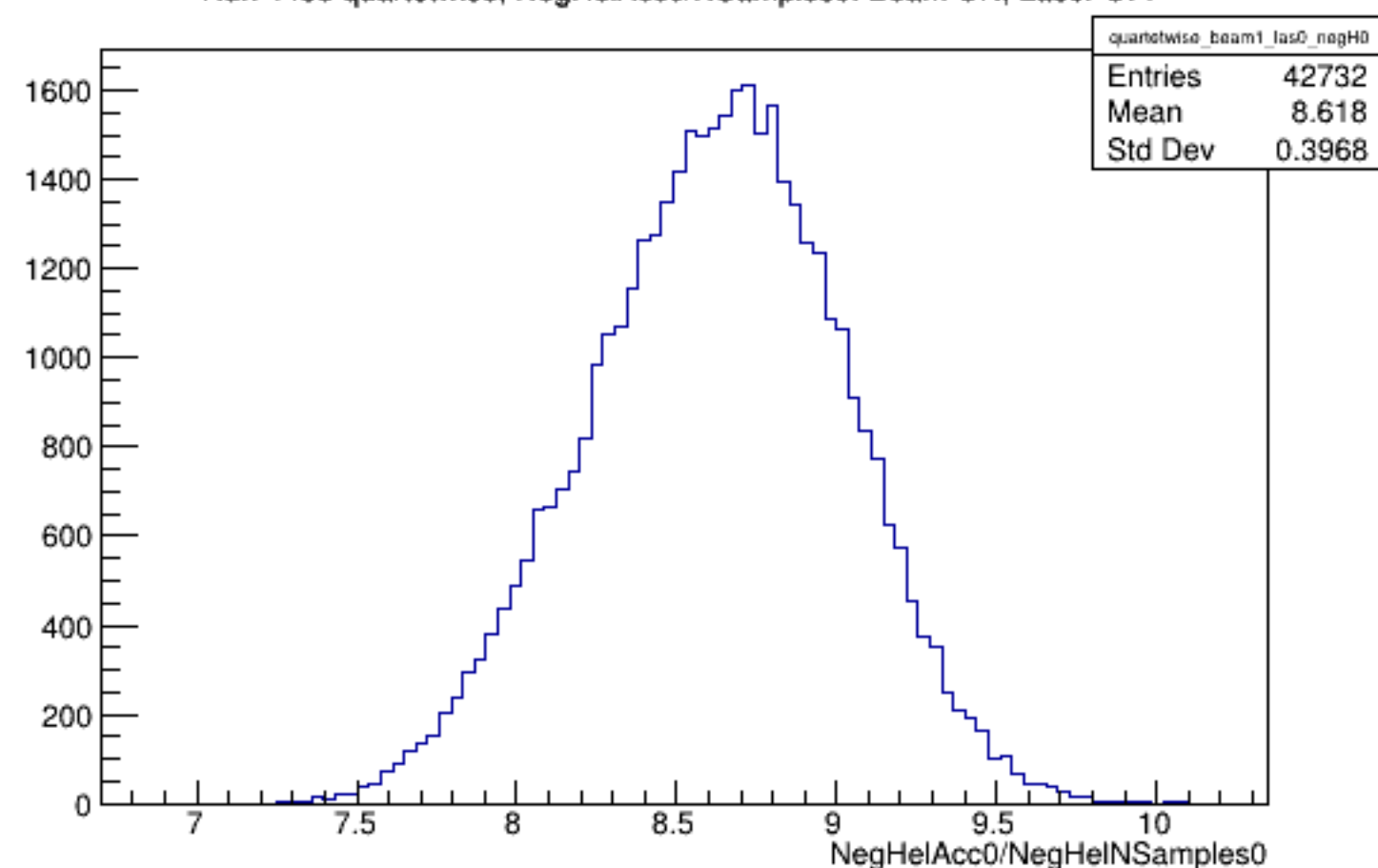
Run 4438 quartetwise, NegHelAcc0/NSamples0: Beam ON, Laser OFF
