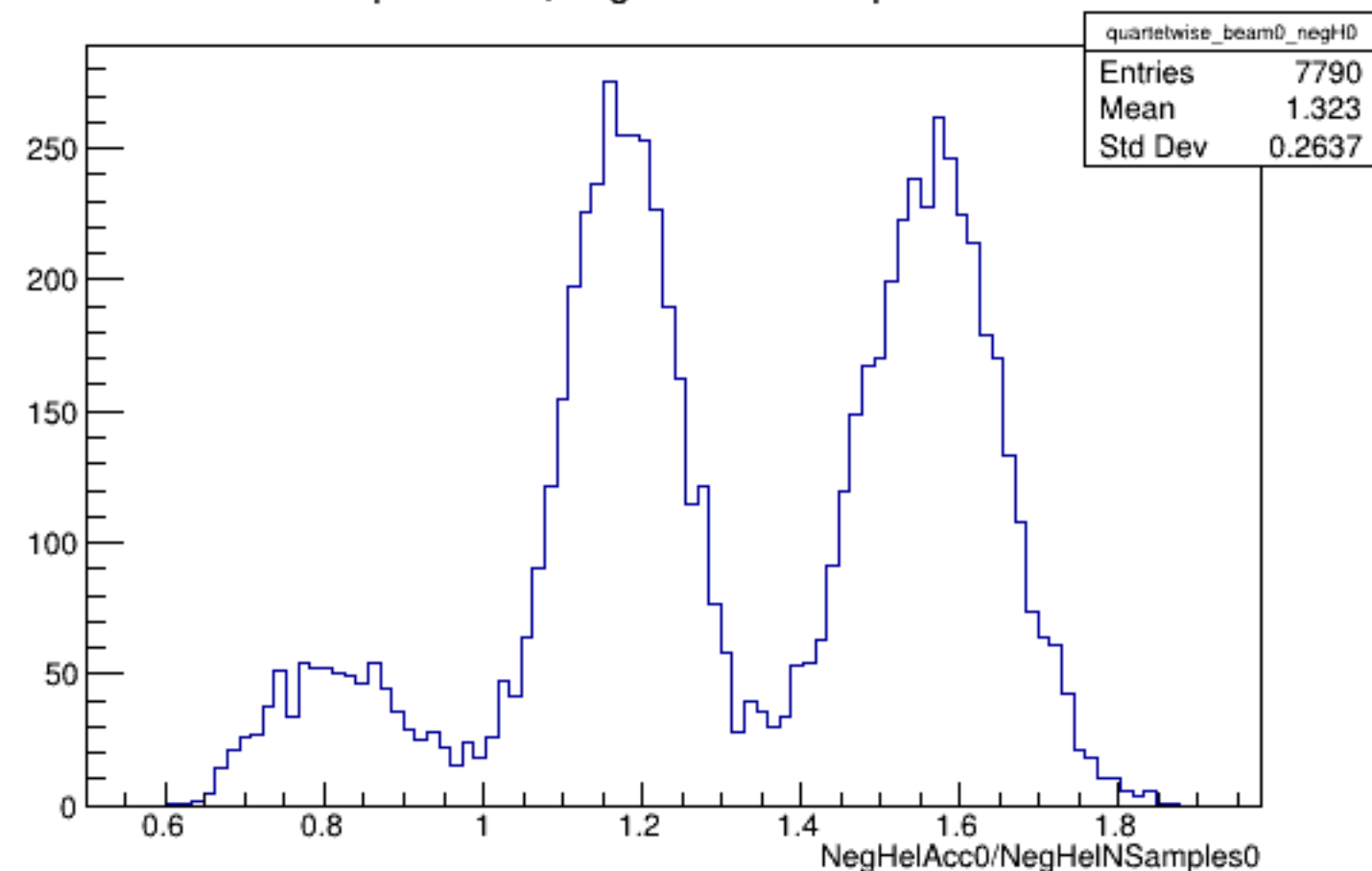
Run 4438 quartetwise, NegHelAcc0/NSamples0: Beam OFF
