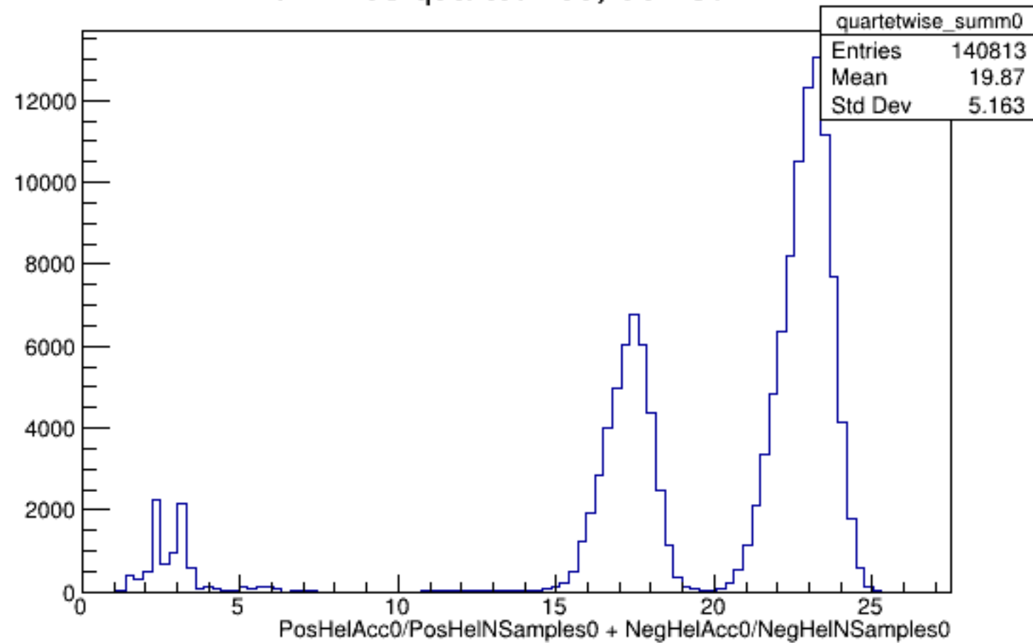
Run 4438 quartetwise, Sums0: All
