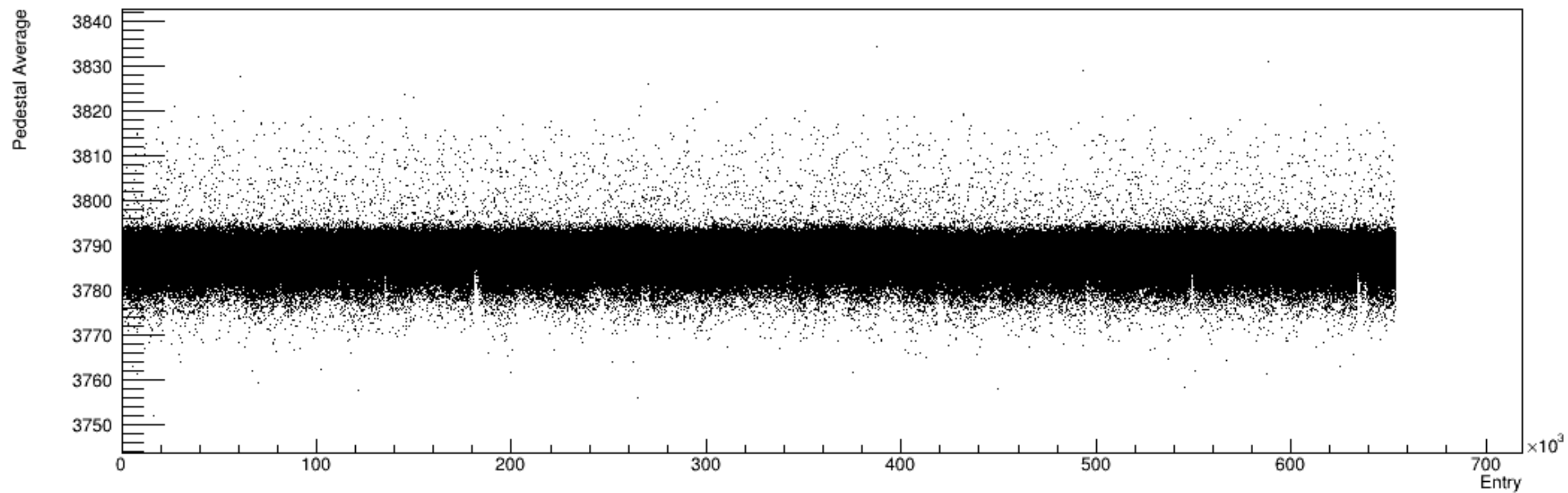
Run 4438, snapshots: Pedestal vs. Time
