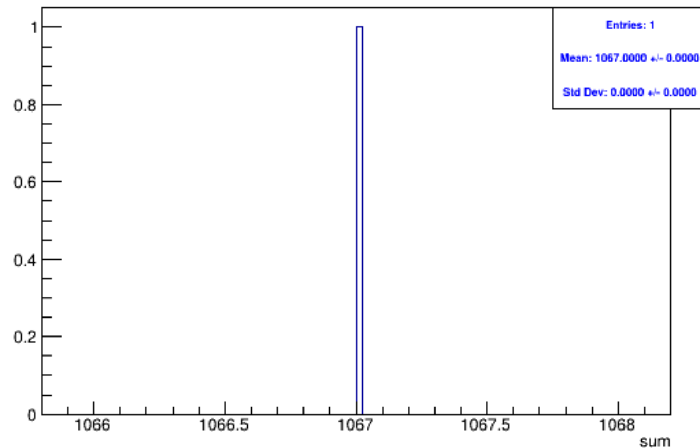
Run 4441 triggerwise, sums: Beam OFF
