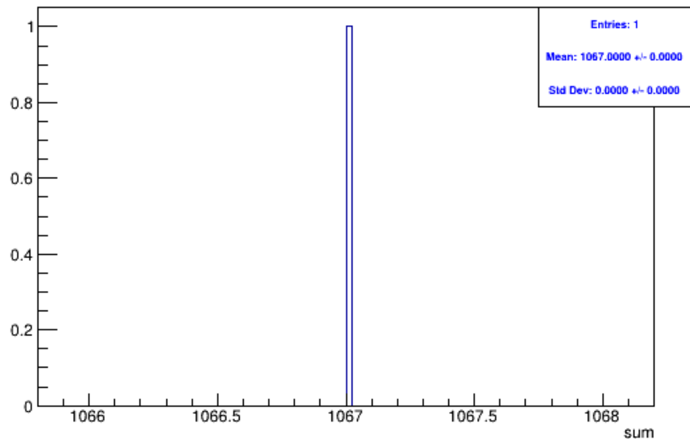
Run 4441 triggerwise, sums: All
