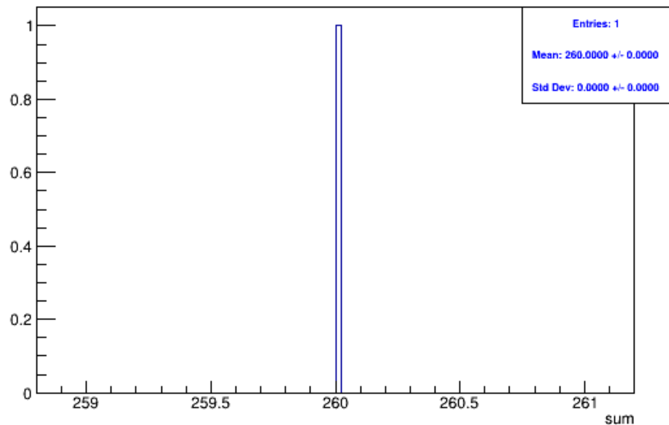
Run 4444 triggerwise, sums: All
