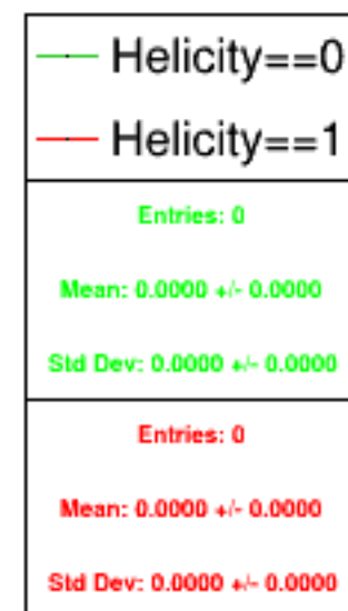
Run 4444 triggerwise, sums: Beam ON, Laser OFF
