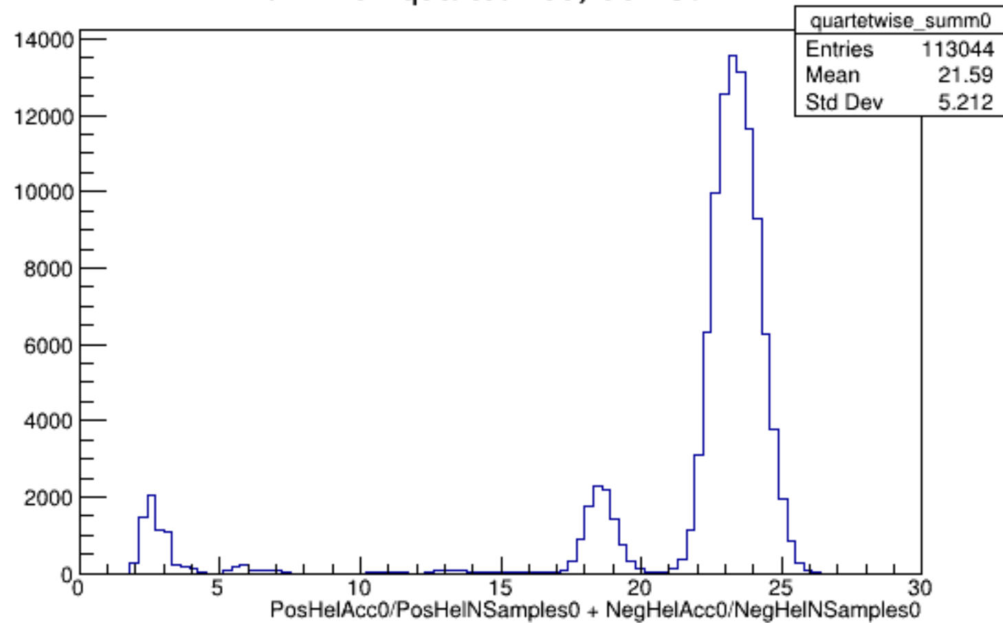
Run 4451 quartetwise, Sums0: All
