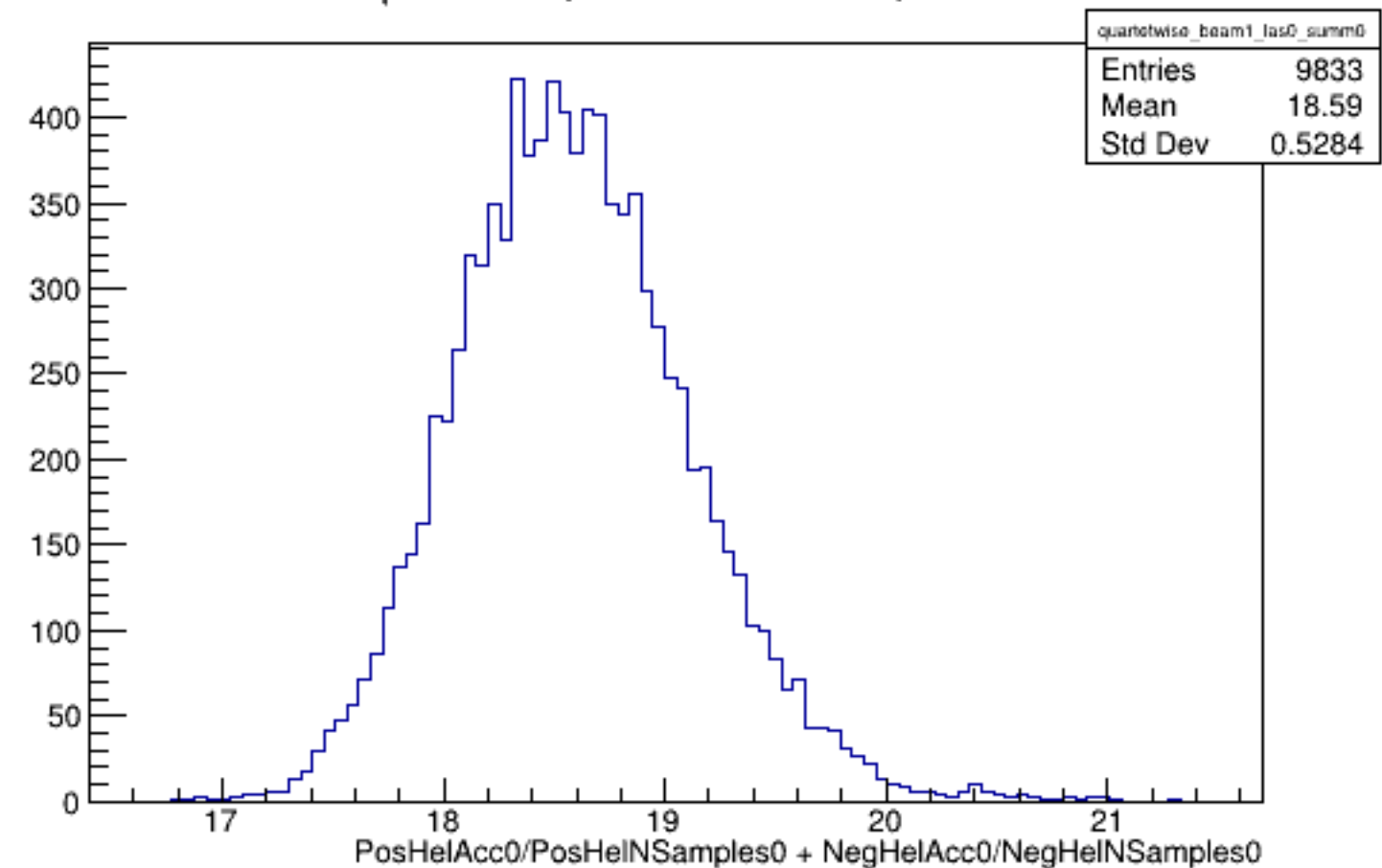
Run 4451 quartetwise, Sums0: Beam ON, Laser OFF
