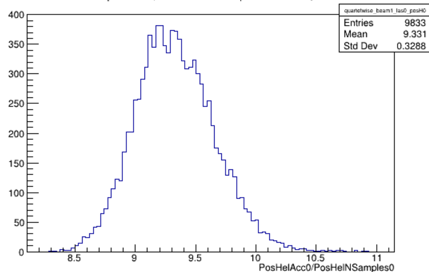
Run 4451 quartetwise, PosHelAcc0/NSamples0: Beam ON, Laser OFF
