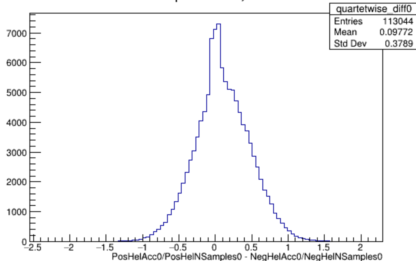
Run 4451 quartetwise, Diffs0: All
