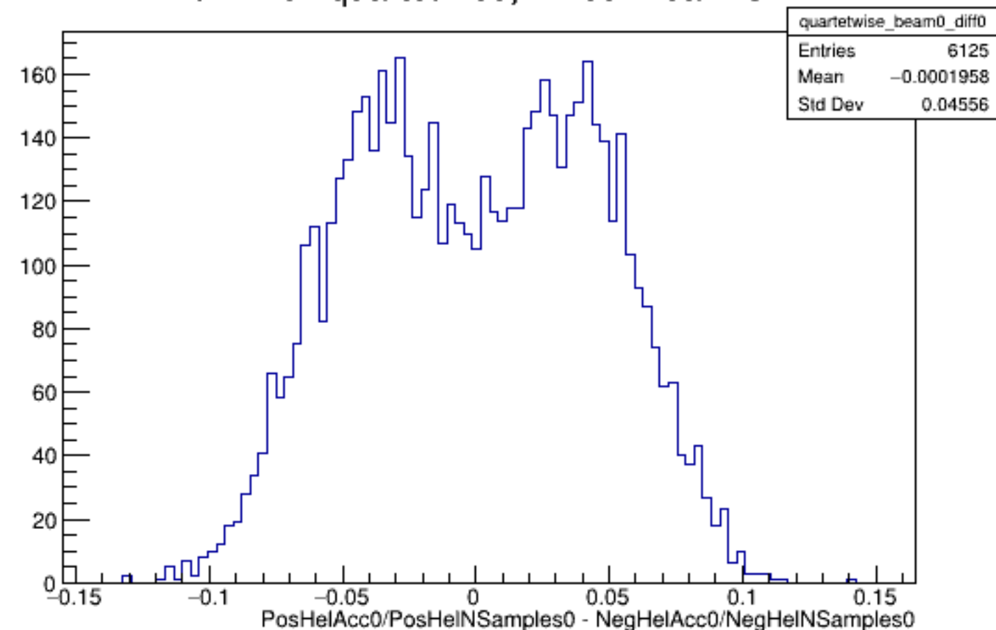
Run 4451 quartetwise, Diffs0: Beam OFF
