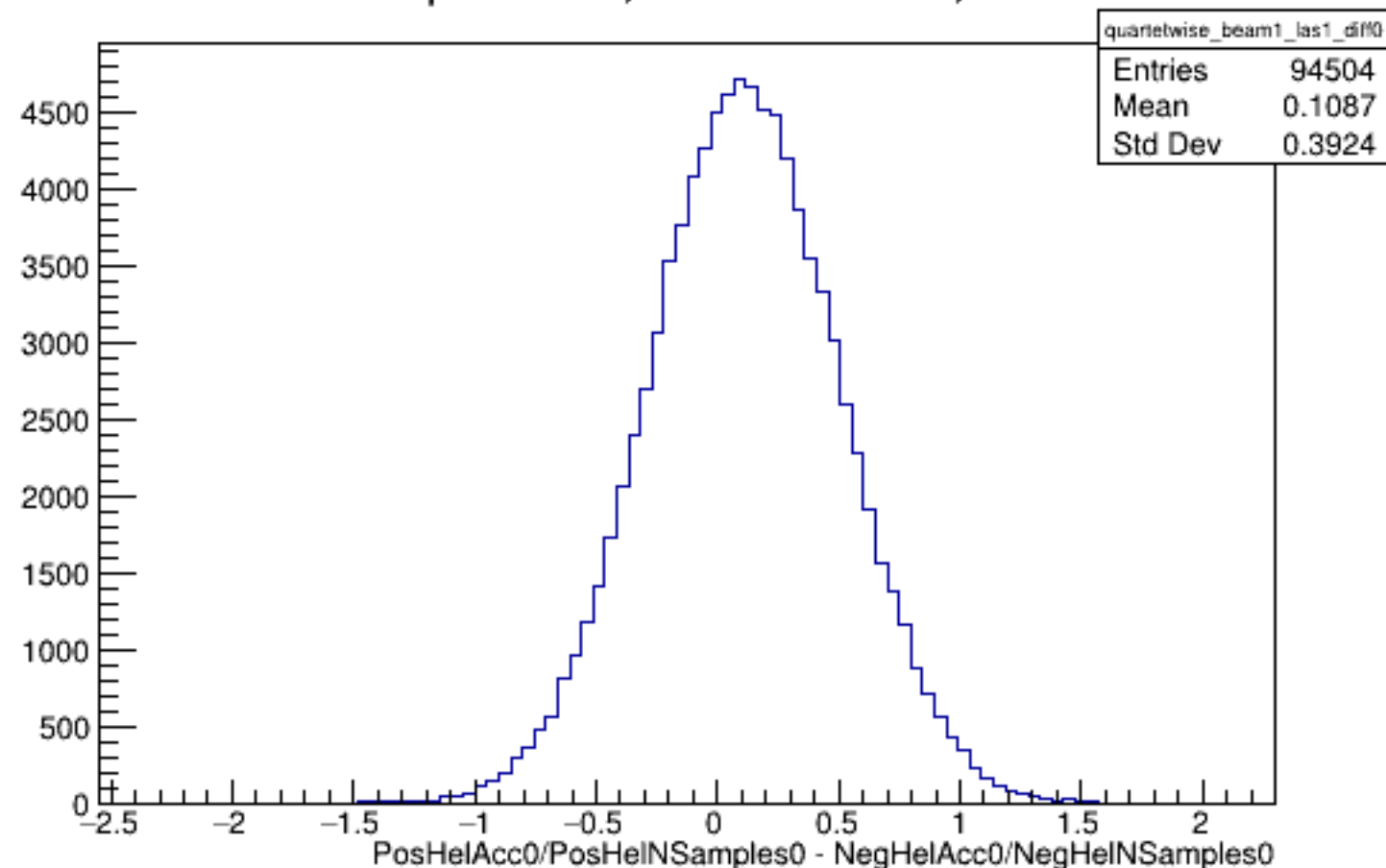
Run 4451 quartetwise, Diffs0: Beam ON, Laser ON
