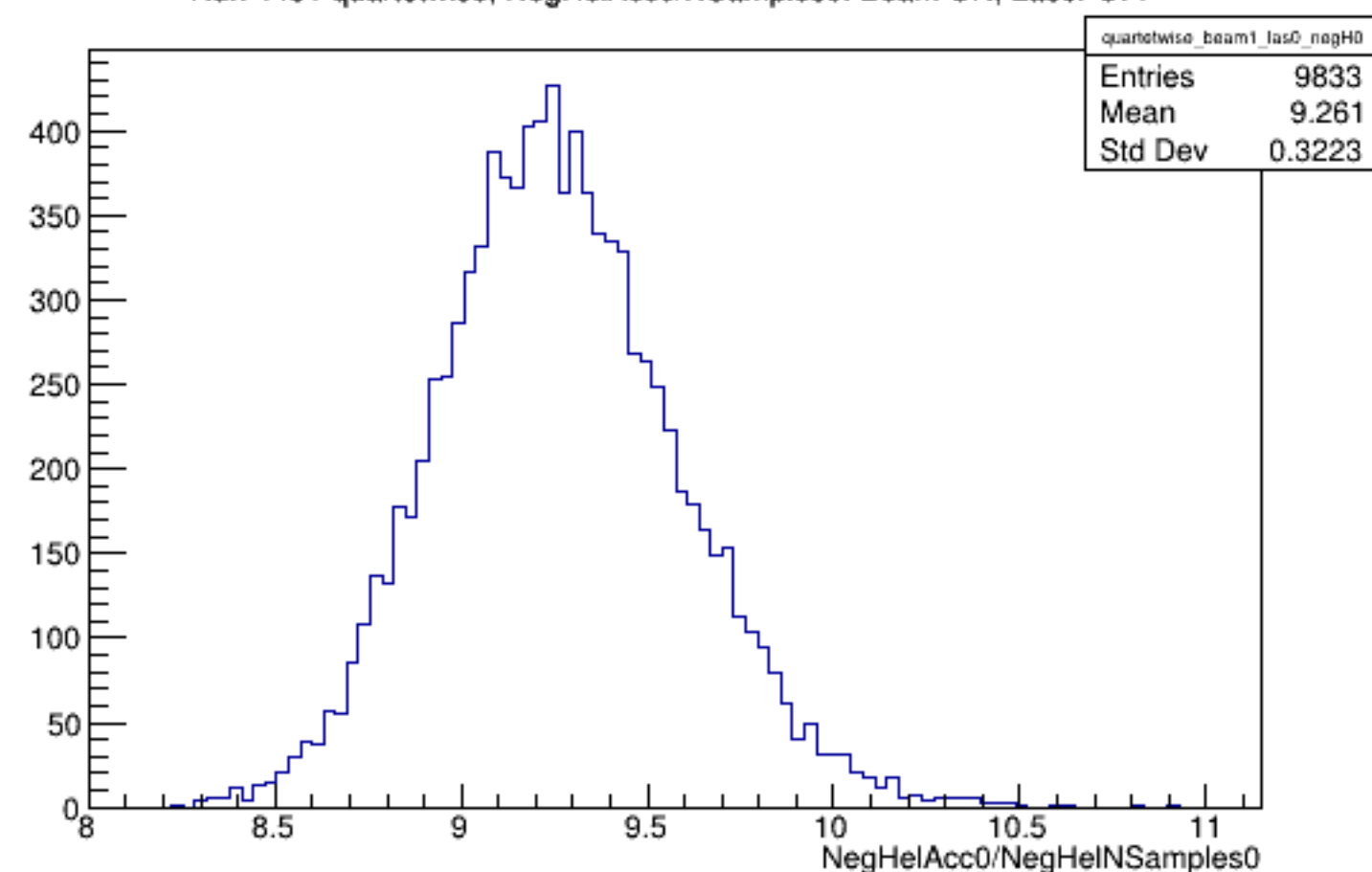
Run 4451 quartetwise, NegHelAcc0/NSamples0: Beam ON, Laser OFF
