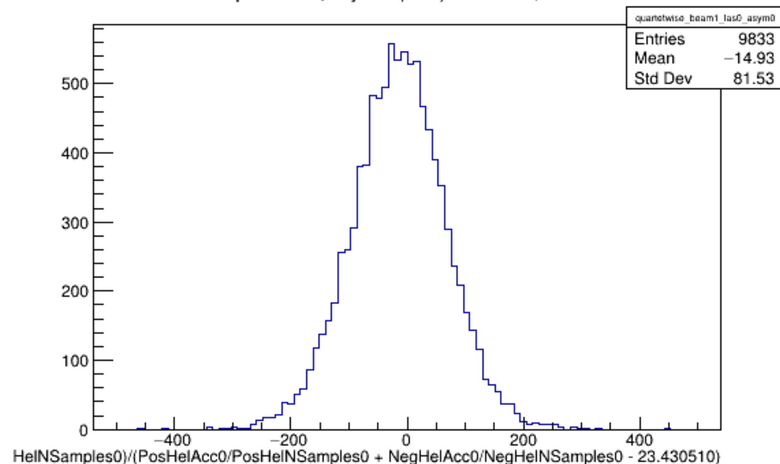
Run 4451 quartetwise, Asyms0 (Raw): Beam ON, Laser OFF
