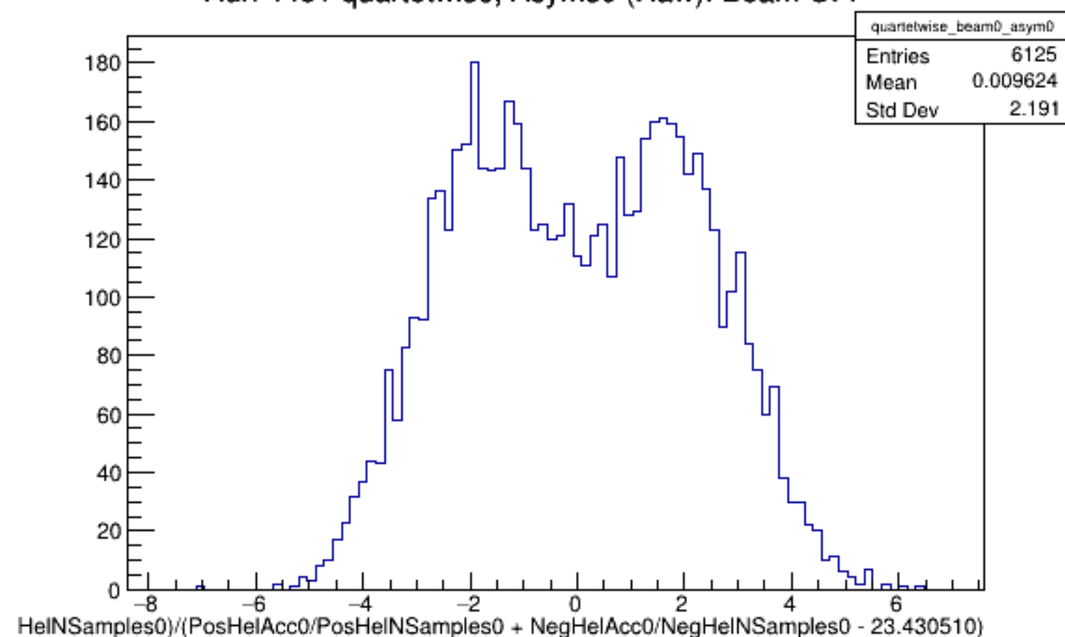
Run 4451 quartetwise, Asyms0 (Raw): Beam OFF
