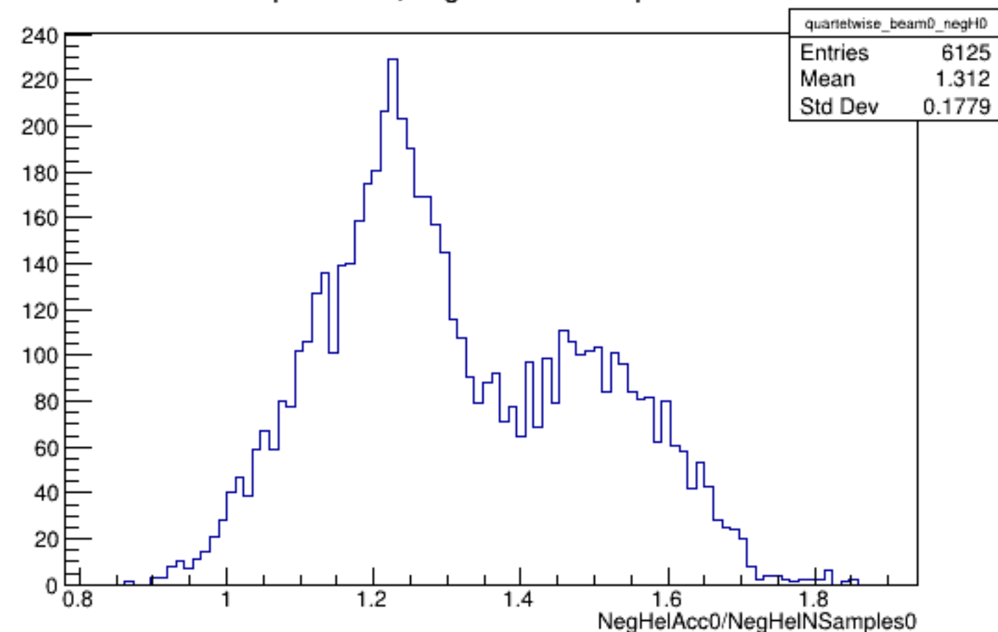
Run 4451 quartetwise, NegHelAcc0/NSamples0: Beam OFF
