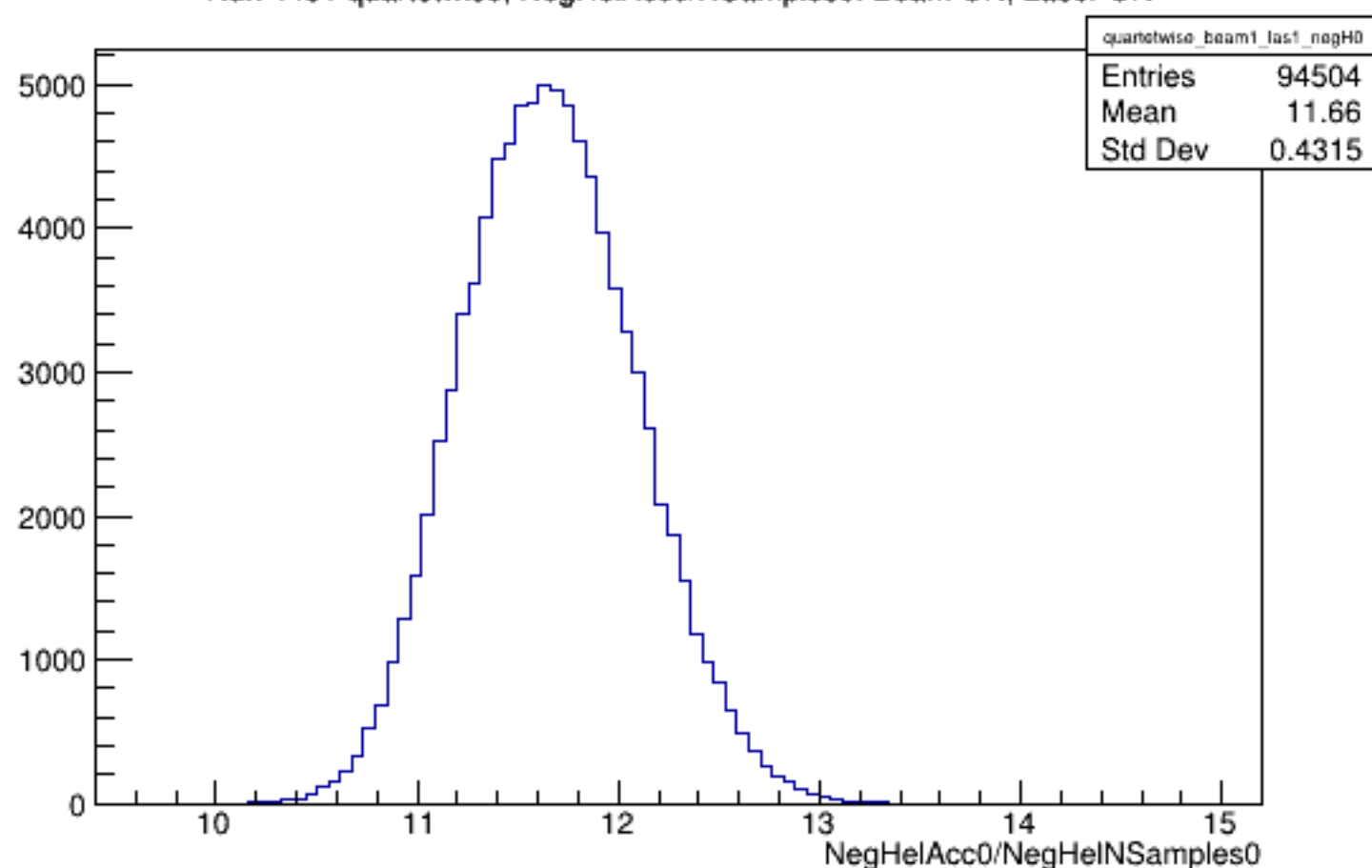
Run 4451 quartetwise, NegHelAcc0/NSamples0: Beam ON, Laser ON
