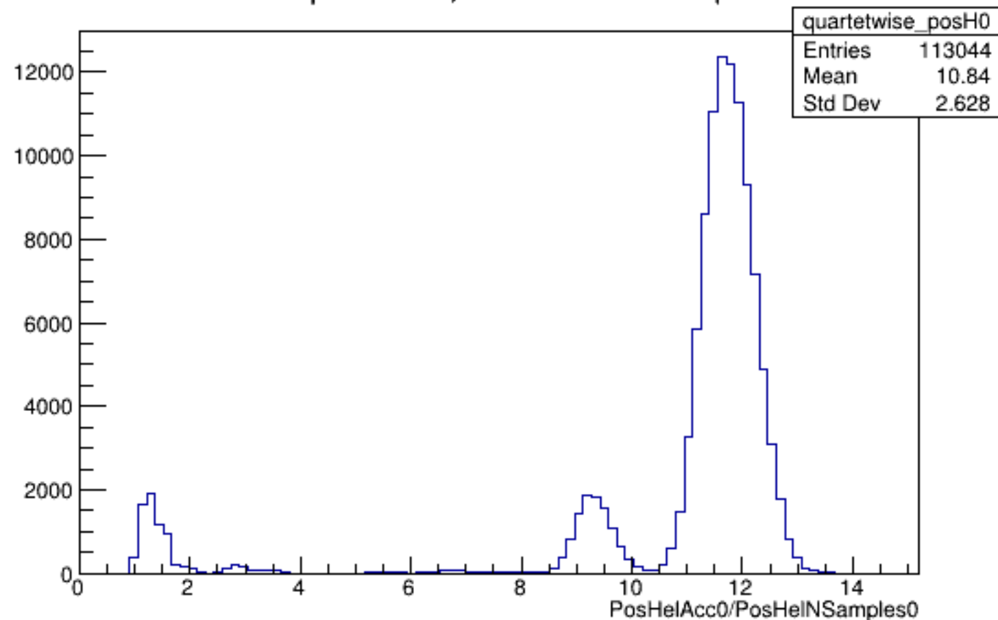
Run 4451 quartetwise, PosHelAcc0/NSamples0: All
