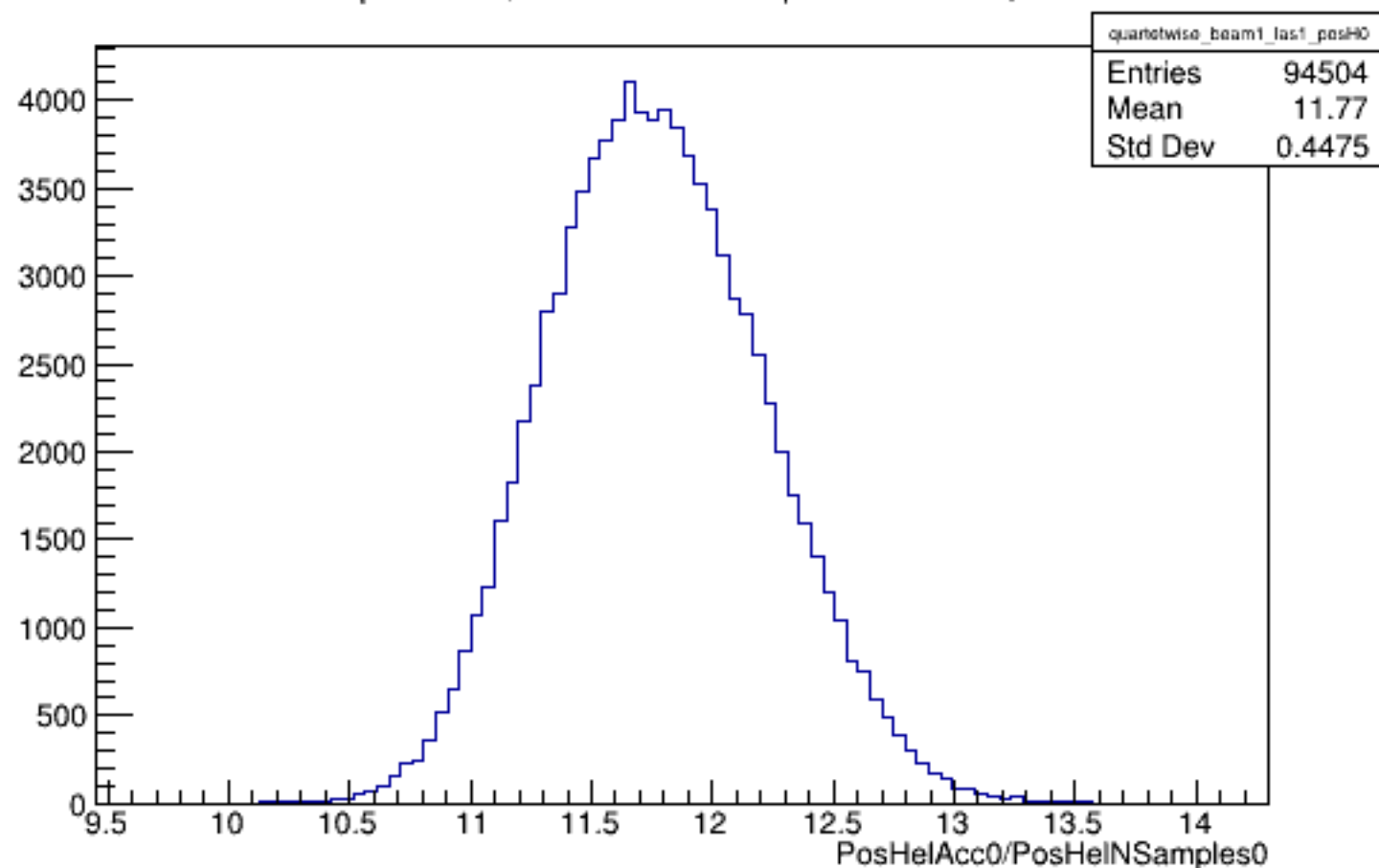
Run 4451 quartetwise, PosHelAcc0/NSamples0: Beam ON, Laser ON
