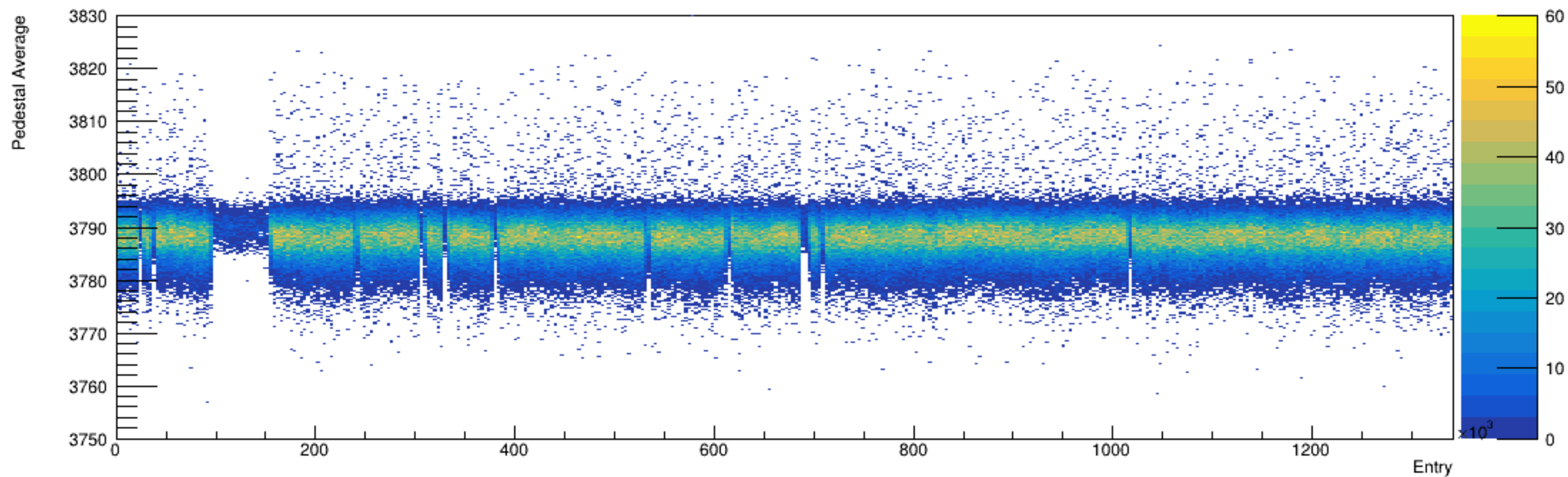
Run 4454, snapshots: Pedestal vs. Time
