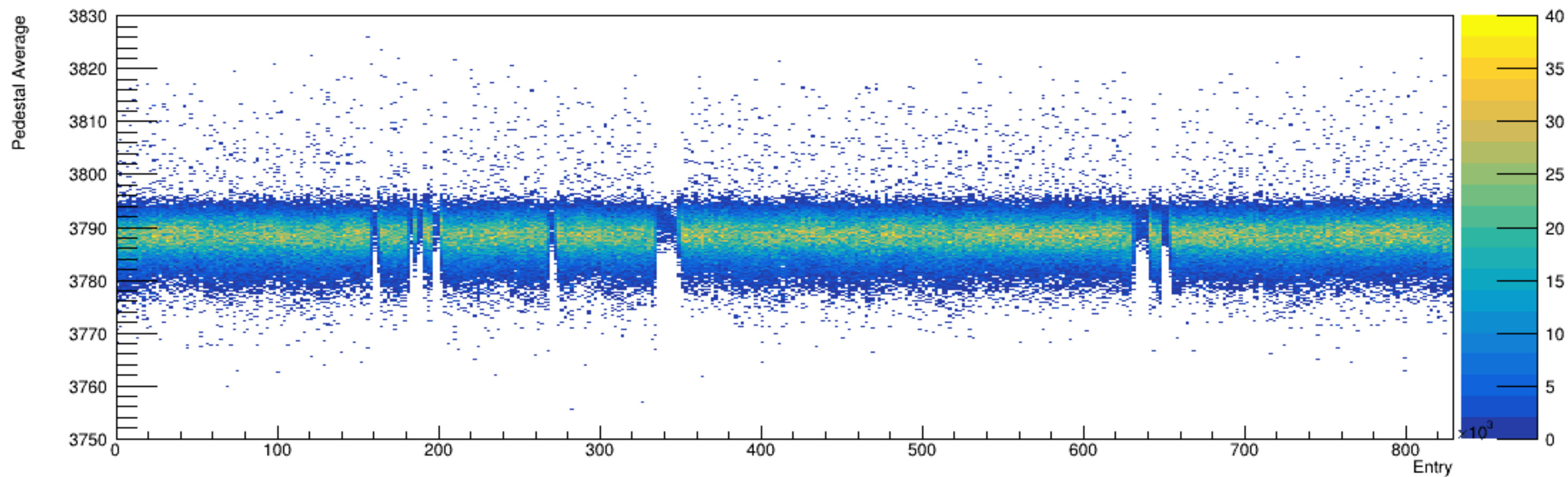
Run 4456, snapshots: Pedestal vs. Time
