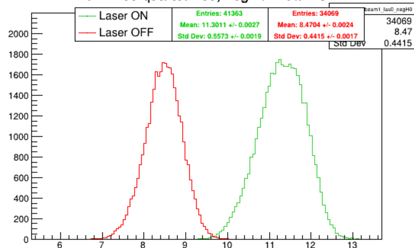
Run 4459 quartetwise, negH0: Beam ON
