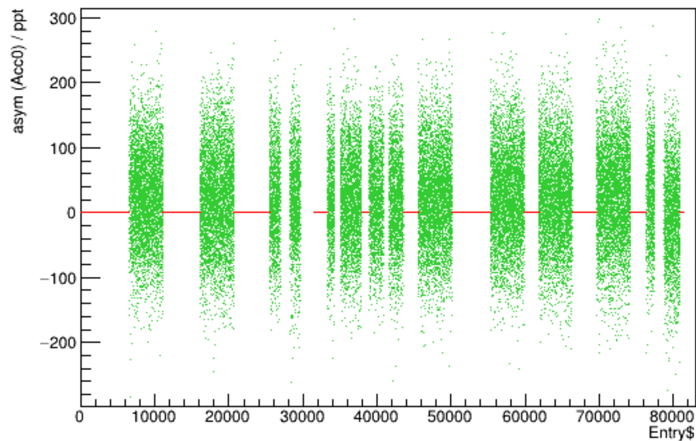
Run 4459 quartetwise, asym0sub vs time
