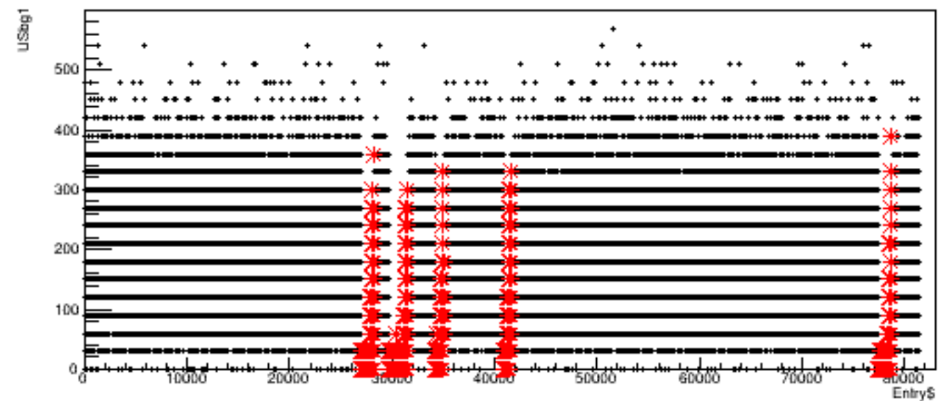
Run 4459, quartetwise: USbg1 vs time
