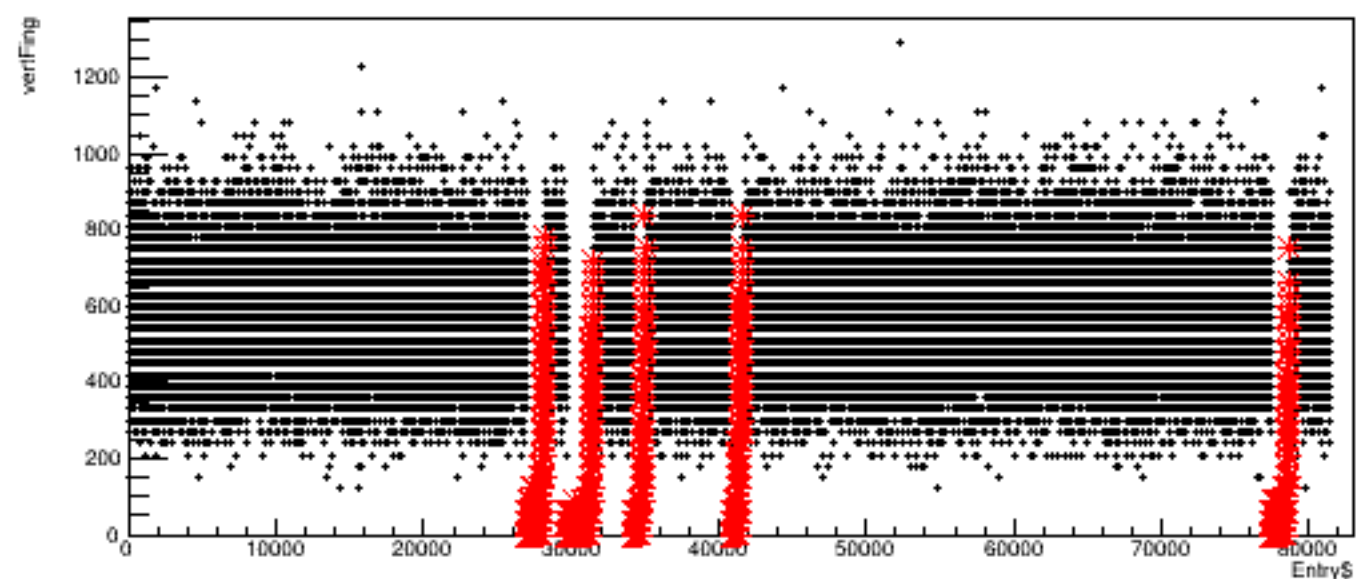
Run 4459, quartetwise: vertFing vs time
