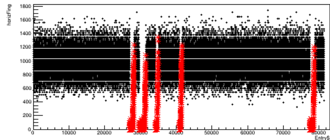
Run 4459, quartetwise: horizFing vs time
