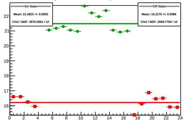
Cycle 4459.5: Multiplet Sums
