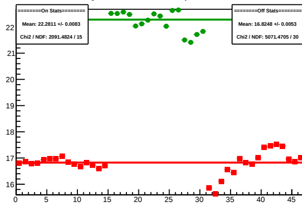
Cycle 4459.2: Multiplet Sums
