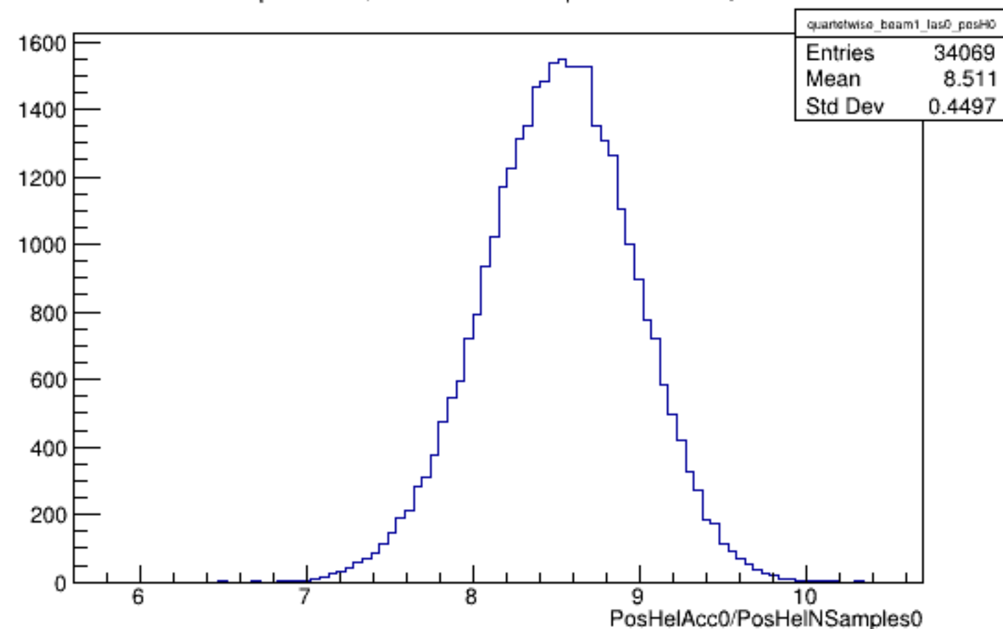
Run 4459 quartetwise, PosHelAcc0/NSamples0: Beam ON, Laser OFF
