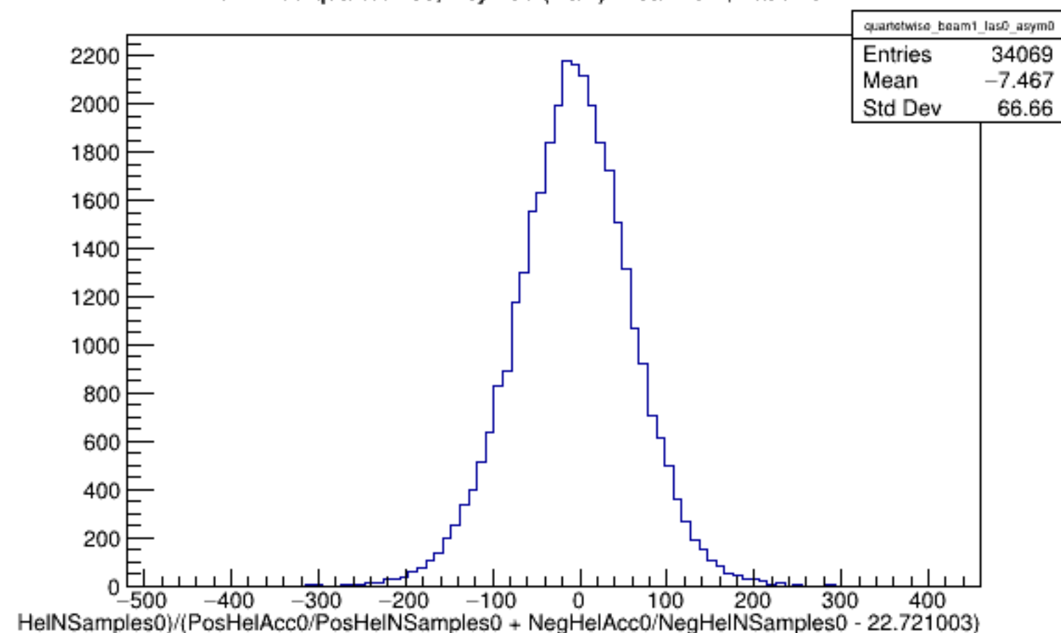
Run 4459 quartetwise, Asyms0 (Raw): Beam ON, Laser OFF
