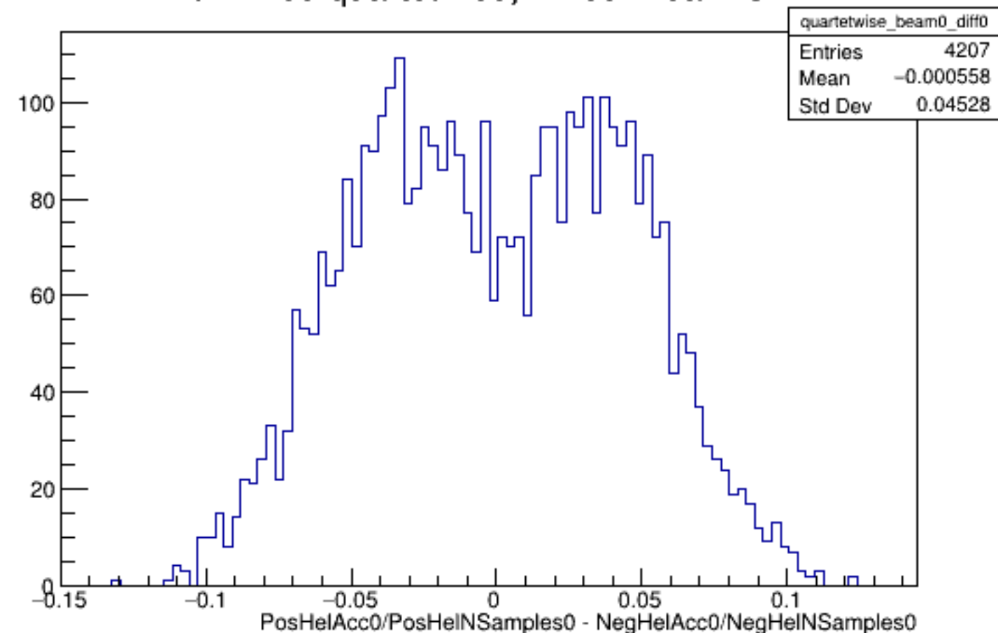
Run 4459 quartetwise, Diffs0: Beam OFF
