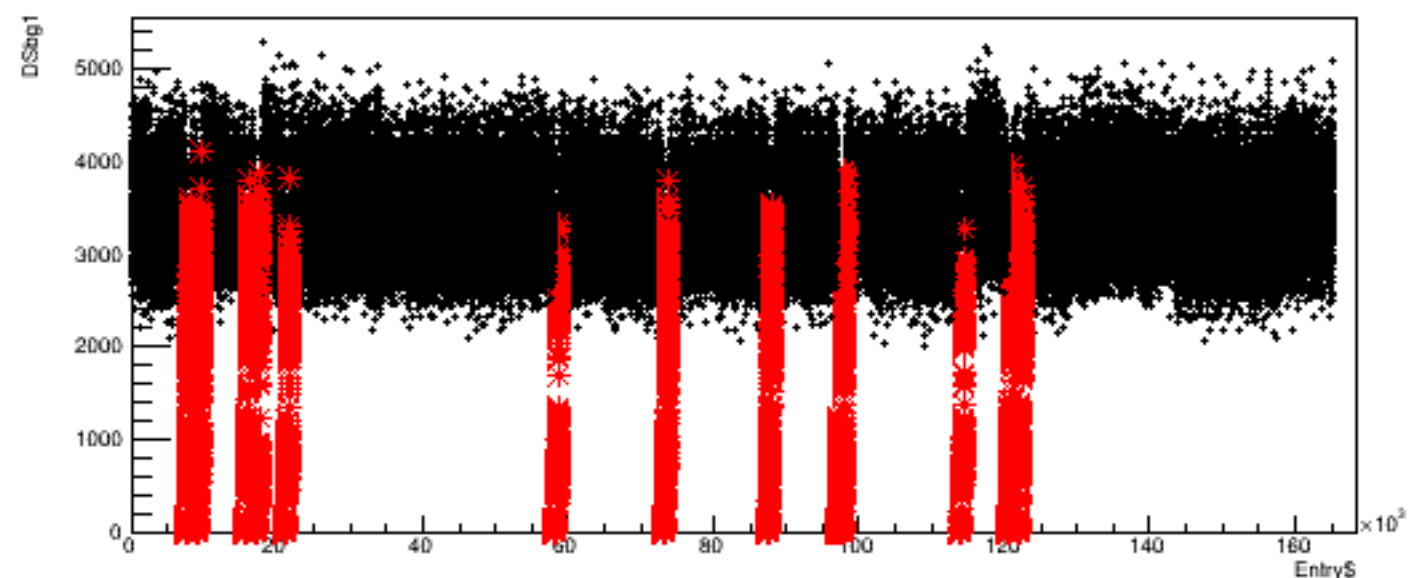
Run 4461, quartetwise: DSbg1 vs time
