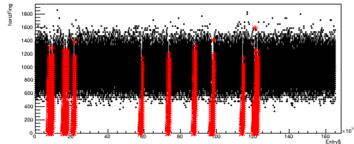
Run 4461, quartetwise: horizFing vs time
