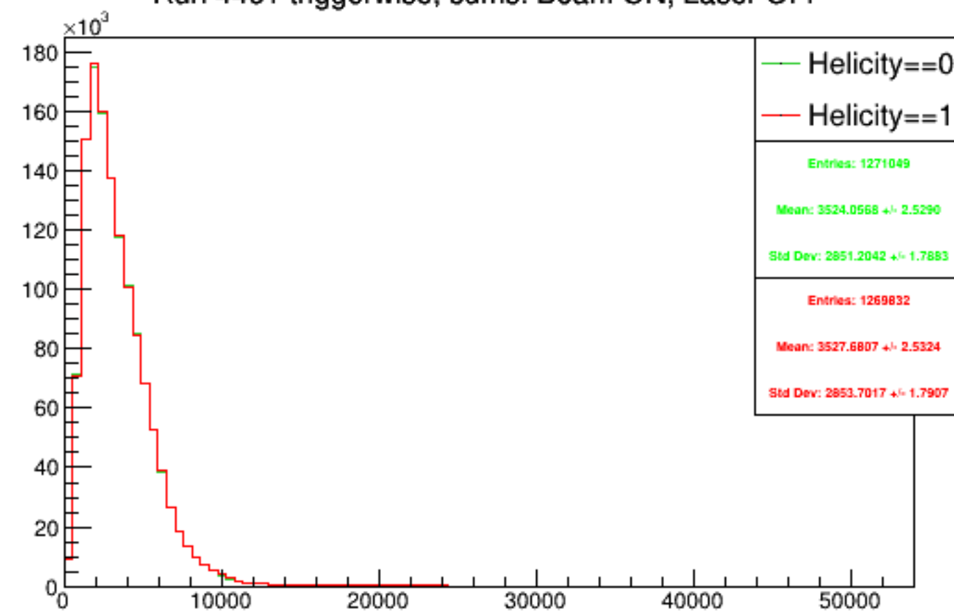
Run 4461 triggerwise, sums: Beam ON, Laser OFF
