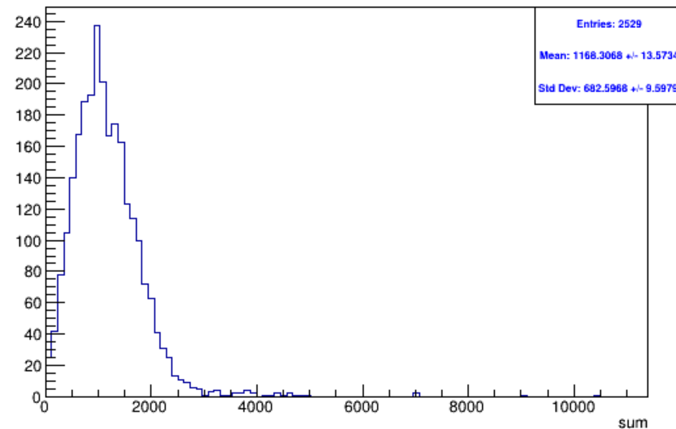
Run 4461 triggerwise, sums: Beam OFF
