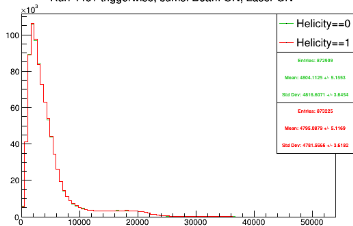
Run 4461 triggerwise, sums: Beam ON, Laser ON
