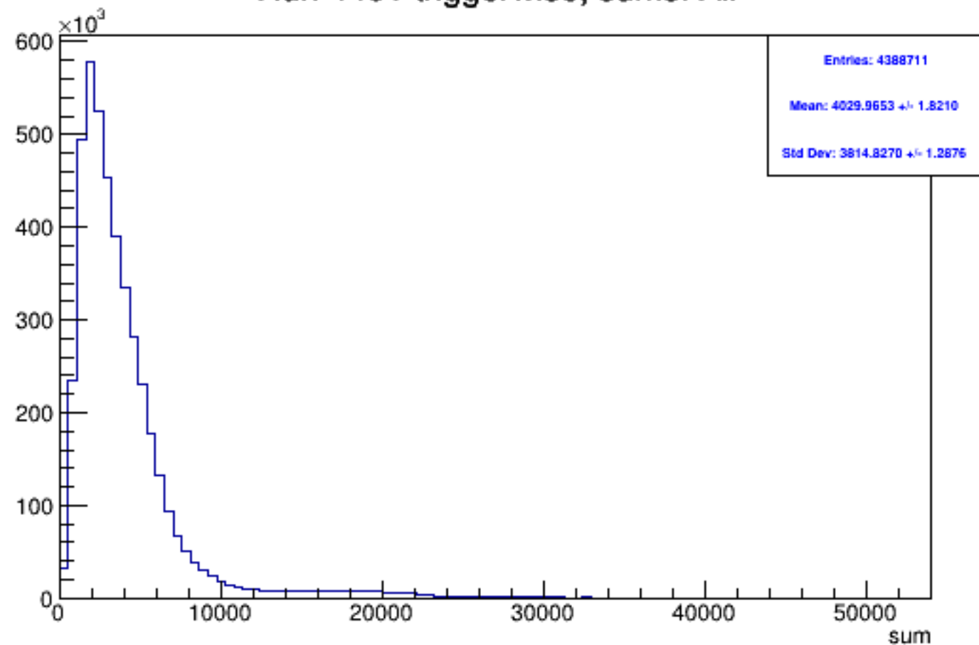
Run 4461 triggerwise, sums: All
