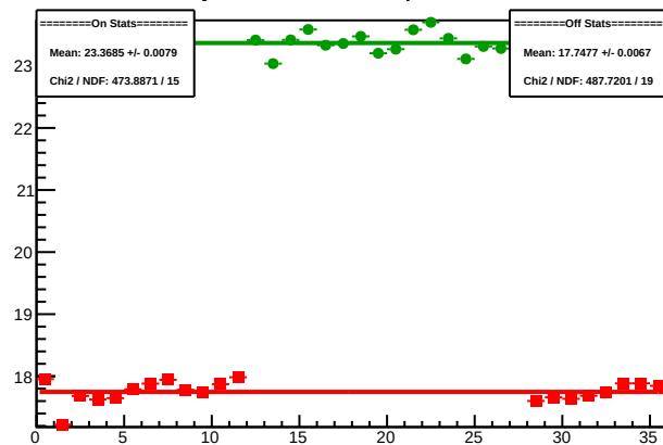
Cycle 4464.3: Multiplet Sums
