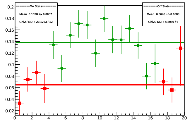
Cycle 4464.1: Multiplet Diffs
