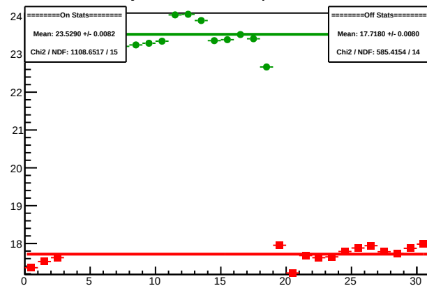
Cycle 4464.2: Multiplet Sums
