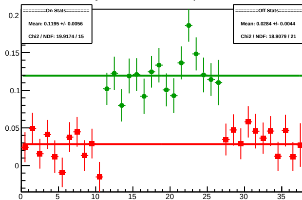
Cycle 4464.11: Multiplet Diffs
