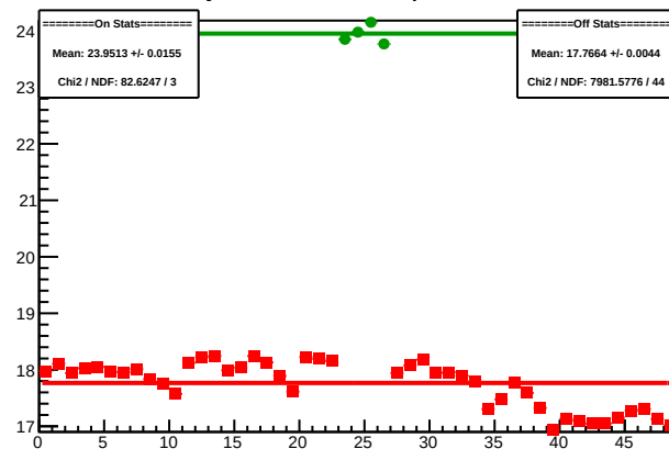
Cycle 4464.8: Multiplet Sums
