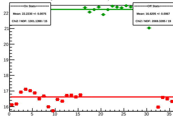
Cycle 4464.13: Multiplet Sums
