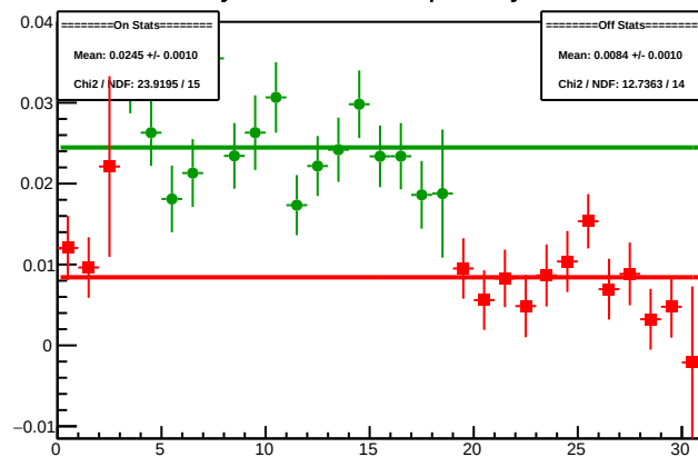
Cycle 4464.2: Multiplet Asyms
