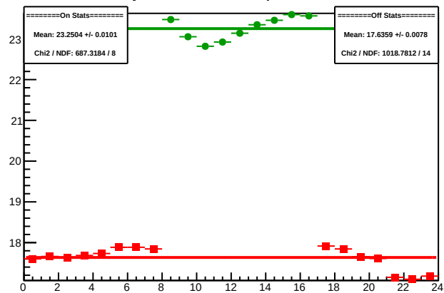
Cycle 4464.4: Multiplet Sums
