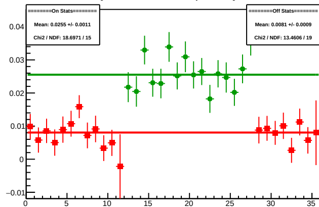
Cycle 4464.3: Multiplet Asyms
