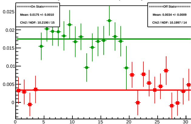
Cycle 4464.10: Multiplet Asyms
