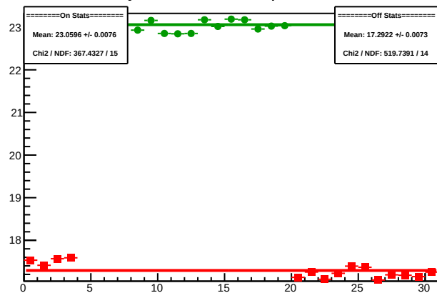
Cycle 4464.10: Multiplet Sums
