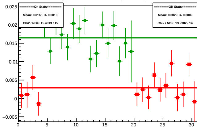
Cycle 4464.6: Multiplet Asyms
