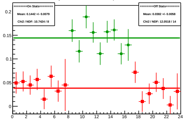
Cycle 4464.4: Multiplet Diffs
