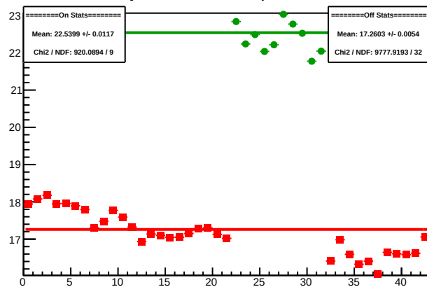
Cycle 4464.9: Multiplet Sums
