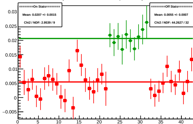
Cycle 4464.9: Multiplet Asyms
