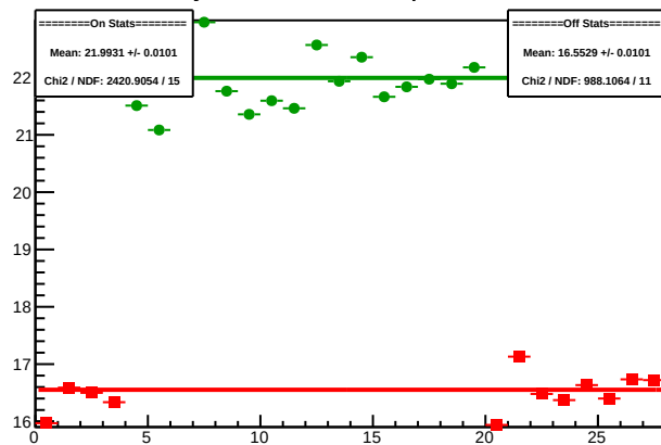
Cycle 4464.14: Multiplet Sums
