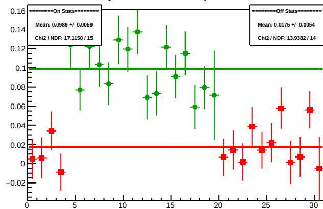
Cycle 4464.6: Multiplet Diffs
