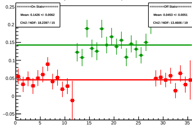
Cycle 4464.3: Multiplet Diffs
