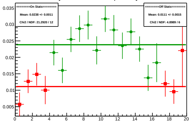
Cycle 4464.1: Multiplet Asyms
