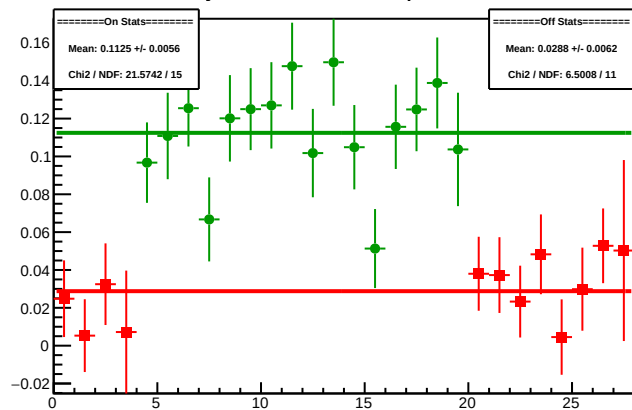
Cycle 4464.14: Multiplet Diffs
