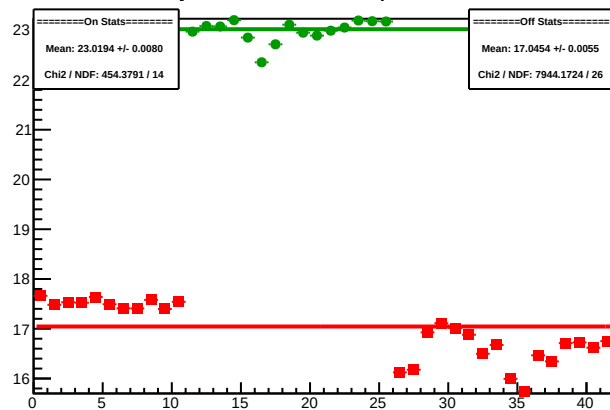
Cycle 4464.12: Multiplet Sums
