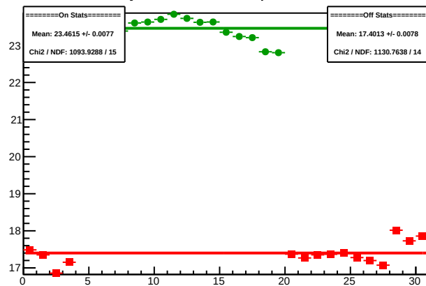
Cycle 4464.6: Multiplet Sums
