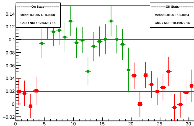
Cycle 4464.10: Multiplet Diffs
