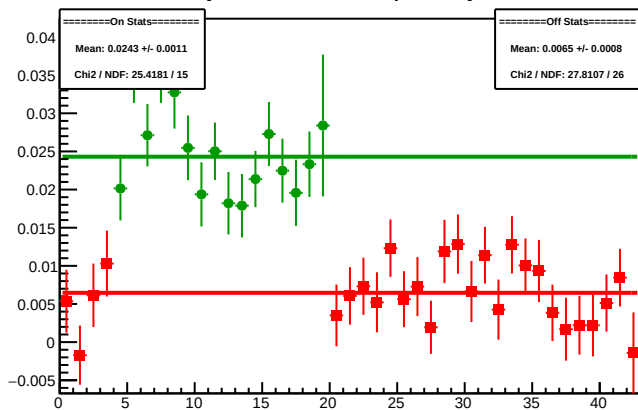
Cycle 4464.7: Multiplet Asyms
