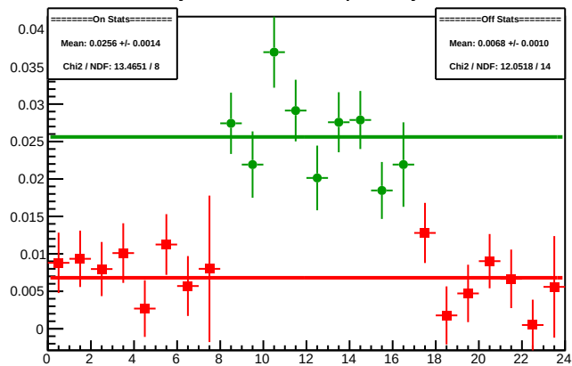
Cycle 4464.4: Multiplet Asyms
