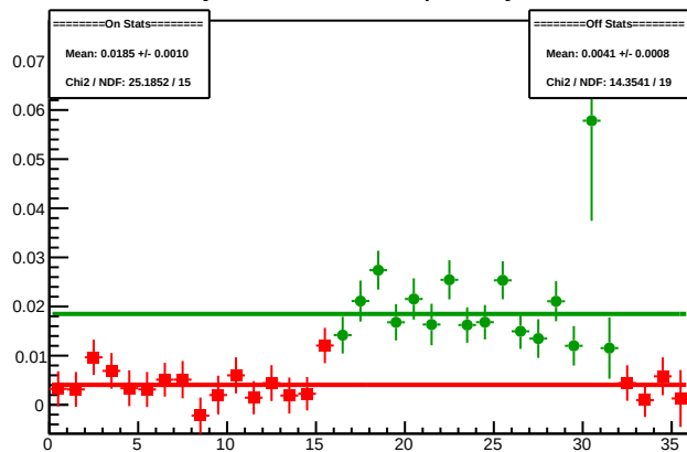
Cycle 4464.13: Multiplet Asyms
