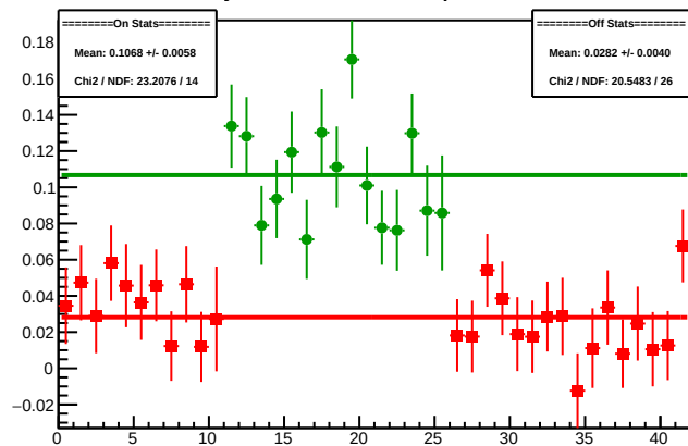
Cycle 4464.12: Multiplet Diffs
