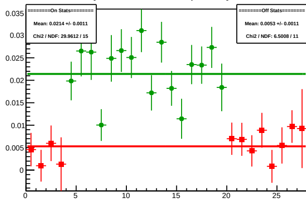
Cycle 4464.14: Multiplet Asyms
