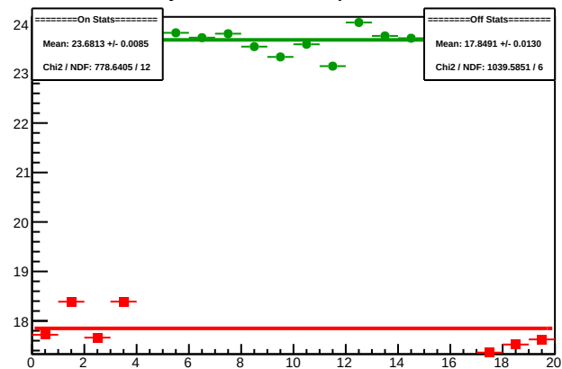
Cycle 4464.1: Multiplet Sums
