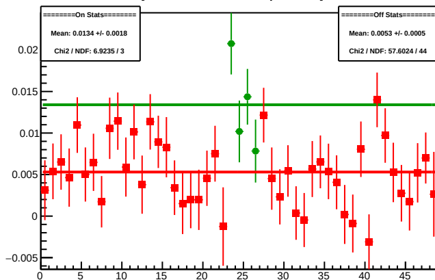
Cycle 4464.8: Multiplet Asyms
