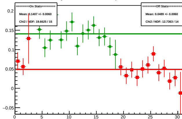
Cycle 4464.2: Multiplet Diffs
