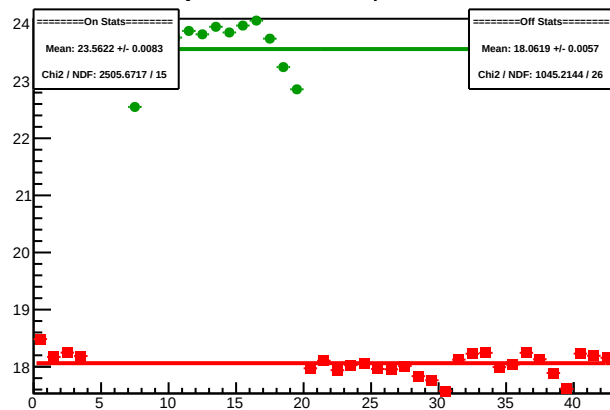
Cycle 4464.7: Multiplet Sums
