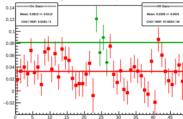
Cycle 4464.8: Multiplet Diffs
