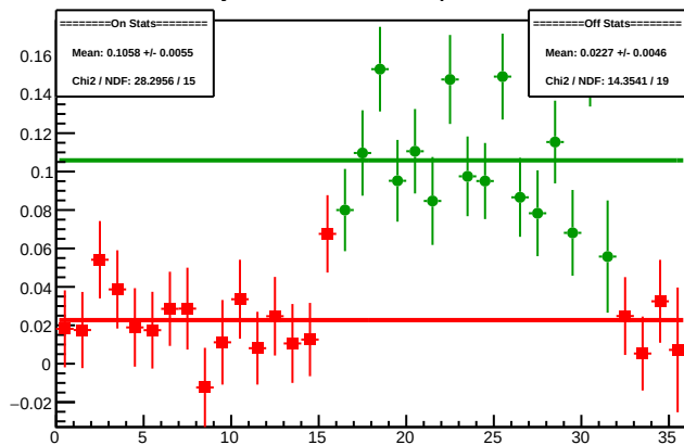
Cycle 4464.13: Multiplet Diffs
