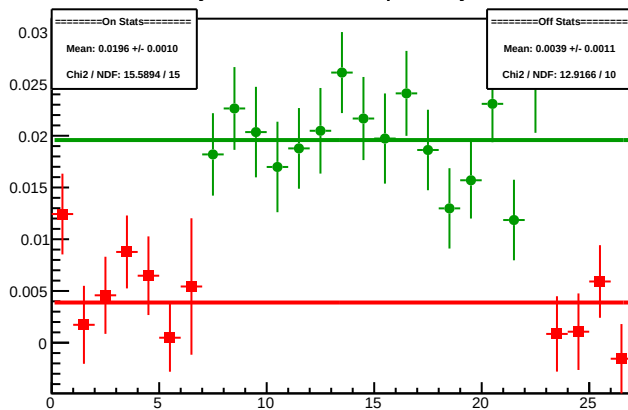
Cycle 4464.5: Multiplet Asyms
