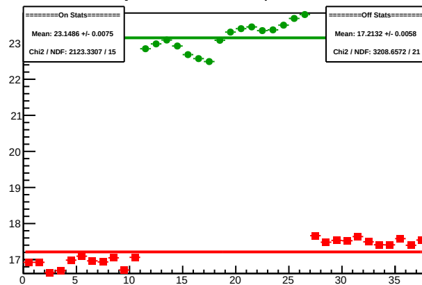
Cycle 4464.11: Multiplet Sums
