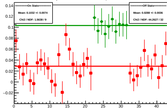
Cycle 4464.9: Multiplet Diffs
