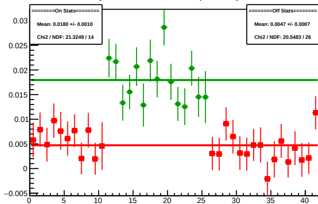
Cycle 4464.12: Multiplet Asyms
