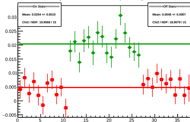
Cycle 4464.11: Multiplet Asyms
