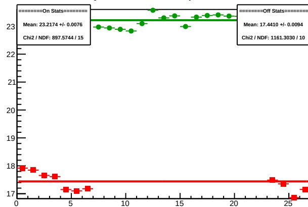
Cycle 4464.5: Multiplet Sums
