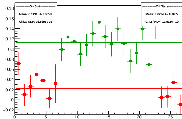
Cycle 4464.5: Multiplet Diffs
