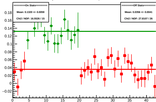
Cycle 4464.7: Multiplet Diffs
