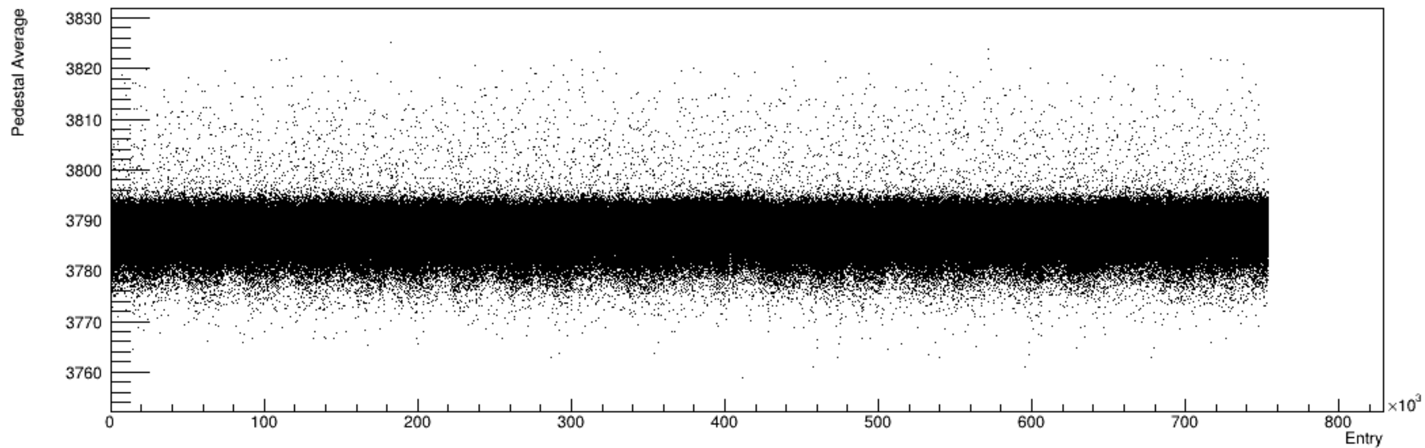
Run 4464, snapshots: Pedestal vs. Time
