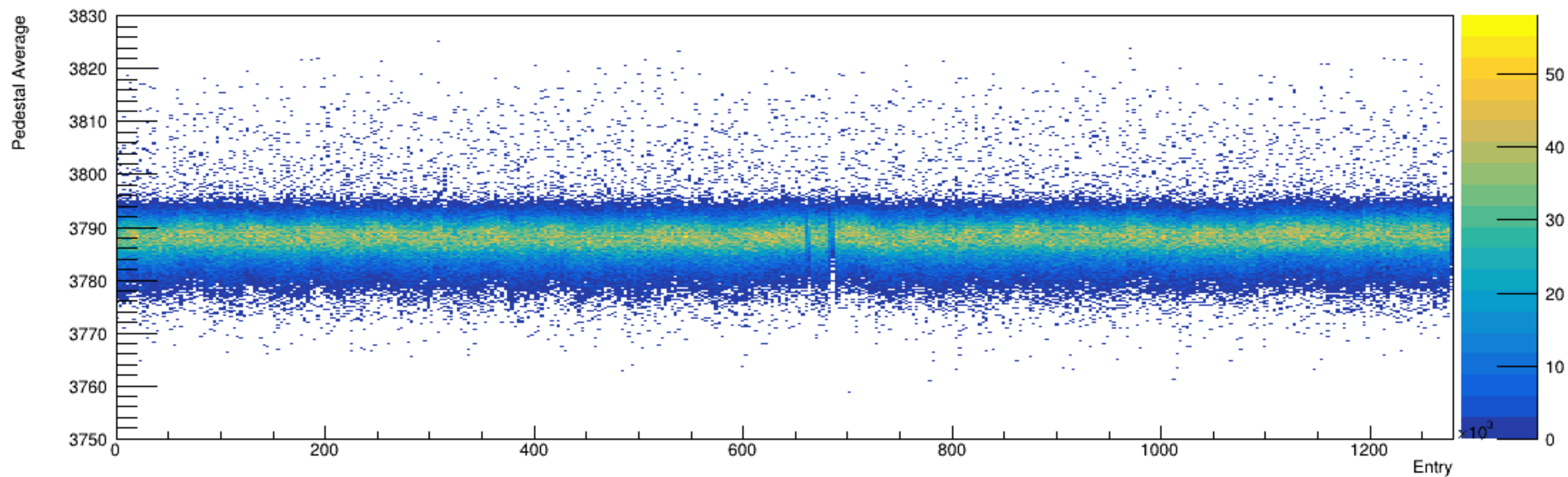
Run 4464, snapshots: Pedestal vs. Time
