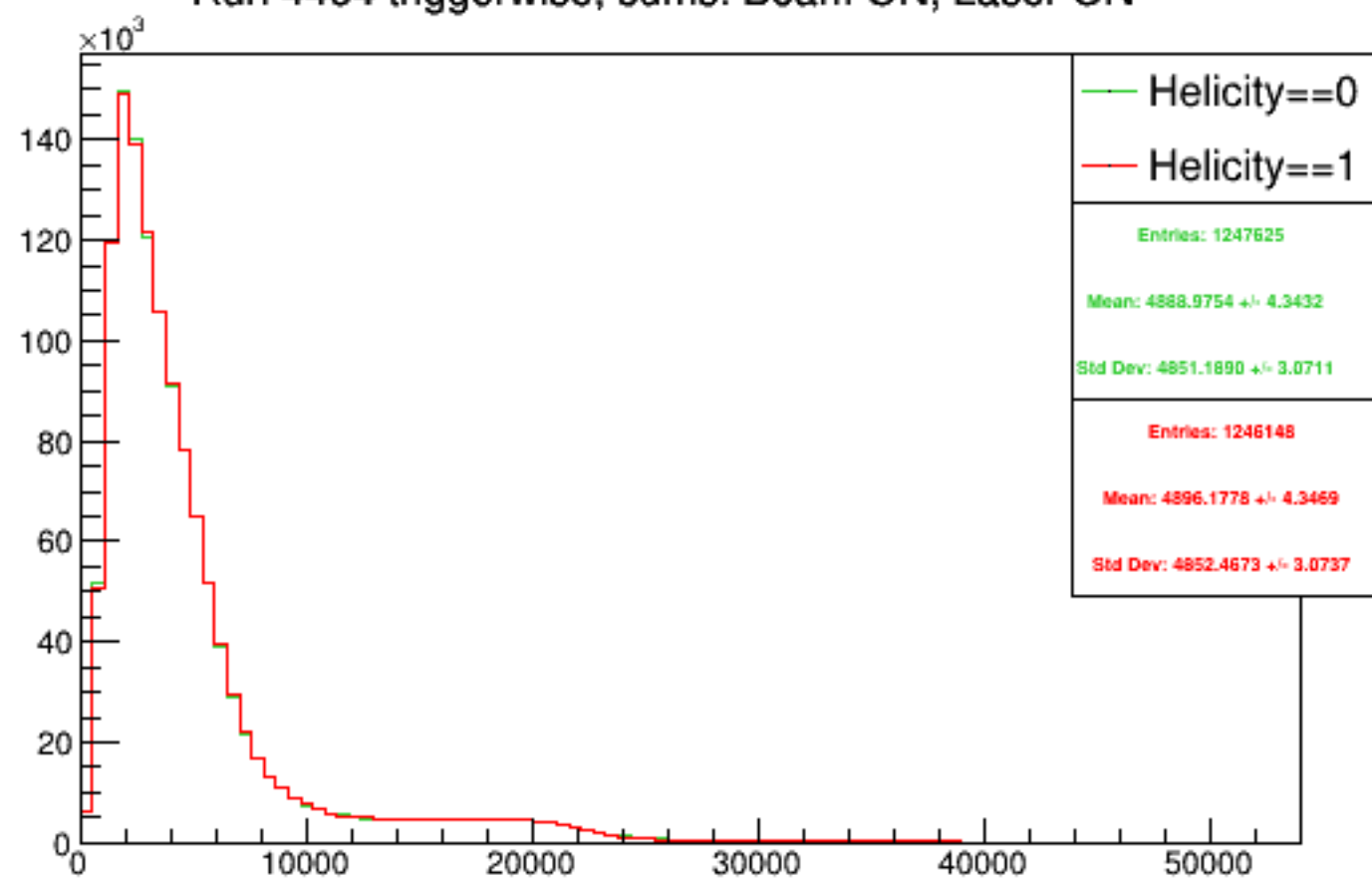
Run 4464 triggerwise, sums: Beam ON, Laser ON
