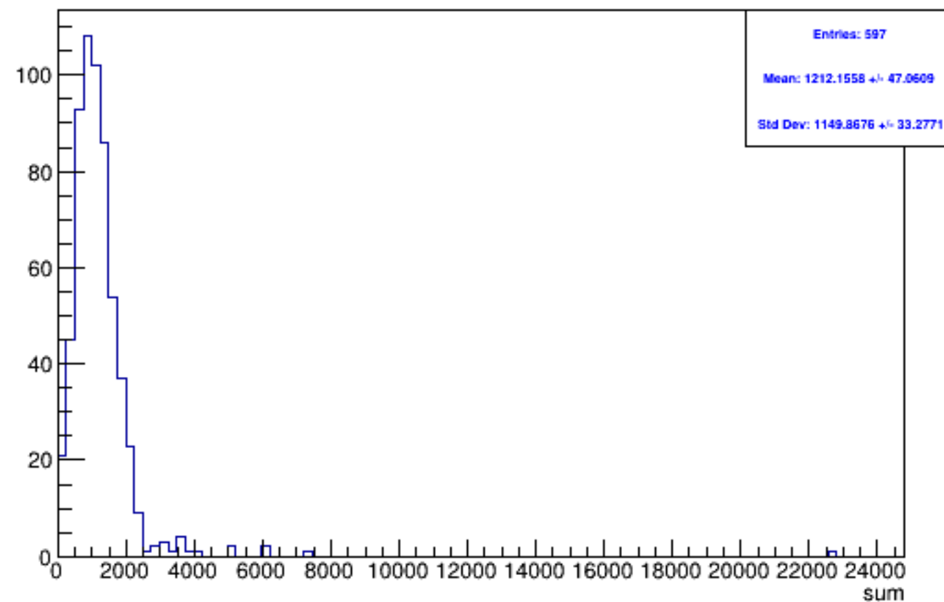
Run 4464 triggerwise, sums: Beam OFF
