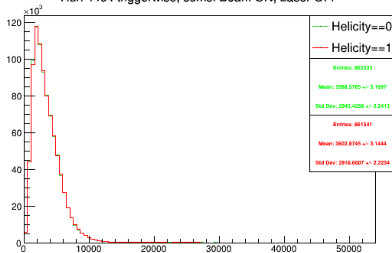
Run 4464 triggerwise, sums: Beam ON, Laser OFF
