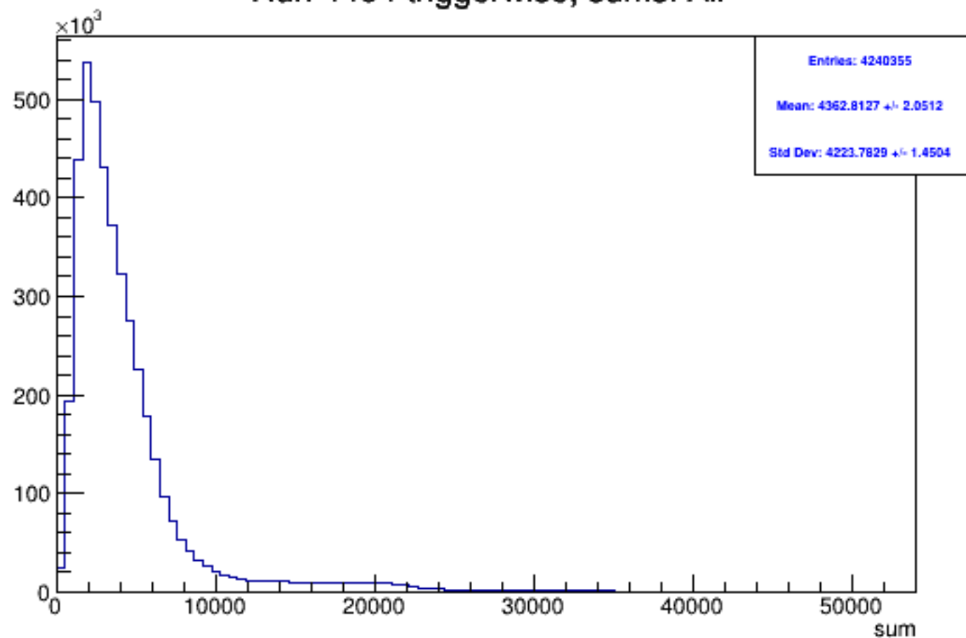
Run 4464 triggerwise, sums: All
