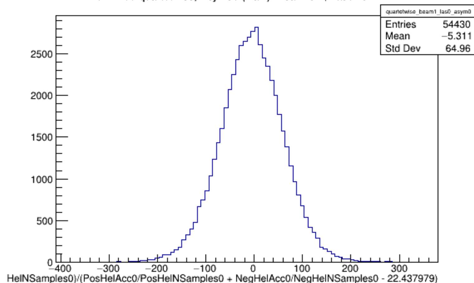
Run 4465 quartetwise, Asyms0 (Raw): Beam ON, Laser OFF
