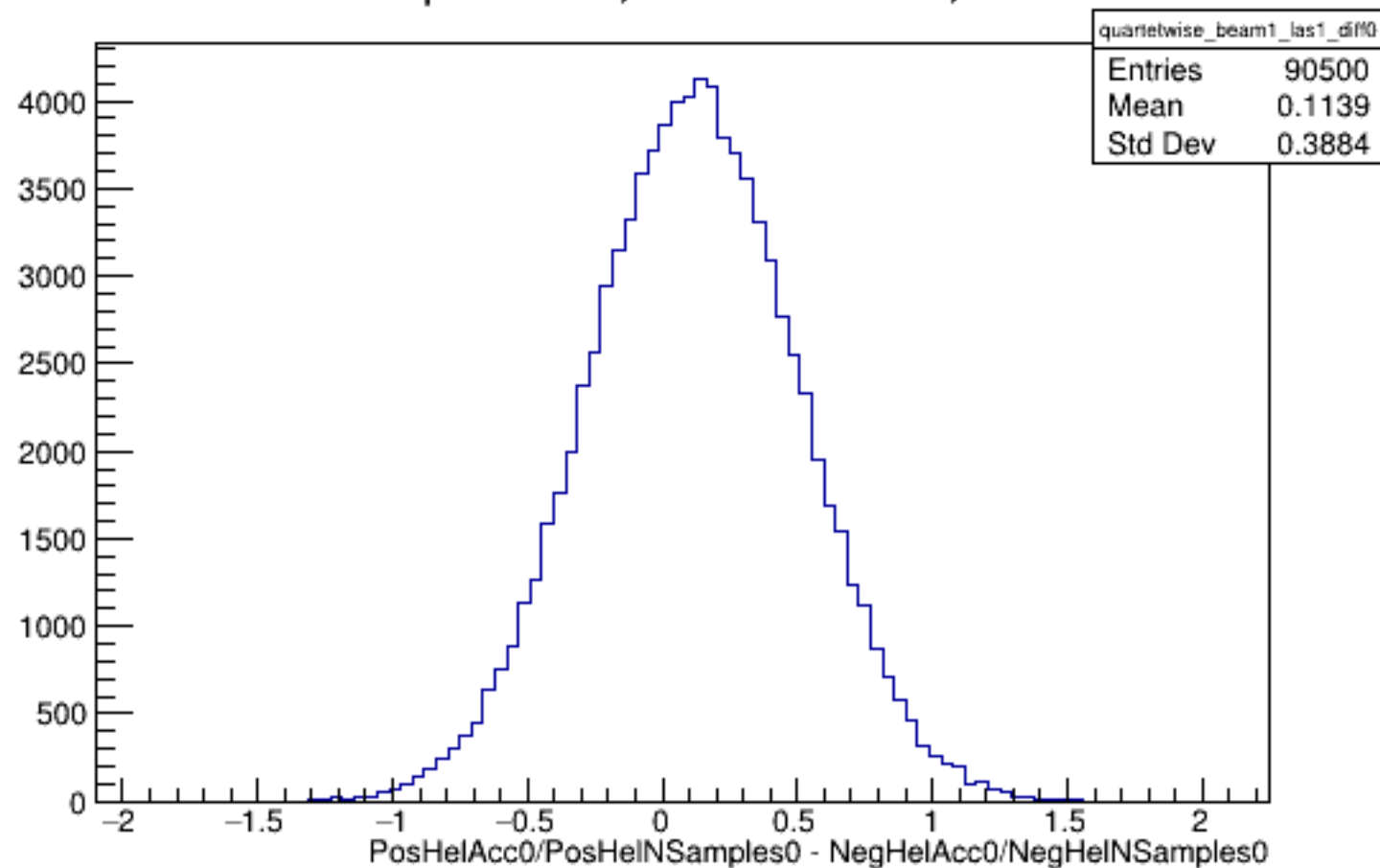
Run 4465 quartetwise, Diffs0: Beam ON, Laser ON
