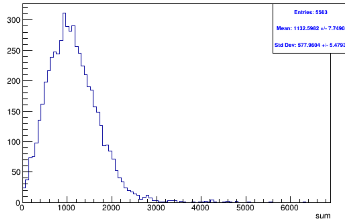
Run 4465 triggerwise, sums: Beam OFF
