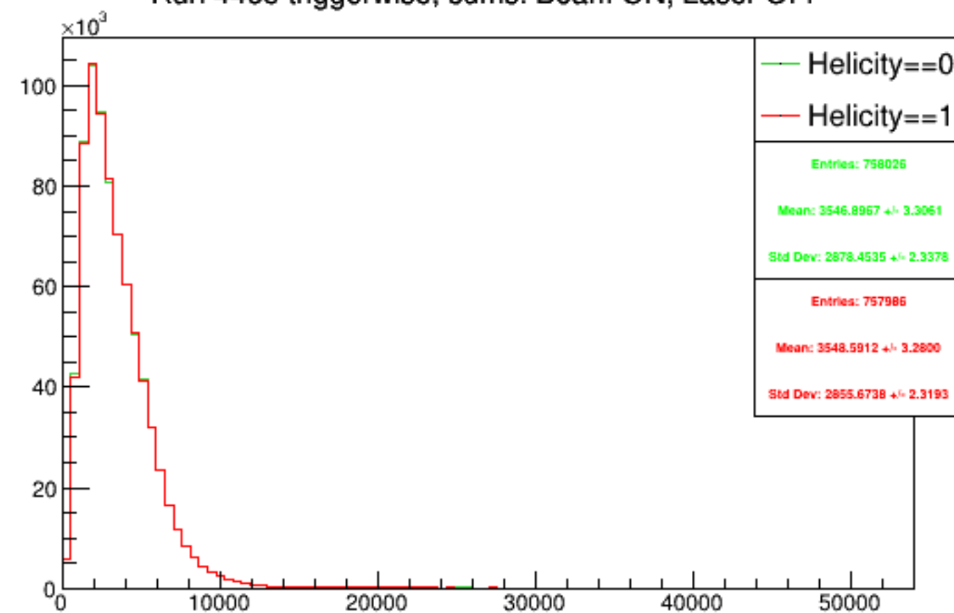
Run 4465 triggerwise, sums: Beam ON, Laser OFF
