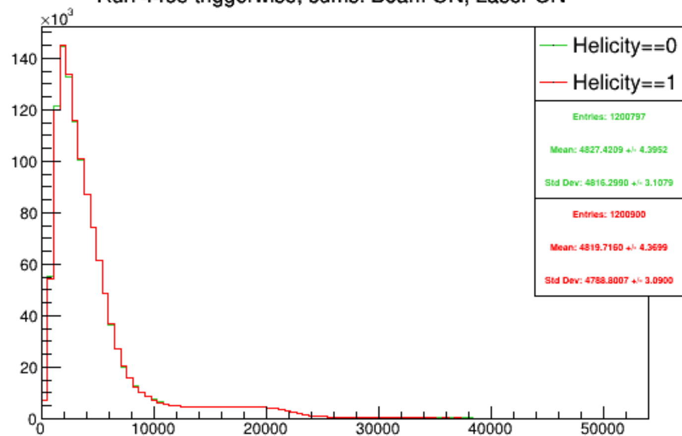
Run 4465 triggerwise, sums: Beam ON, Laser ON
