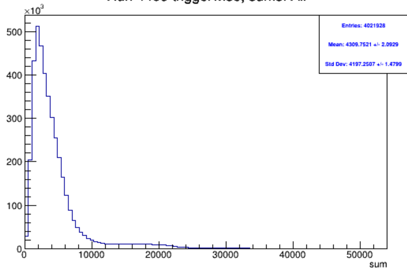
Run 4465 triggerwise, sums: All
