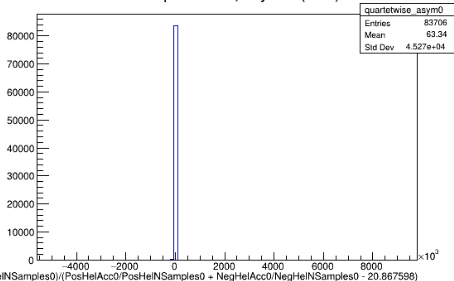
Run 4471 quartetwise, Asyms0 (Raw): All
