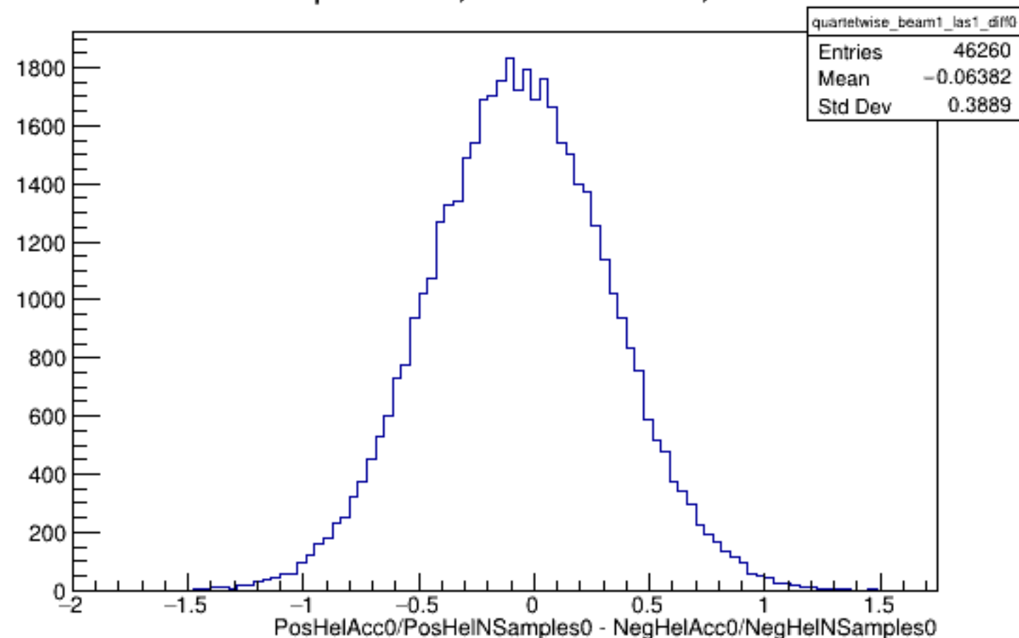
Run 4471 quartetwise, Diffs0: Beam ON, Laser ON
