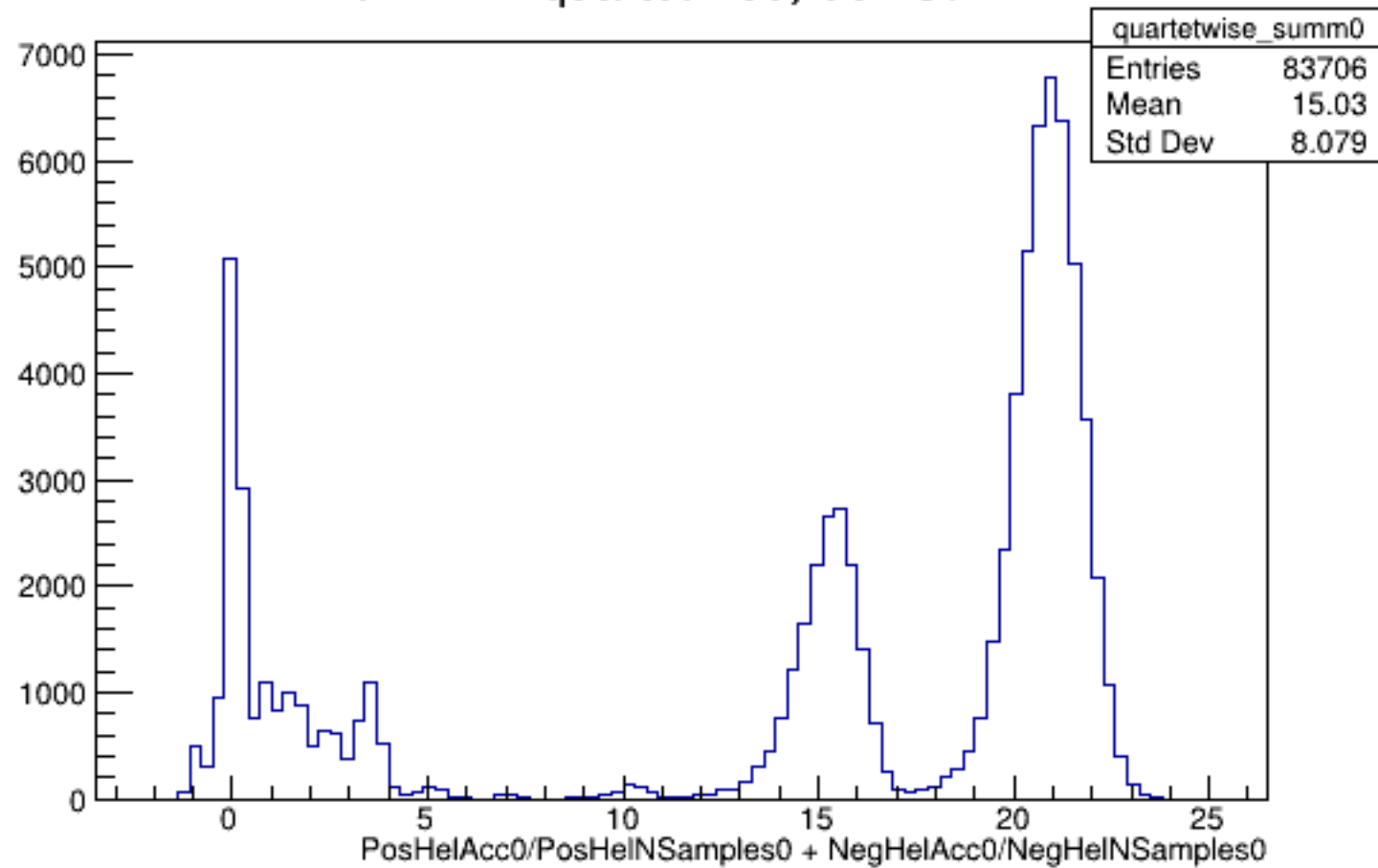
Run 4471 quartetwise, Sums0: All
