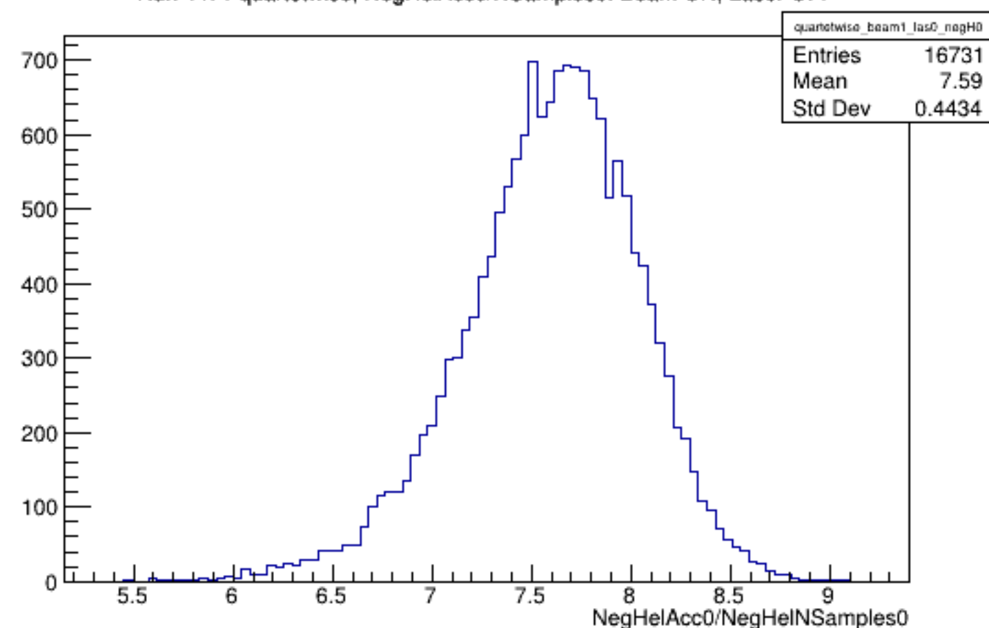
Run 4471 quartetwise, NegHelAcc0/NSamples0: Beam ON, Laser OFF
