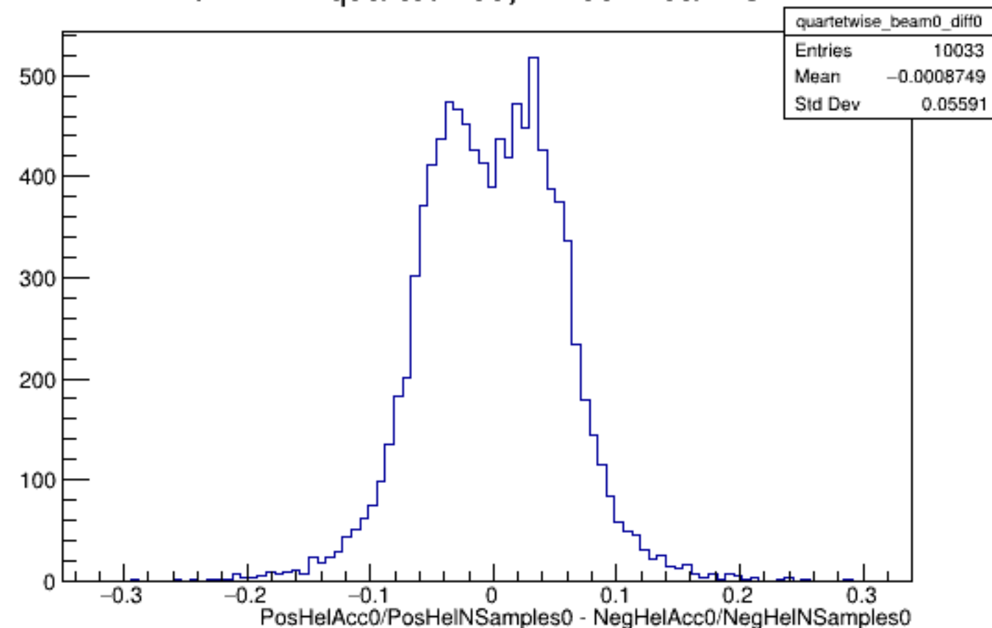
Run 4471 quartetwise, Diffs0: Beam OFF
