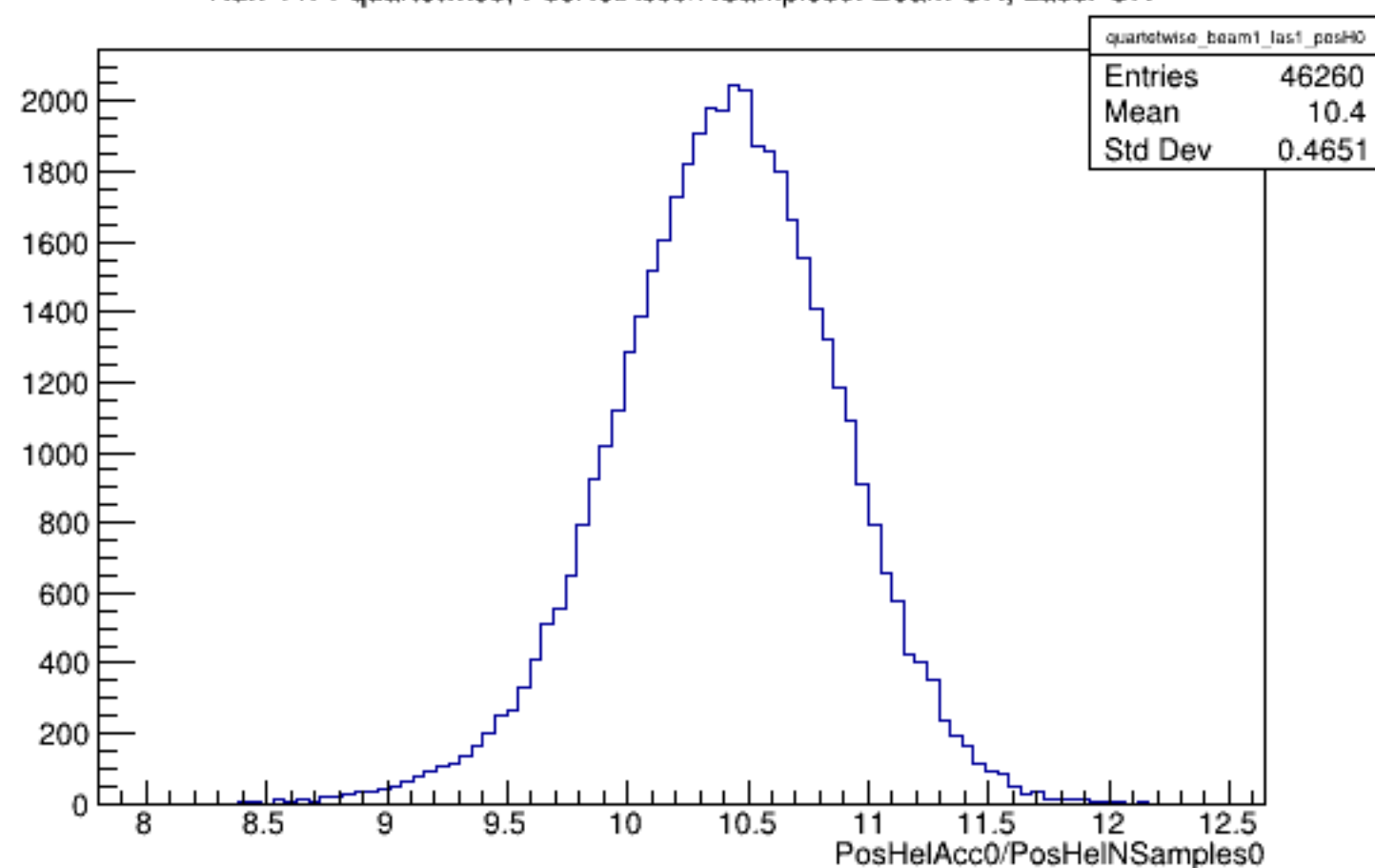
Run 4471 quartetwise, PosHelAcc0/NSamples0: Beam ON, Laser ON
