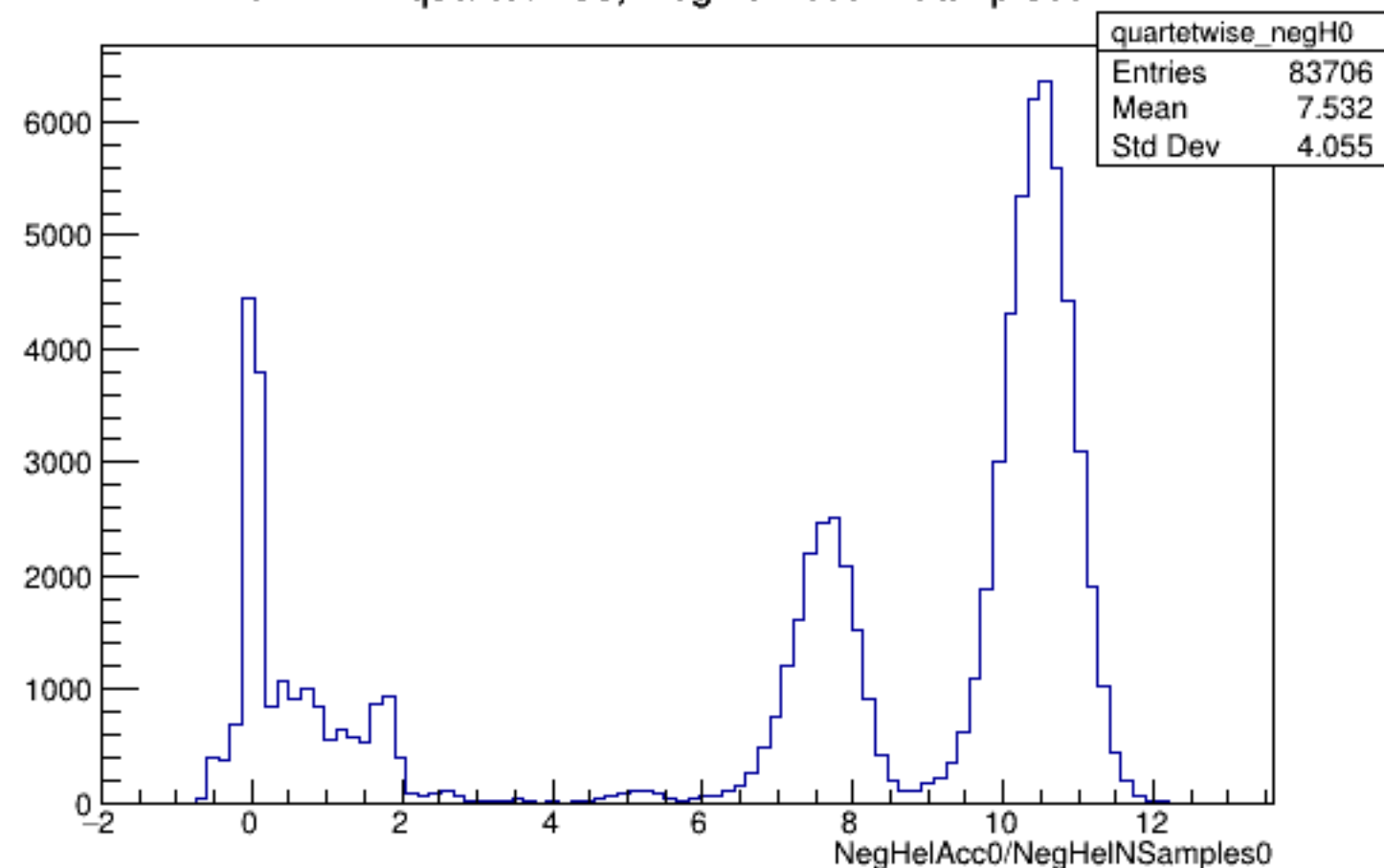
Run 4471 quartetwise, NegHelAcc0/NSamples0: All
