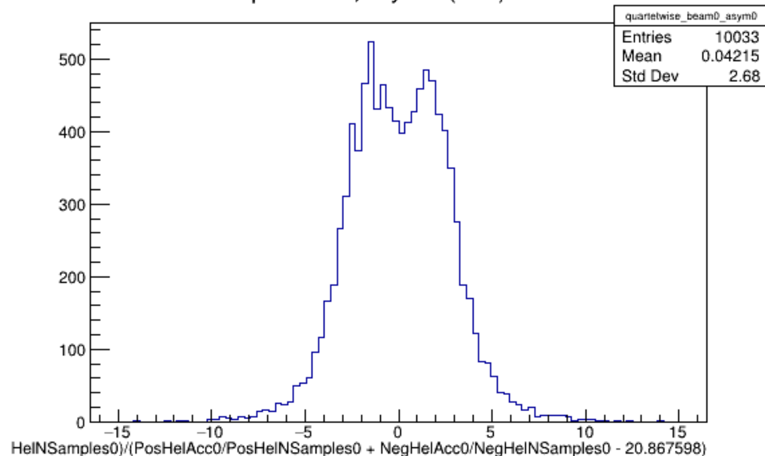
Run 4471 quartetwise, Asyms0 (Raw): Beam OFF
