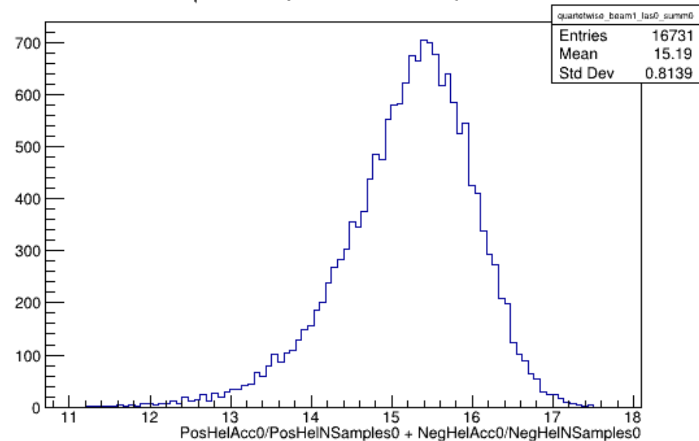
Run 4471 quartetwise, Sums0: Beam ON, Laser OFF
