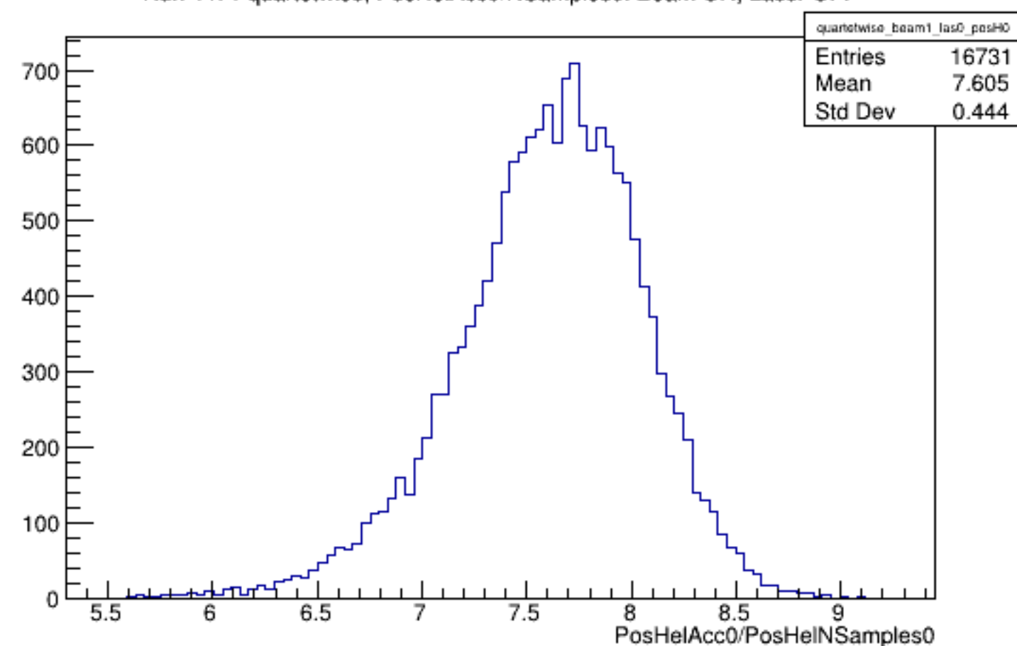
Run 4471 quartetwise, PosHelAcc0/NSamples0: Beam ON, Laser OFF
