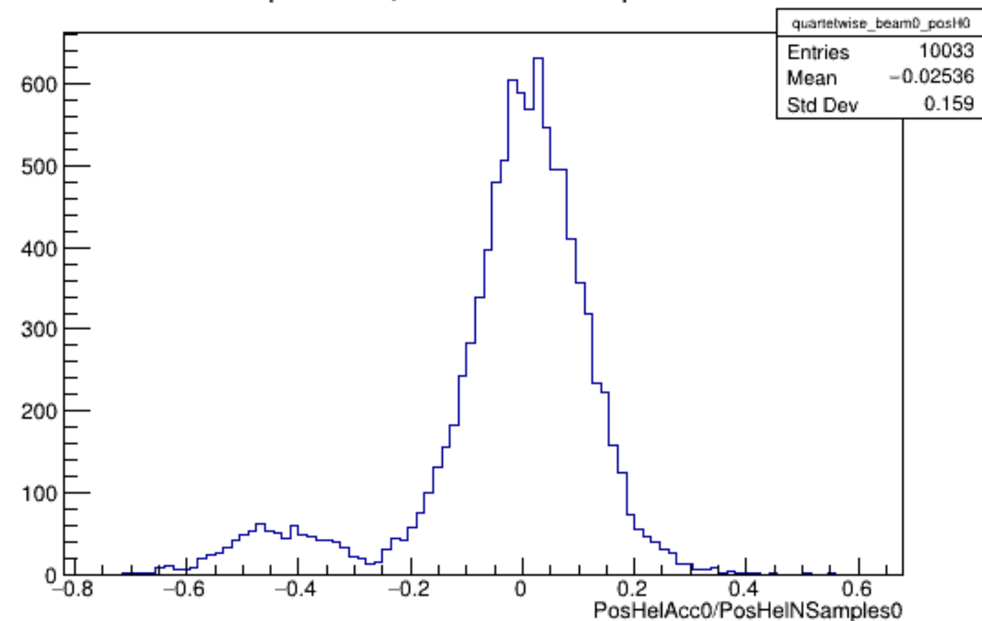
Run 4471 quartetwise, PosHelAcc0/NSamples0: Beam OFF
