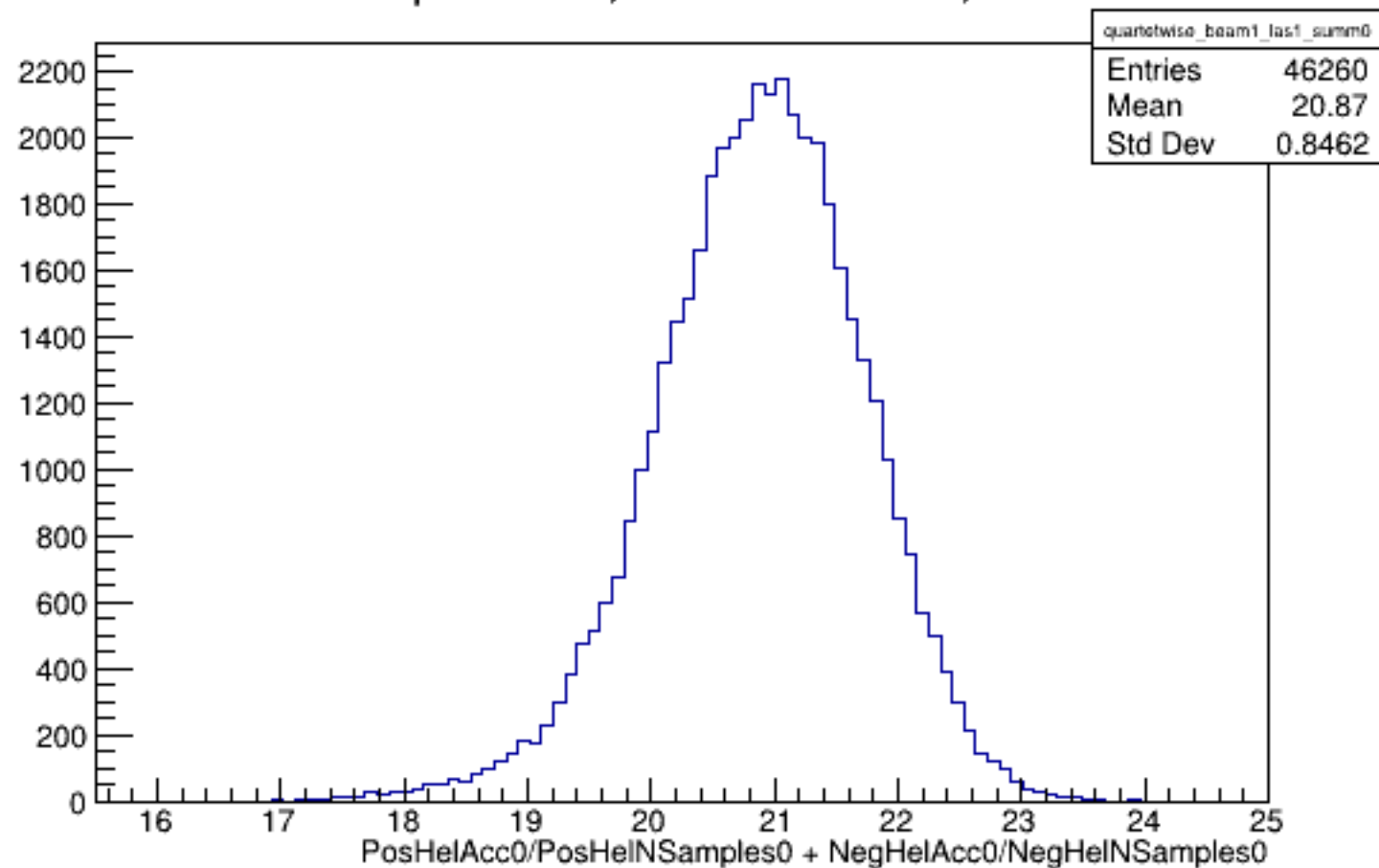
Run 4471 quartetwise, Sums0: Beam ON, Laser ON
