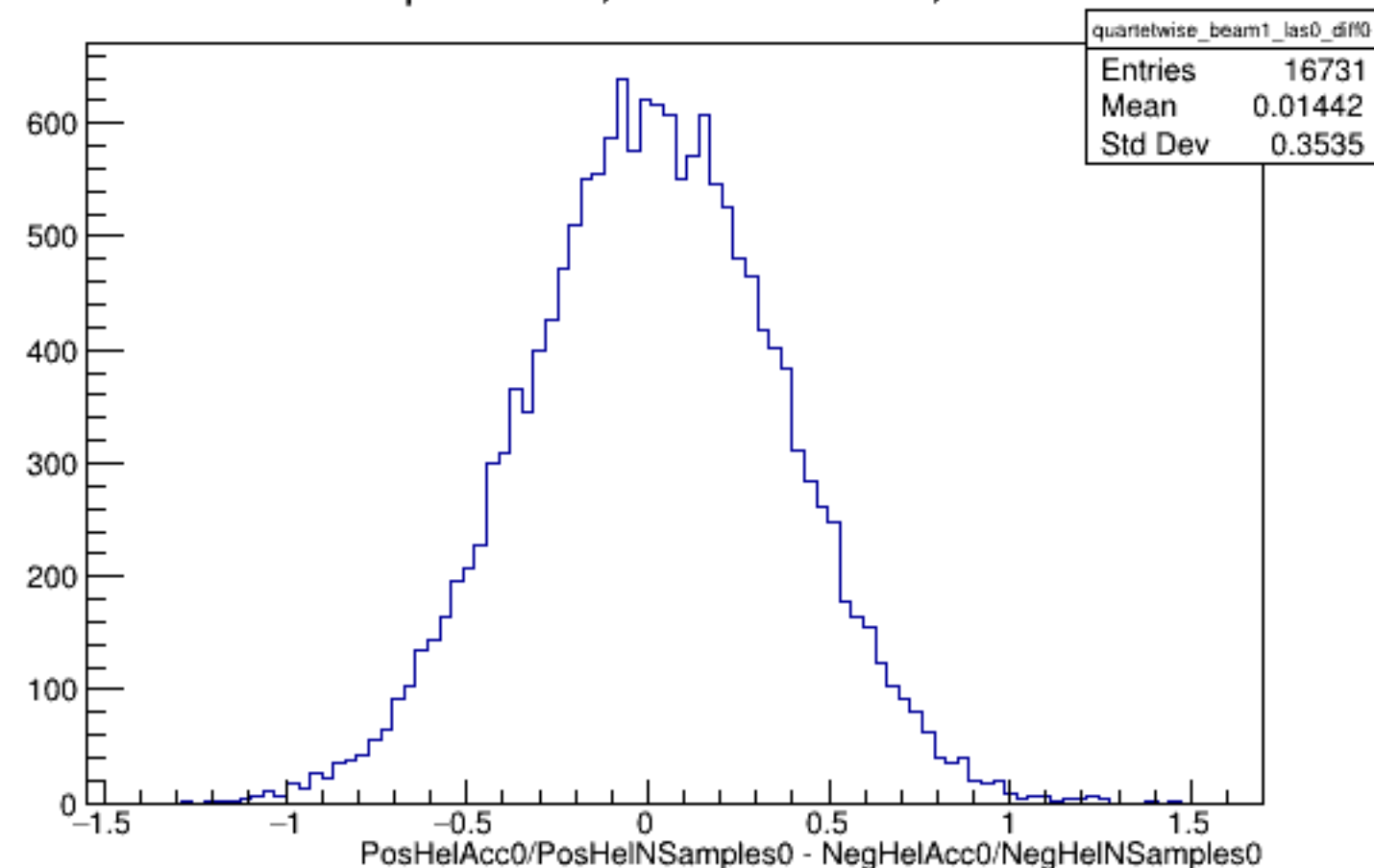
Run 4471 quartetwise, Diffs0: Beam ON, Laser OFF
