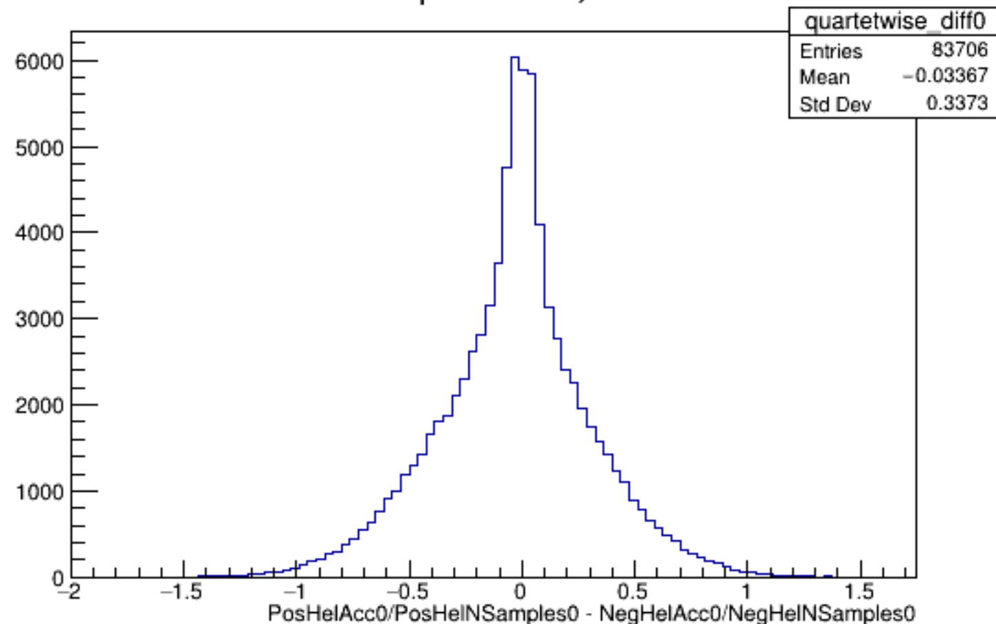
Run 4471 quartetwise, Diffs0: All
