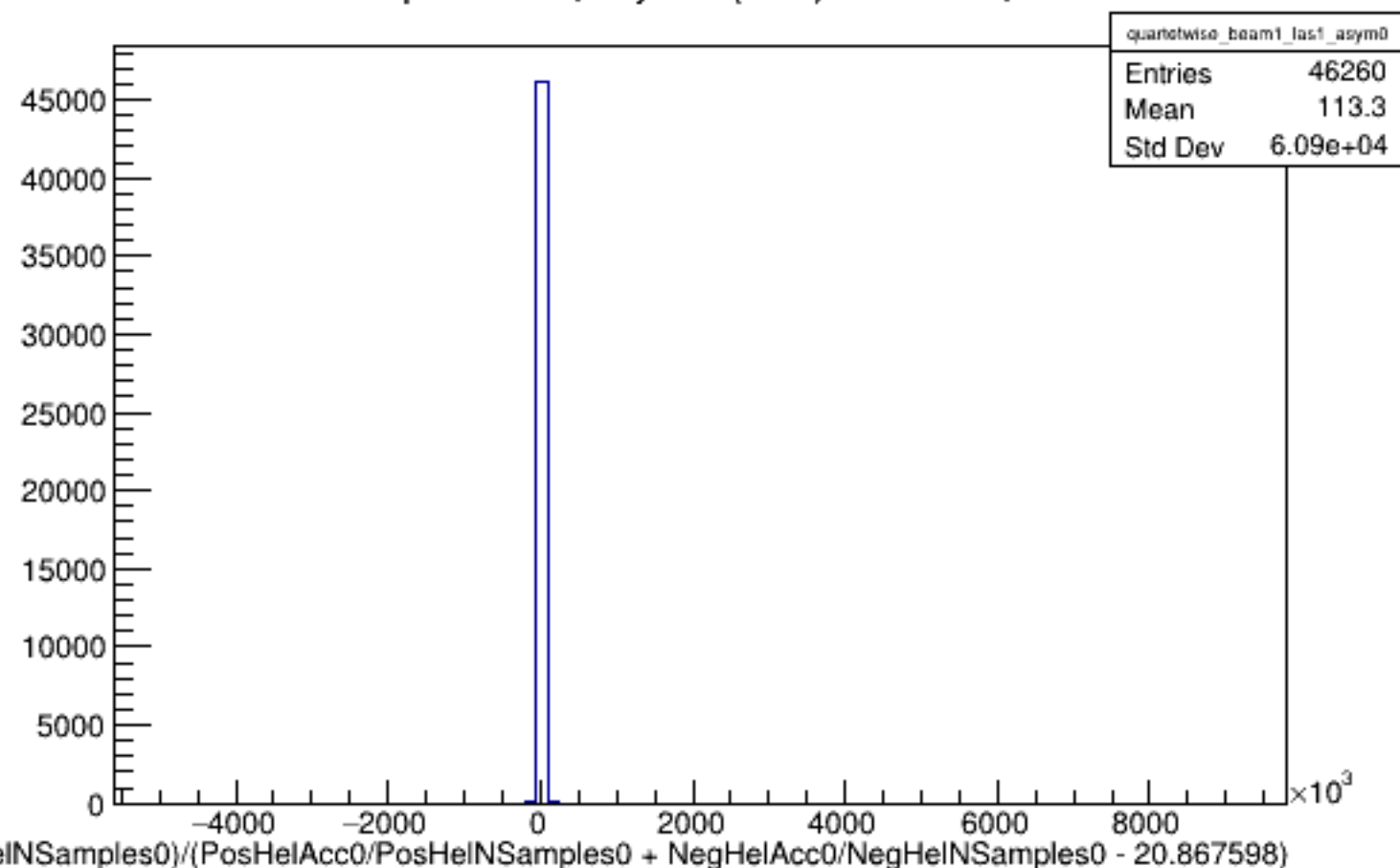
Run 4471 quartetwise, Asyms0 (Raw): Beam ON, Laser ON
