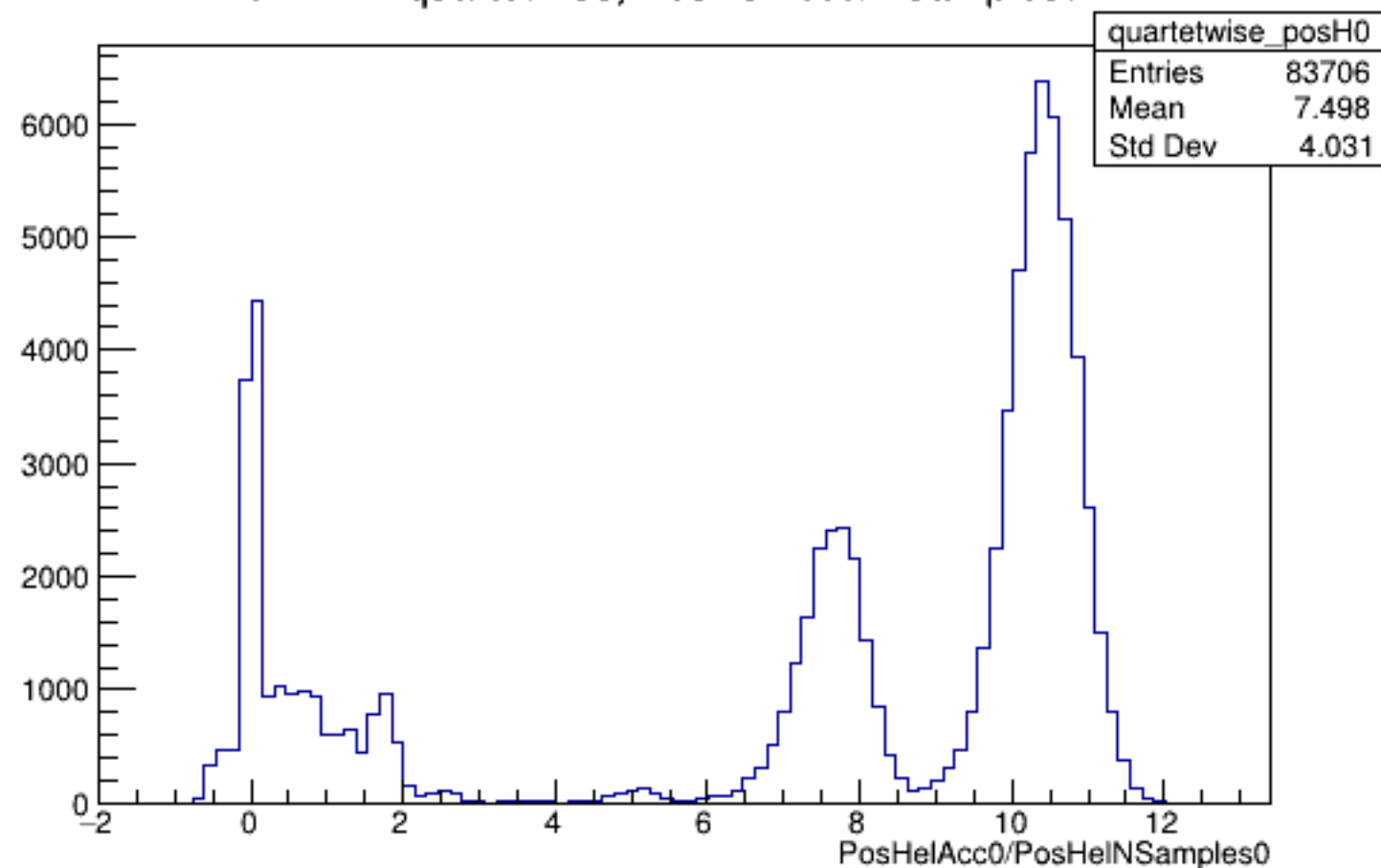
Run 4471 quartetwise, PosHelAcc0/NSamples0: All
