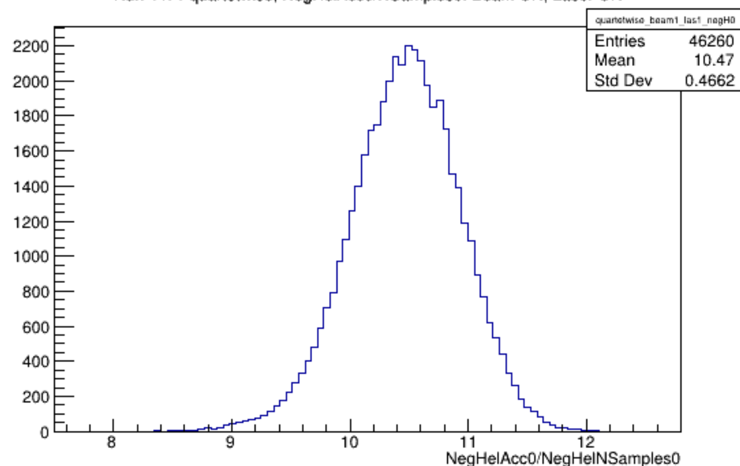
Run 4471 quartetwise, NegHelAcc0/NSamples0: Beam ON, Laser ON
