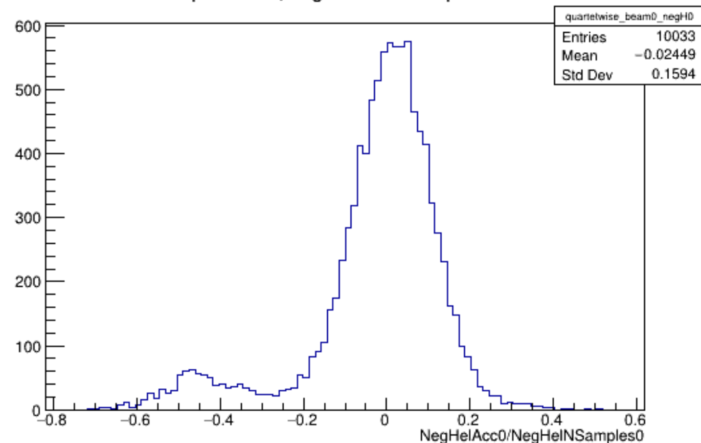
Run 4471 quartetwise, NegHelAcc0/NSamples0: Beam OFF
