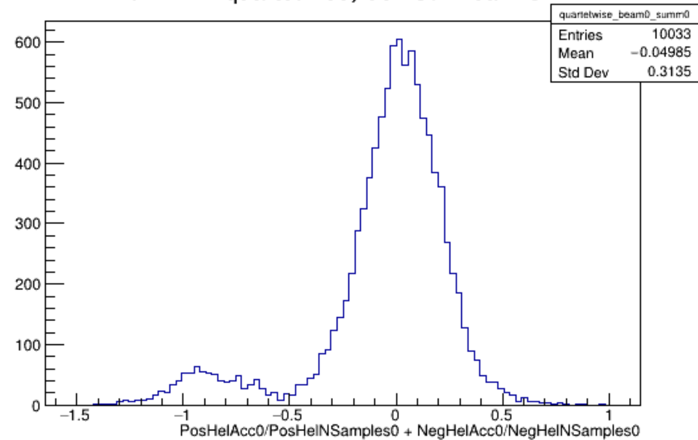
Run 4471 quartetwise, Sums0: Beam OFF
