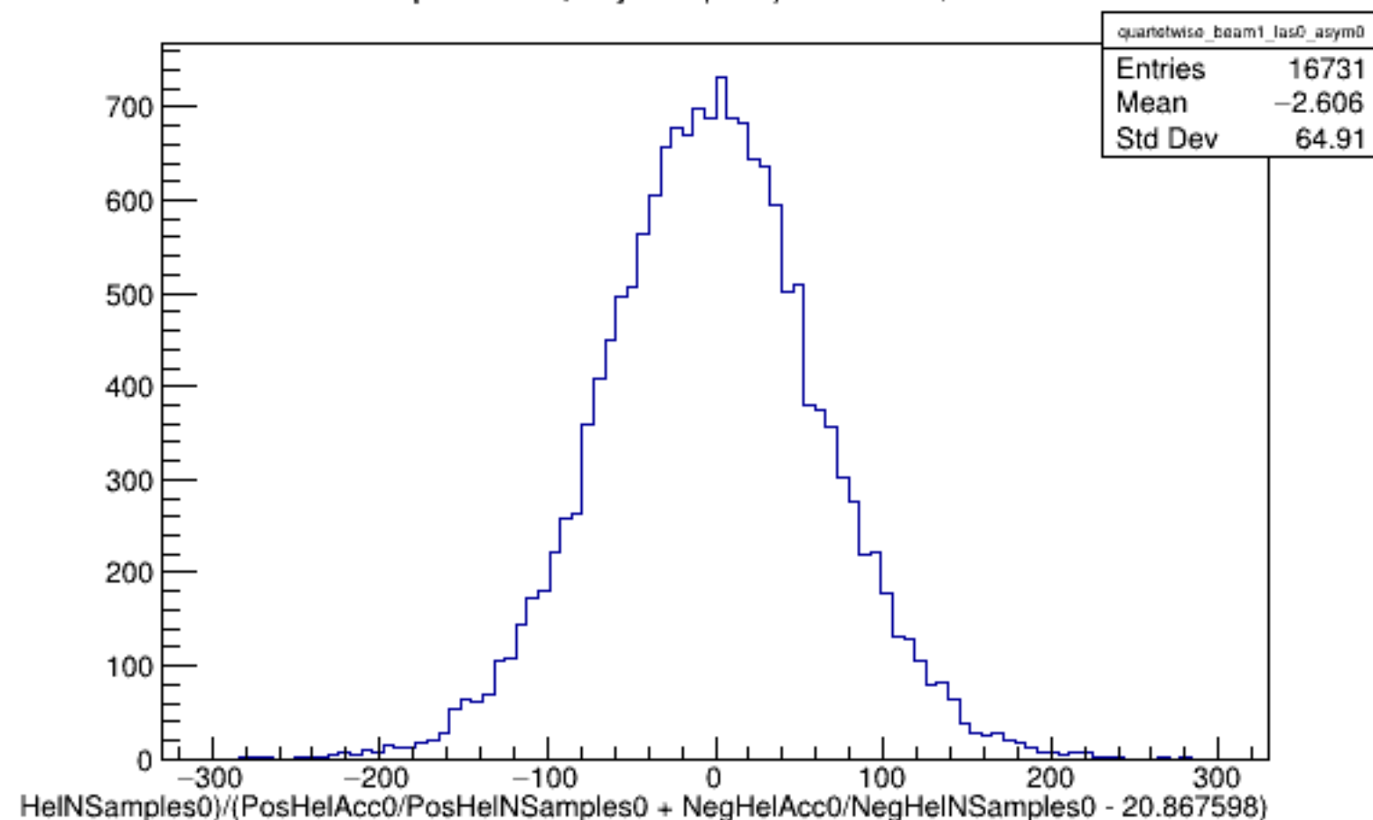
Run 4471 quartetwise, Asyms0 (Raw): Beam ON, Laser OFF
