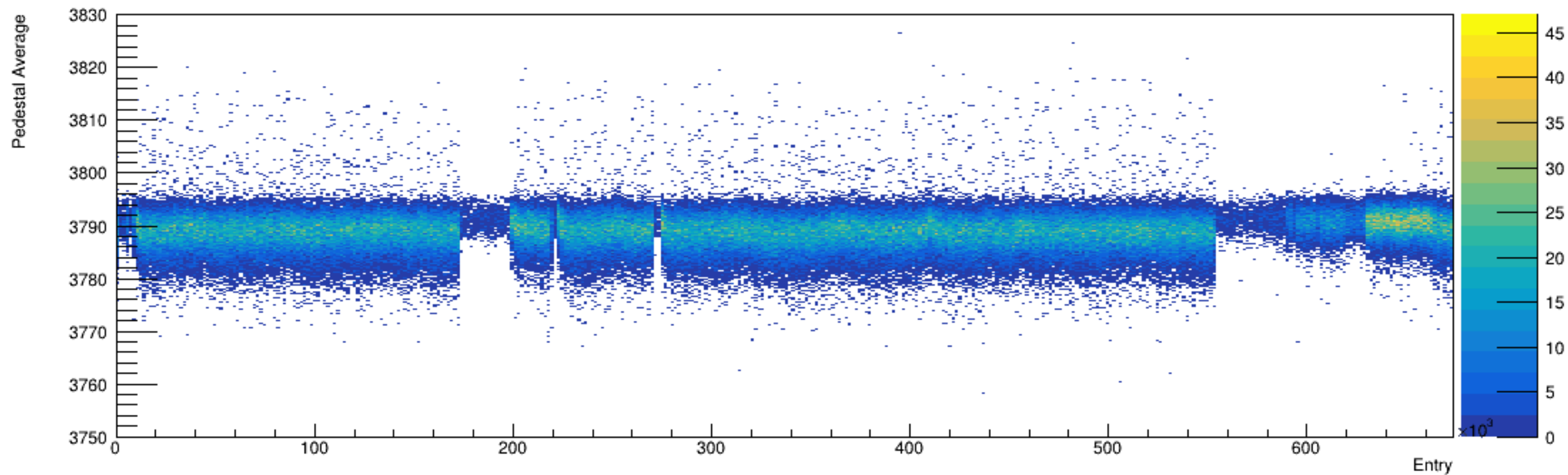
Run 4471, snapshots: Pedestal vs. Time
