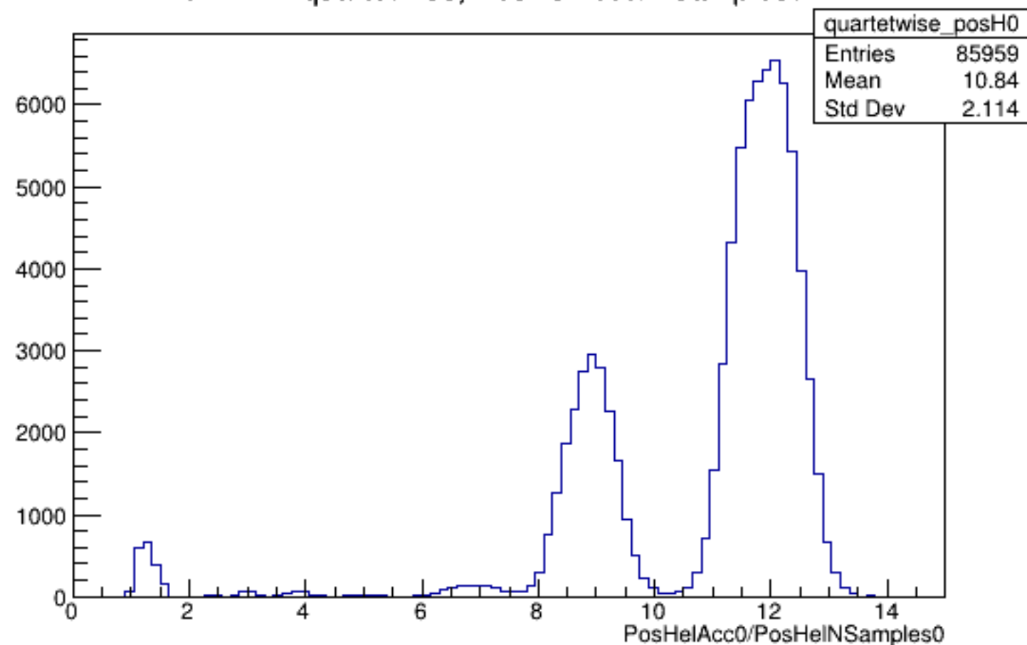
Run 4472 quartetwise, PosHelAcc0/NSamples0: All
