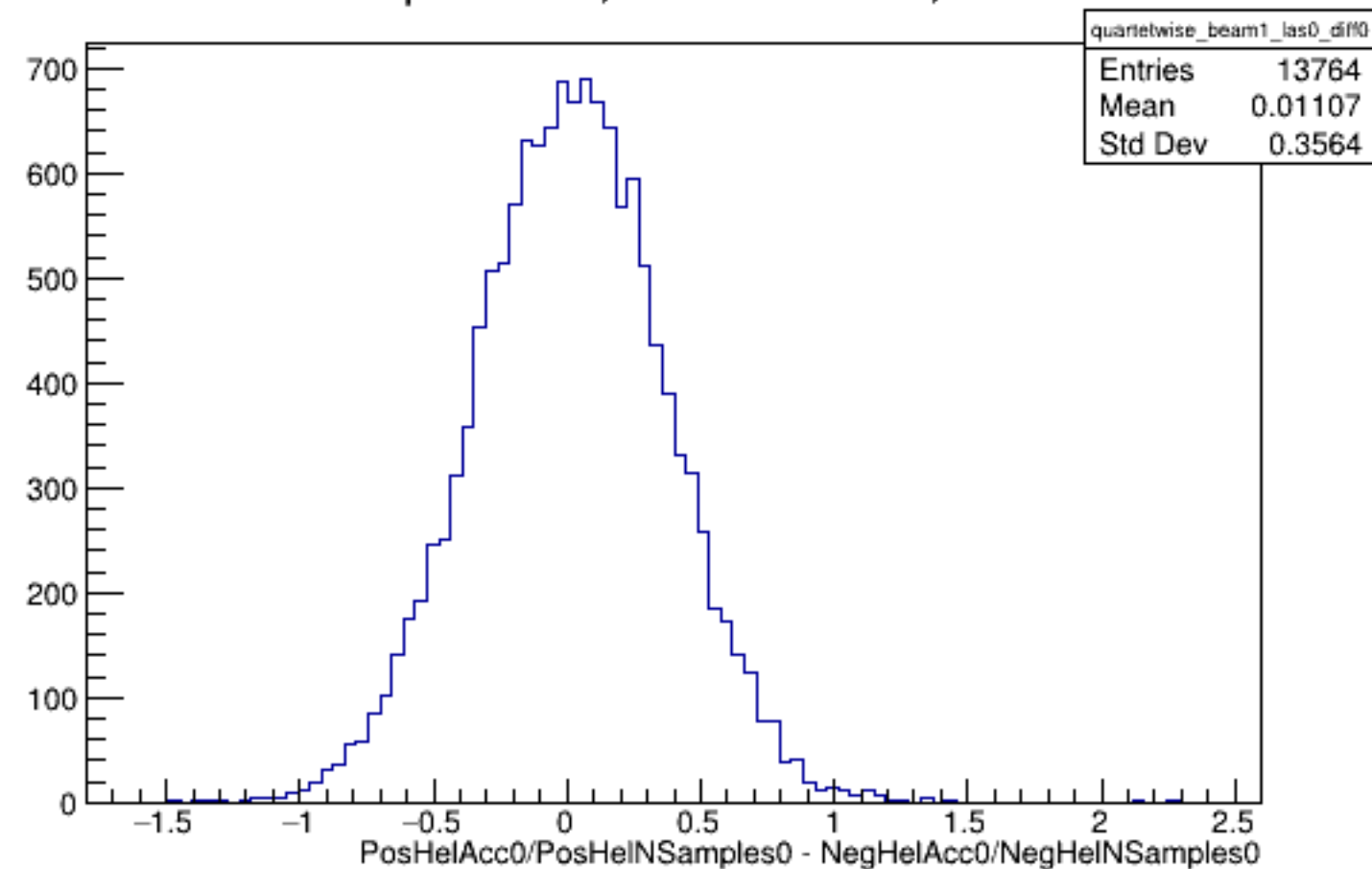
Run 4472 quartetwise, Diffs0: Beam ON, Laser OFF
