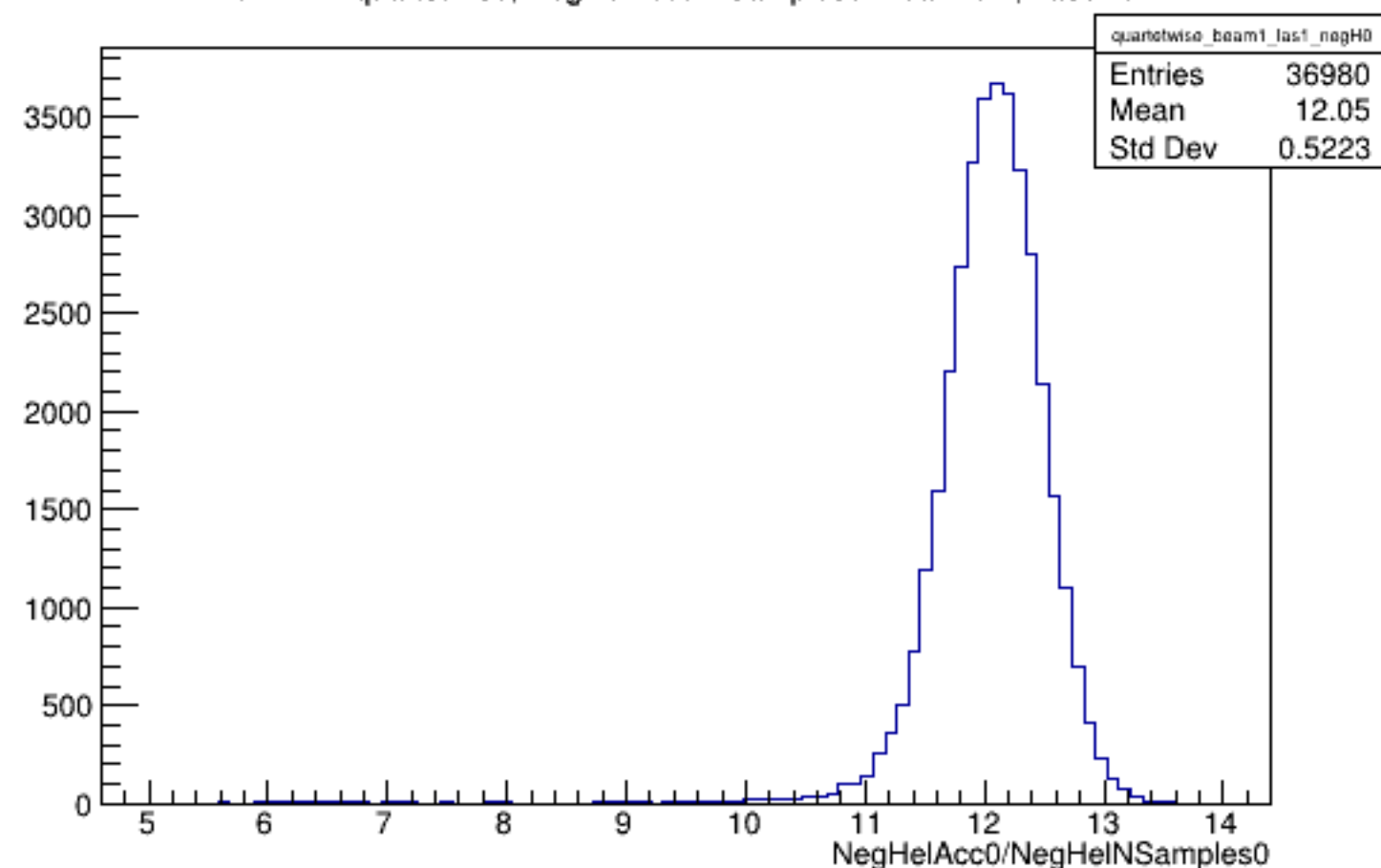
Run 4472 quartetwise, NegHelAcc0/NSamples0: Beam ON, Laser ON
