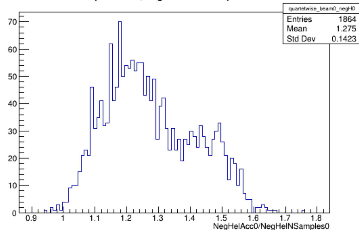
Run 4472 quartetwise, NegHelAcc0/NSamples0: Beam OFF
