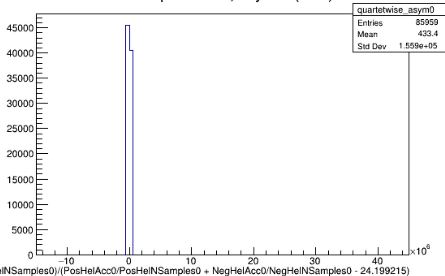
Run 4472 quartetwise, Asyms0 (Raw): All
