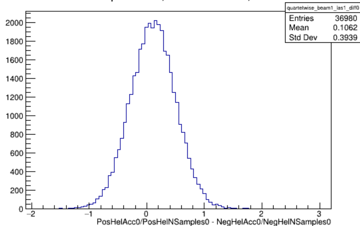
Run 4472 quartetwise, Diffs0: Beam ON, Laser ON
