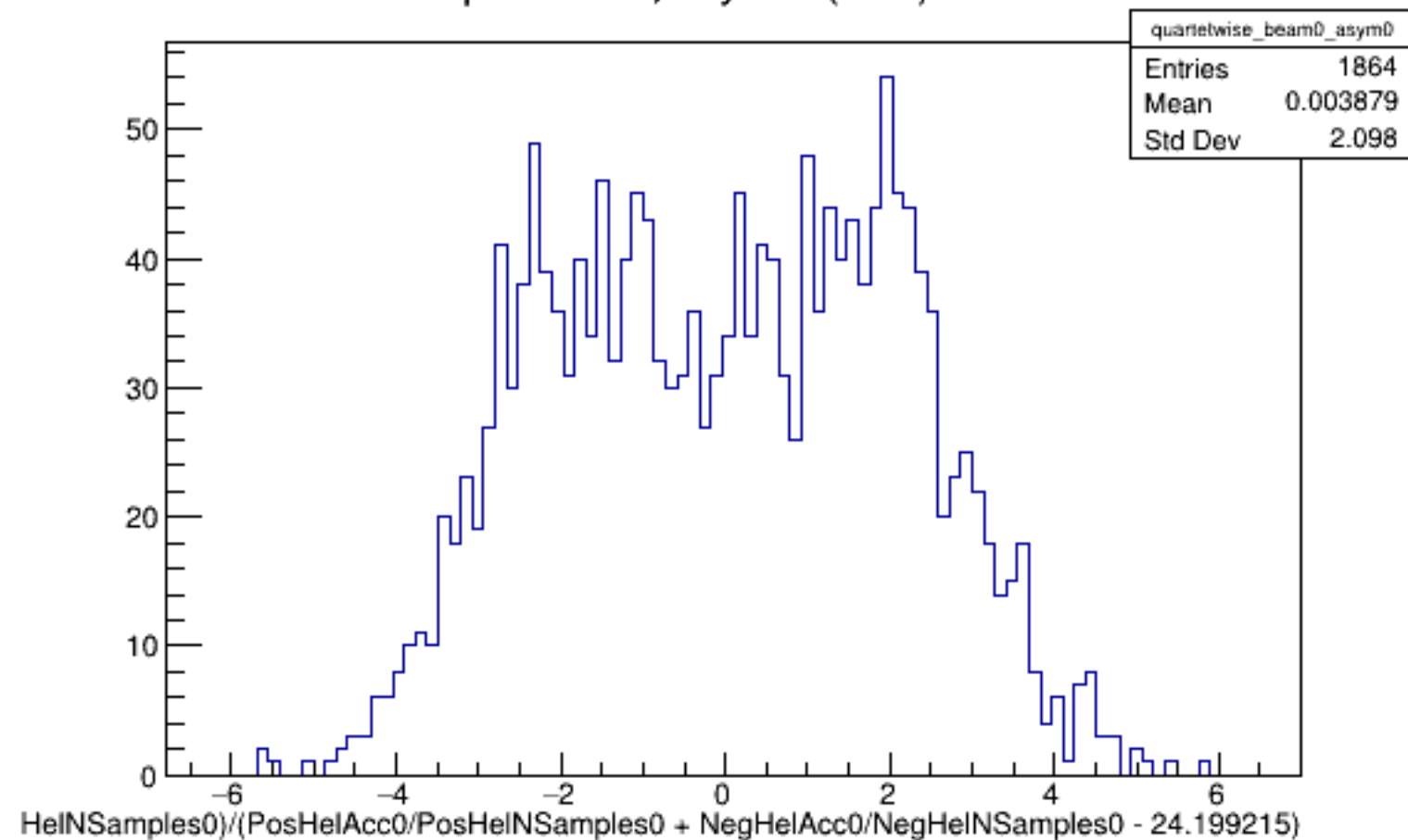
Run 4472 quartetwise, Asyms0 (Raw): Beam OFF
