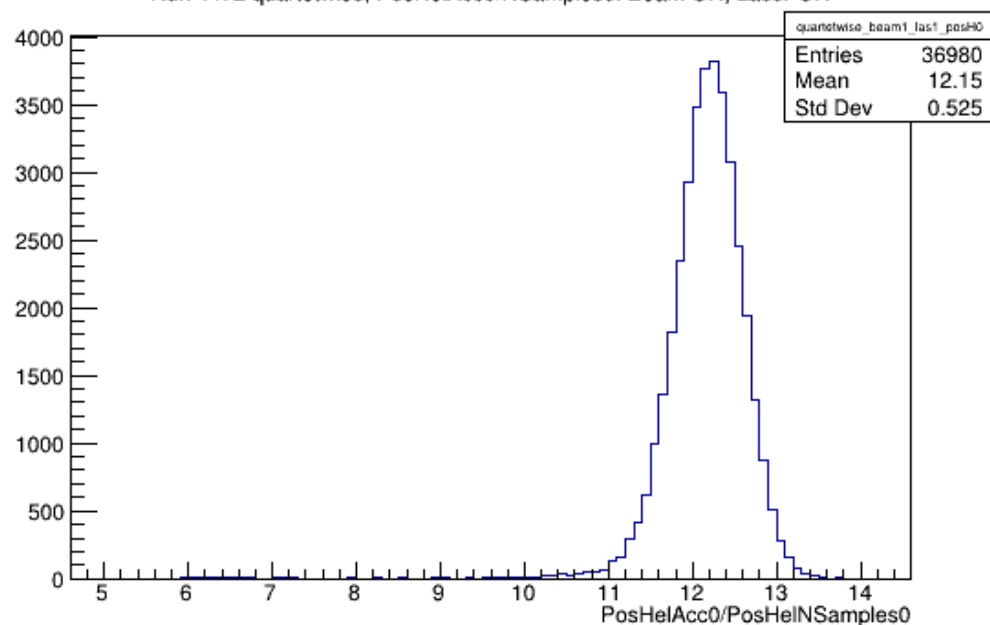
Run 4472 quartetwise, PosHelAcc0/NSamples0: Beam ON, Laser ON
