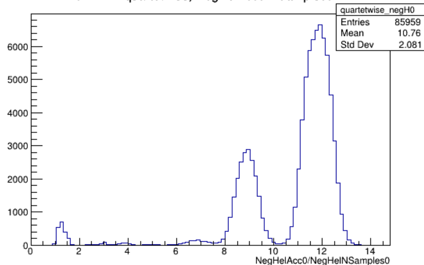
Run 4472 quartetwise, NegHelAcc0/NSamples0: All
