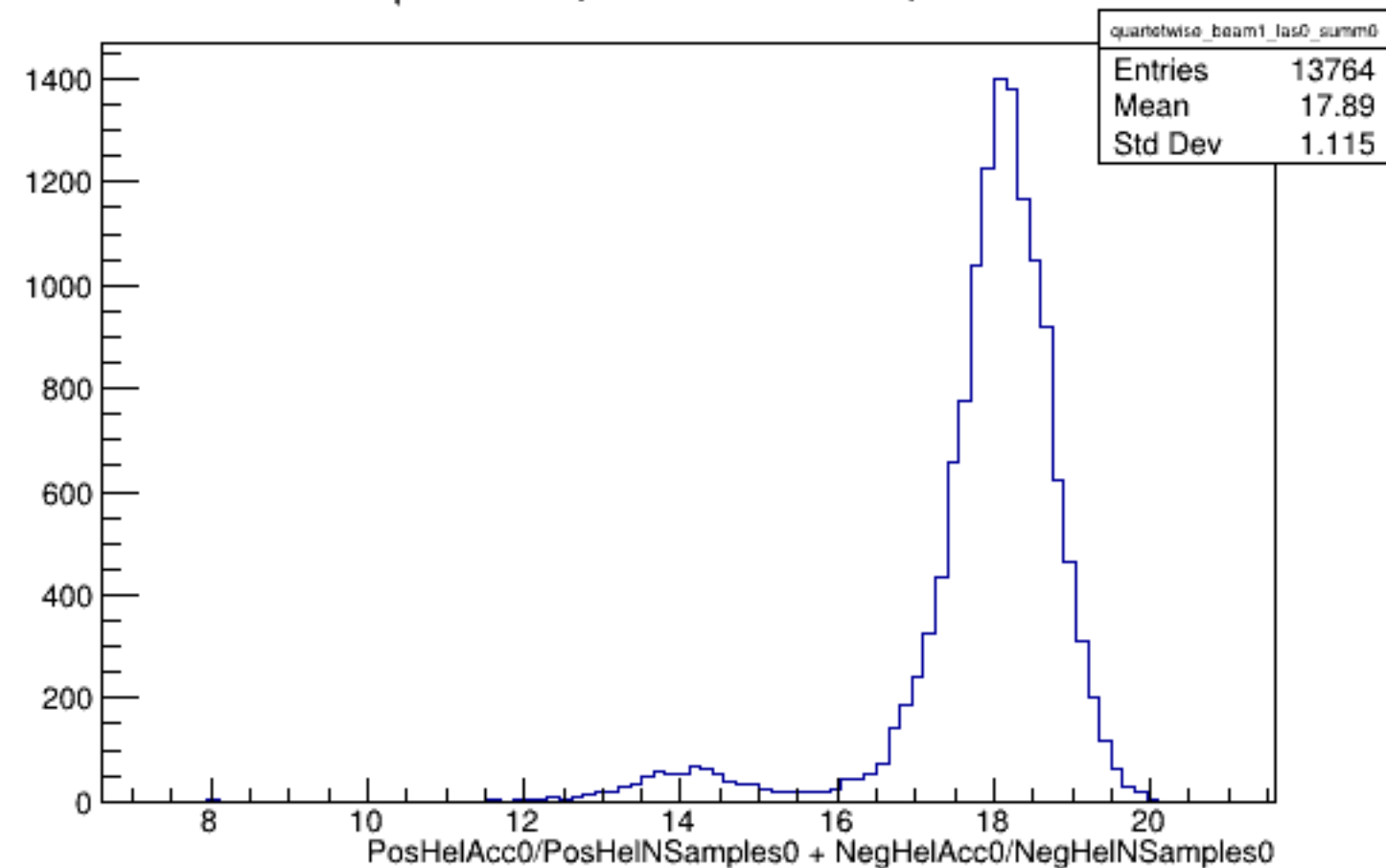
Run 4472 quartetwise, Sums0: Beam ON, Laser OFF
