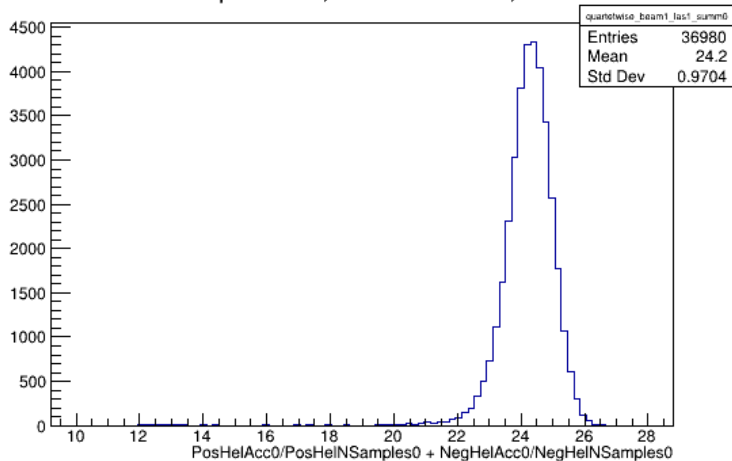
Run 4472 quartetwise, Sums0: Beam ON, Laser ON
