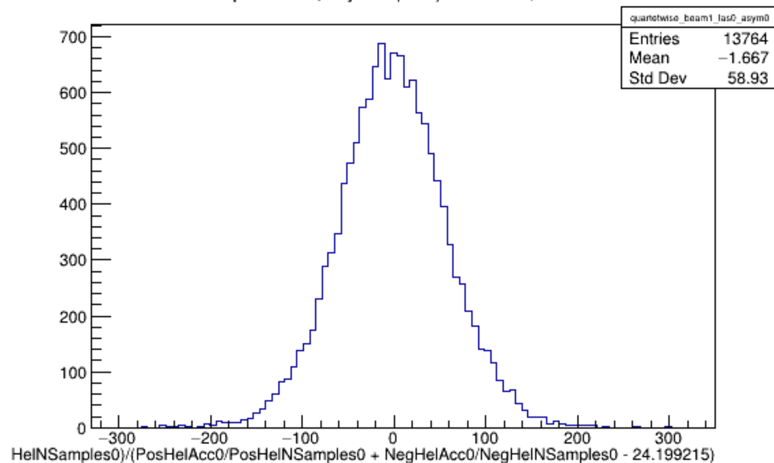
Run 4472 quartetwise, Asyms0 (Raw): Beam ON, Laser OFF
