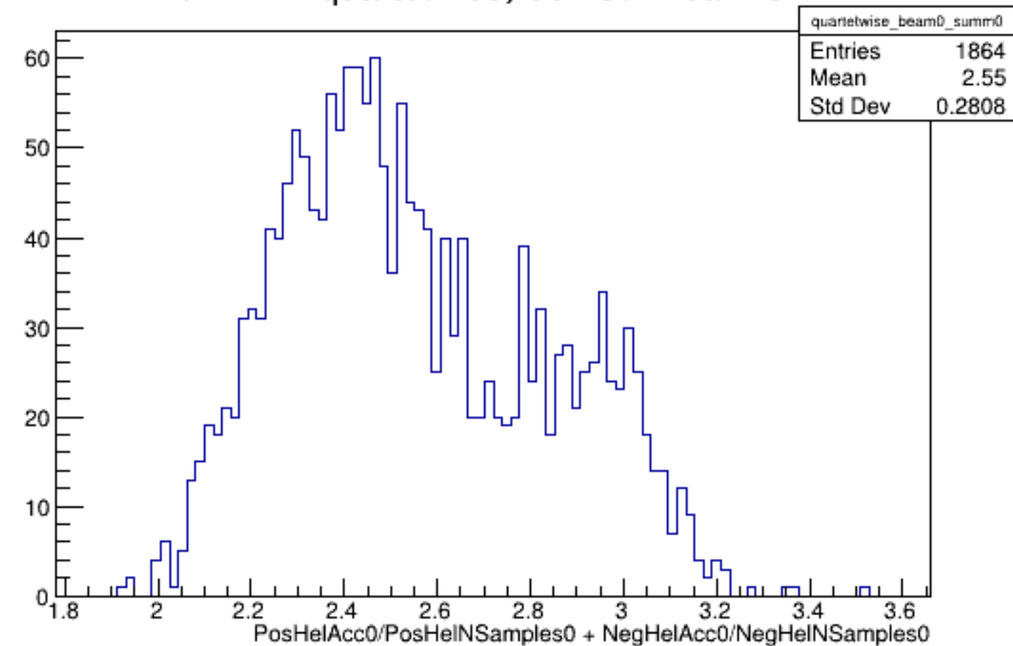
Run 4472 quartetwise, Sums0: Beam OFF
