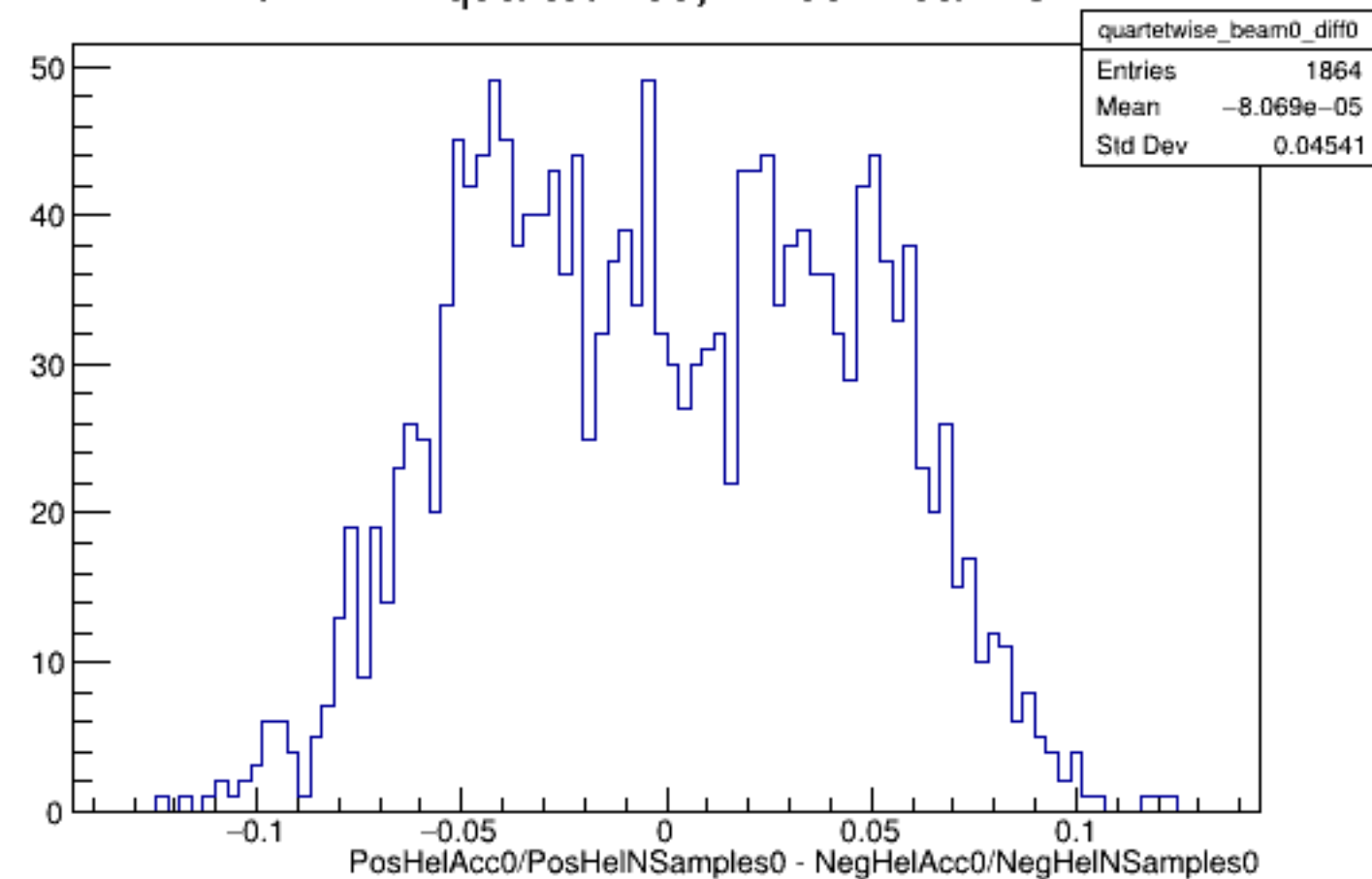
Run 4472 quartetwise, Diffs0: Beam OFF
