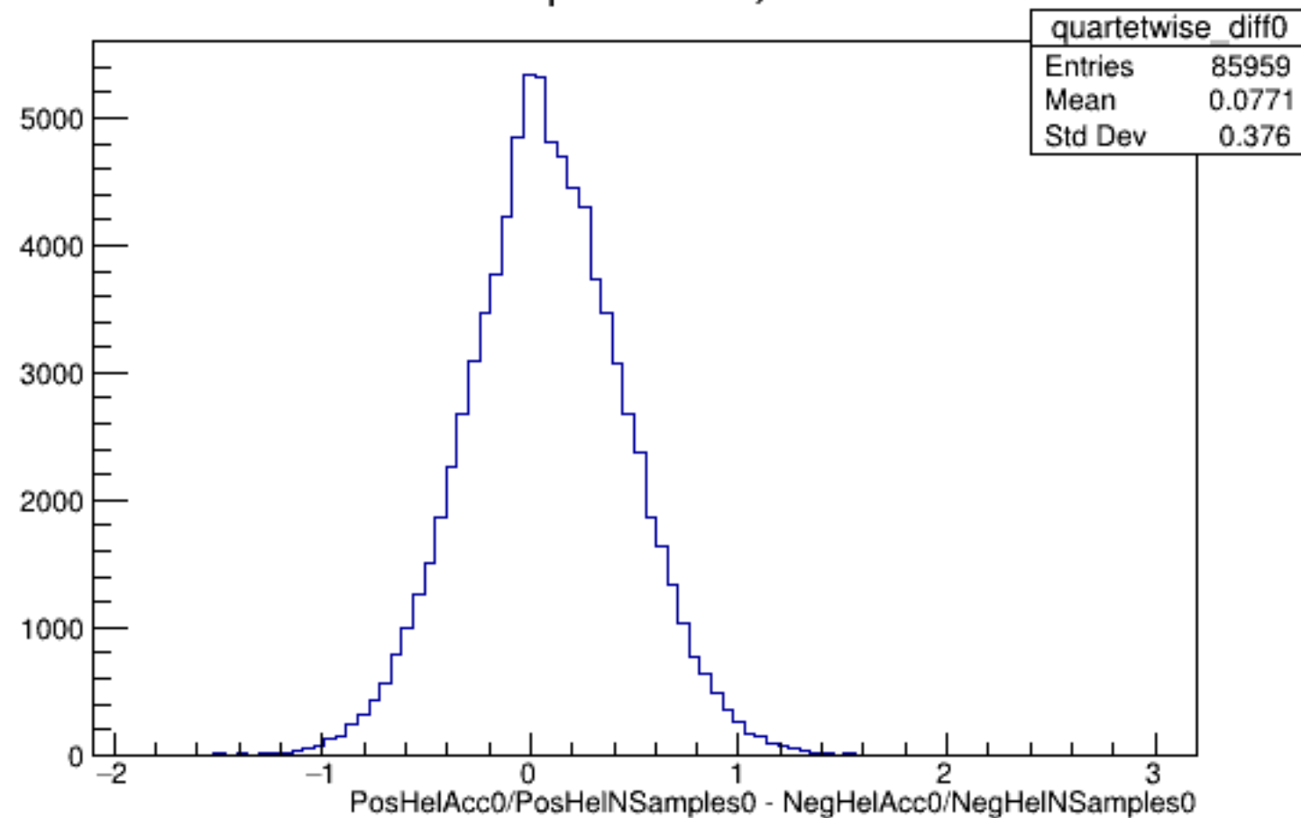
Run 4472 quartetwise, Diffs0: All
