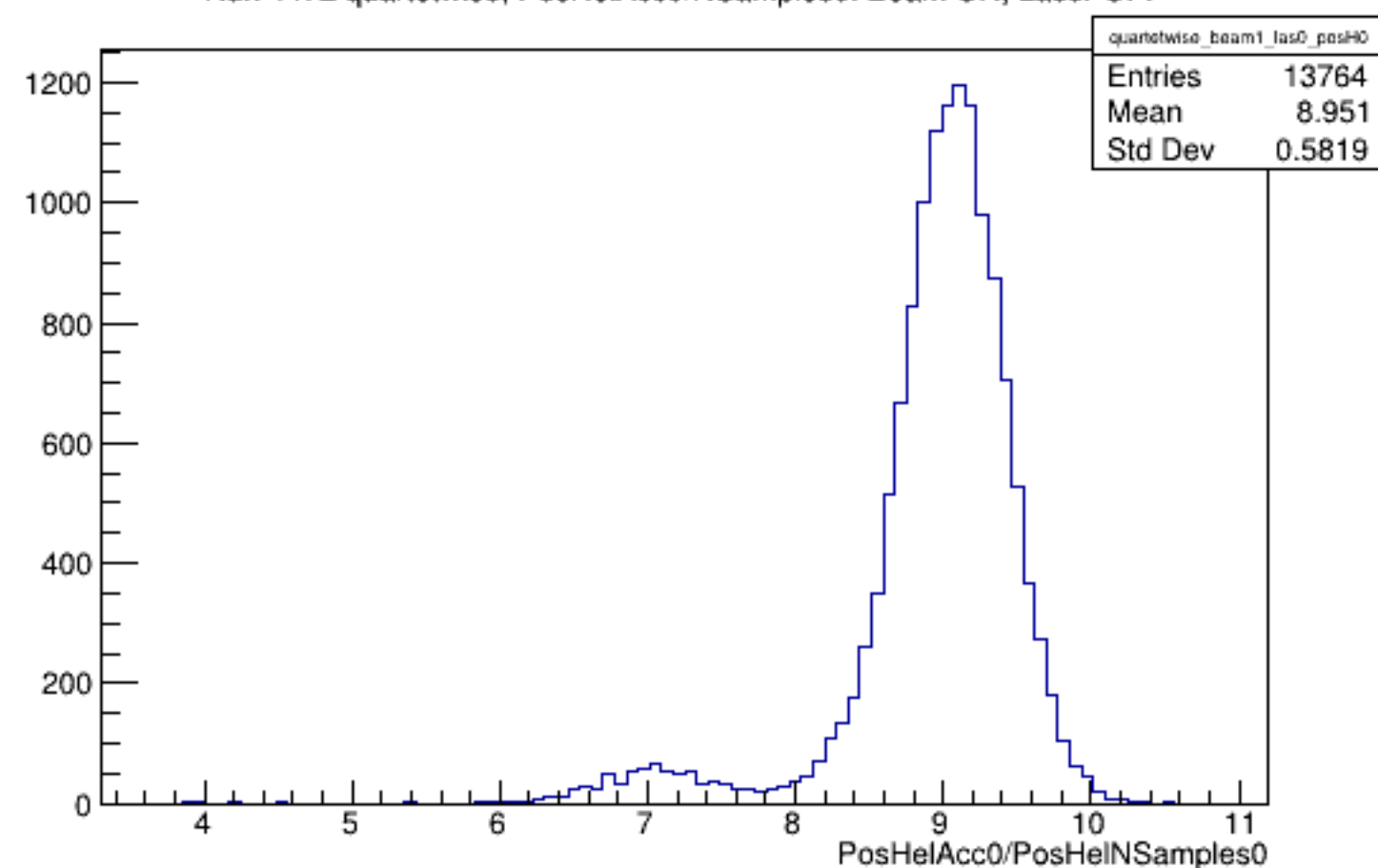
Run 4472 quartetwise, PosHelAcc0/NSamples0: Beam ON, Laser OFF
