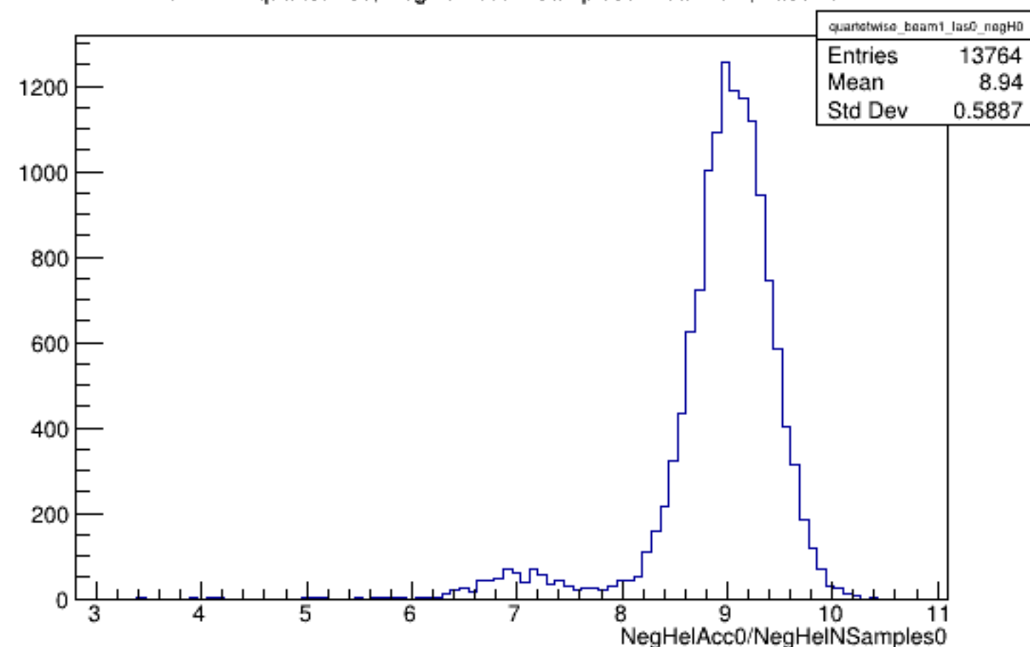
Run 4472 quartetwise, NegHelAcc0/NSamples0: Beam ON, Laser OFF
