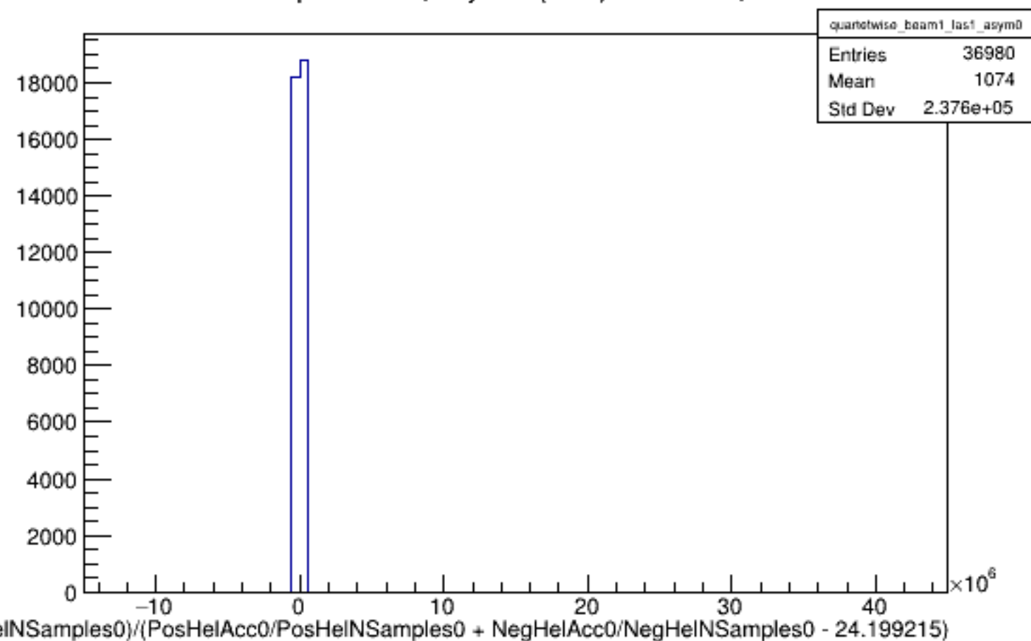
Run 4472 quartetwise, Asyms0 (Raw): Beam ON, Laser ON
