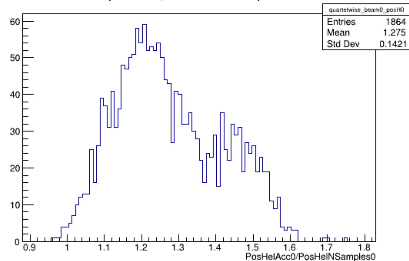
Run 4472 quartetwise, PosHelAcc0/NSamples0: Beam OFF
