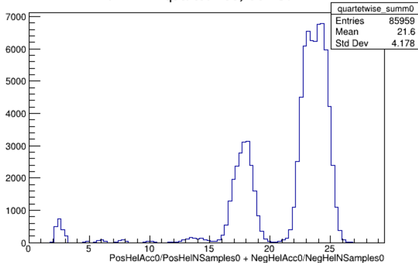
Run 4472 quartetwise, Sums0: All
