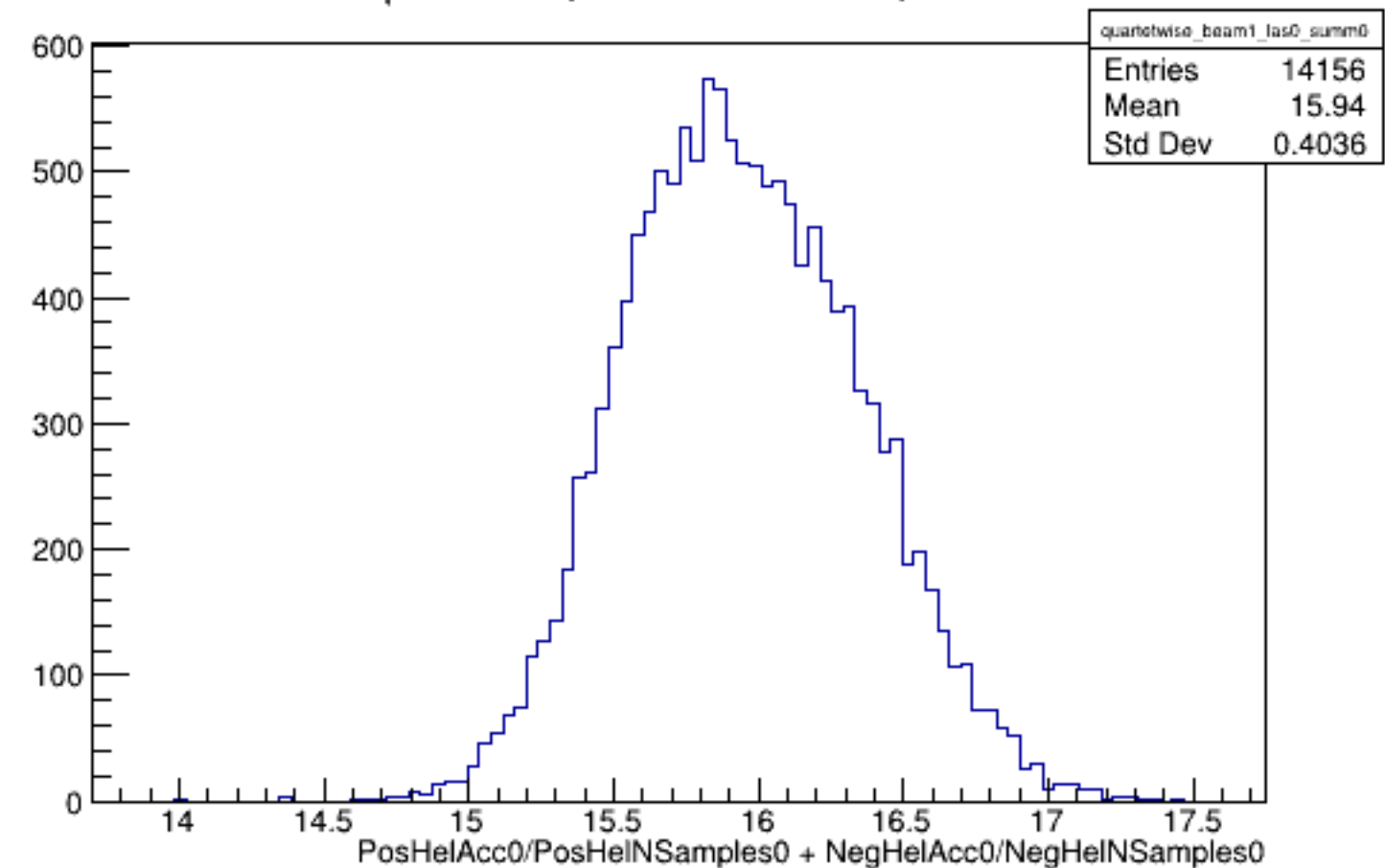
Run 4483 quartetwise, Sums0: Beam ON, Laser OFF
