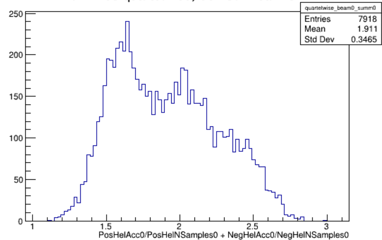
Run 4483 quartetwise, Sums0: Beam OFF
