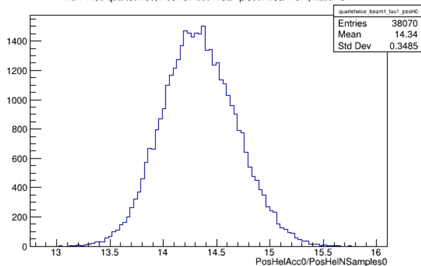
Run 4483 quartetwise, PosHelAcc0/NSamples0: Beam ON, Laser ON
