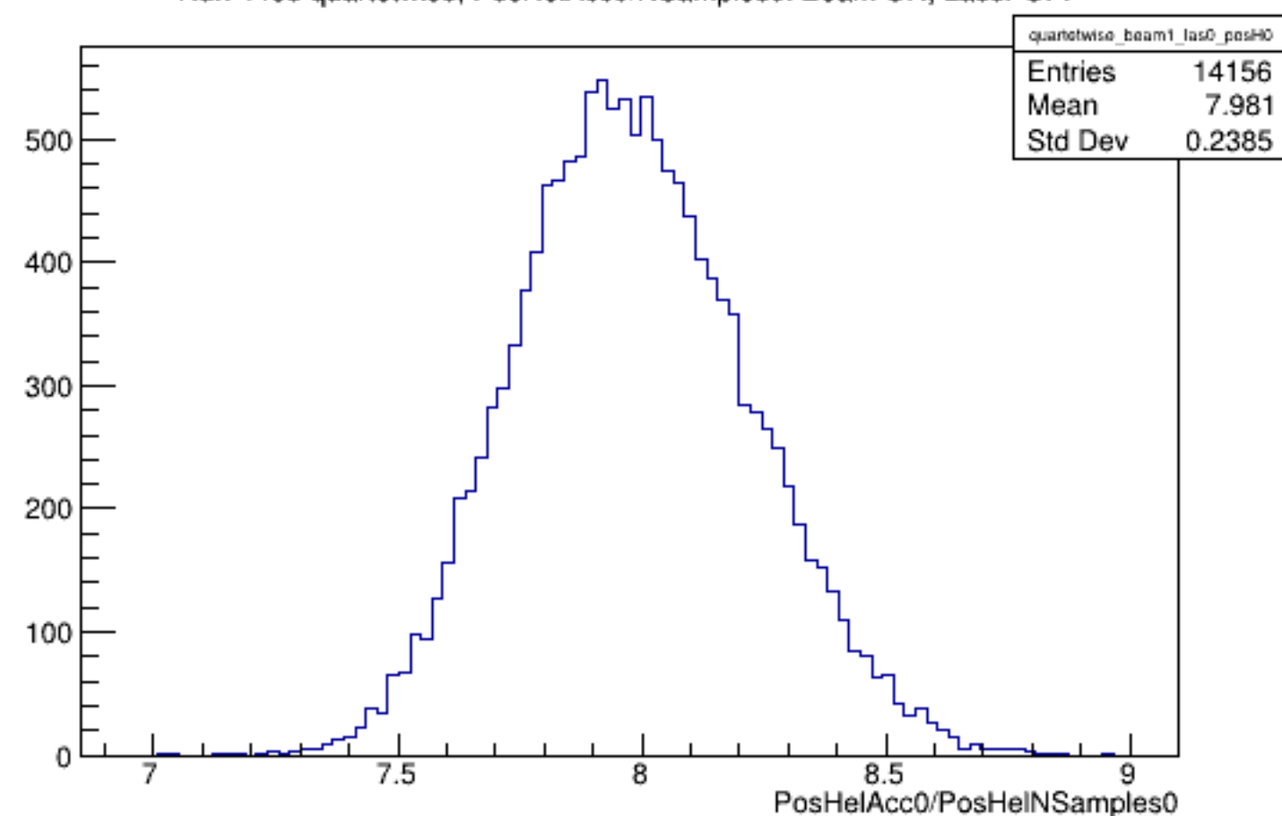
Run 4483 quartetwise, PosHelAcc0/NSamples0: Beam ON, Laser OFF
