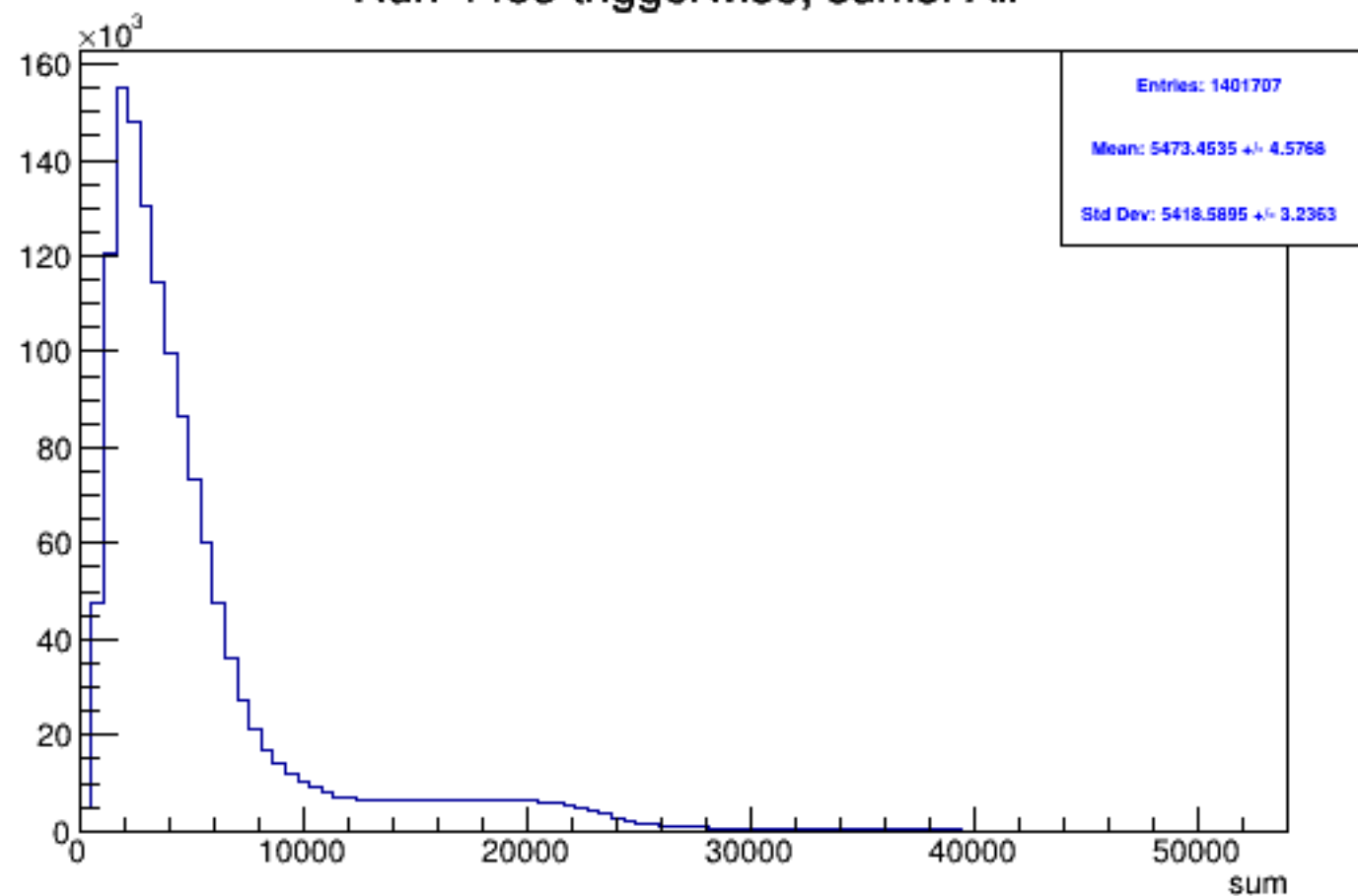
Run 4483 triggerwise, sums: All
