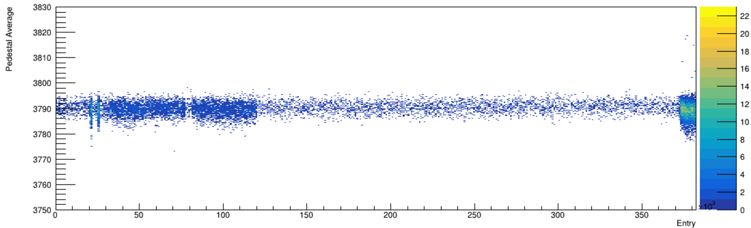
Run 4484, snapshots: Pedestal vs. Time
