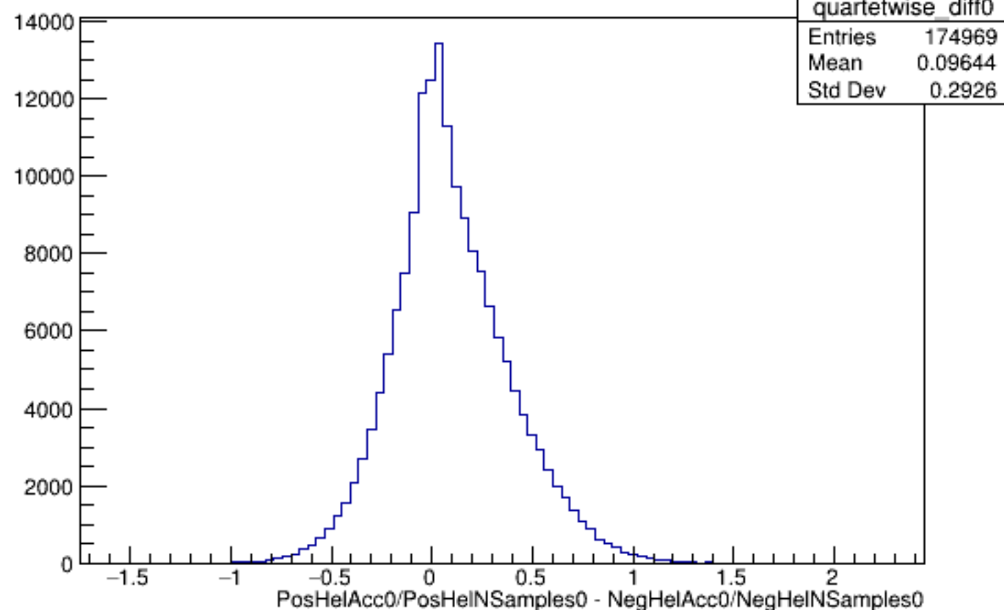
Run 4485 quartetwise, Diffs0: All
