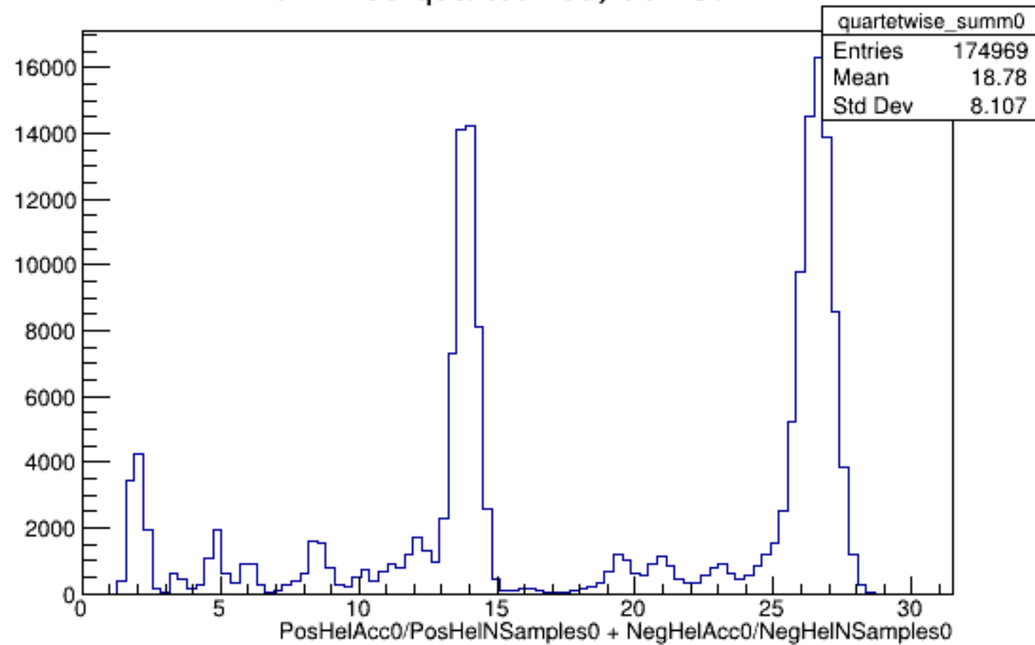
Run 4485 quartetwise, Sums0: All
