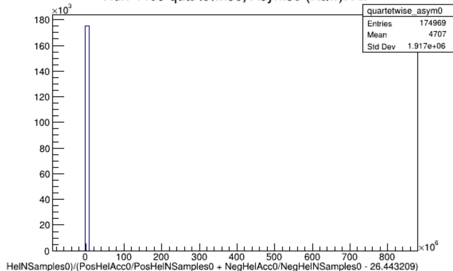
Run 4485 quartetwise, Asyms0 (Raw): All
