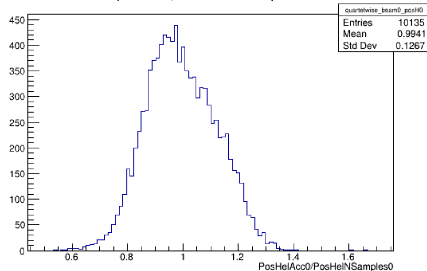
Run 4485 quartetwise, PosHelAcc0/NSamples0: Beam OFF
