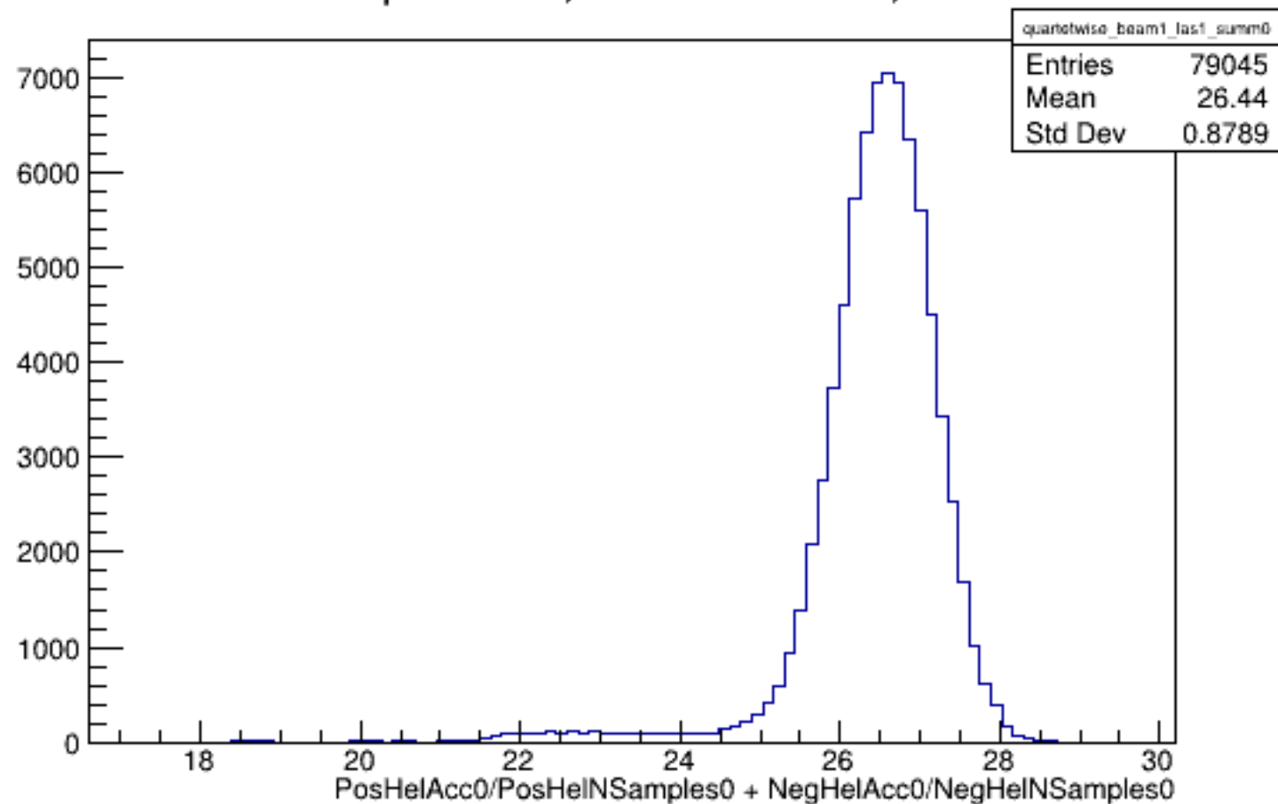
Run 4485 quartetwise, Sums0: Beam ON, Laser ON
