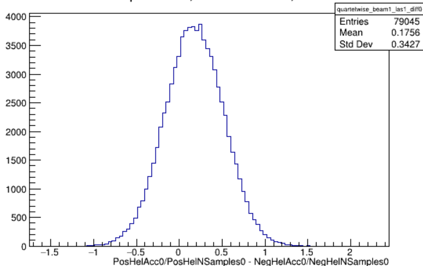
Run 4485 quartetwise, Diffs0: Beam ON, Laser ON
