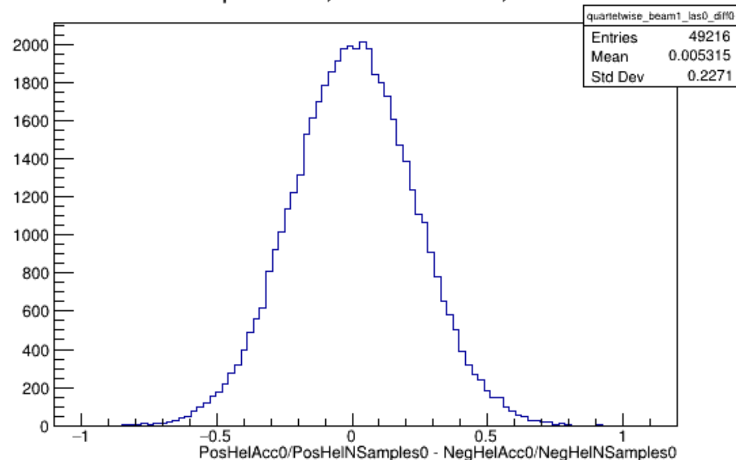
Run 4485 quartetwise, Diffs0: Beam ON, Laser OFF
