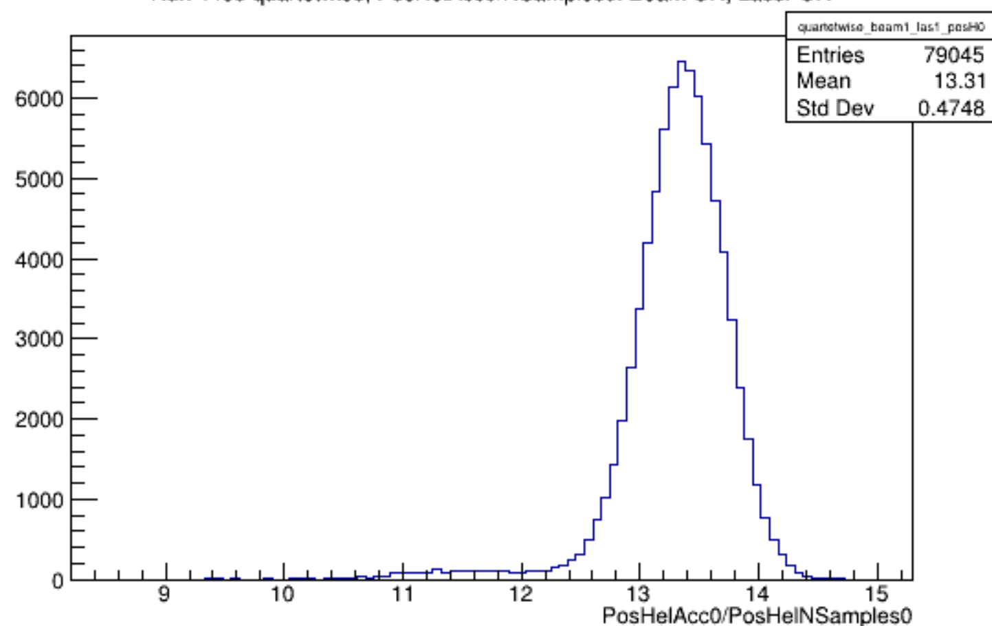
Run 4485 quartetwise, PosHelAcc0/NSamples0: Beam ON, Laser ON
