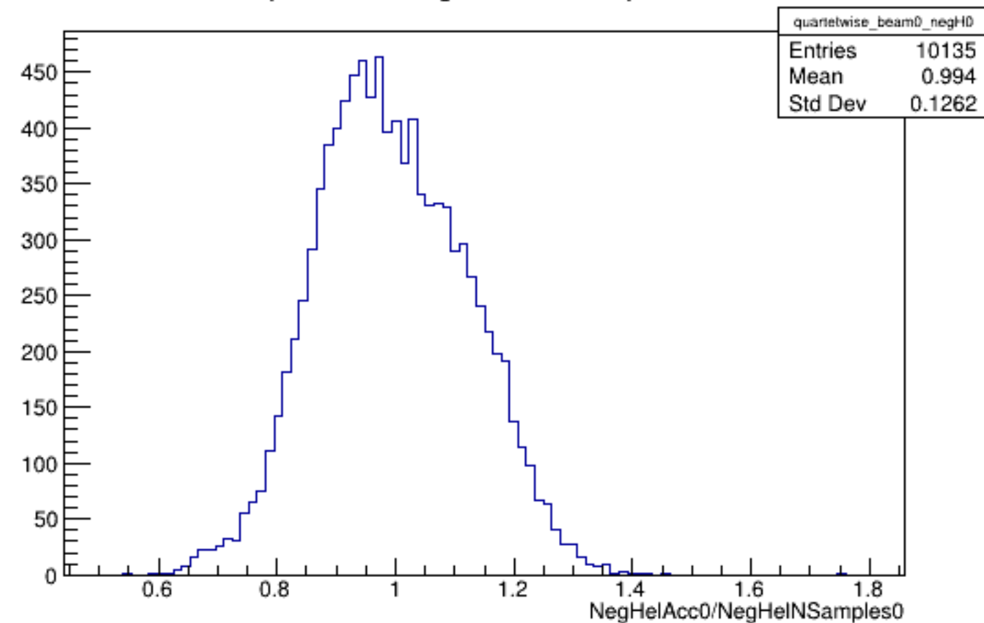
Run 4485 quartetwise, NegHelAcc0/NSamples0: Beam OFF
