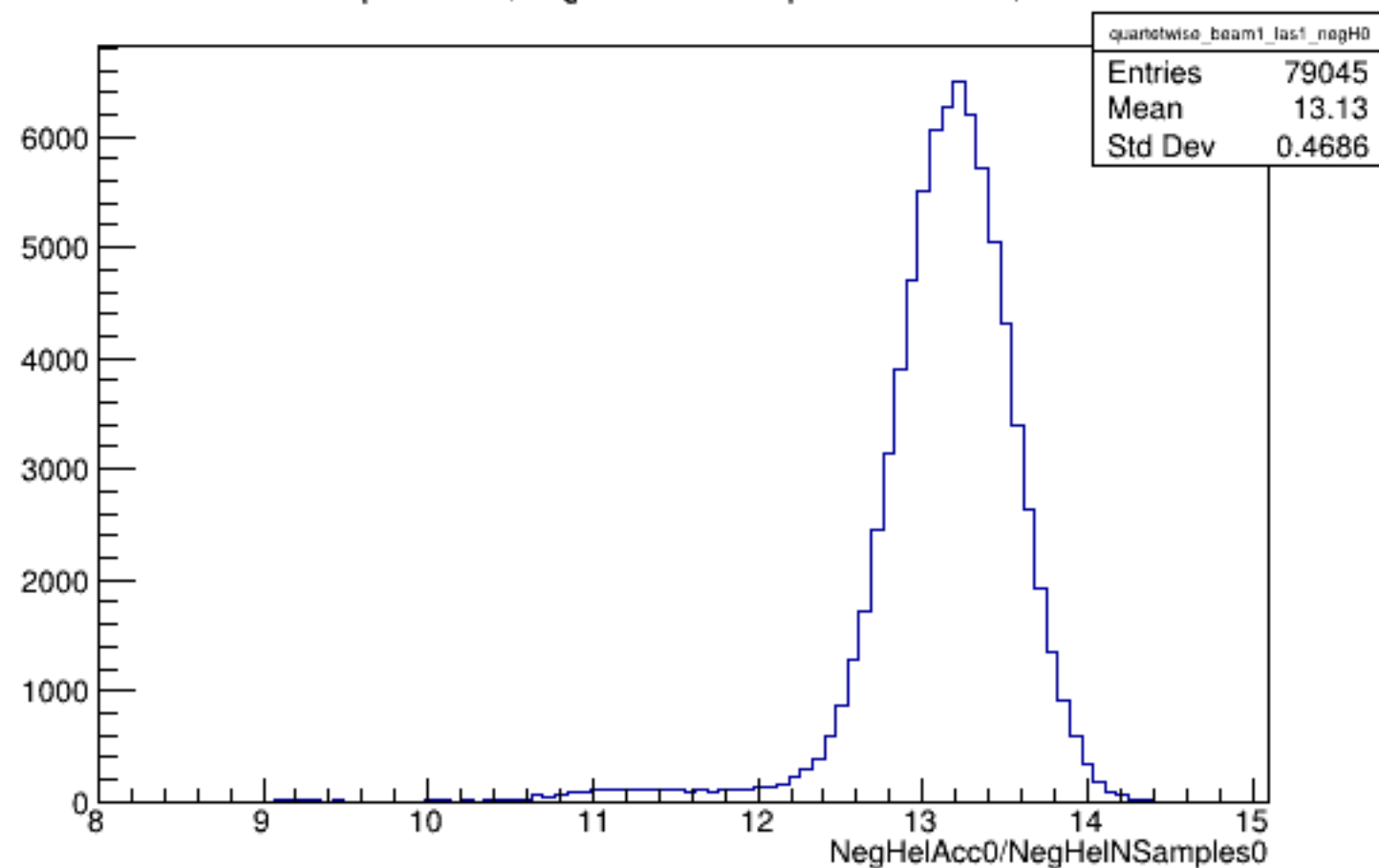
Run 4485 quartetwise, NegHelAcc0/NSamples0: Beam ON, Laser ON
