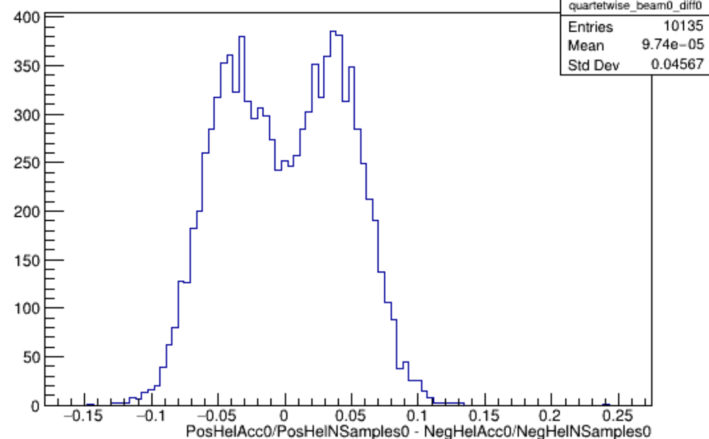
Run 4485 quartetwise, Diffs0: Beam OFF
