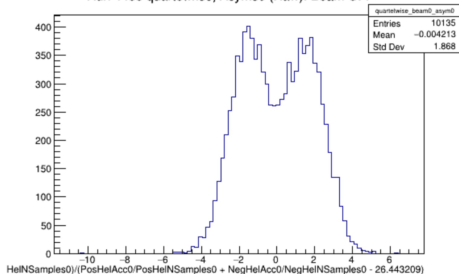
Run 4485 quartetwise, Asyms0 (Raw): Beam OFF
