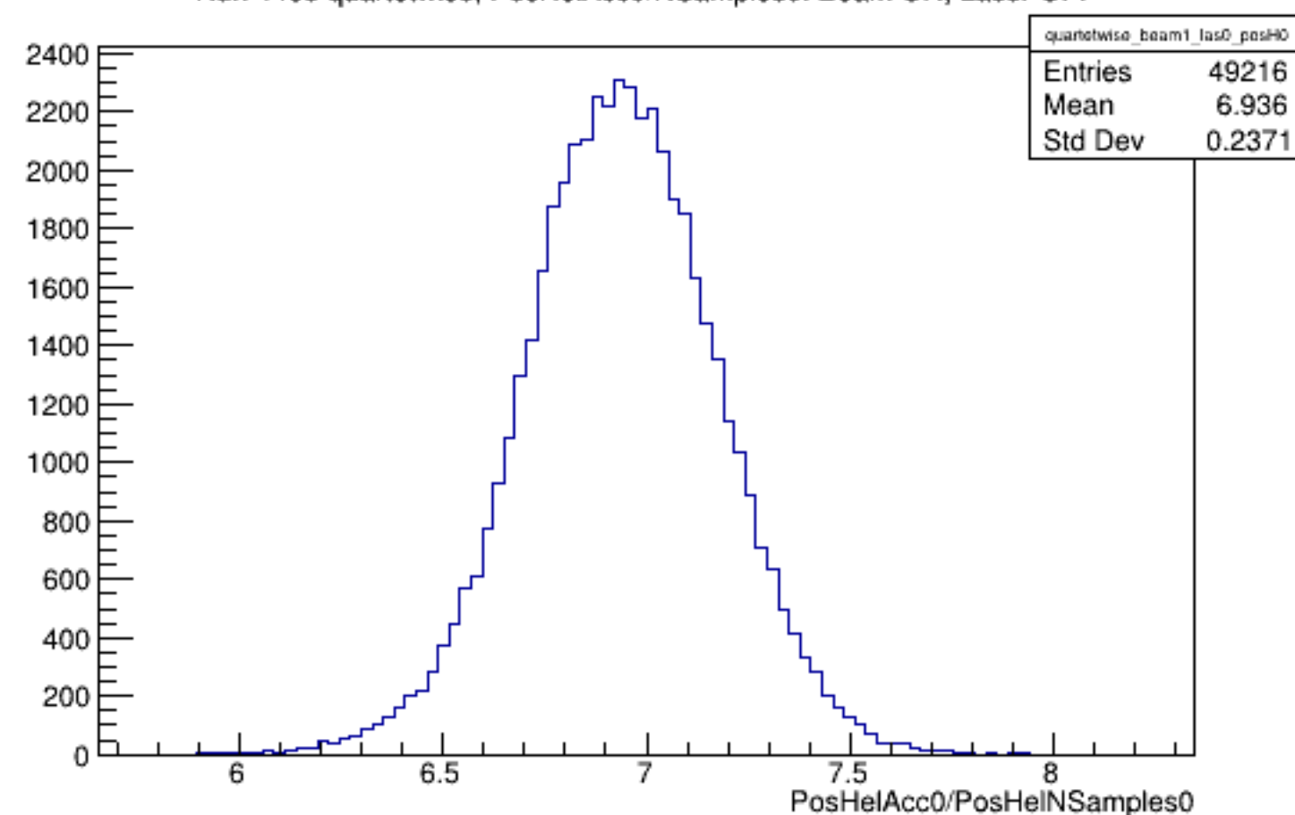
Run 4485 quartetwise, PosHelAcc0/NSamples0: Beam ON, Laser OFF
