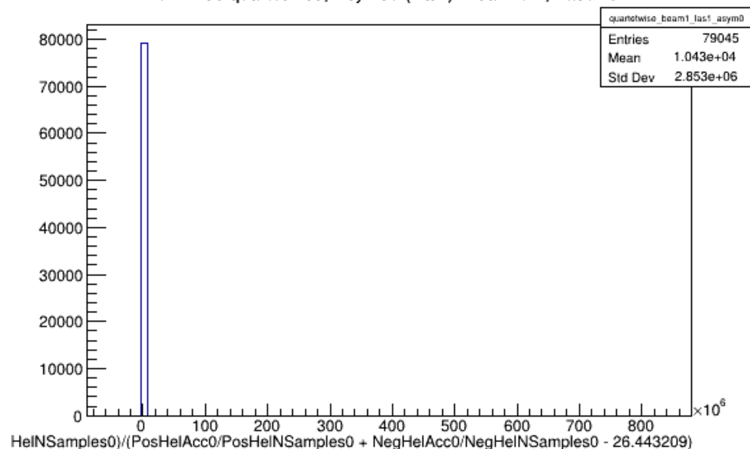
Run 4485 quartetwise, Asyms0 (Raw): Beam ON, Laser ON
