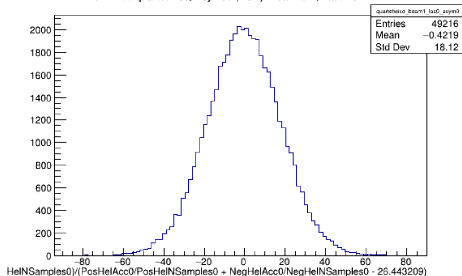
Run 4485 quartetwise, Asyms0 (Raw): Beam ON, Laser OFF
