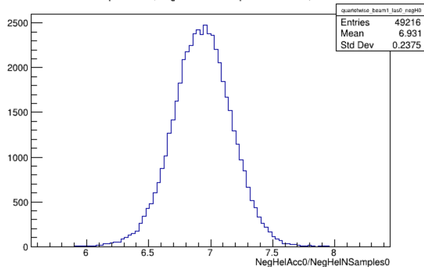
Run 4485 quartetwise, NegHelAcc0/NSamples0: Beam ON, Laser OFF
