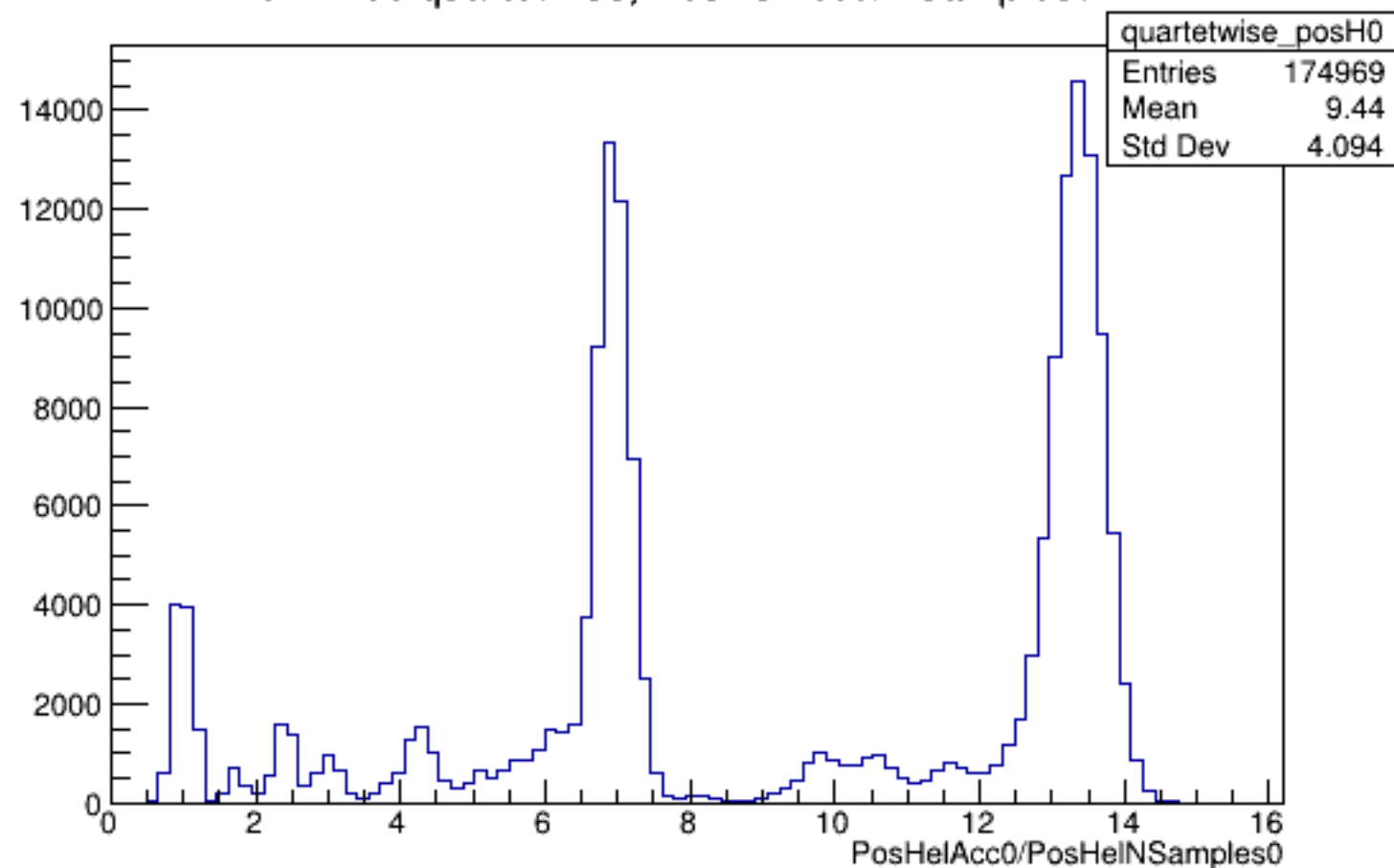
Run 4485 quartetwise, PosHelAcc0/NSamples0: All
