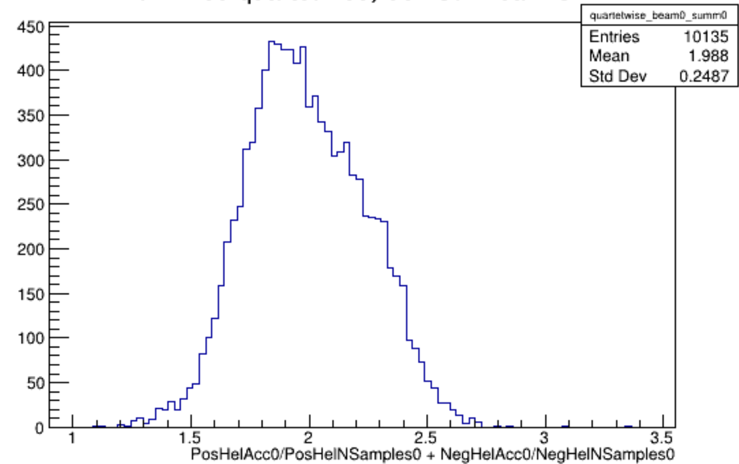
Run 4485 quartetwise, Sums0: Beam OFF
