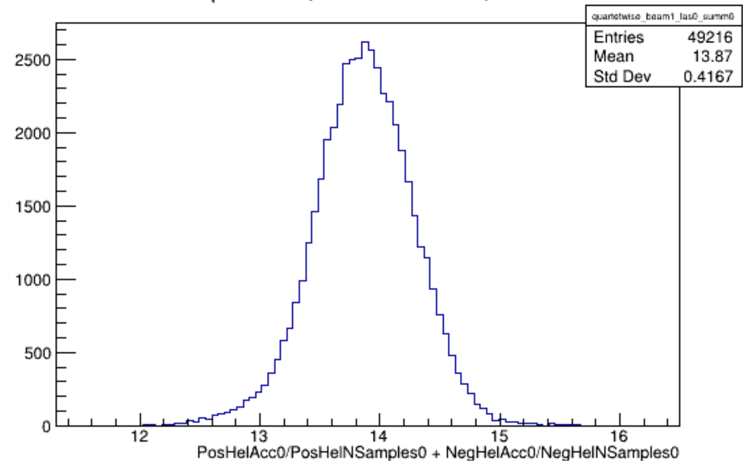
Run 4485 quartetwise, Sums0: Beam ON, Laser OFF
