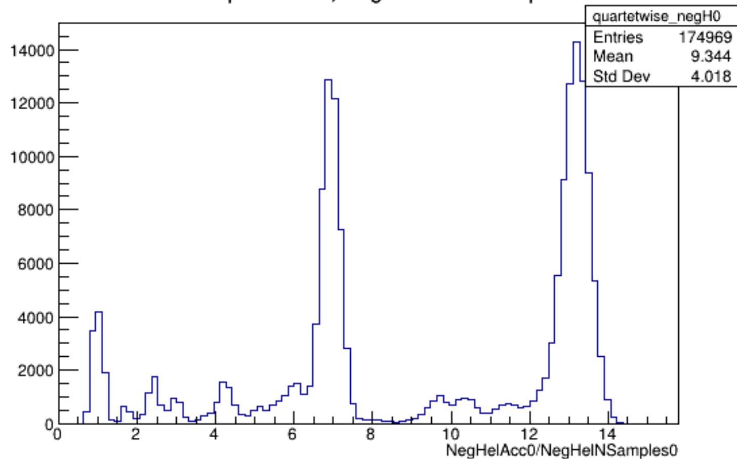
Run 4485 quartetwise, NegHelAcc0/NSamples0: All
