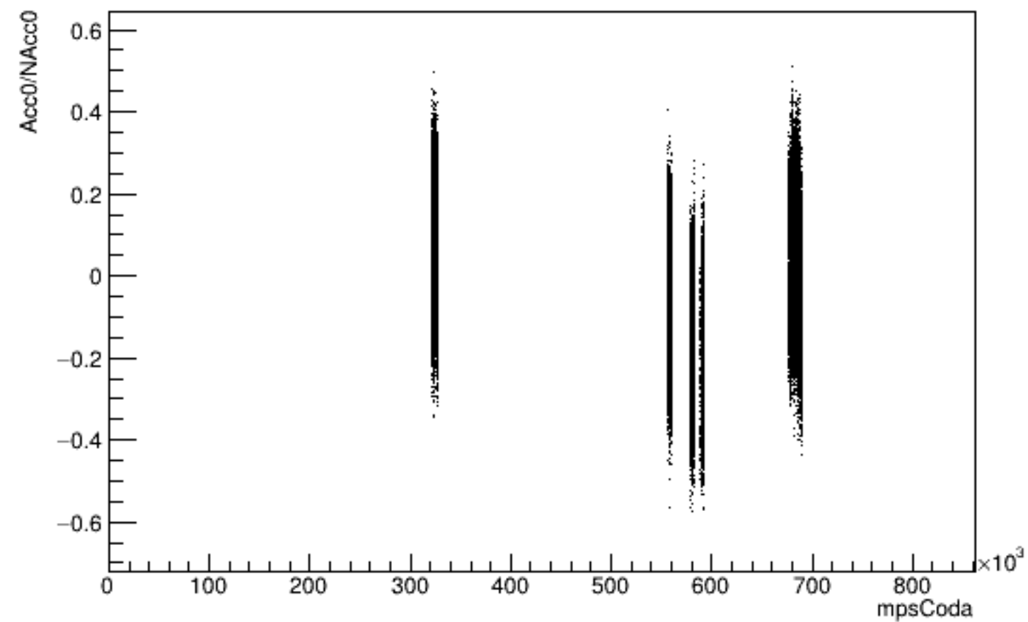
Run 4491 mpwise, Acc0/NAcc0:mpsCoda, beam OFF
