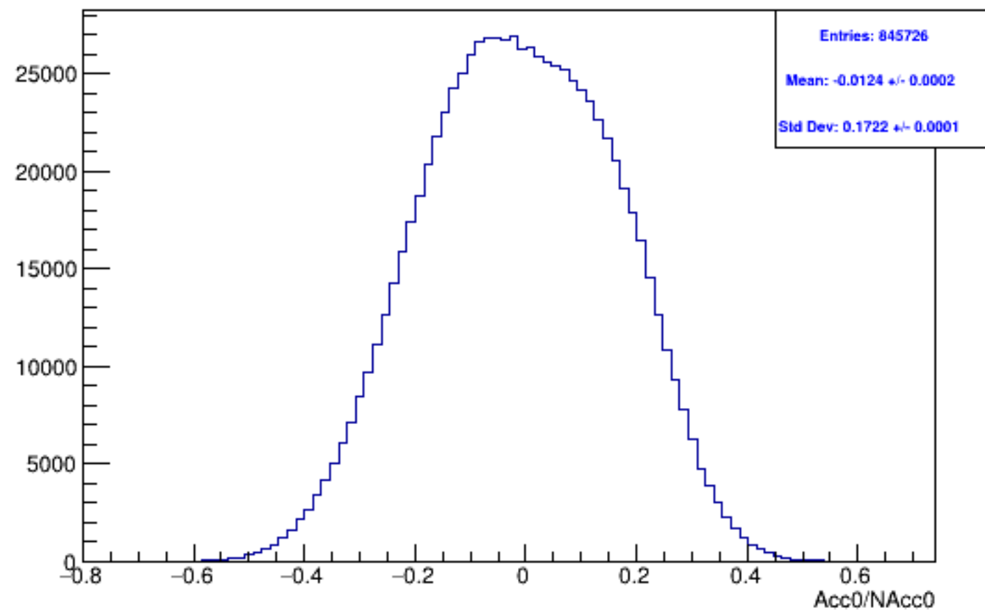
Run 4491 mpwise, acc0: All
