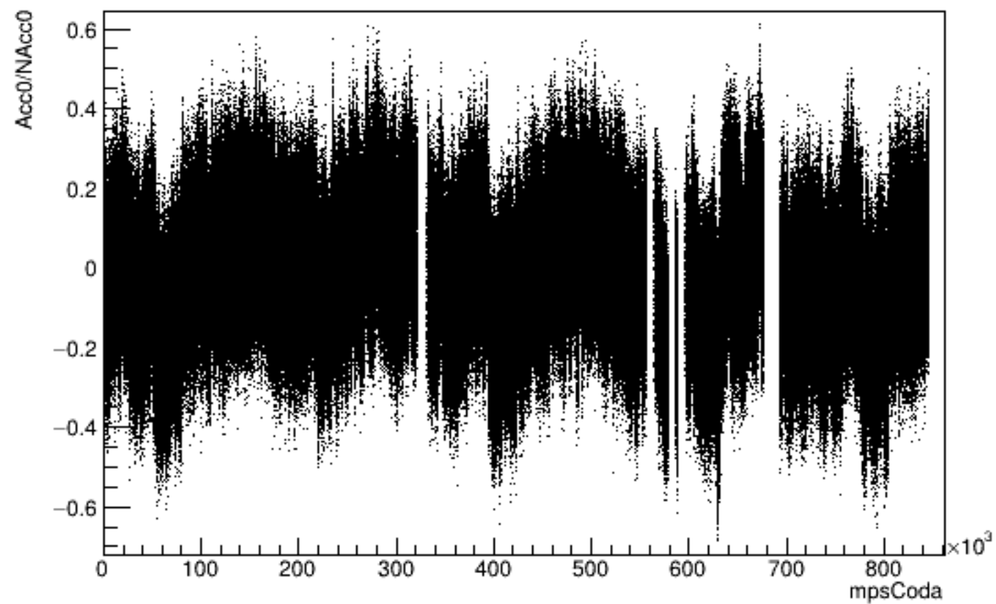
Run 4491 mpwise, Acc0/NAcc0:mpsCoda, beam ON, laser OFF
