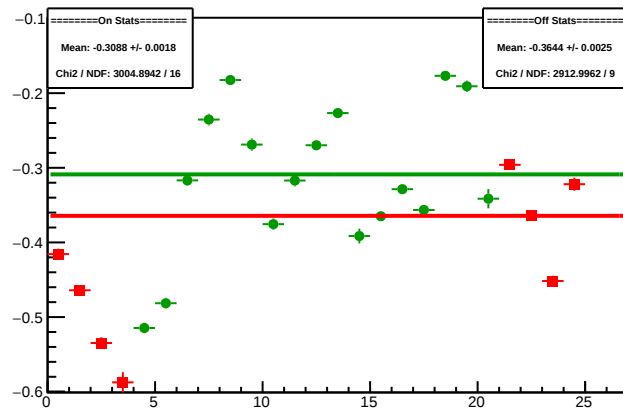
Cycle 4496.12: Multiplet Sums
