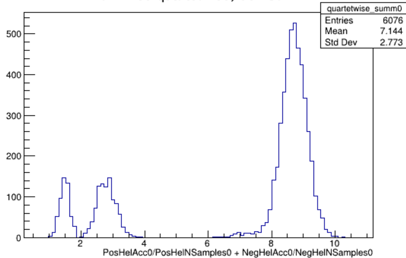
Run 4499 quartetwise, Sums0: All
