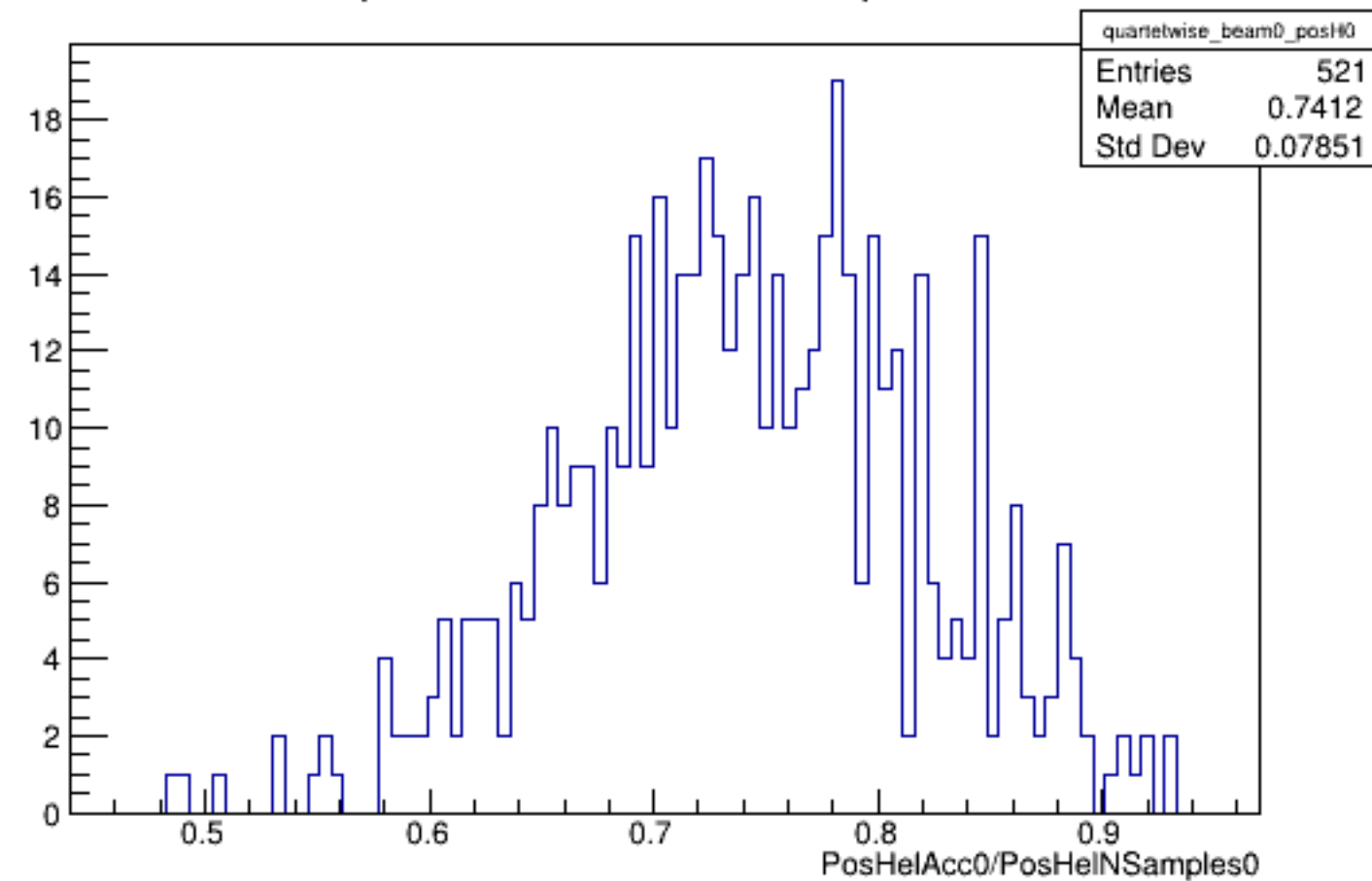
Run 4499 quartetwise, PosHelAcc0/NSamples0: Beam OFF
