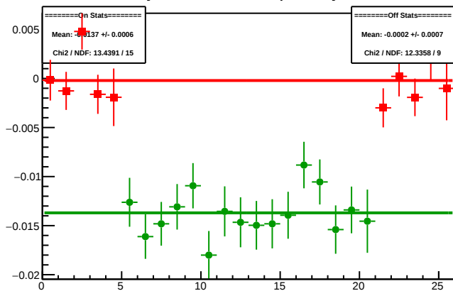
Cycle 4508.8: Multiplet Asyms
