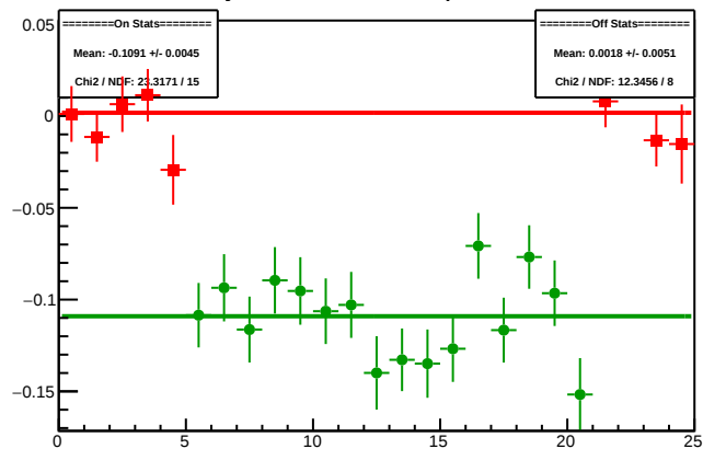
Cycle 4508.11: Multiplet Diffs
