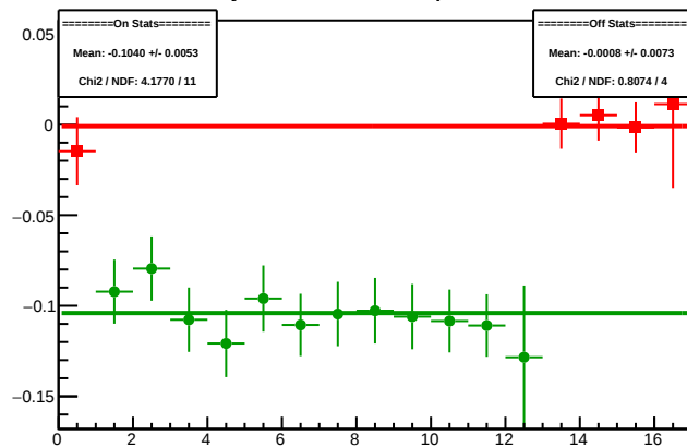
Cycle 4508.3: Multiplet Diffs
