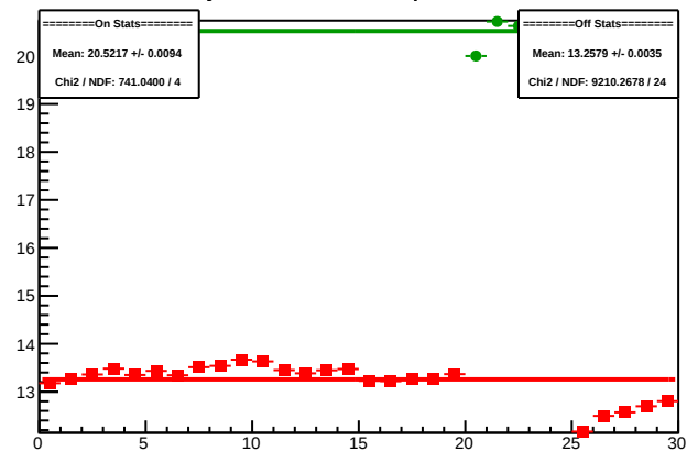
Cycle 4508.7: Multiplet Sums
