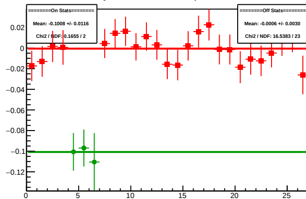
Cycle 4508.6: Multiplet Diffs
