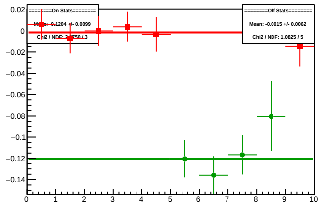
Cycle 4508.2: Multiplet Diffs
