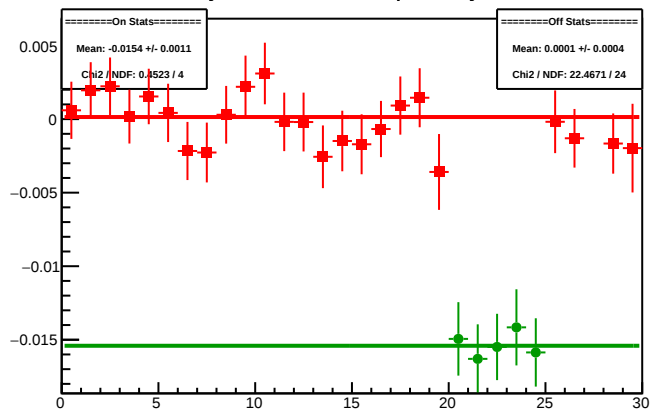
Cycle 4508.7: Multiplet Asyms
