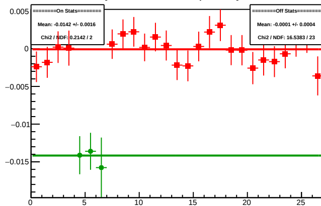
Cycle 4508.6: Multiplet Asyms
