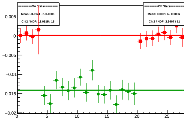
Cycle 4508.4: Multiplet Asyms
