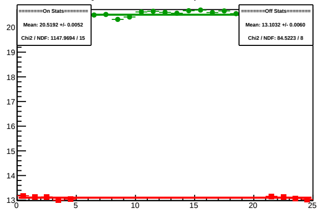
Cycle 4508.11: Multiplet Sums
