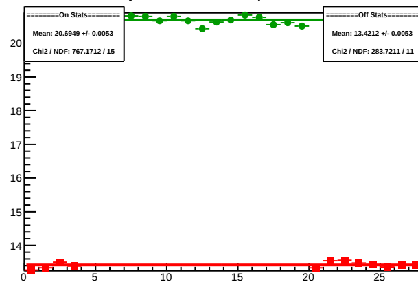
Cycle 4508.4: Multiplet Sums
