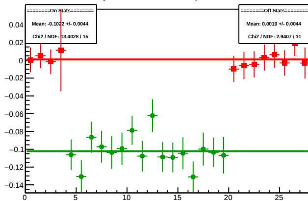
Cycle 4508.4: Multiplet Diffs
