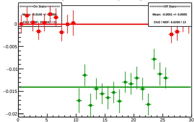
Cycle 4508.5: Multiplet Asyms
