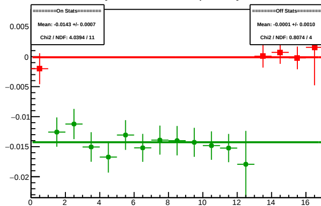
Cycle 4508.3: Multiplet Asyms
