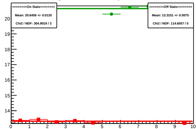
Cycle 4508.2: Multiplet Sums
