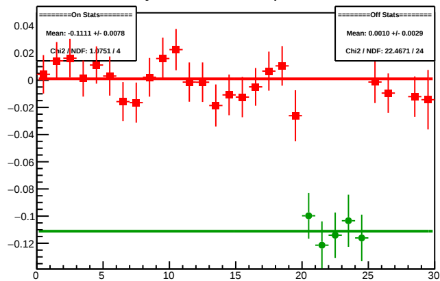
Cycle 4508.7: Multiplet Diffs
