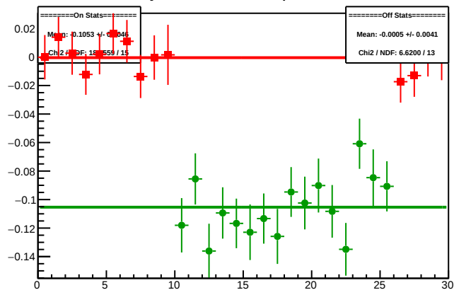
Cycle 4508.5: Multiplet Diffs
