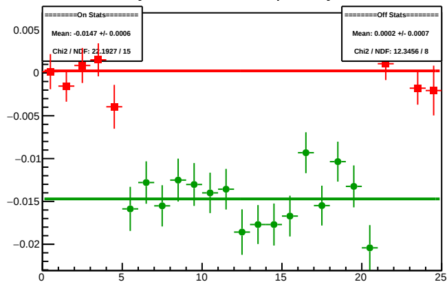
Cycle 4508.11: Multiplet Asyms
