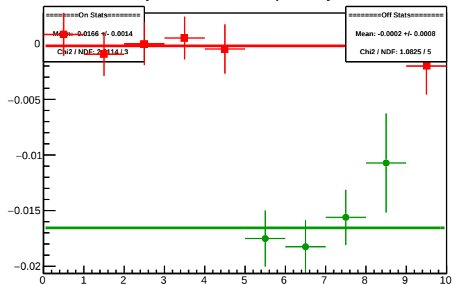
Cycle 4508.2: Multiplet Asyms
