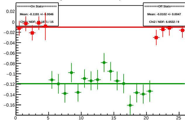
Cycle 4508.10: Multiplet Diffs
