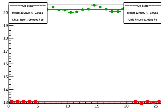
Cycle 4508.10: Multiplet Sums
