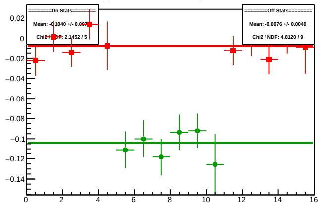
Cycle 4508.9: Multiplet Diffs
