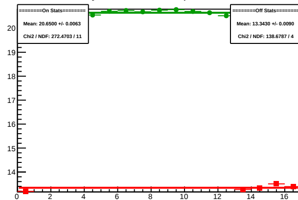
Cycle 4508.3: Multiplet Sums
