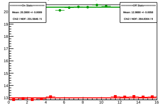
Cycle 4508.9: Multiplet Sums
