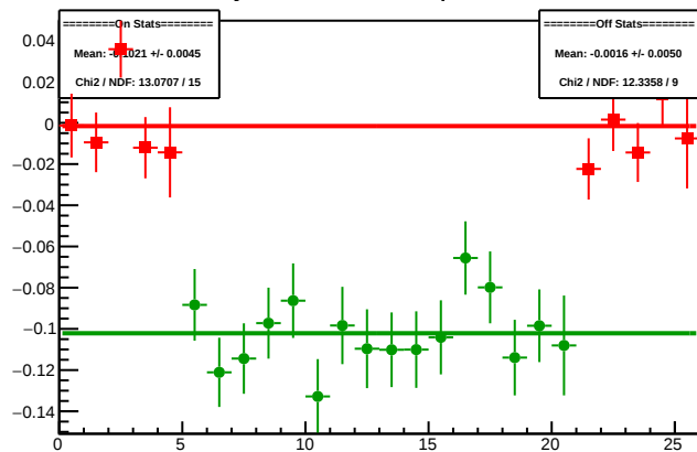
Cycle 4508.8: Multiplet Diffs
