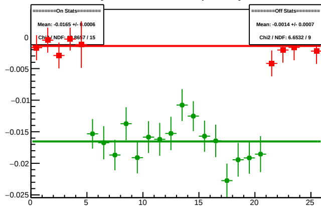
Cycle 4508.10: Multiplet Asyms
