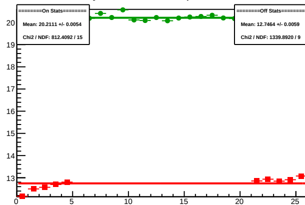
Cycle 4508.8: Multiplet Sums
