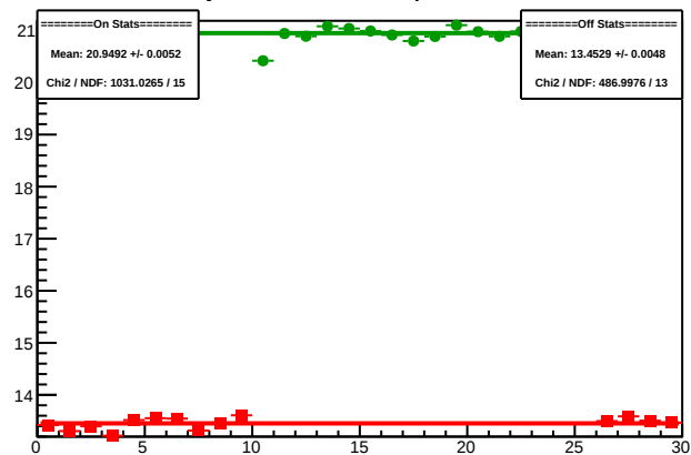
Cycle 4508.5: Multiplet Sums
