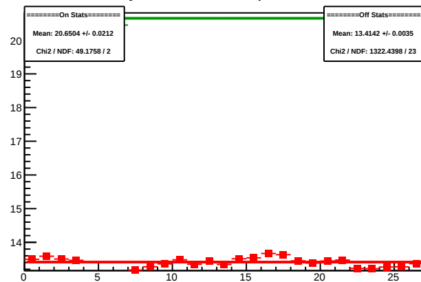
Cycle 4508.6: Multiplet Sums
