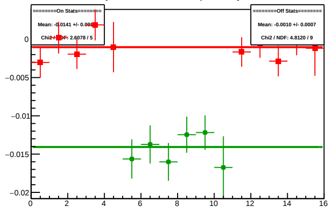
Cycle 4508.9: Multiplet Asyms
