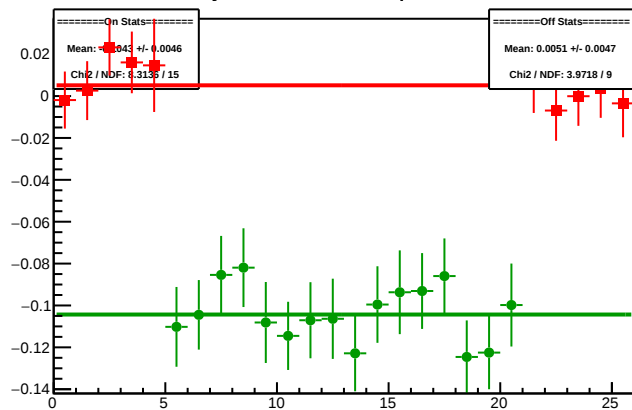
Cycle 4508.1: Multiplet Diffs
