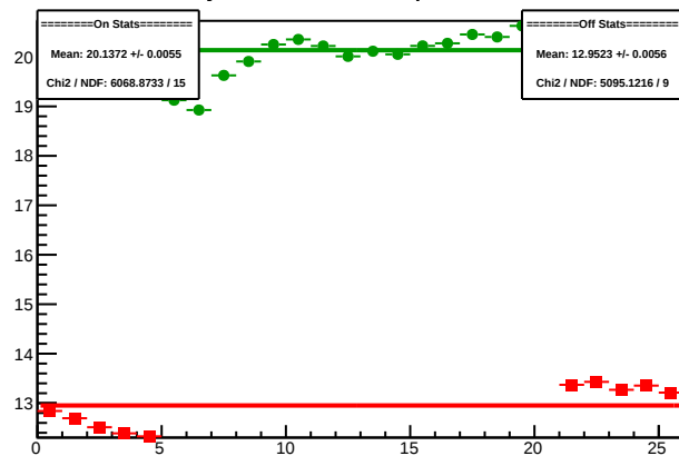
Cycle 4508.1: Multiplet Sums
