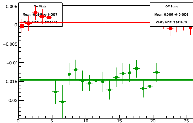
Cycle 4508.1: Multiplet Asyms
