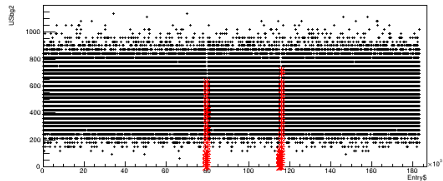
Run 4522, quartetwise: USbg2 vs time
