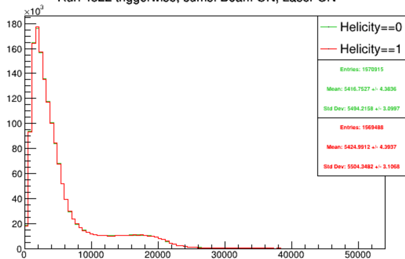
Run 4522 triggerwise, sums: Beam ON, Laser ON
