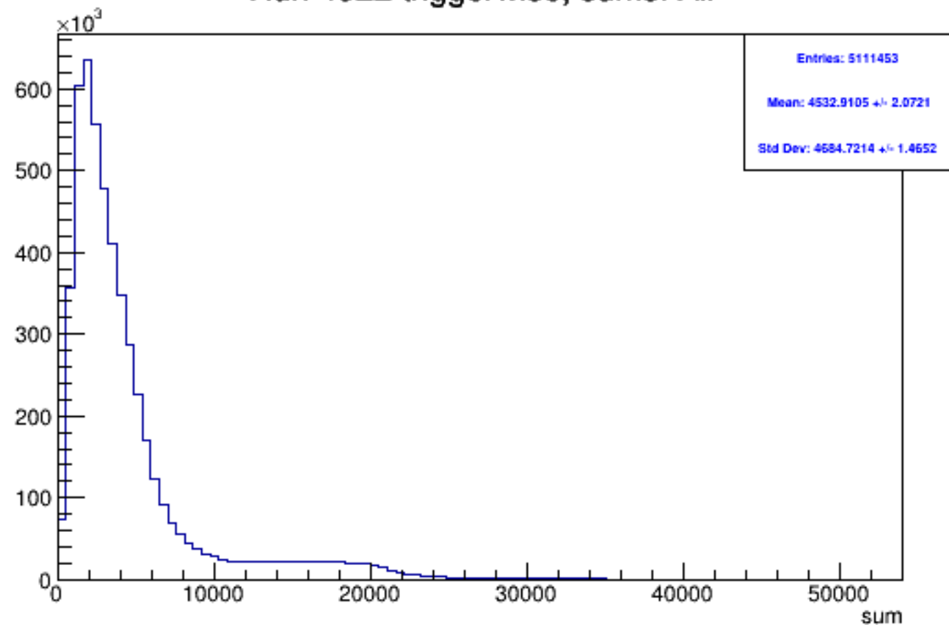
Run 4522 triggerwise, sums: All
