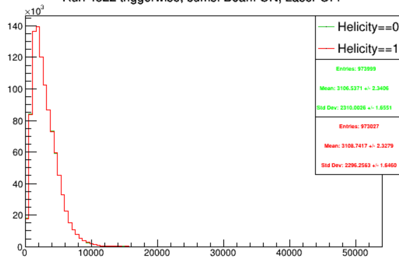
Run 4522 triggerwise, sums: Beam ON, Laser OFF
