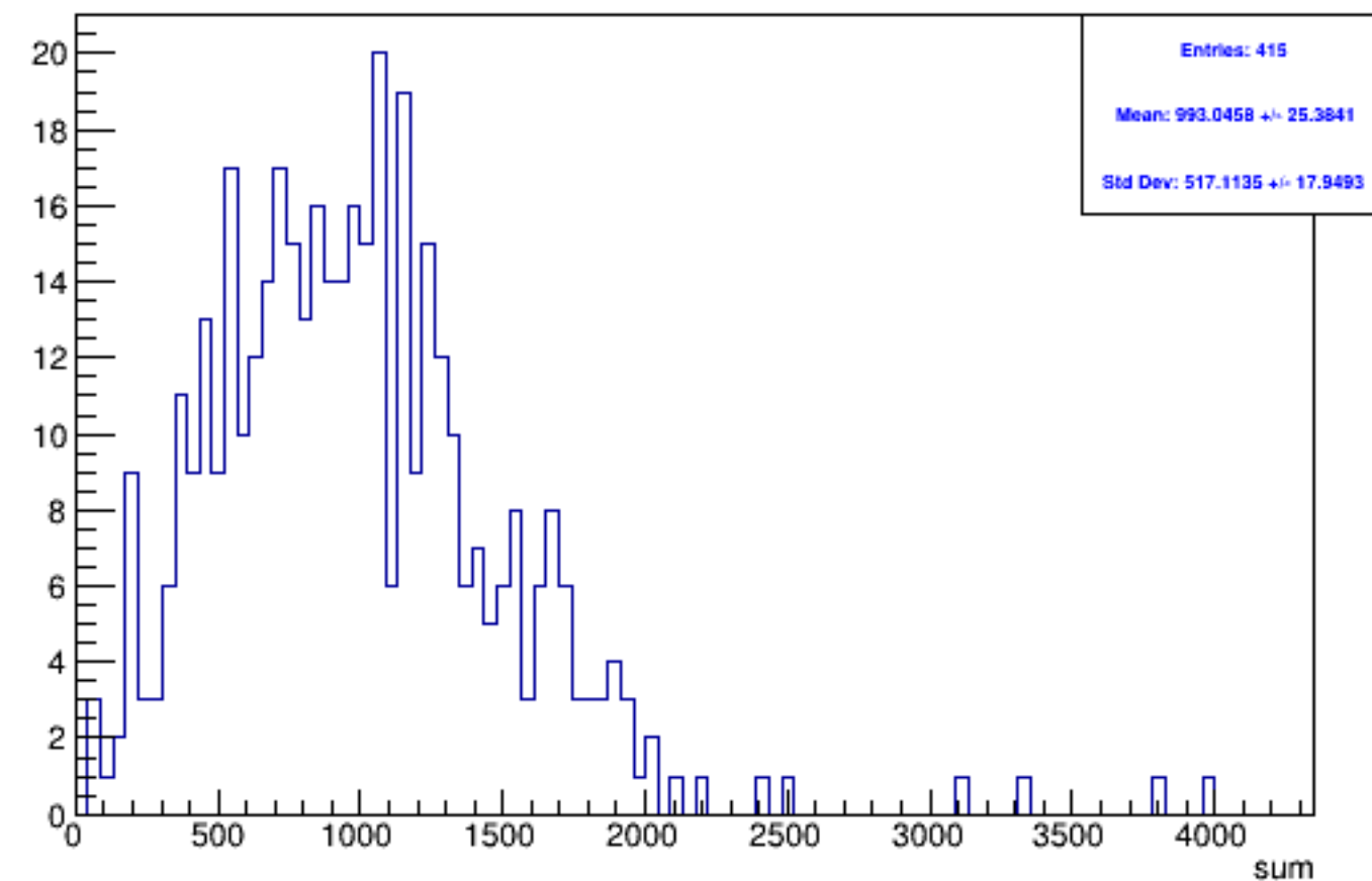
Run 4522 triggerwise, sums: Beam OFF
