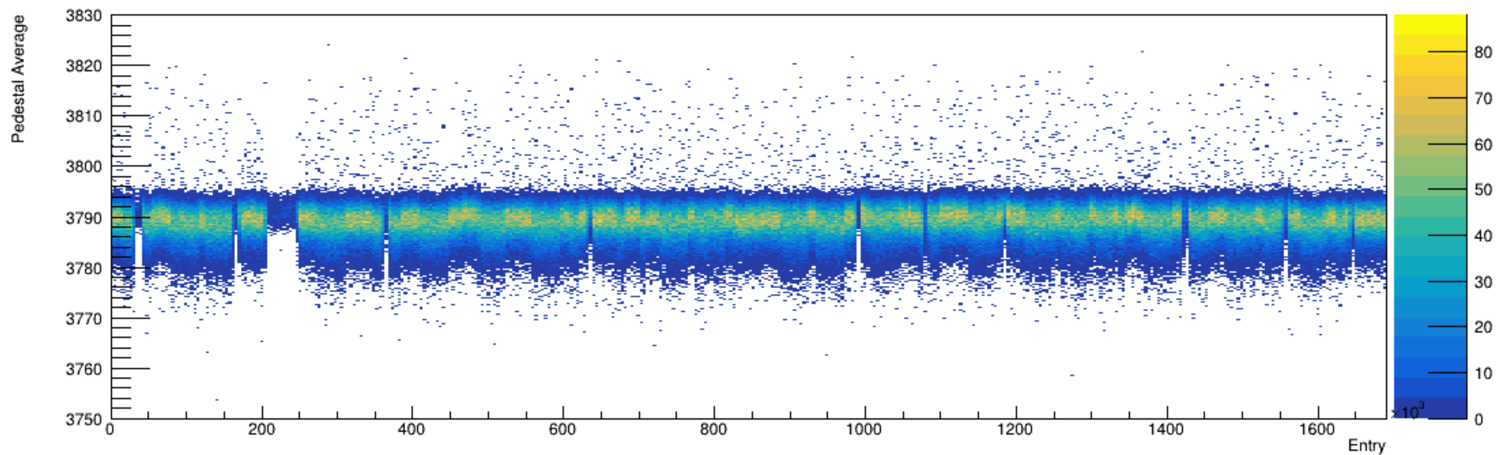
Run 4530, snapshots: Pedestal vs. Time
