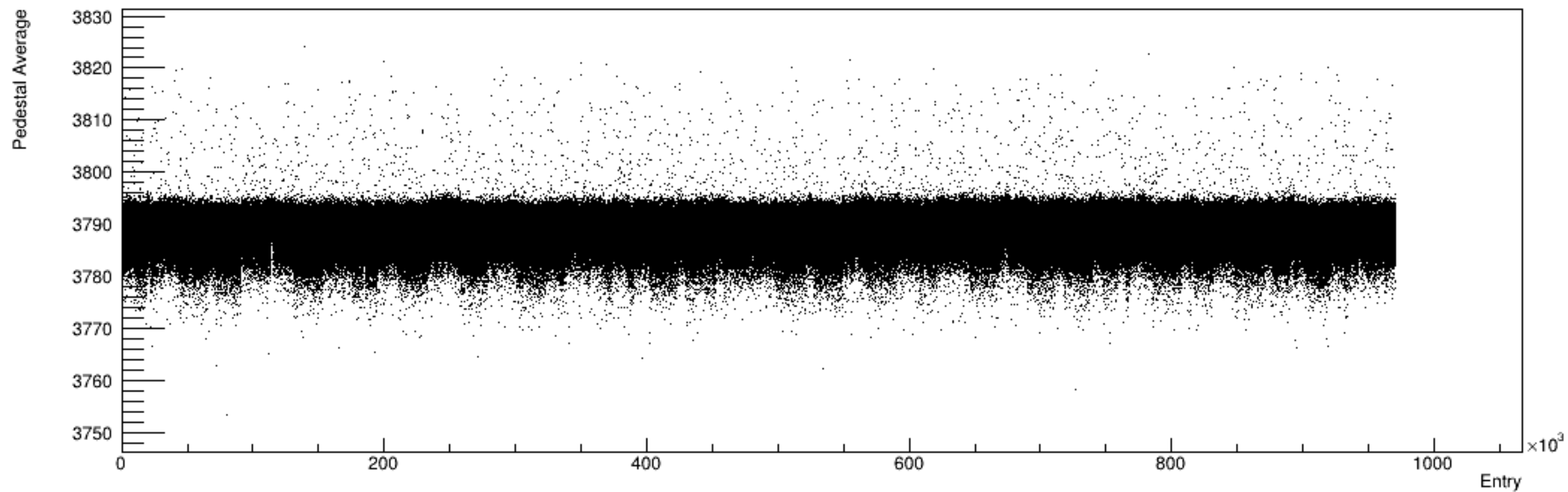
Run 4530, snapshots: Pedestal vs. Time
