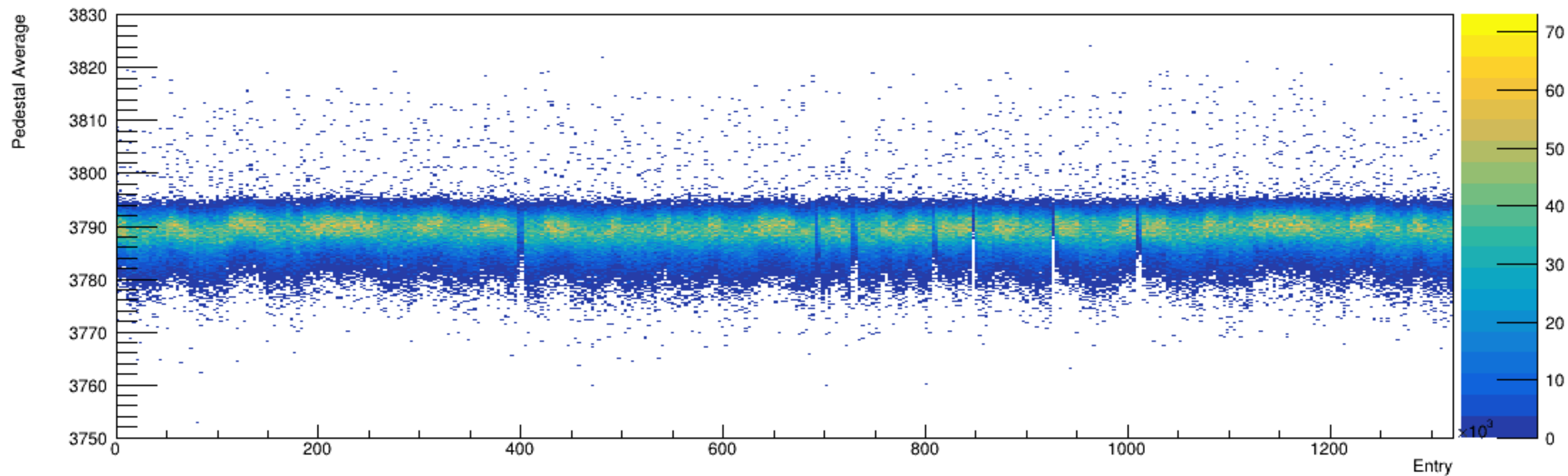
Run 4531, snapshots: Pedestal vs. Time
