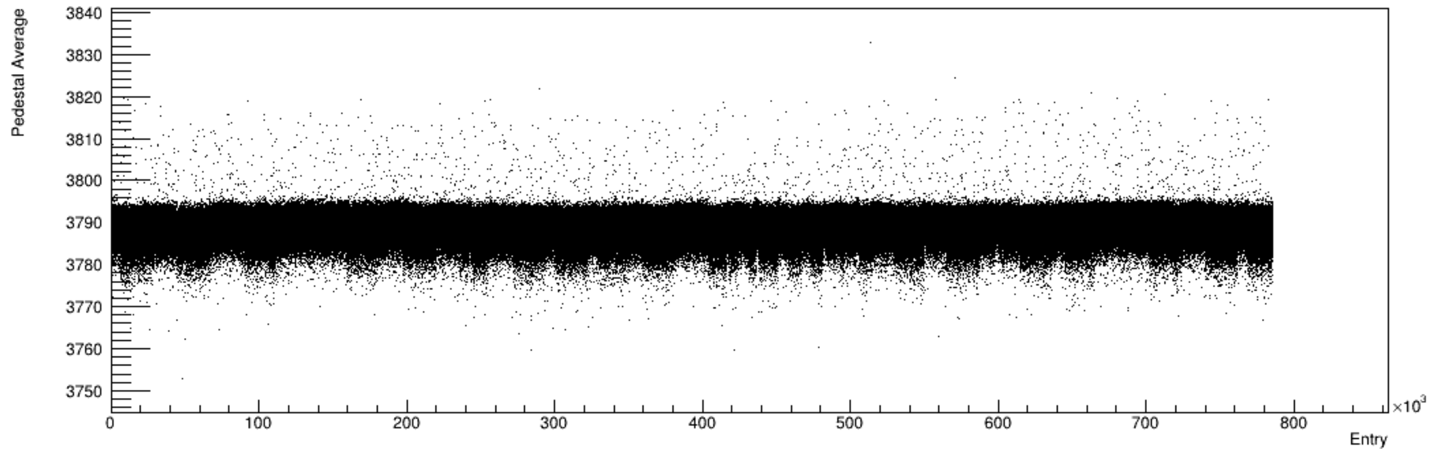
Run 4531, snapshots: Pedestal vs. Time
