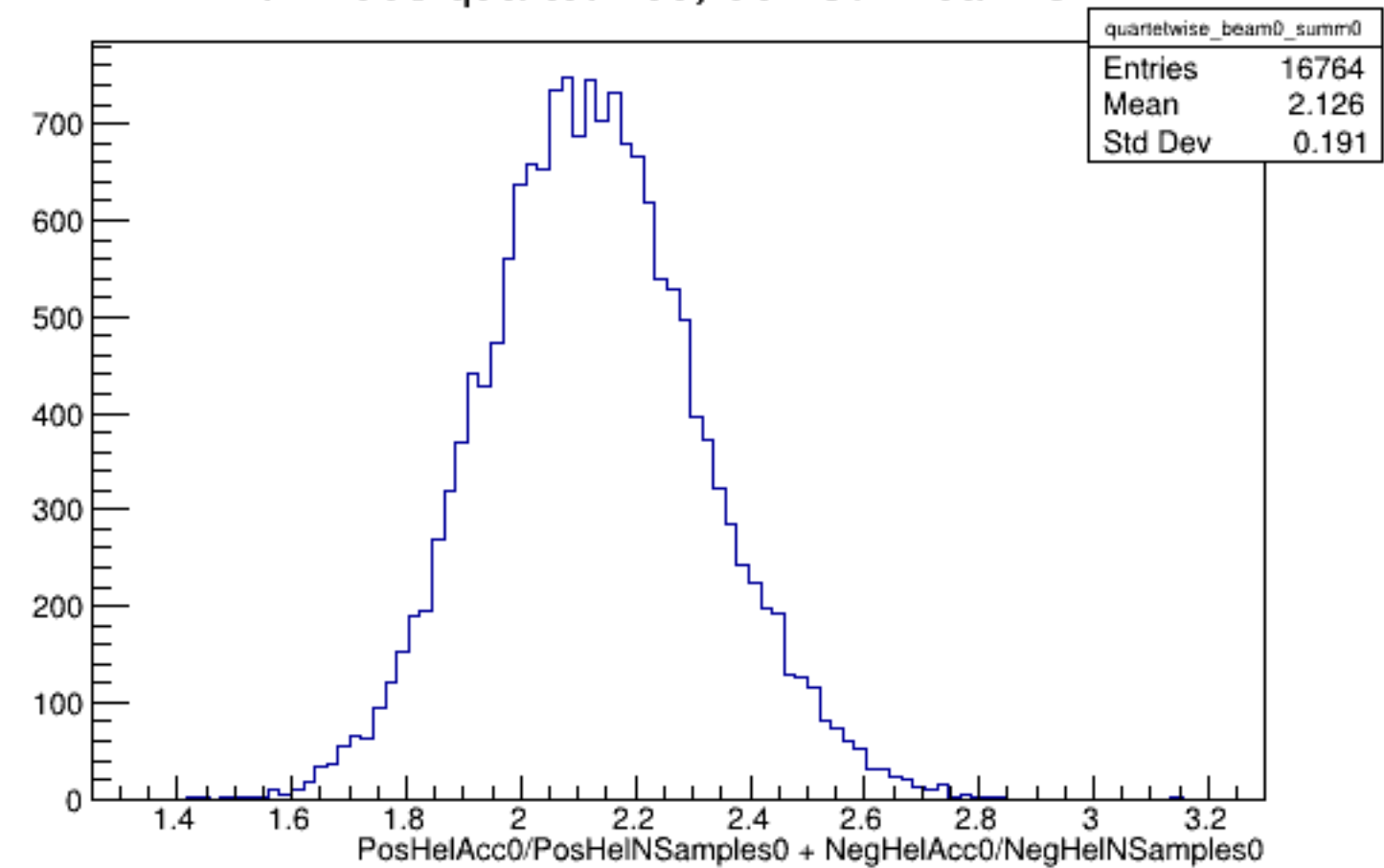
Run 4538 quartetwise, Sums0: Beam OFF
