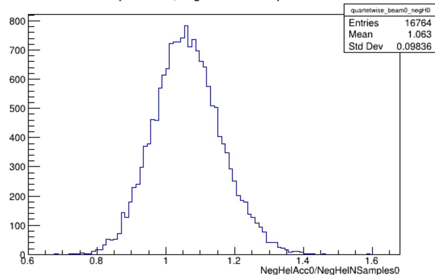
Run 4538 quartetwise, NegHelAcc0/NSamples0: Beam OFF
