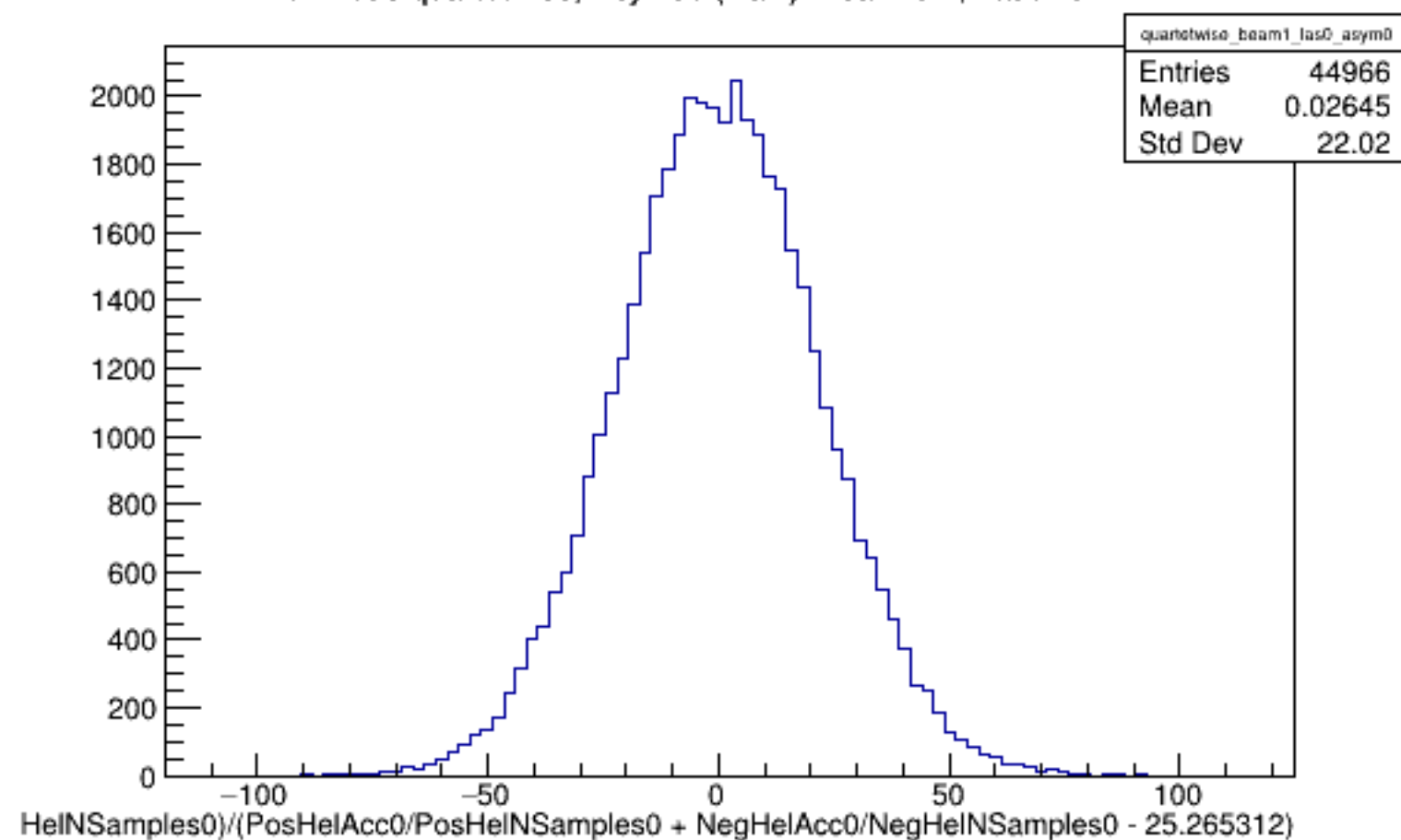
Run 4538 quartetwise, Asyms0 (Raw): Beam ON, Laser OFF
