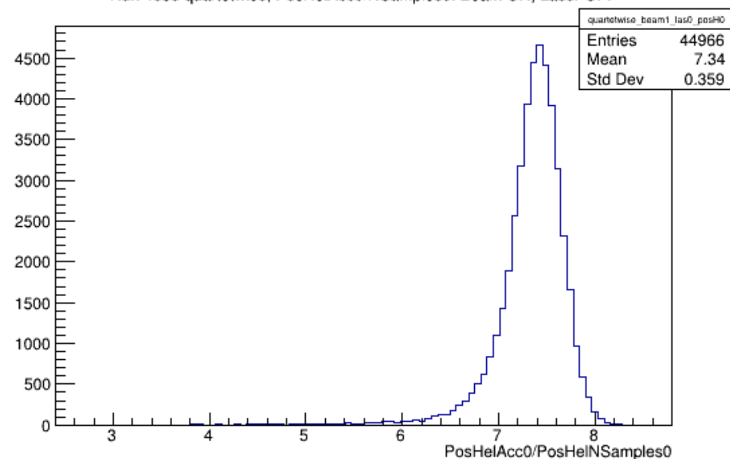
Run 4538 quartetwise, PosHelAcc0/NSamples0: Beam ON, Laser OFF
