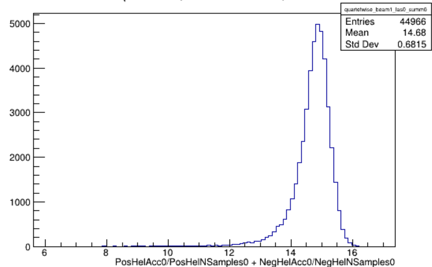
Run 4538 quartetwise, Sums0: Beam ON, Laser OFF
