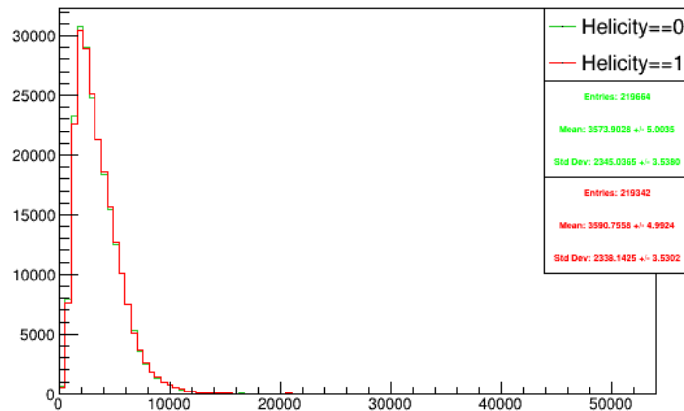
Run 4539 triggerwise, sums: Beam ON, Laser OFF
