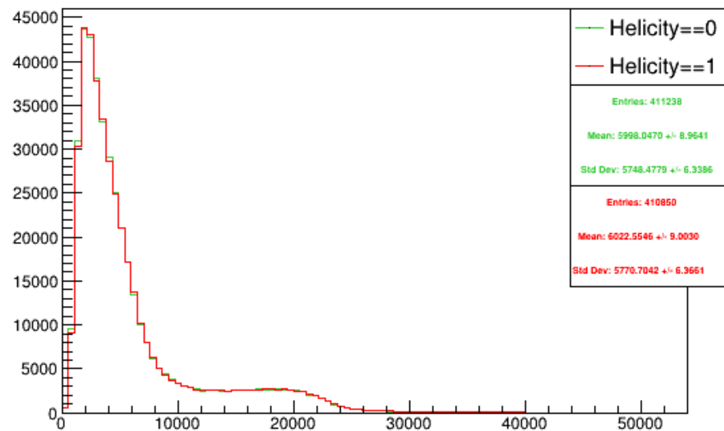
Run 4539 triggerwise, sums: Beam ON, Laser ON
