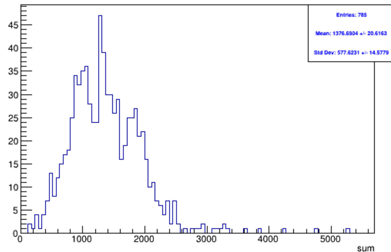
Run 4539 triggerwise, sums: Beam OFF
