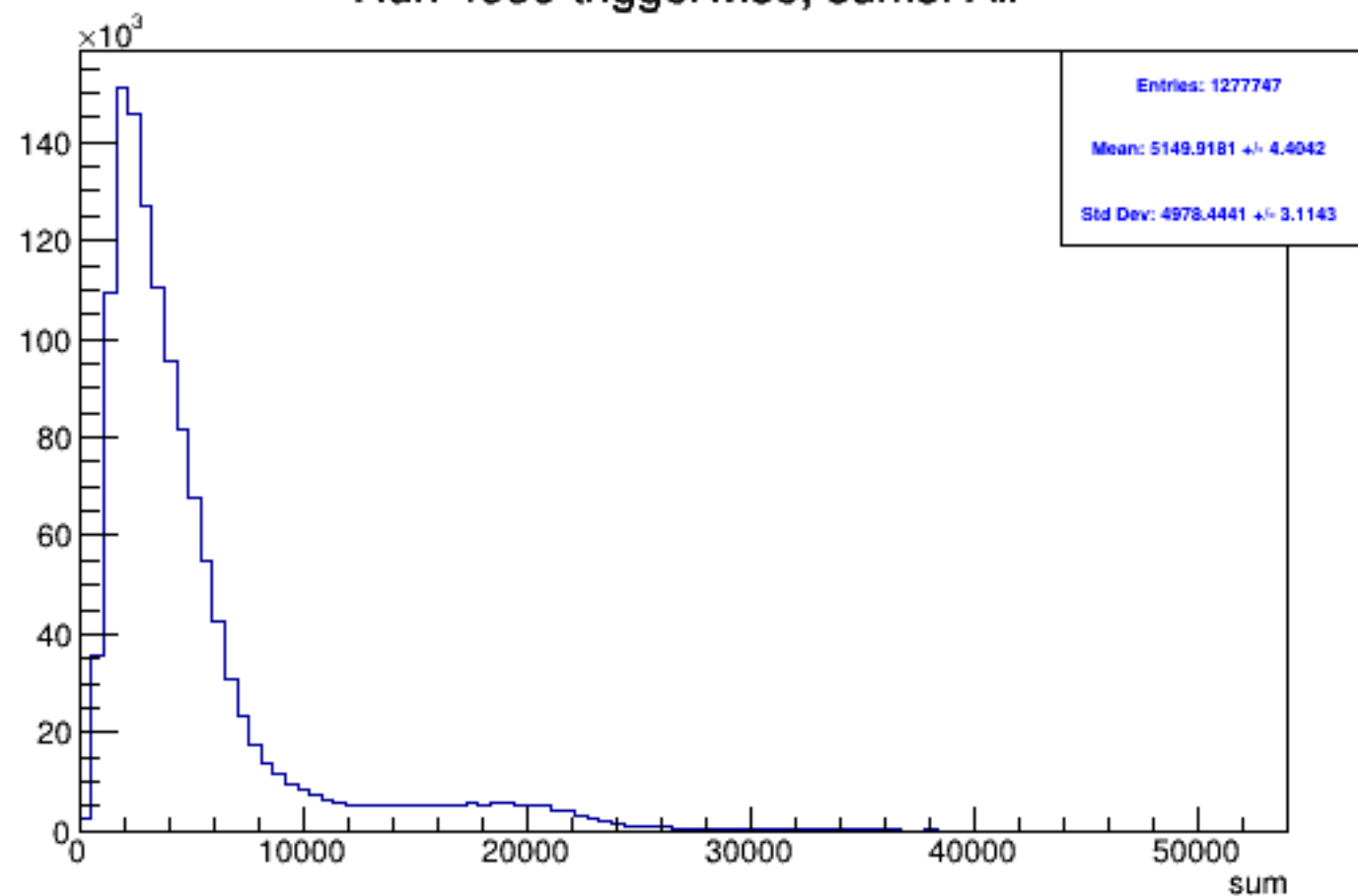
Run 4539 triggerwise, sums: All
