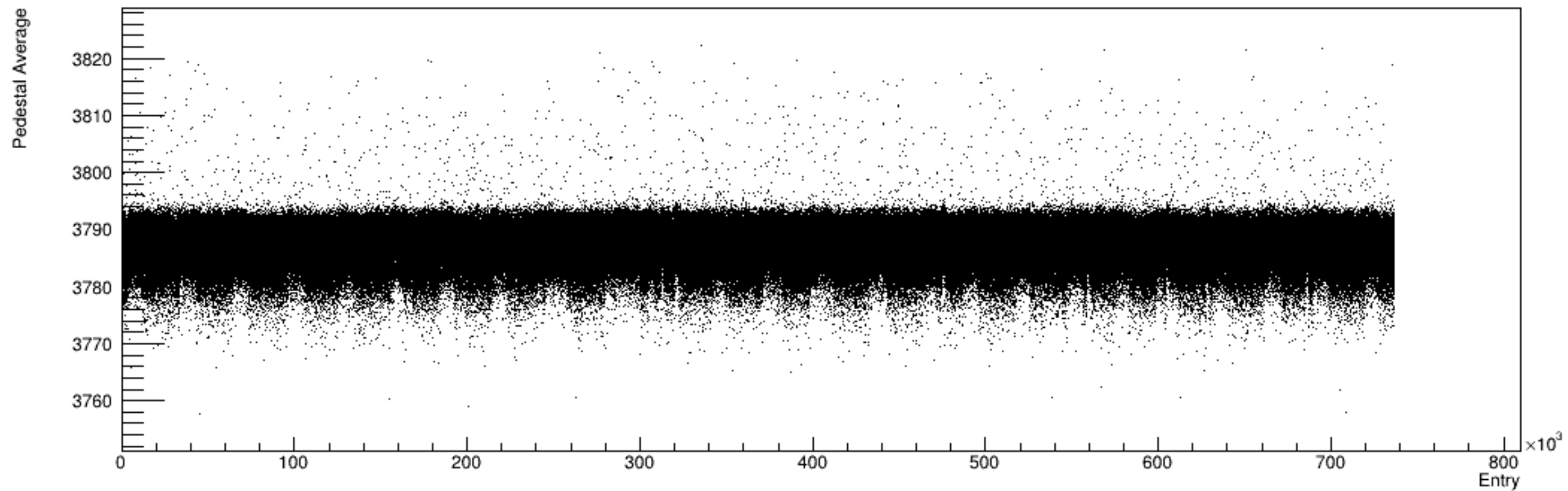
Run 4540, snapshots: Pedestal vs. Time
