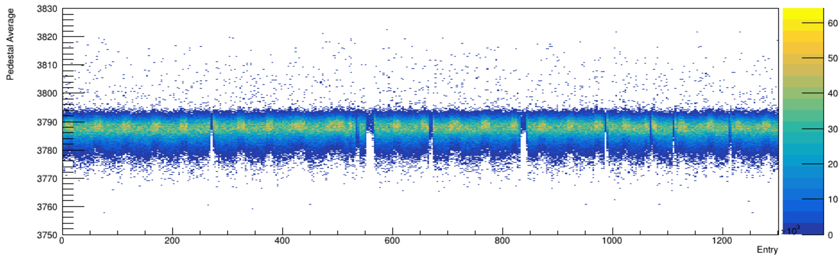
Run 4540, snapshots: Pedestal vs. Time
