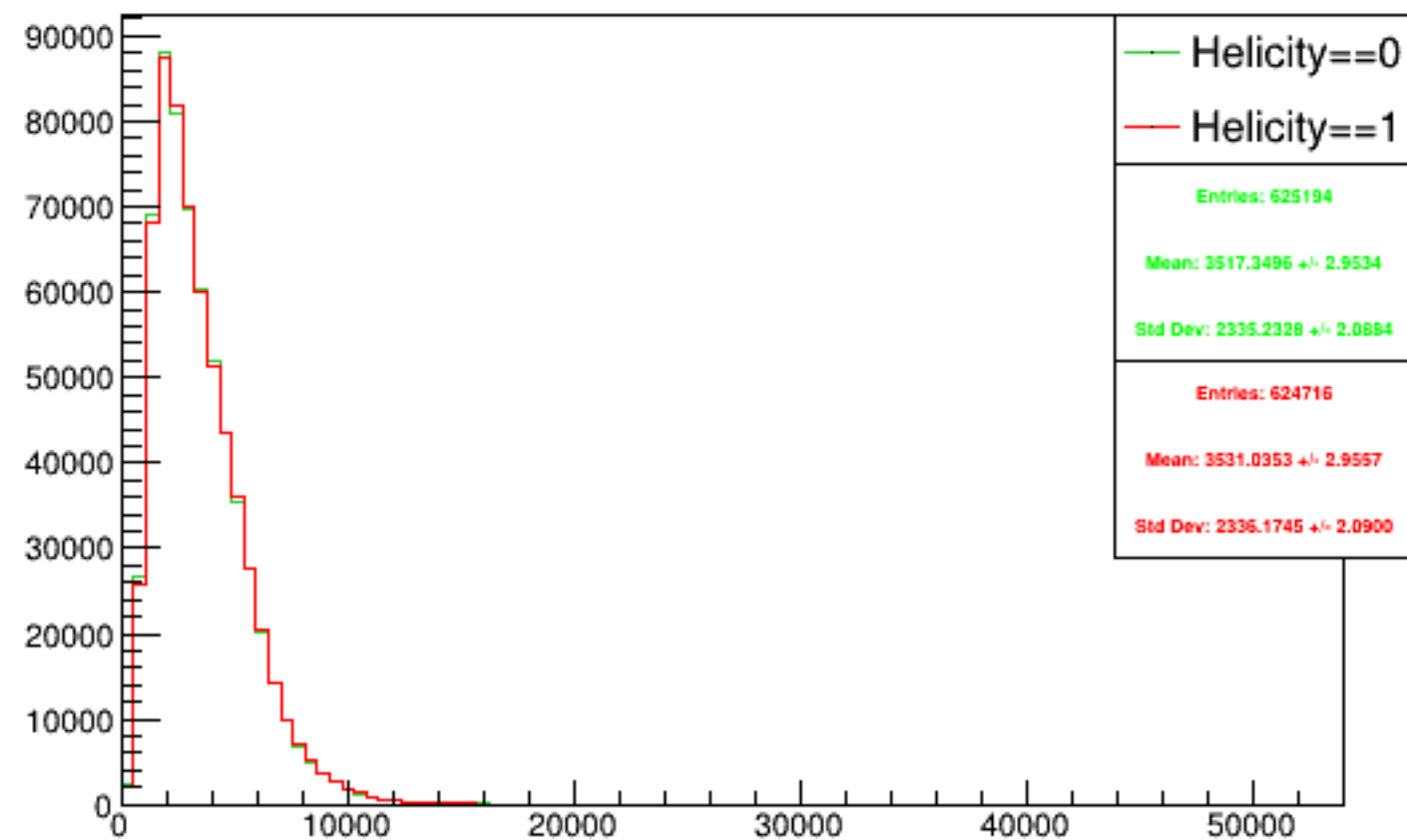
Run 4540 triggerwise, sums: Beam ON, Laser OFF
