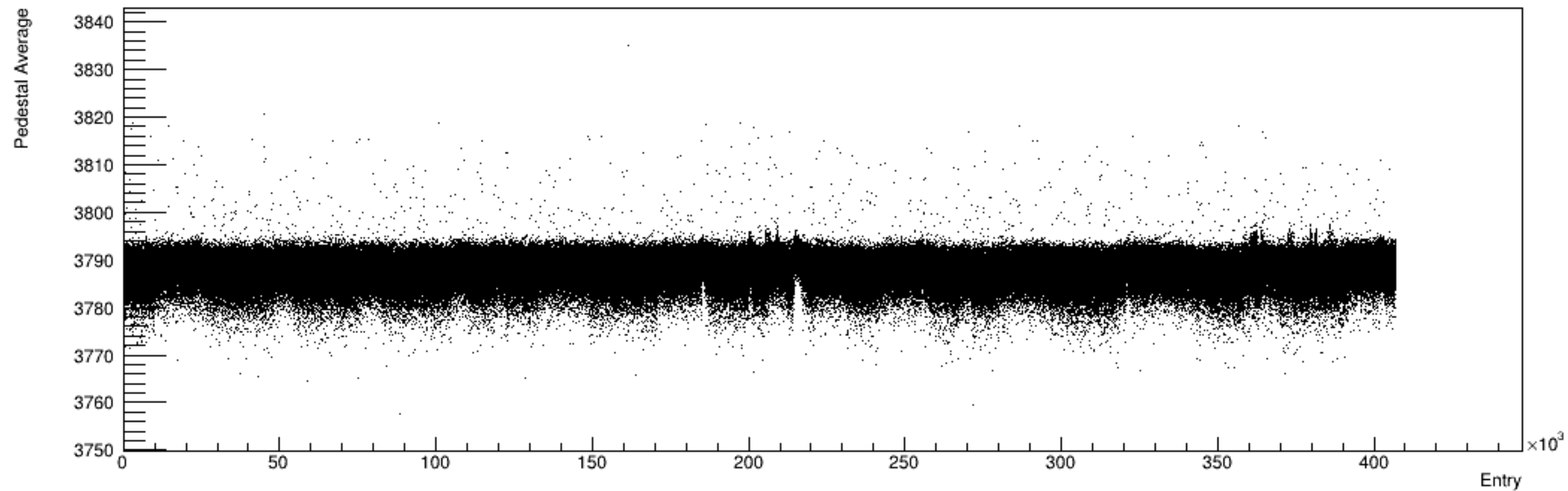
Run 4544, snapshots: Pedestal vs. Time
