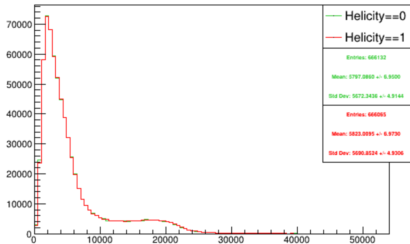
Run 4544 triggerwise, sums: Beam ON, Laser ON
