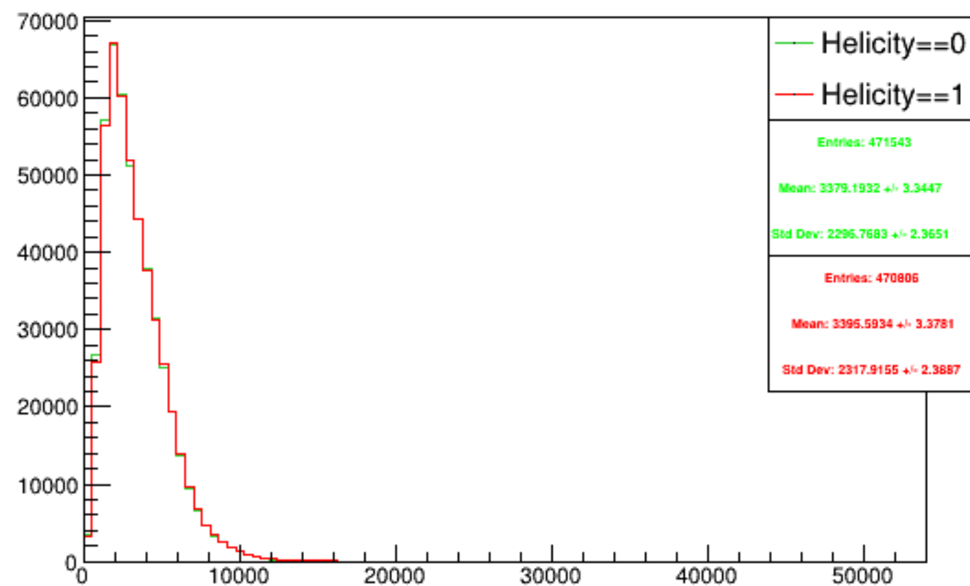
Run 4544 triggerwise, sums: Beam ON, Laser OFF
