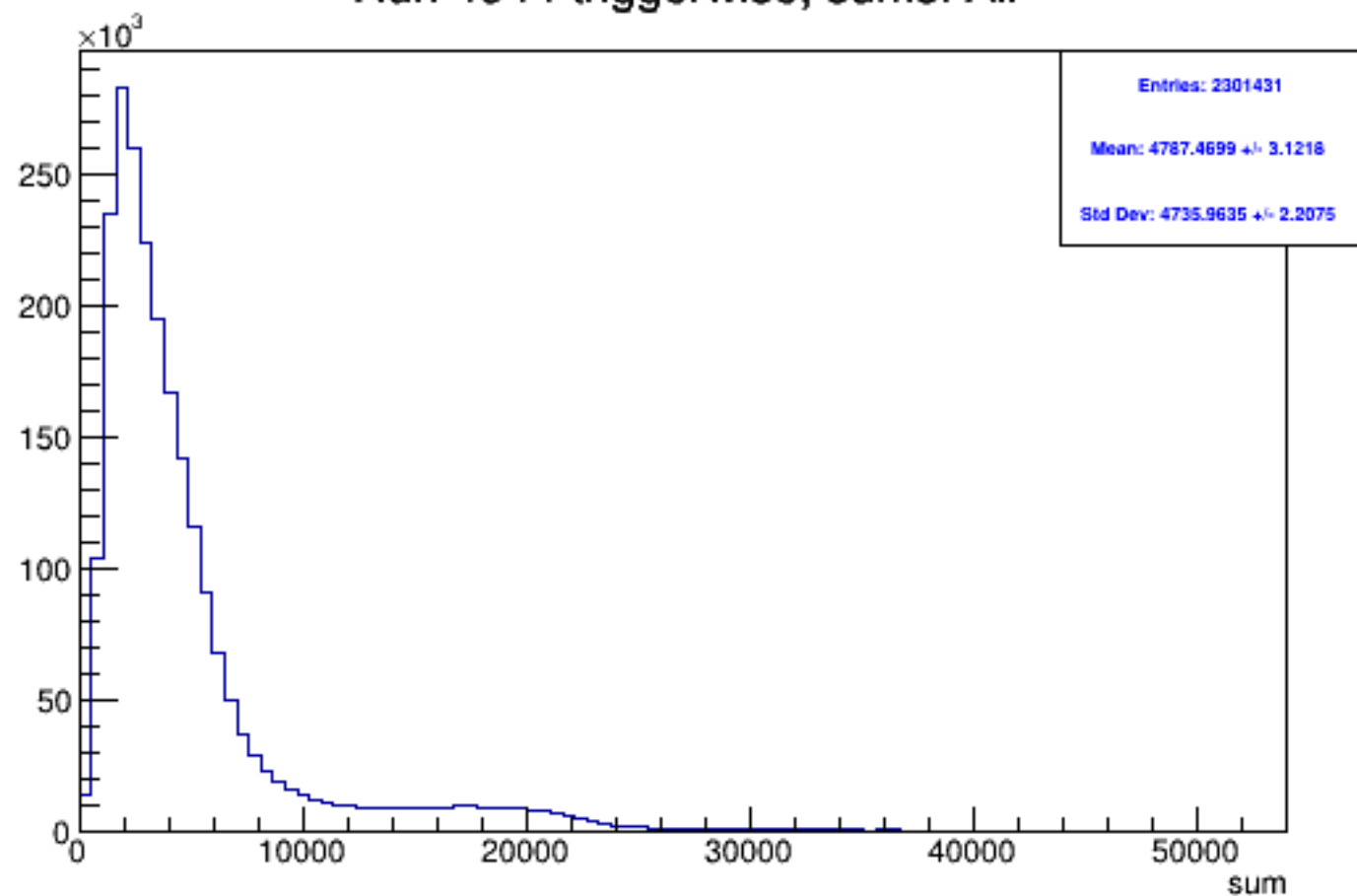
Run 4544 triggerwise, sums: All
