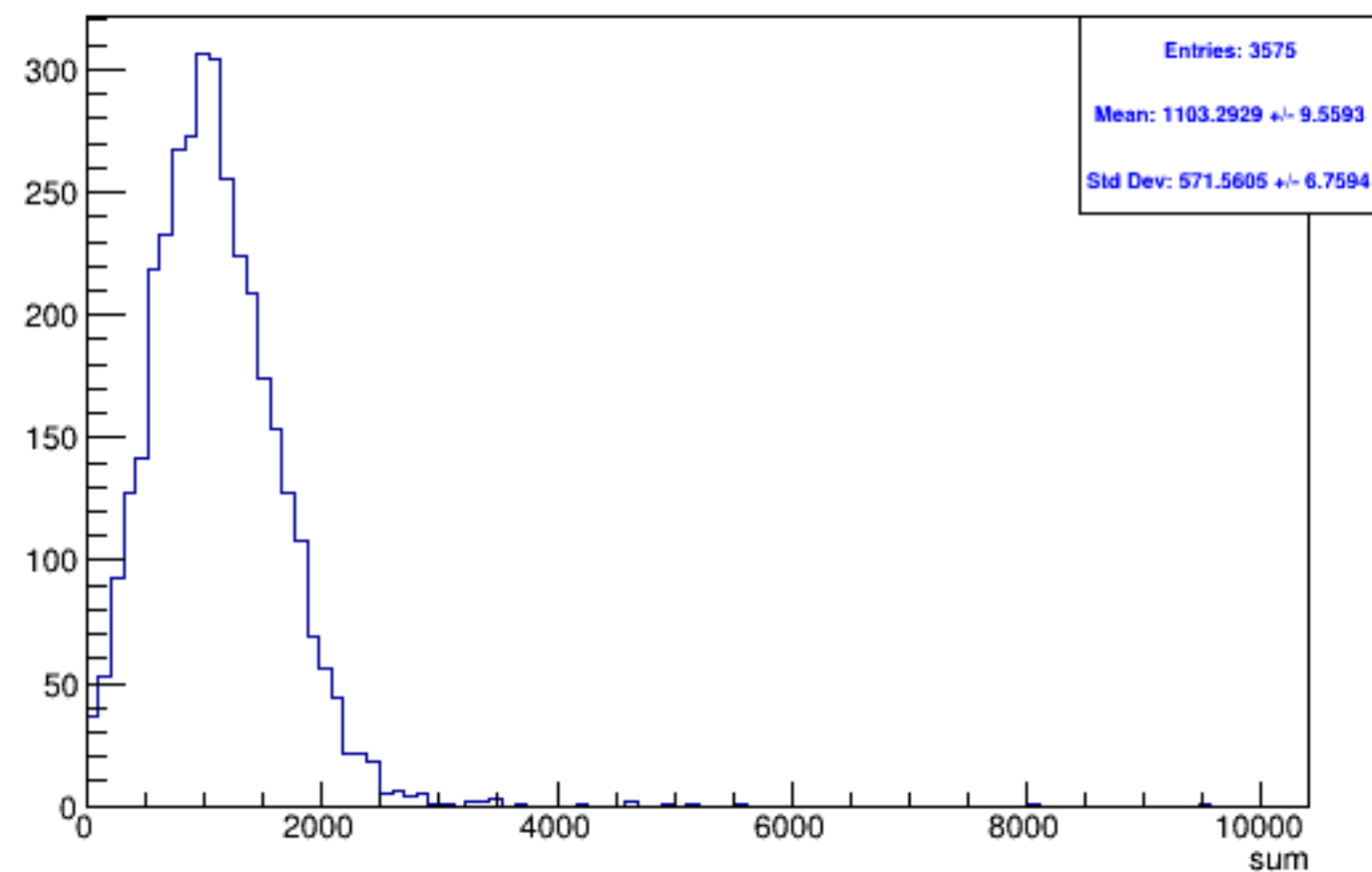
Run 4544 triggerwise, sums: Beam OFF
