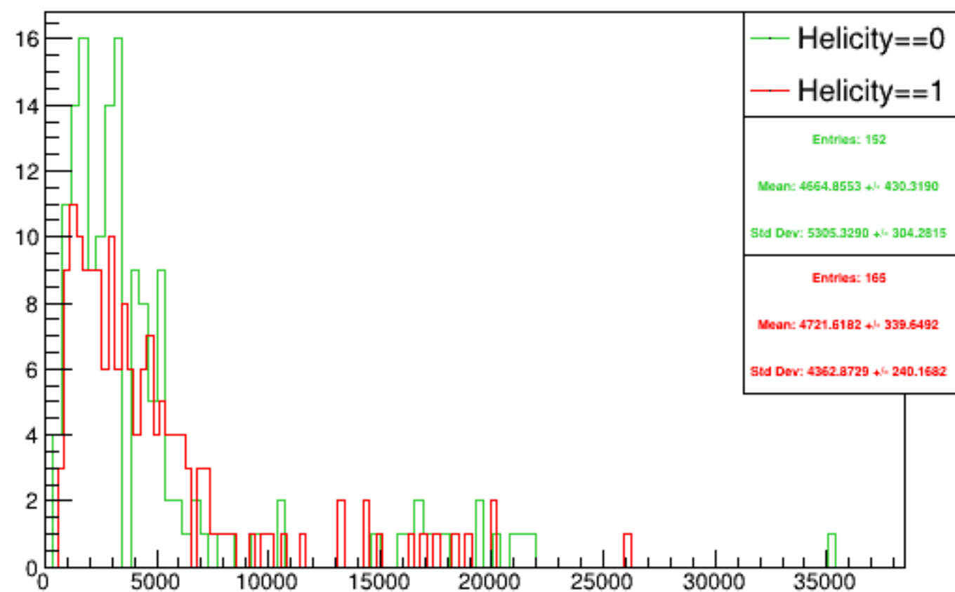
Run 4547 triggerwise, sums: Beam ON, Laser ON
