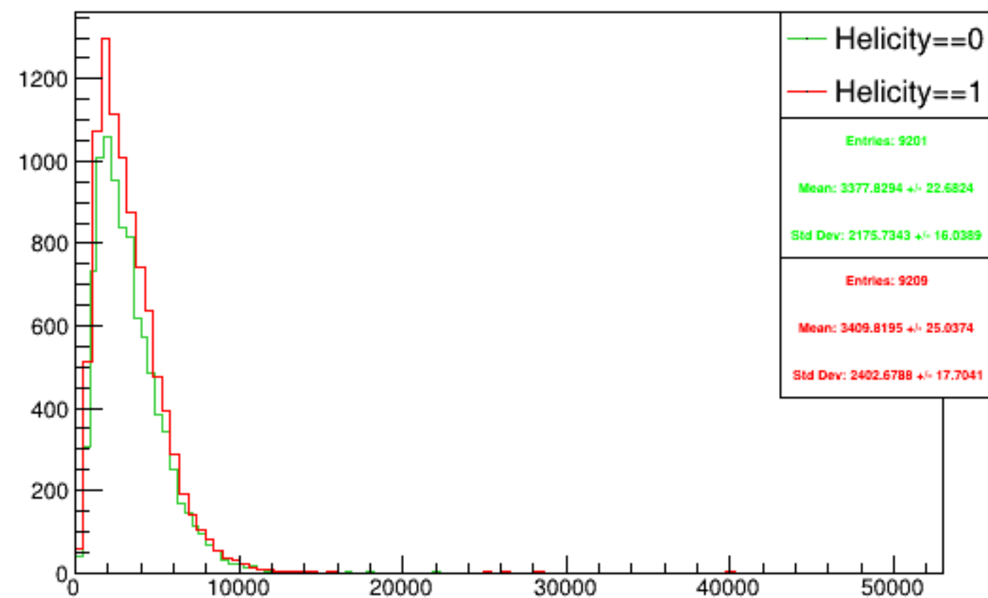
Run 4547 triggerwise, sums: Beam ON, Laser OFF
