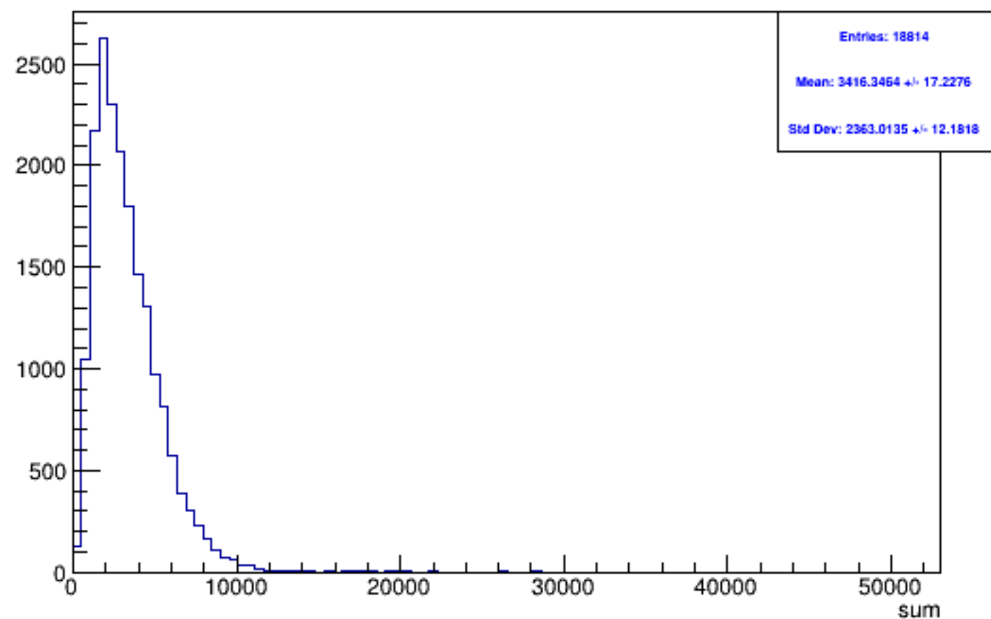
Run 4547 triggerwise, sums: All
