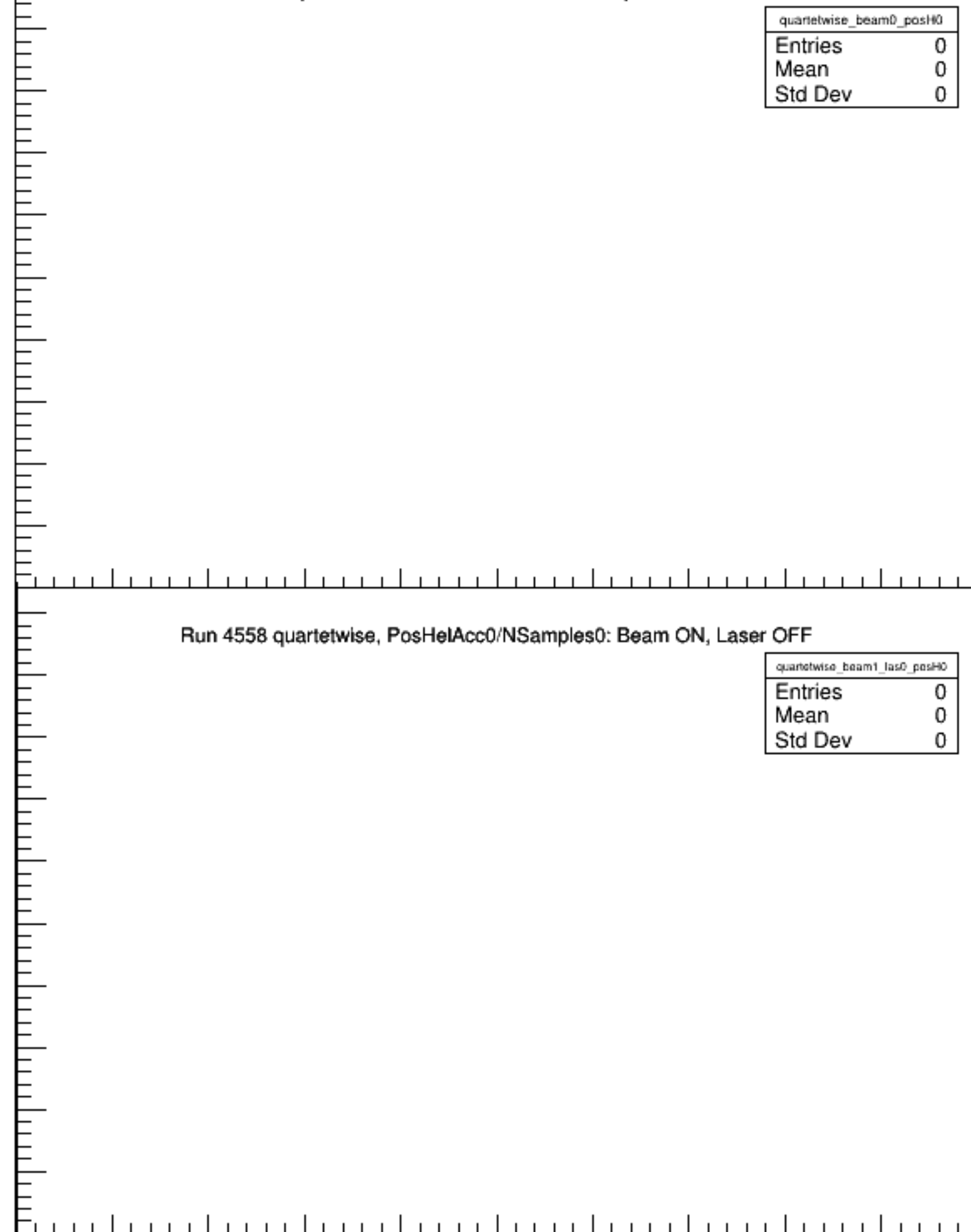
Run 4558 quartetwise, PosHelAcc0/NSamples0: Beam OFF
