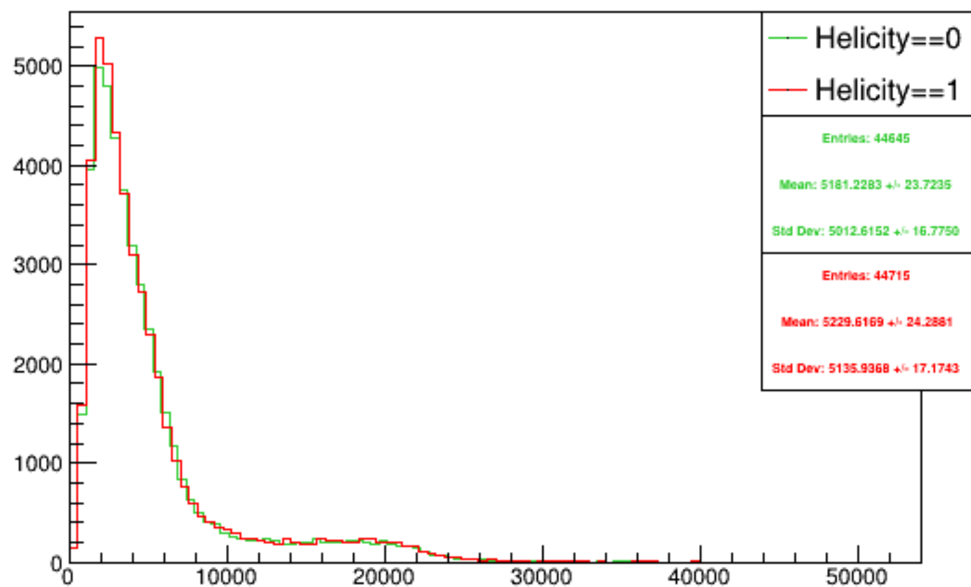
Run 4558 triggerwise, sums: Beam ON, Laser ON
