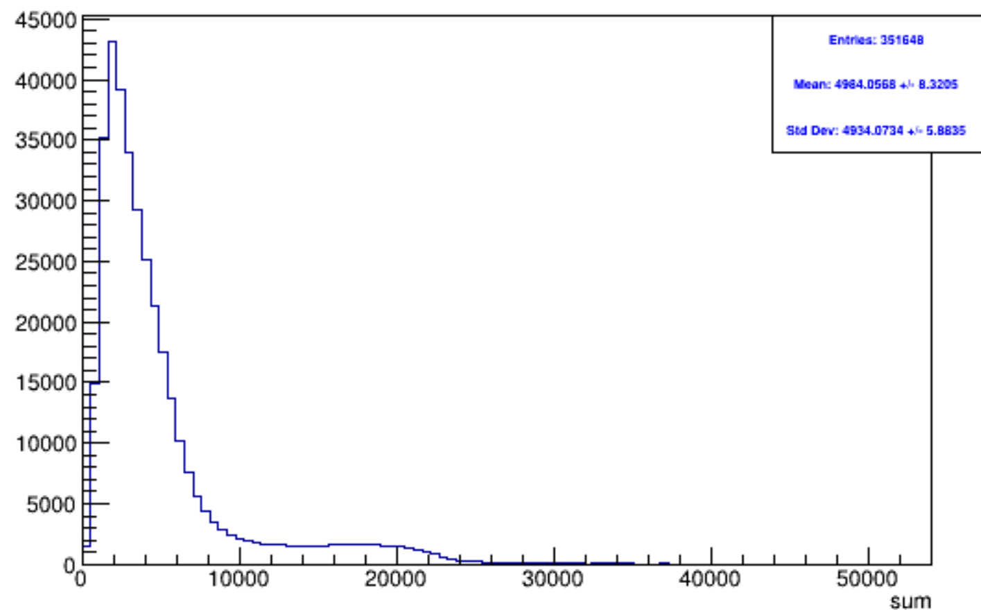
Run 4558 triggerwise, sums: All
