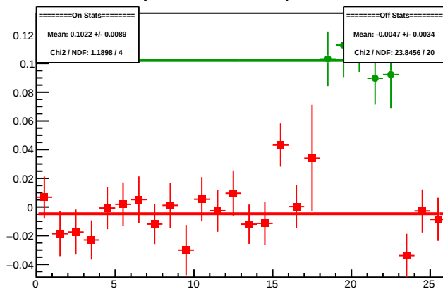
Cycle 4562.16: Multiplet Diffs
