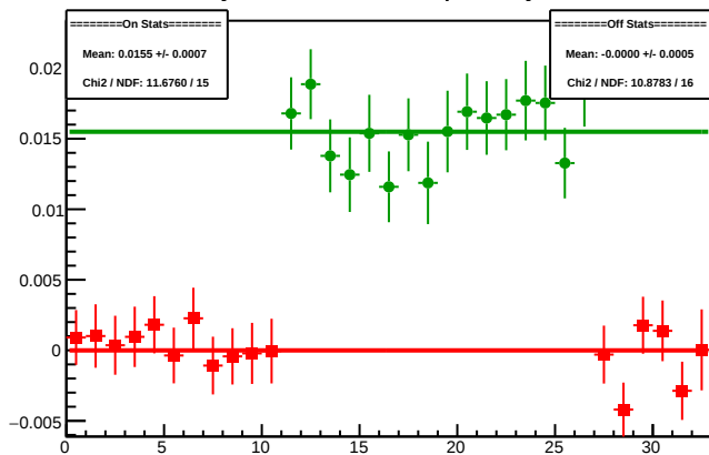
Cycle 4562.24: Multiplet Asyms
