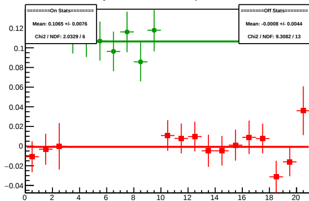
Cycle 4562.4: Multiplet Diffs
