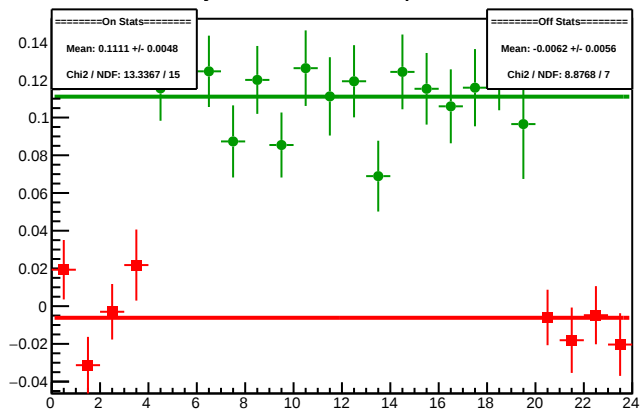
Cycle 4562.21: Multiplet Diffs
