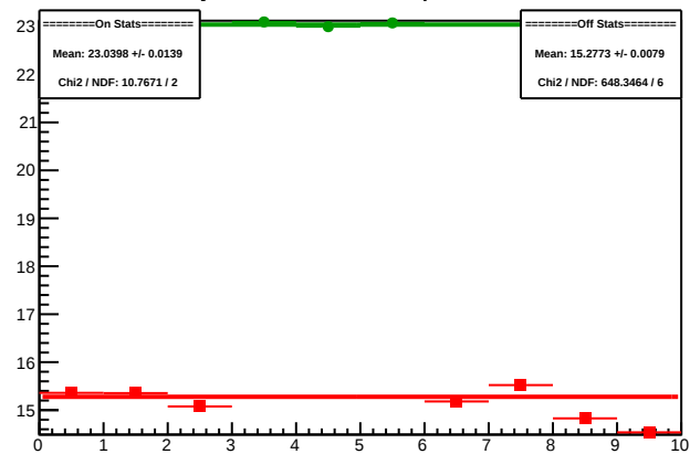
Cycle 4562.17: Multiplet Sums
