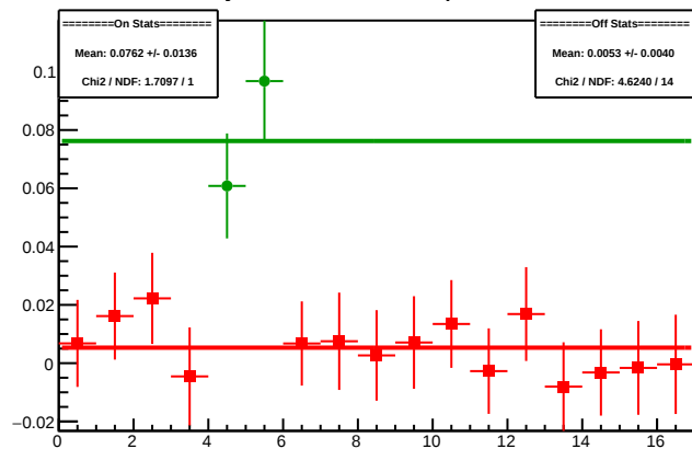
Cycle 4562.23: Multiplet Diffs
