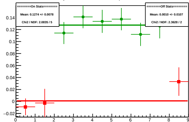
Cycle 4562.3: Multiplet Diffs
