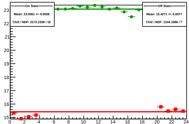
Cycle 4562.22: Multiplet Sums
