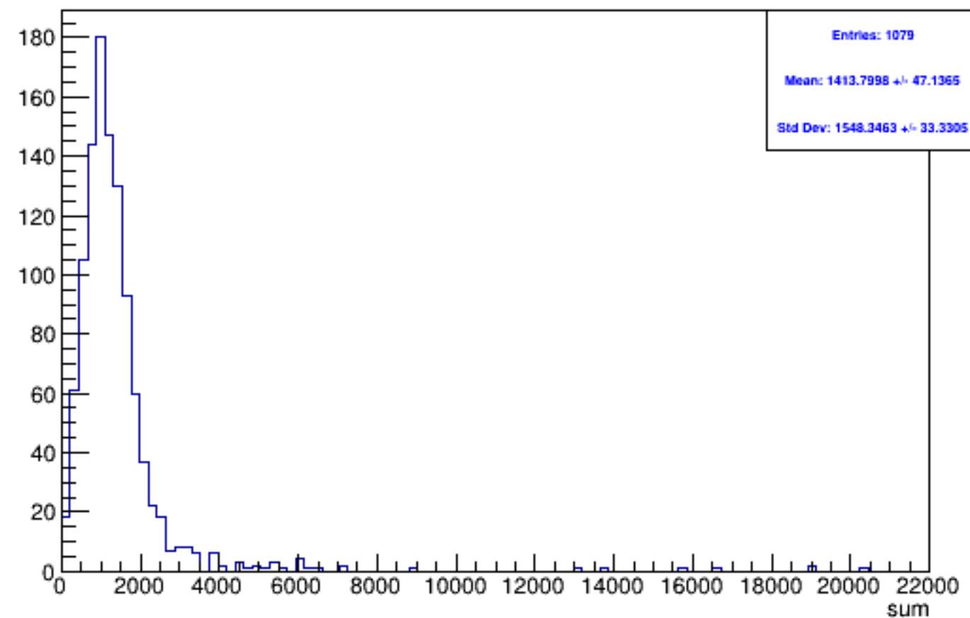
Run 4568 triggerwise, sums: Beam OFF
