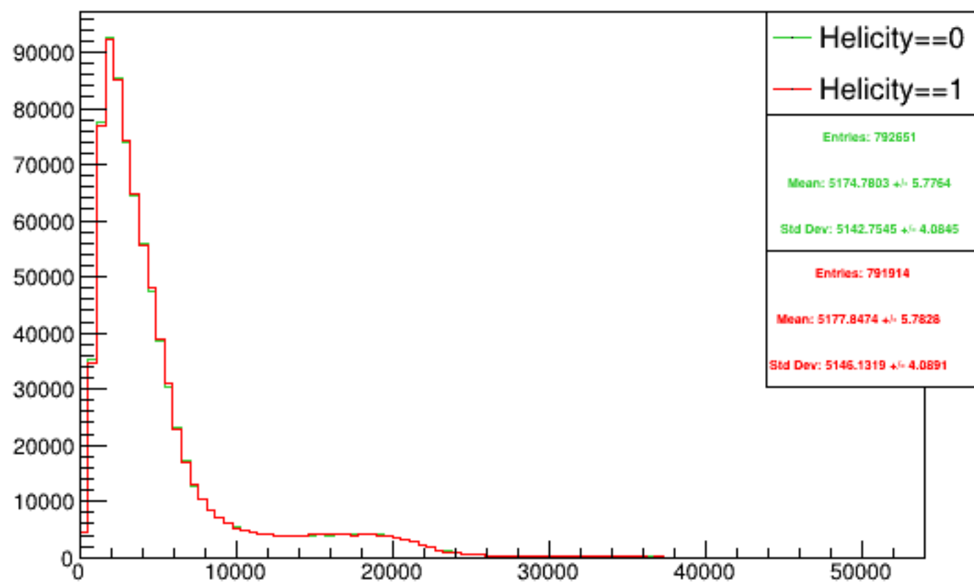
Run 4568 triggerwise, sums: Beam ON, Laser ON
