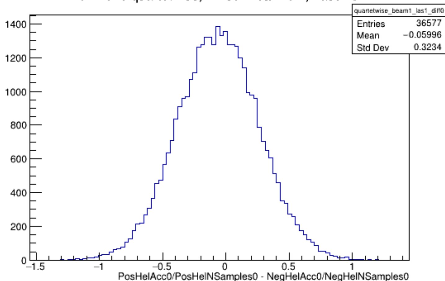
Run 4570 quartetwise, Diffs0: Beam ON, Laser ON
