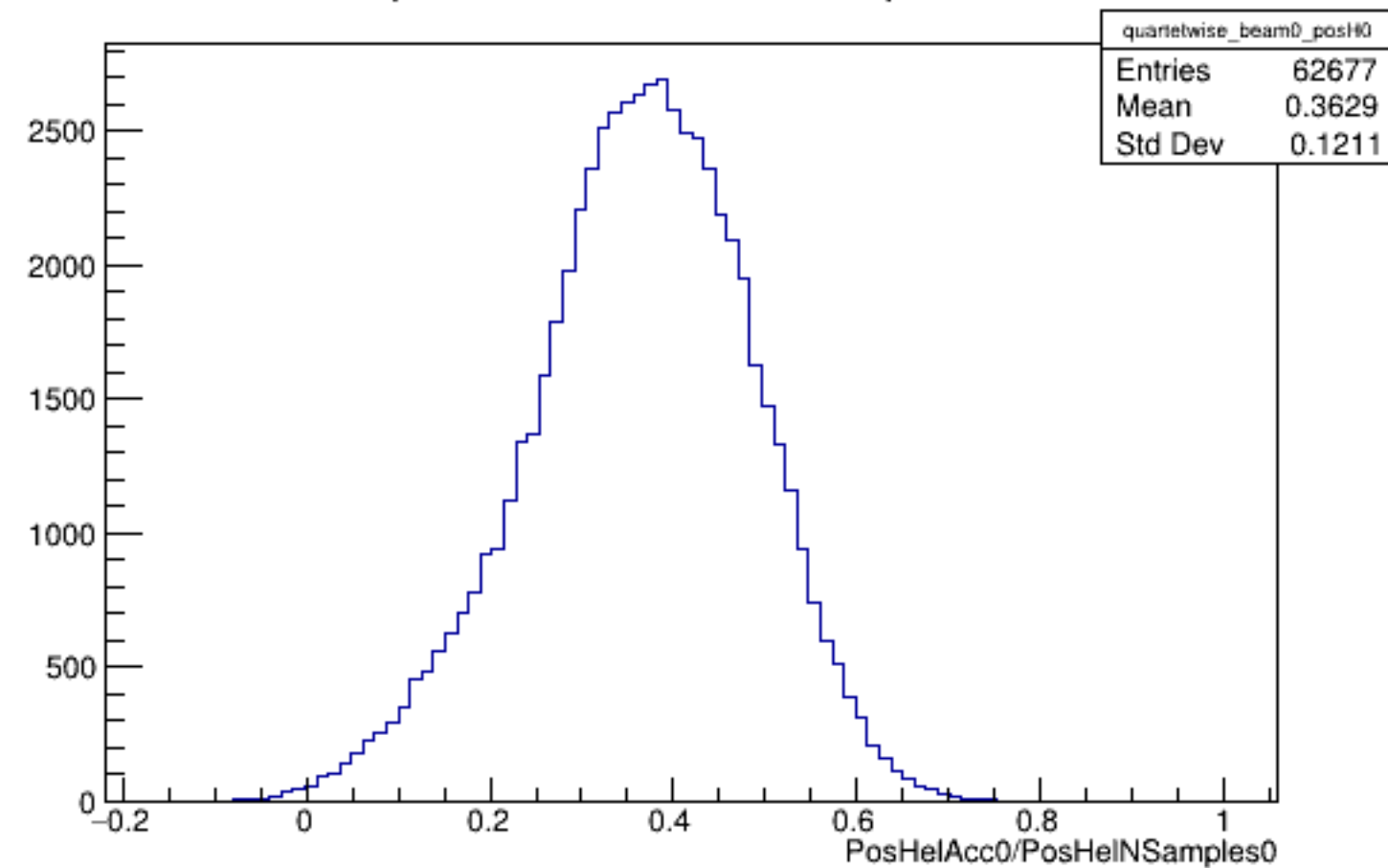
Run 4570 quartetwise, PosHelAcc0/NSamples0: Beam OFF
