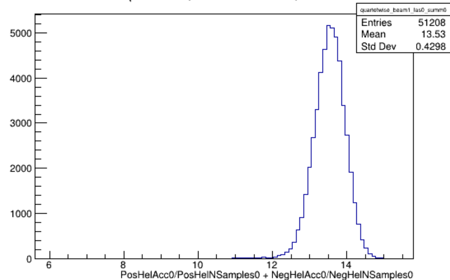
Run 4570 quartetwise, Sums0: Beam ON, Laser OFF
