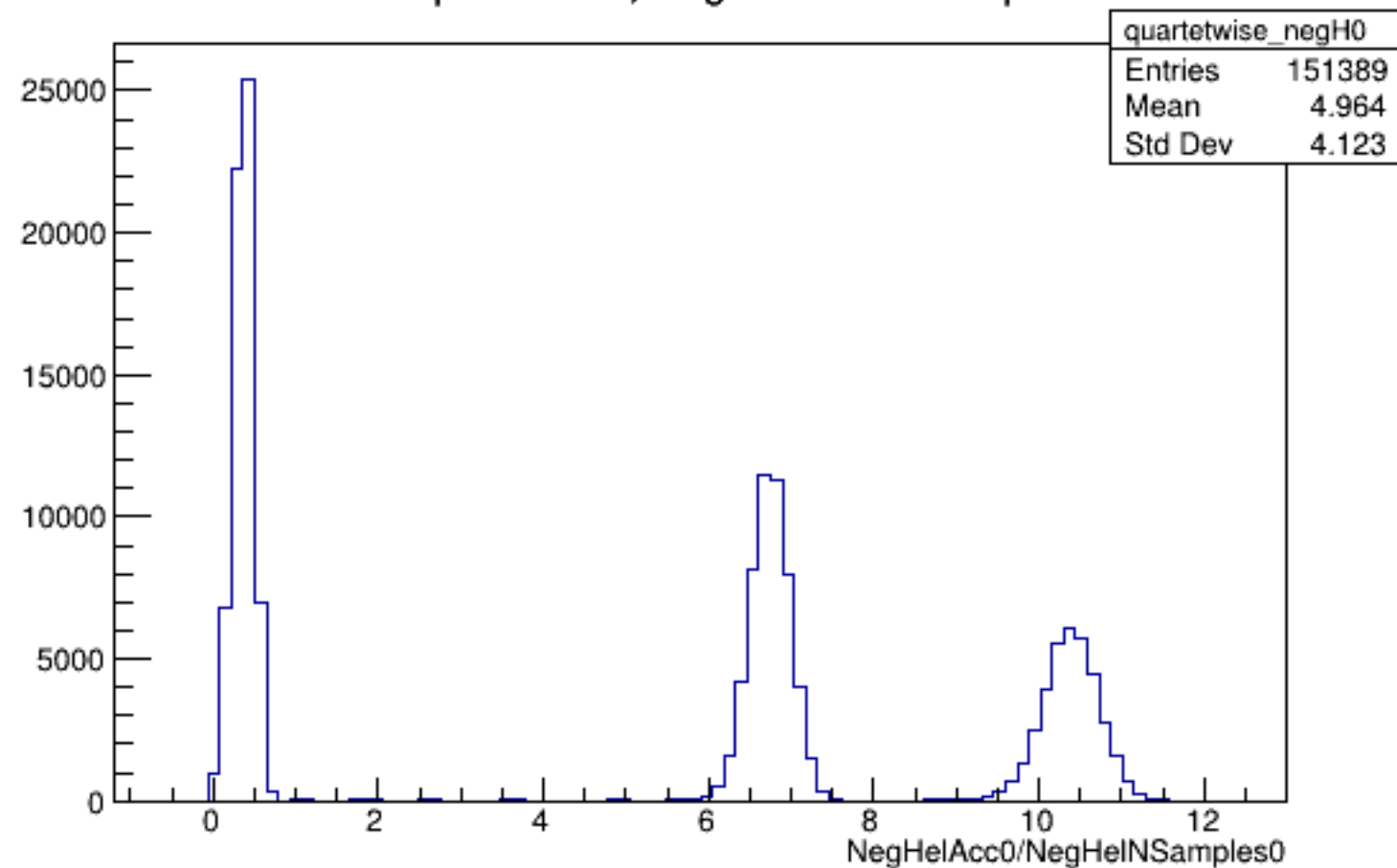
Run 4570 quartetwise, NegHelAcc0/NSamples0: All
