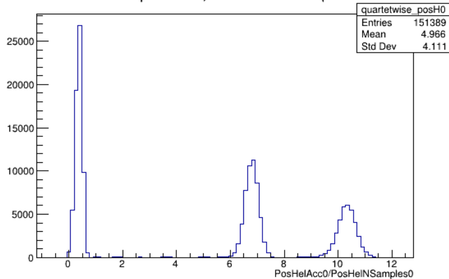
Run 4570 quartetwise, PosHelAcc0/NSamples0: All
