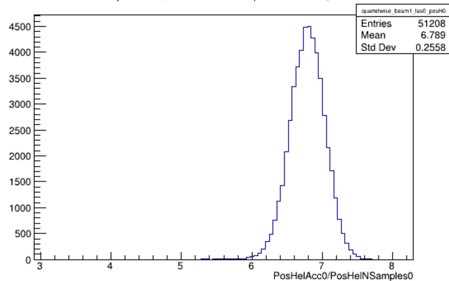
Run 4570 quartetwise, PosHelAcc0/NSamples0: Beam ON, Laser OFF
