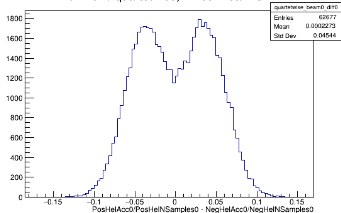
Run 4570 quartetwise, Diffs0: Beam OFF
