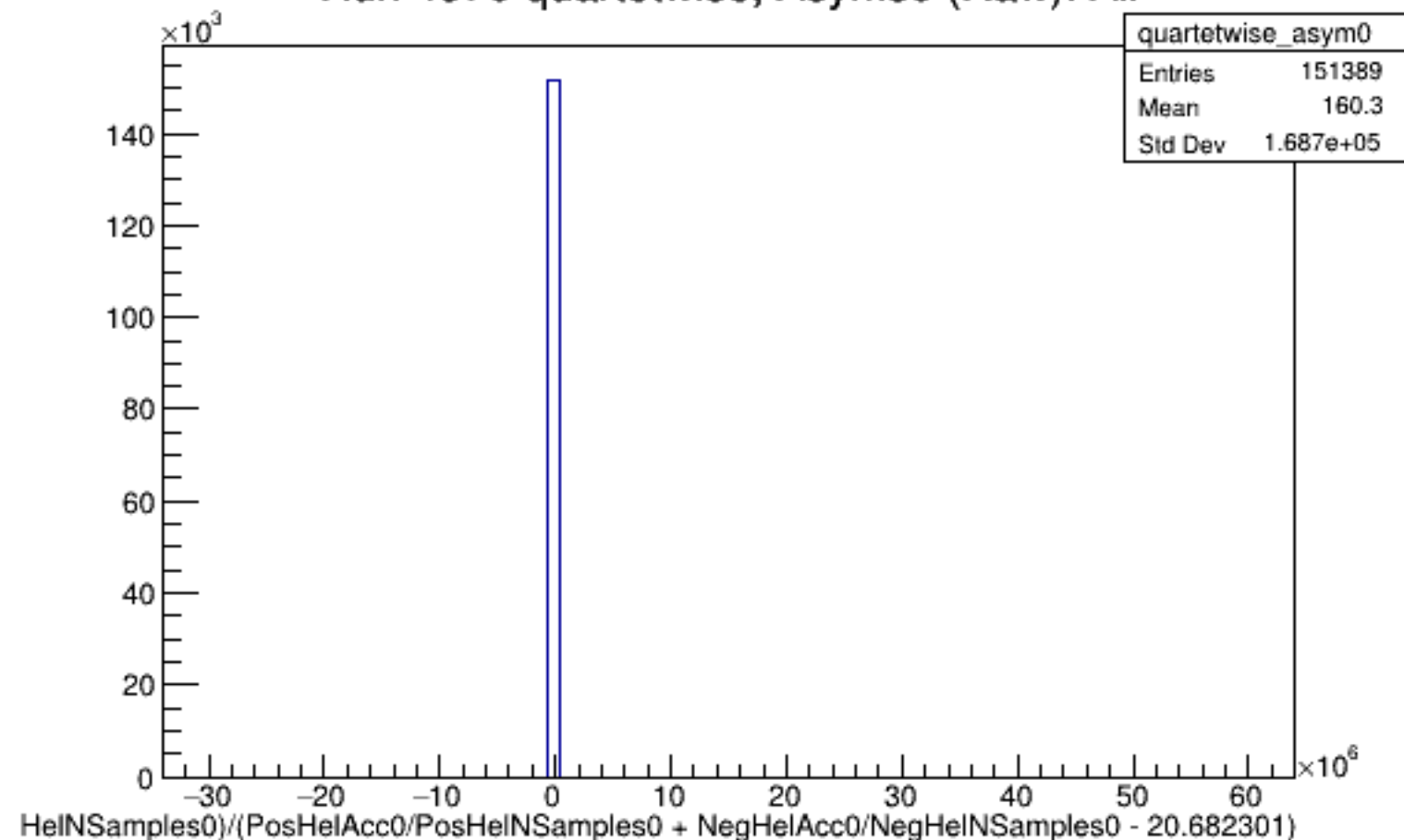
Run 4570 quartetwise, Asyms0 (Raw): All
