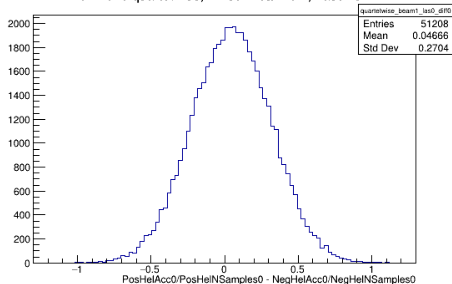
Run 4570 quartetwise, Diffs0: Beam ON, Laser OFF
