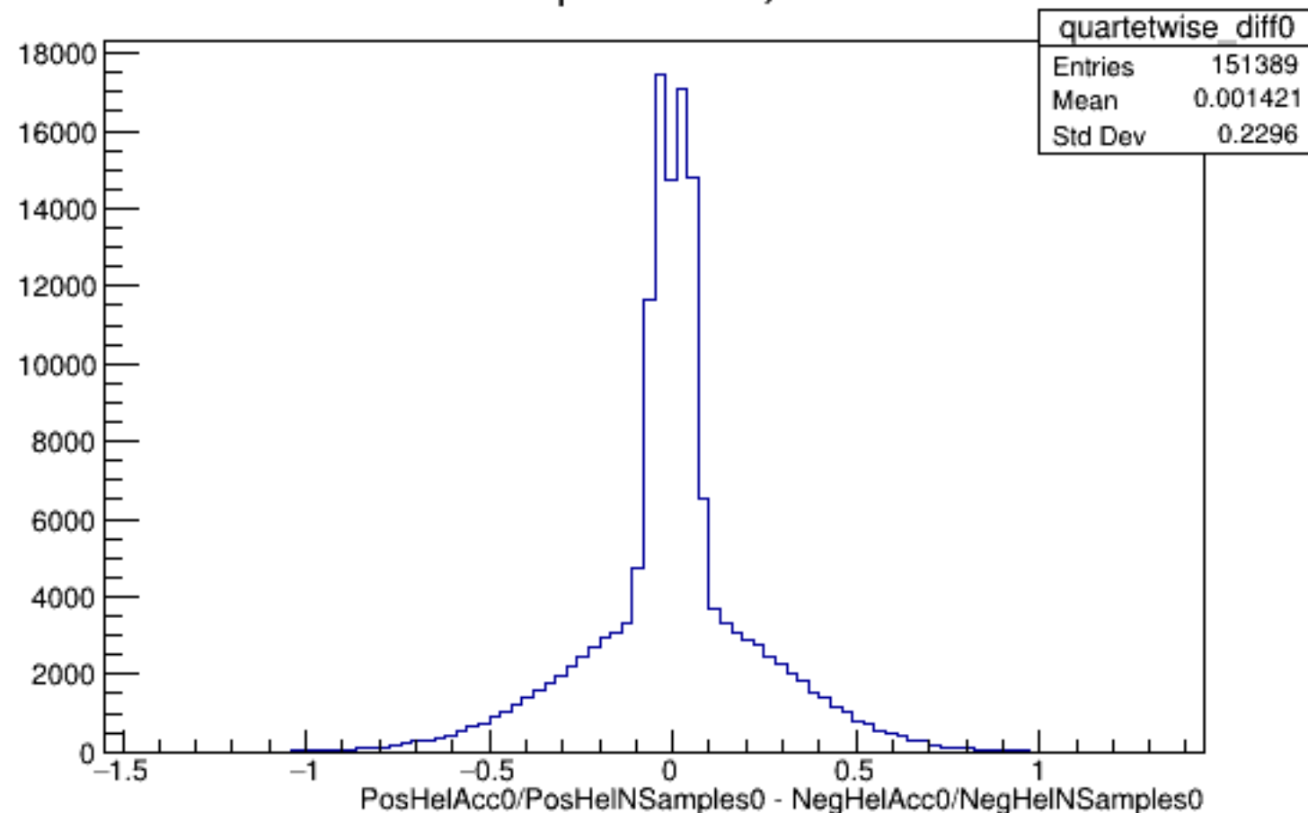
Run 4570 quartetwise, Diffs0: All
