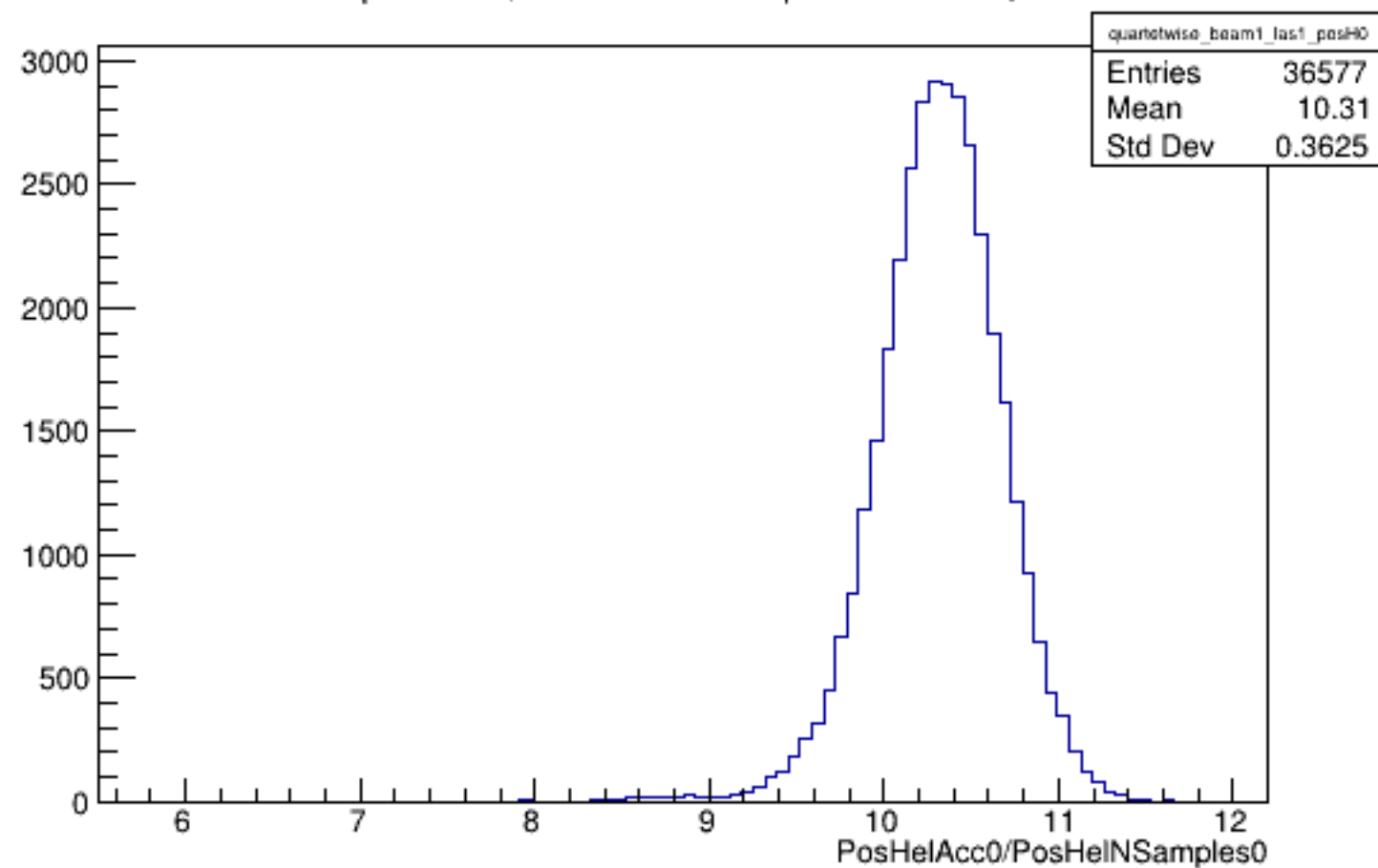
Run 4570 quartetwise, PosHelAcc0/NSamples0: Beam ON, Laser ON
