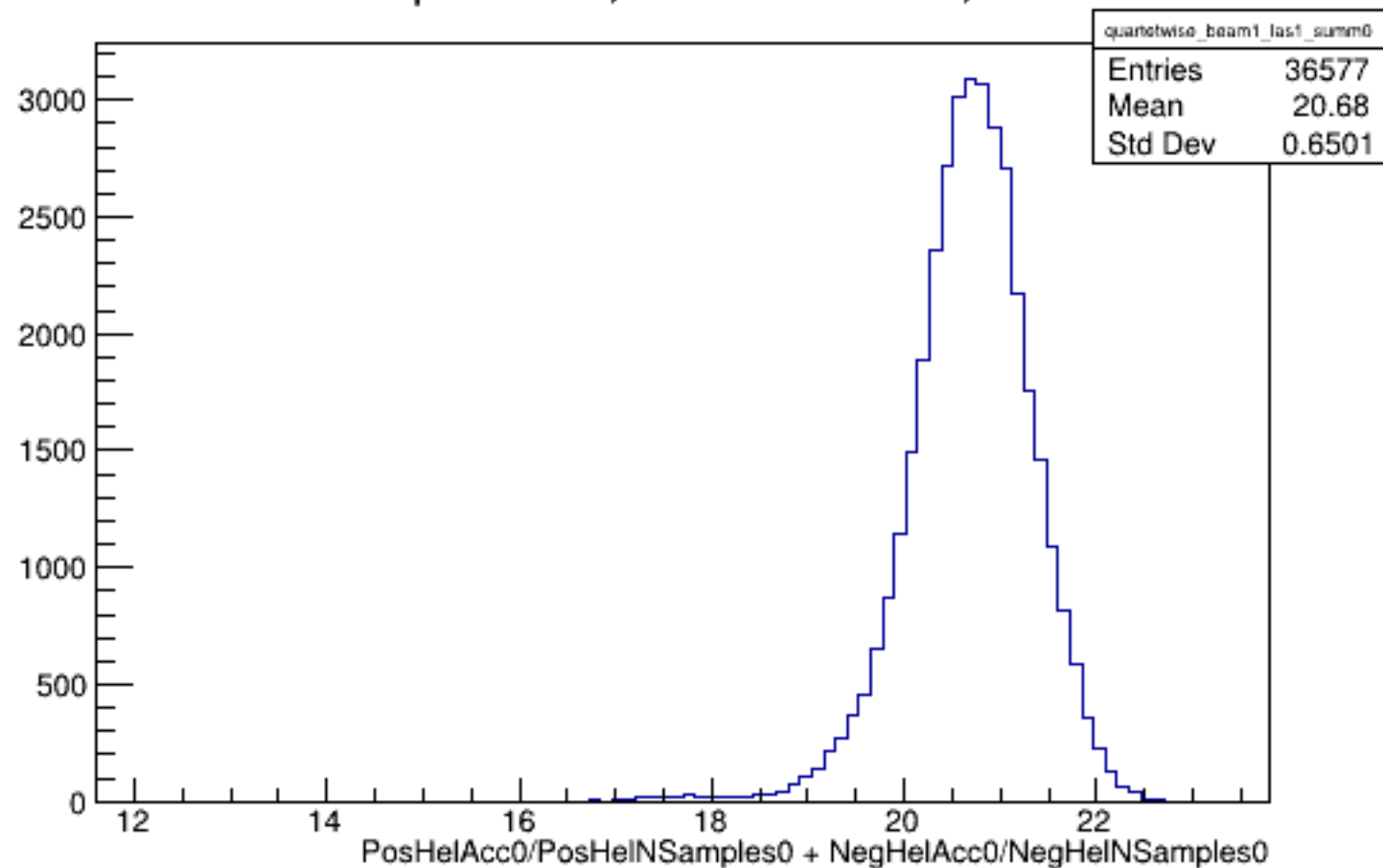
Run 4570 quartetwise, Sums0: Beam ON, Laser ON
