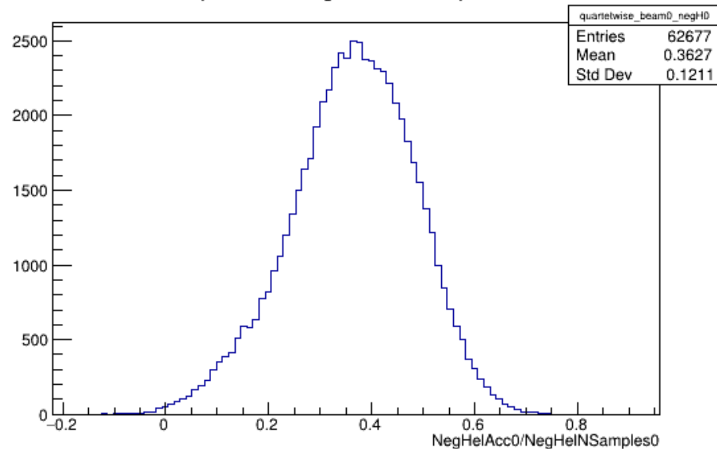
Run 4570 quartetwise, NegHelAcc0/NSamples0: Beam OFF
