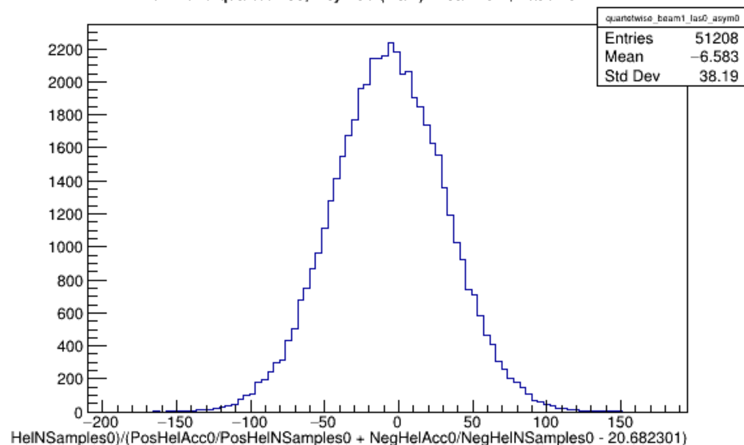
Run 4570 quartetwise, Asyms0 (Raw): Beam ON, Laser OFF
