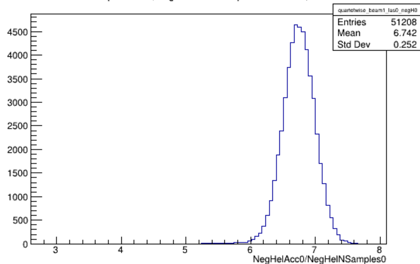
Run 4570 quartetwise, NegHelAcc0/NSamples0: Beam ON, Laser OFF
