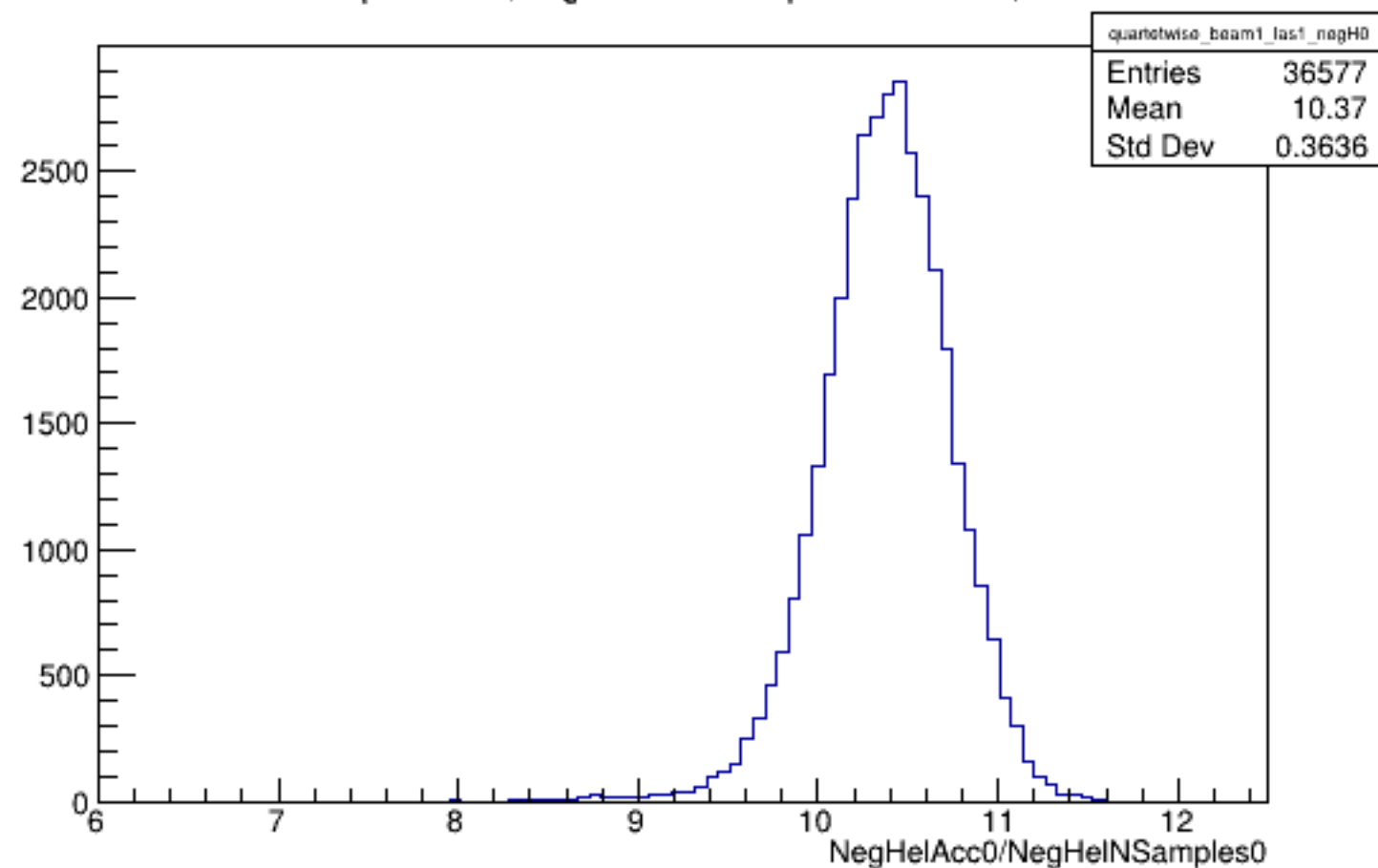
Run 4570 quartetwise, NegHelAcc0/NSamples0: Beam ON, Laser ON
