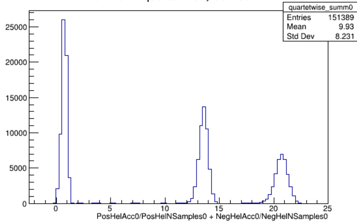
Run 4570 quartetwise, Sums0: All
