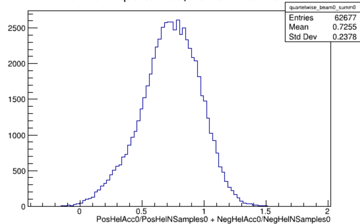
Run 4570 quartetwise, Sums0: Beam OFF
