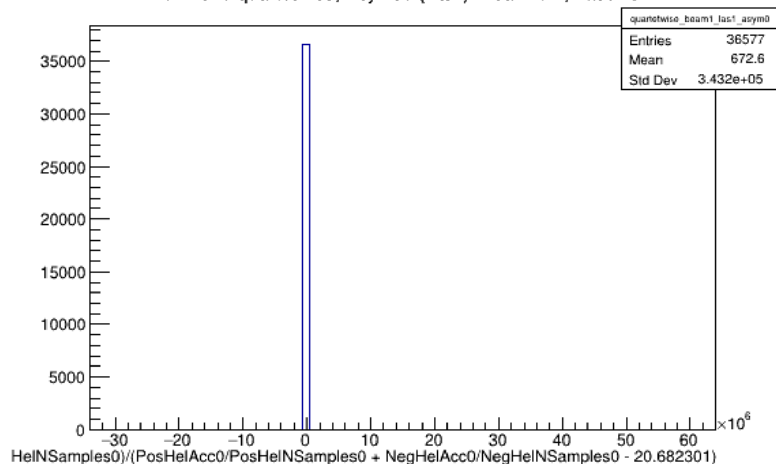
Run 4570 quartetwise, Asyms0 (Raw): Beam ON, Laser ON
