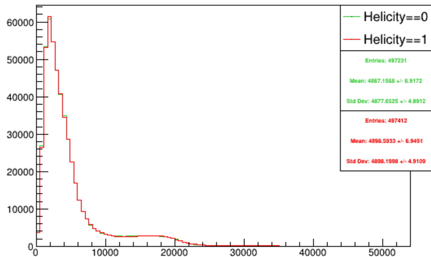
Run 4570 triggerwise, sums: Beam ON, Laser ON
