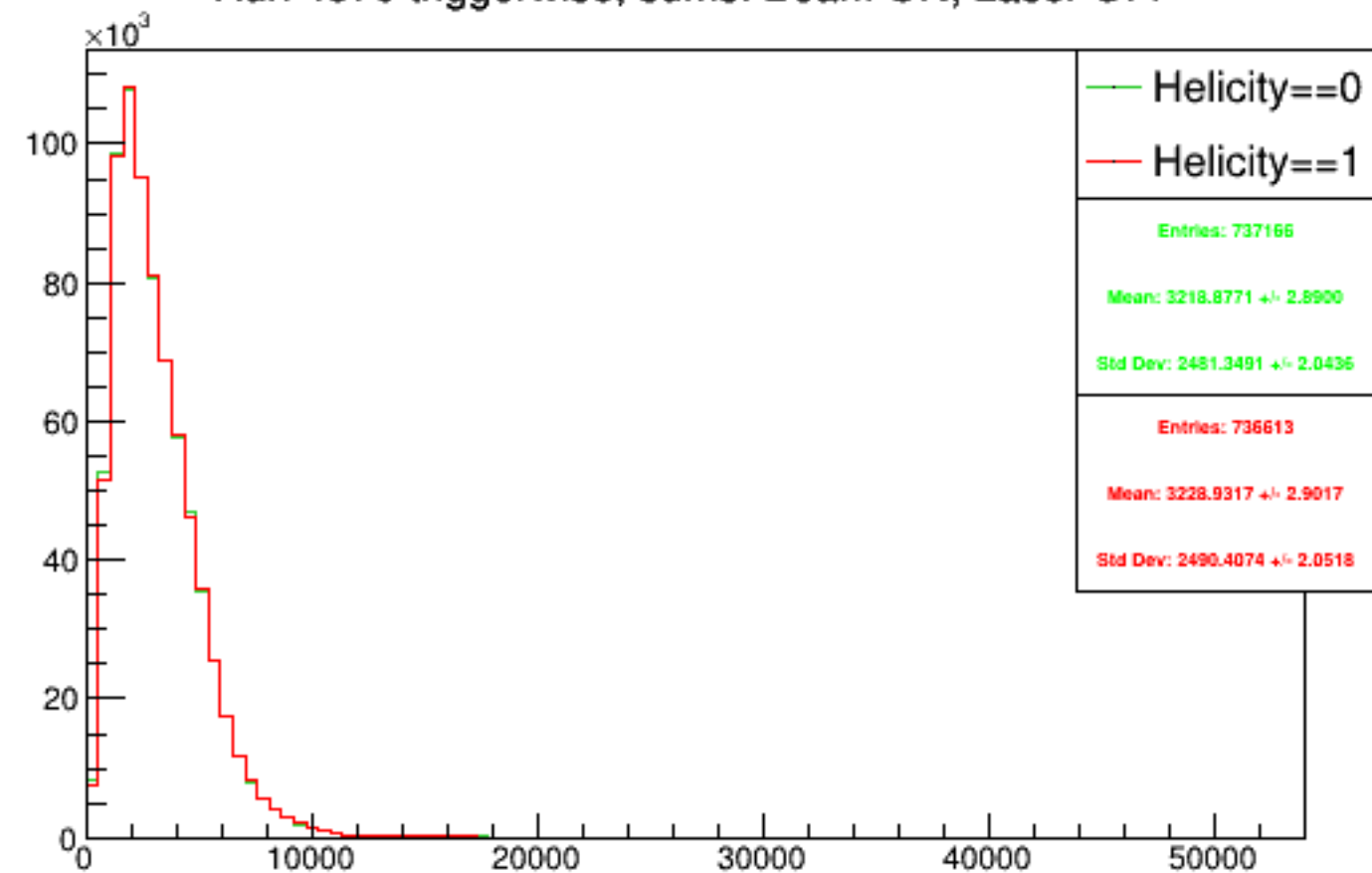
Run 4570 triggerwise, sums: Beam ON, Laser OFF
