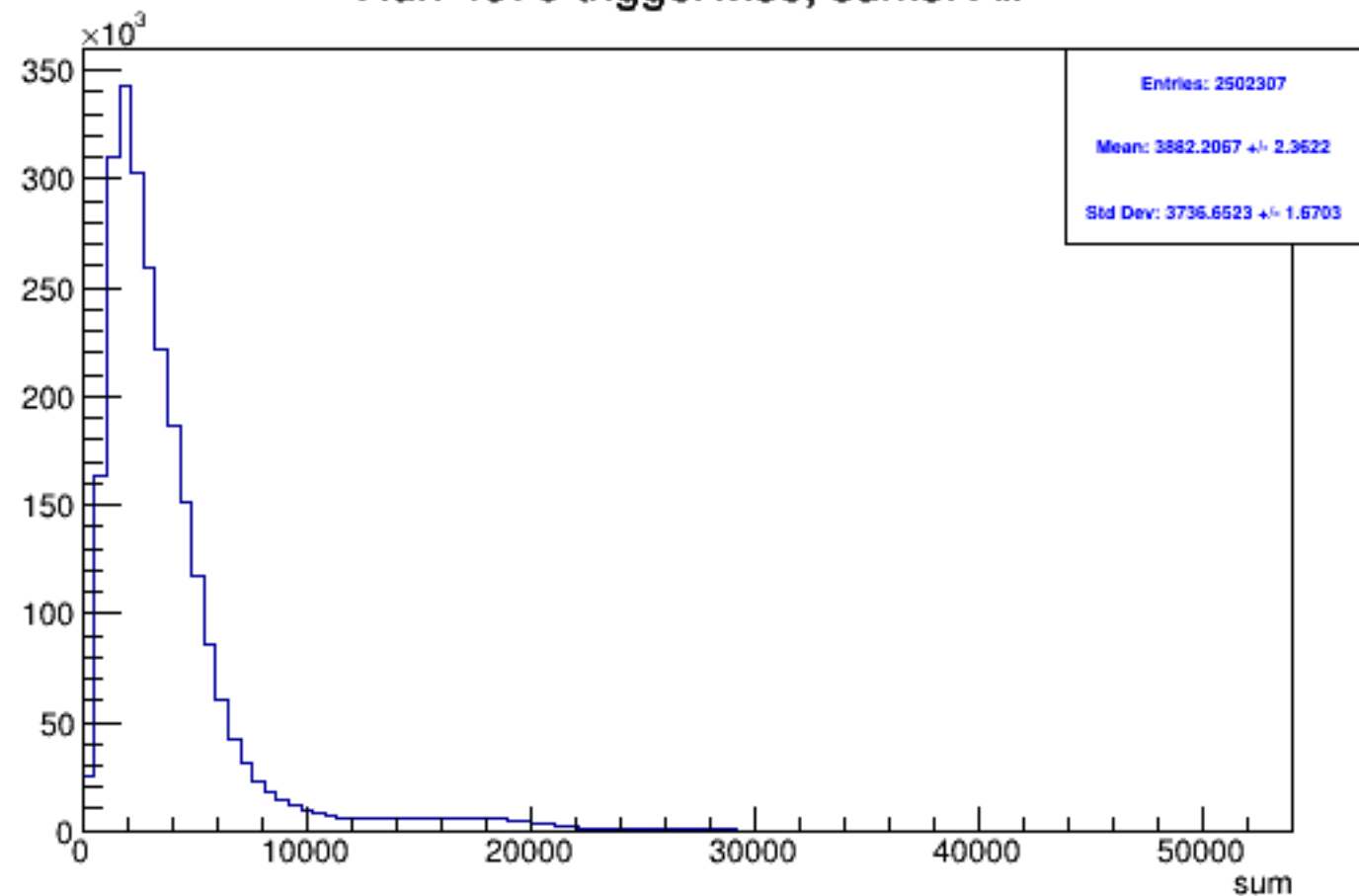
Run 4570 triggerwise, sums: All
