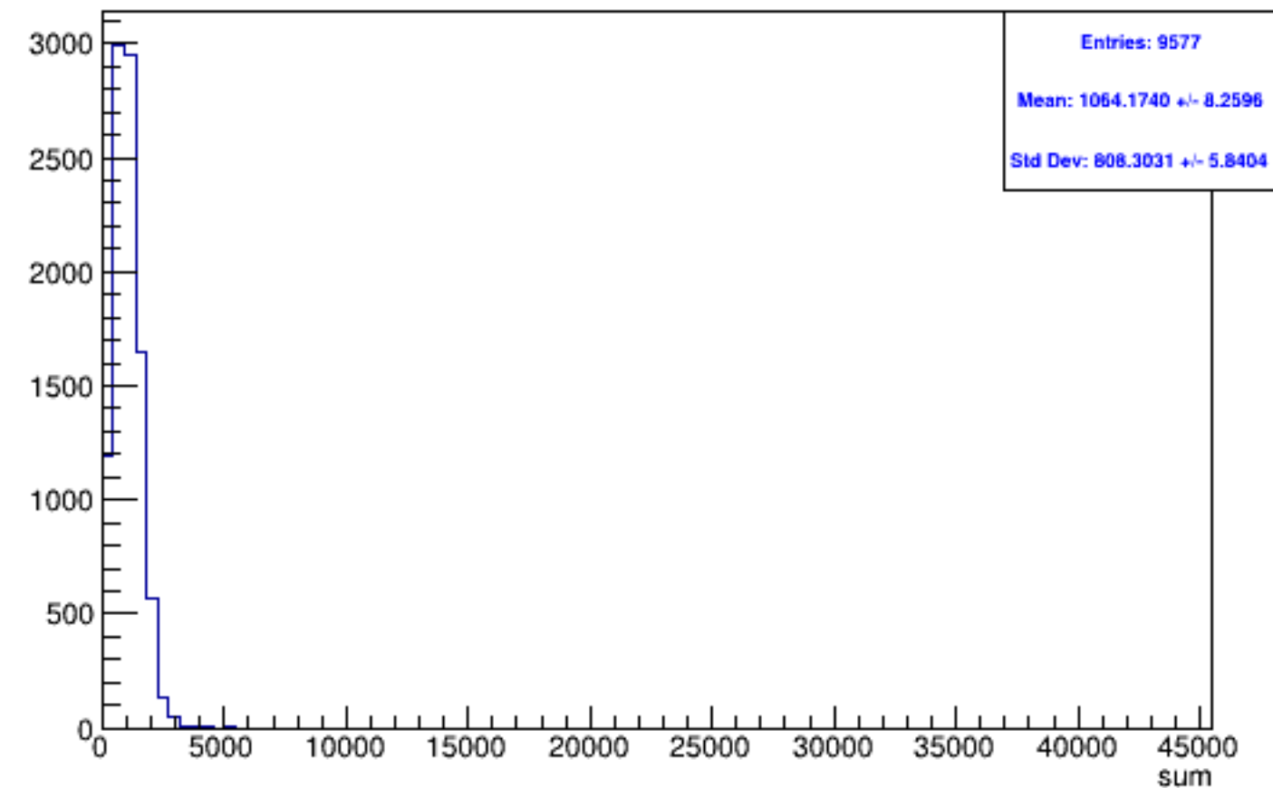
Run 4570 triggerwise, sums: Beam OFF
