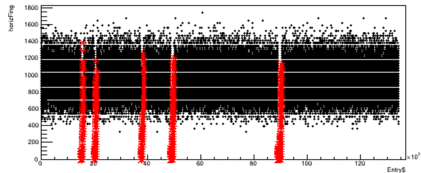
Run 4571, quartetwise: horizFing vs time
