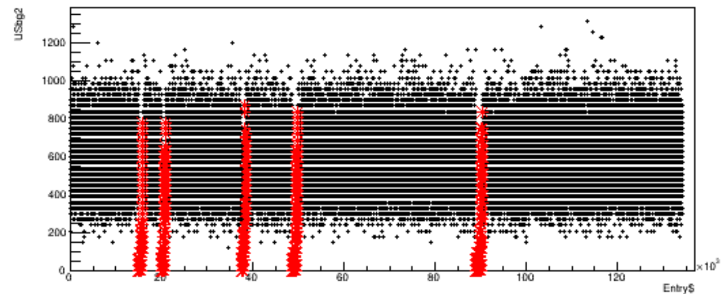
Run 4571, quartetwise: USbg2 vs time
