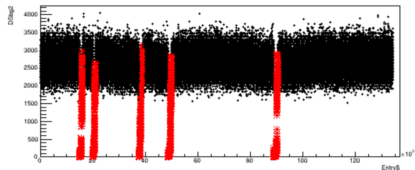
Run 4571, quartetwise: DSbg2 vs time
