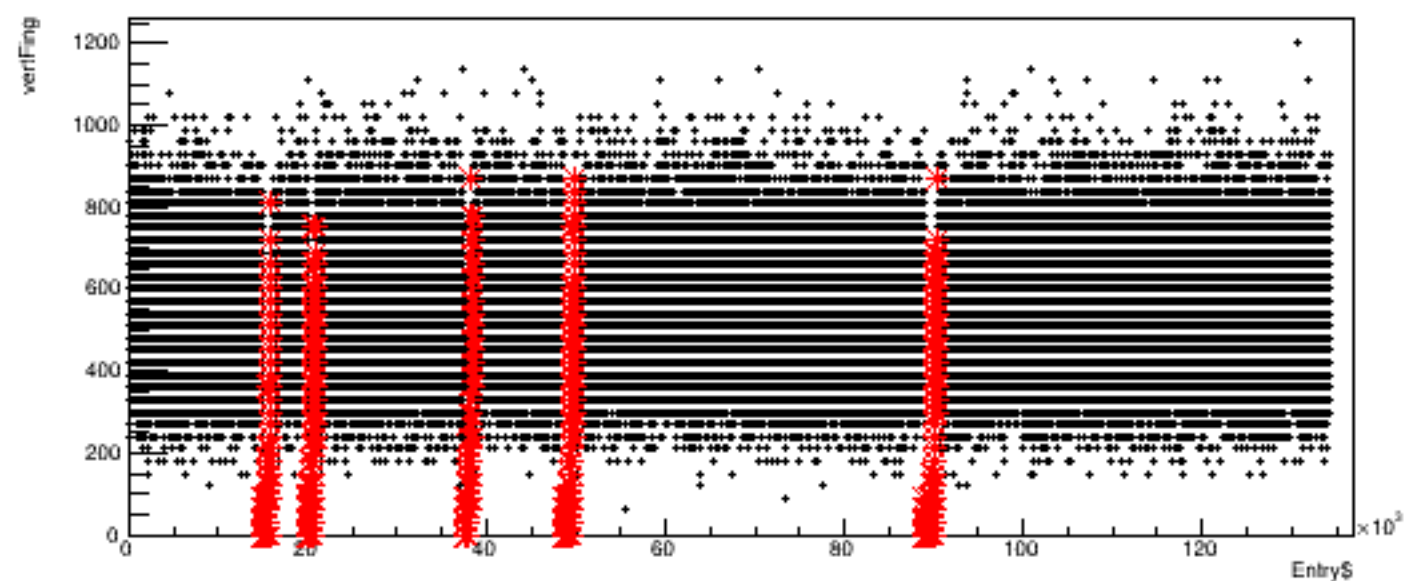
Run 4571, quartetwise: vertFing vs time
