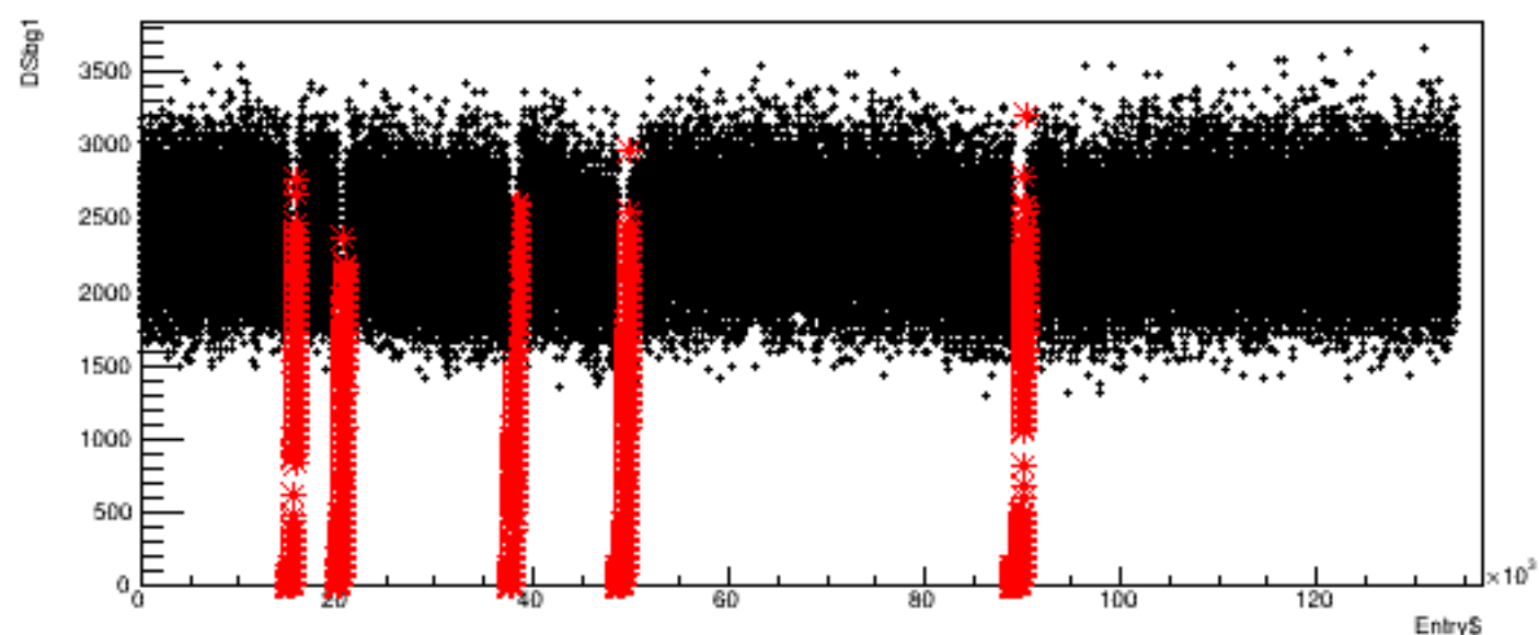
Run 4571, quartetwise: DSbg1 vs time
