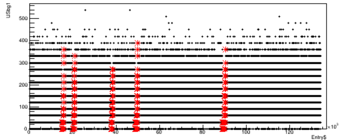
Run 4571, quartetwise: USbg1 vs time
