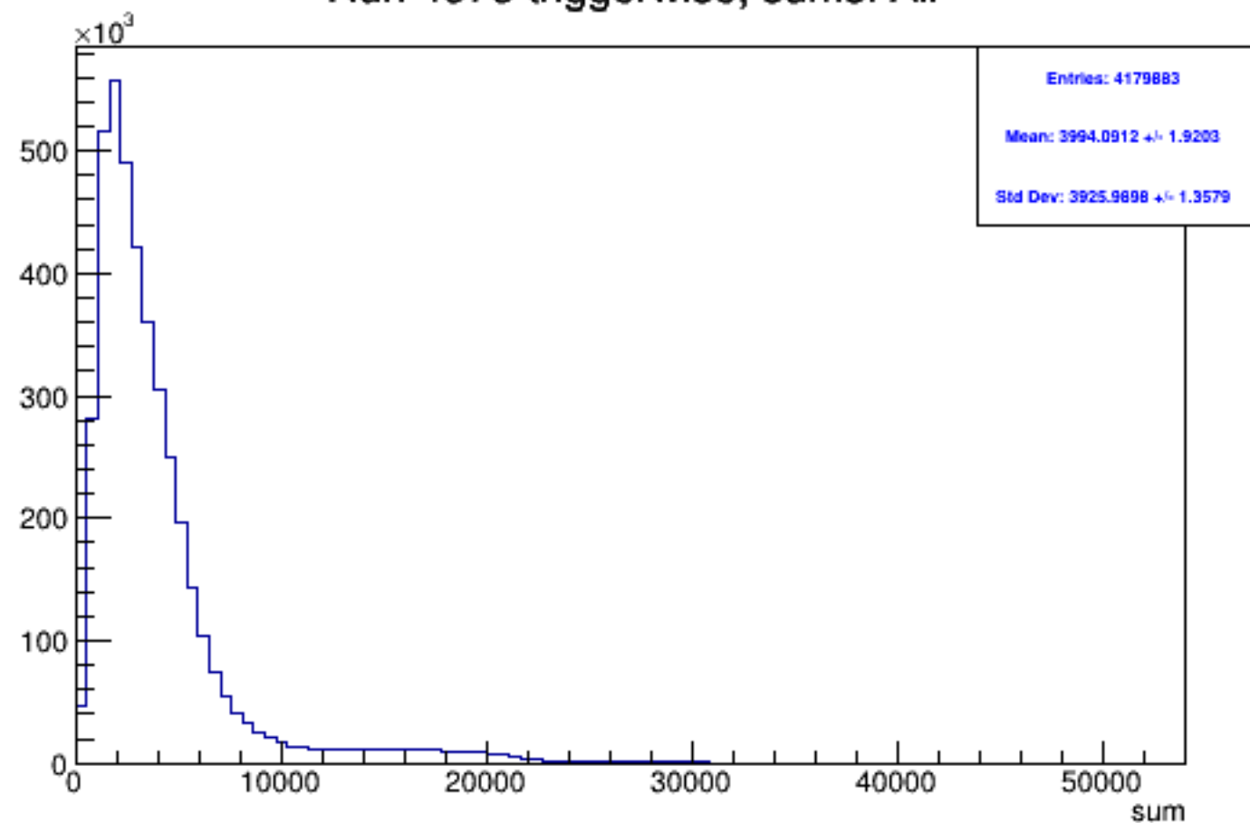
Run 4573 triggerwise, sums: All
