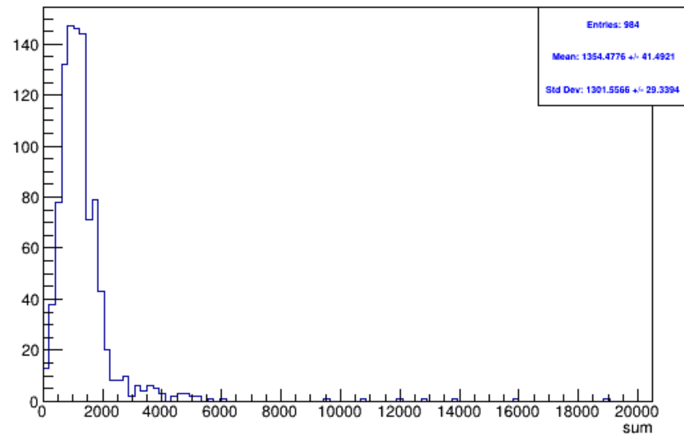
Run 4576 triggerwise, sums: Beam OFF
