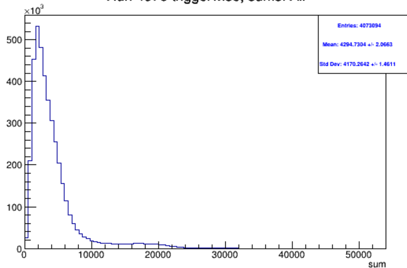
Run 4576 triggerwise, sums: All
