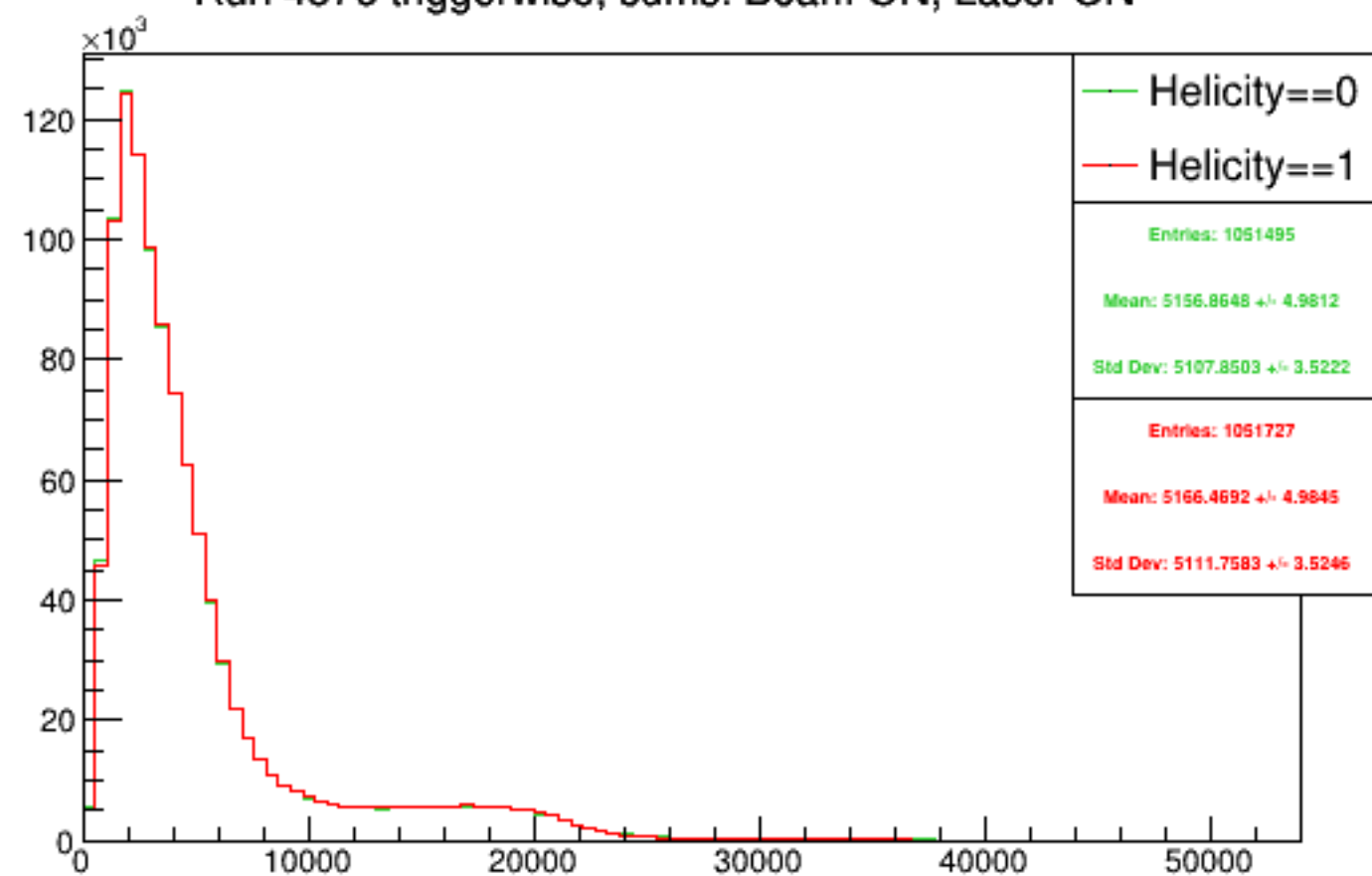
Run 4576 triggerwise, sums: Beam ON, Laser ON
