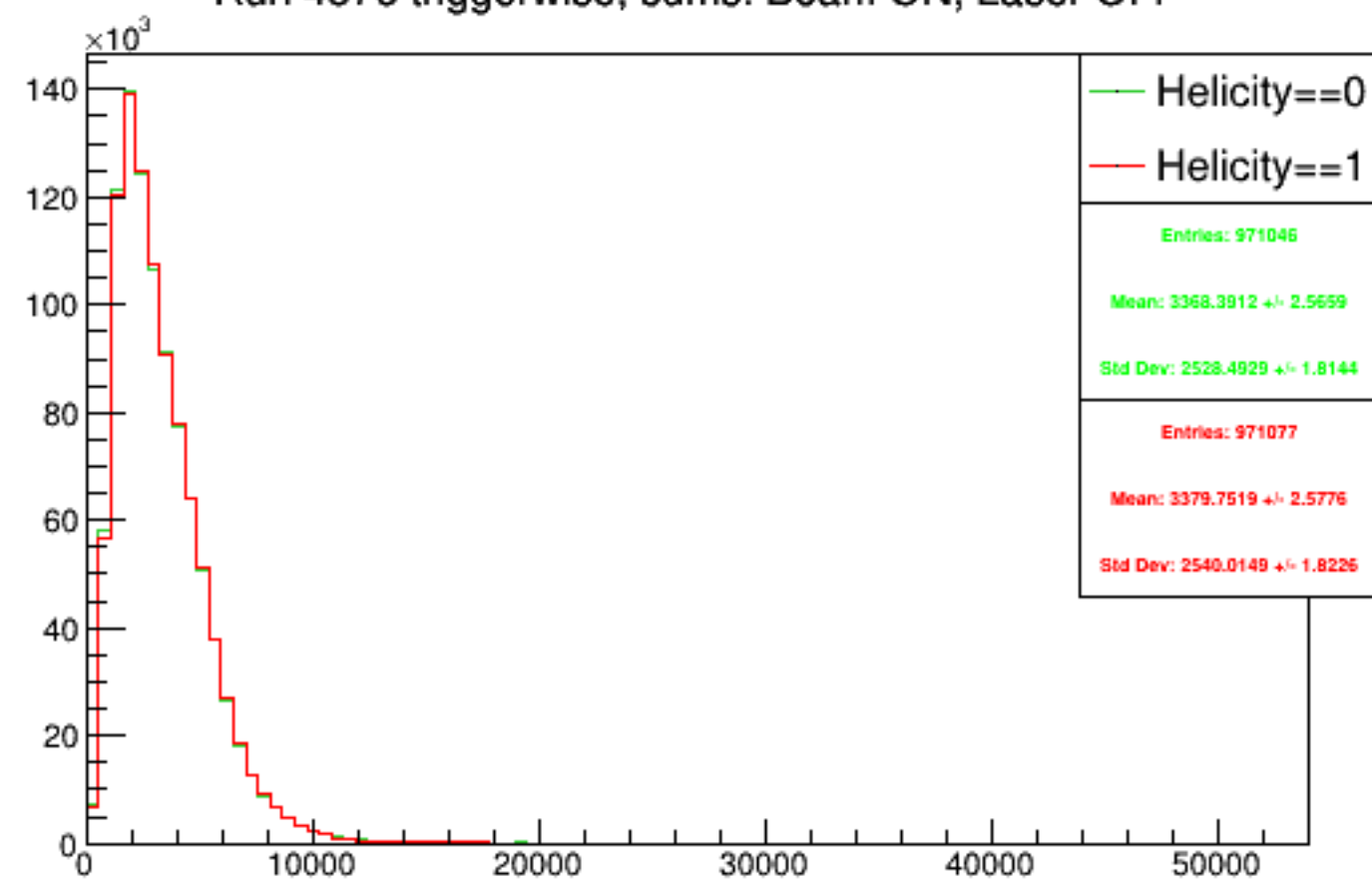
Run 4576 triggerwise, sums: Beam ON, Laser OFF
