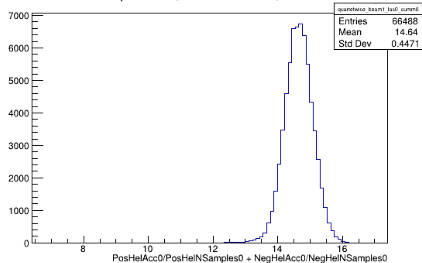
Run 4578 quartetwise, Sums0: Beam ON, Laser OFF
