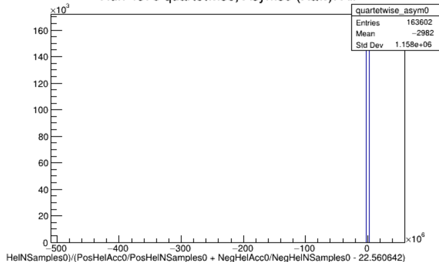
Run 4578 quartetwise, Asyms0 (Raw): All
