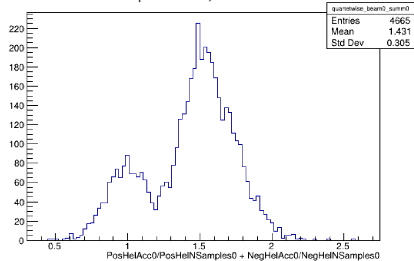
Run 4578 quartetwise, Sums0: Beam OFF
