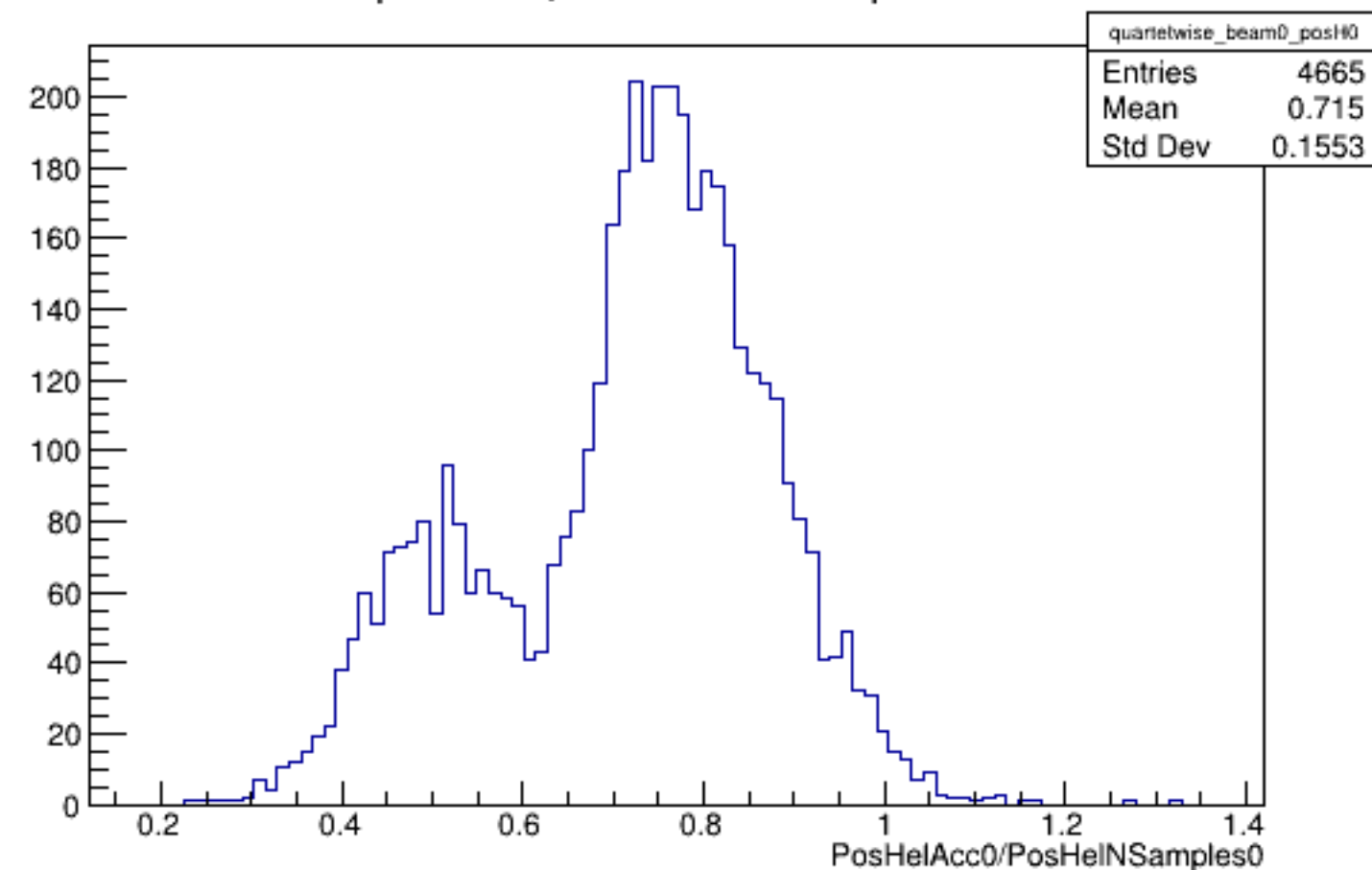
Run 4578 quartetwise, PosHelAcc0/NSamples0: Beam OFF
