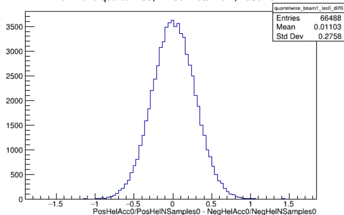
Run 4578 quartetwise, Diffs0: Beam ON, Laser OFF
