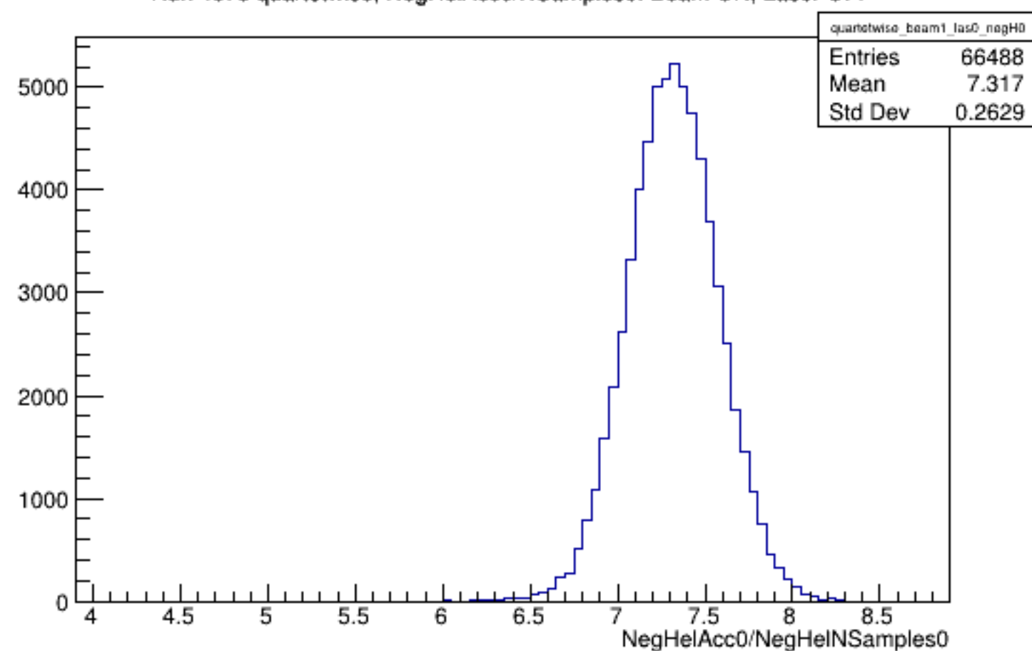
Run 4578 quartetwise, NegHelAcc0/NSamples0: Beam ON, Laser OFF
