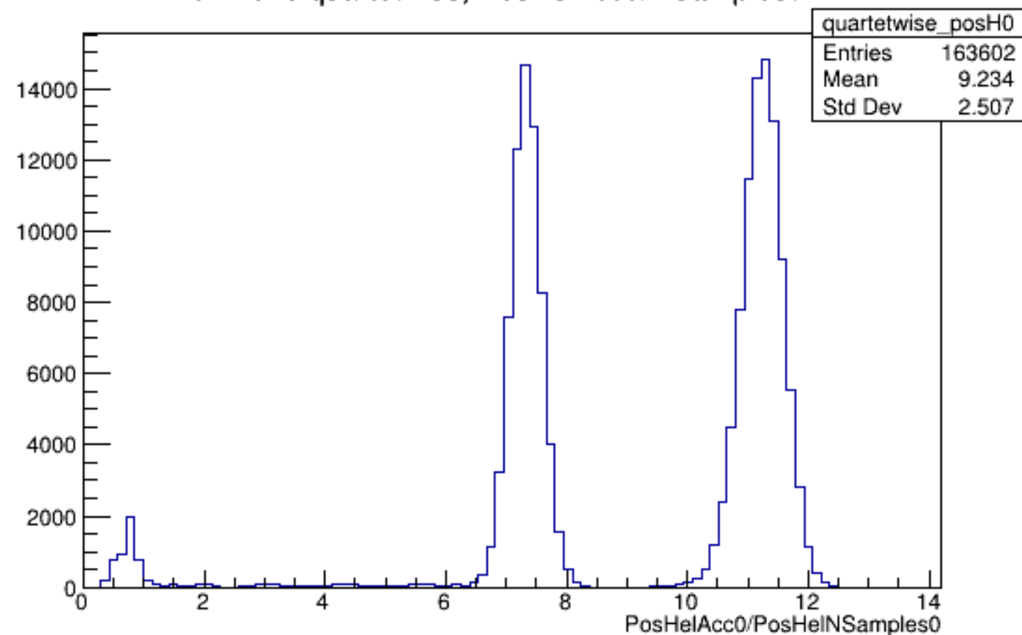
Run 4578 quartetwise, PosHelAcc0/NSamples0: All
