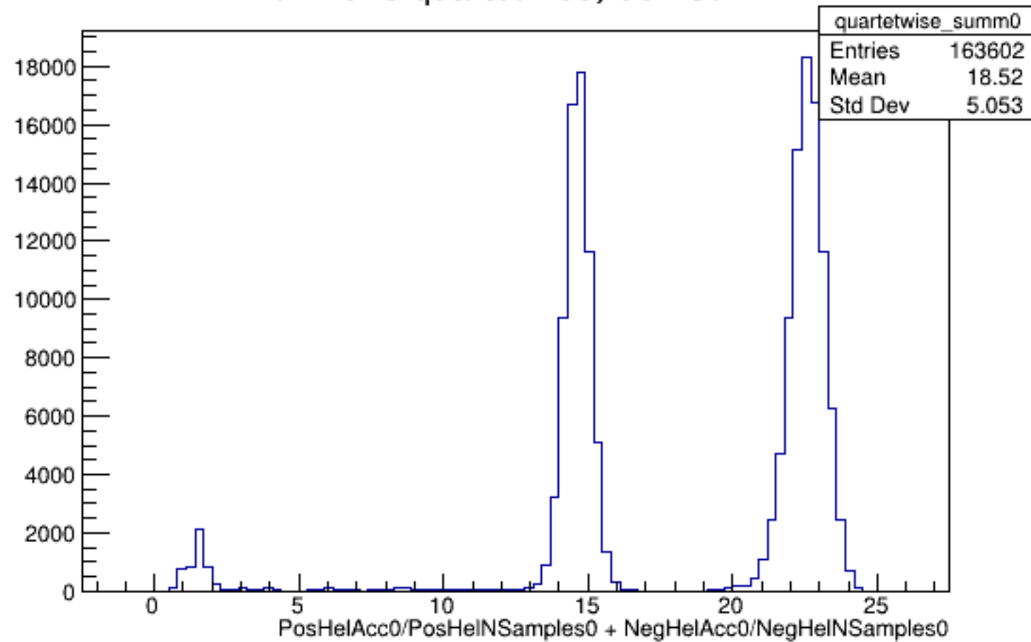
Run 4578 quartetwise, Sums0: All
