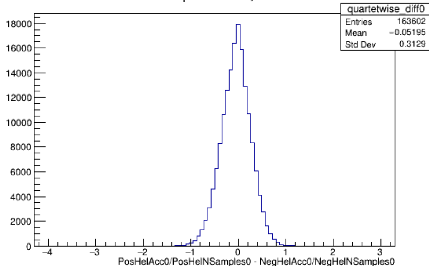
Run 4578 quartetwise, Diffs0: All
