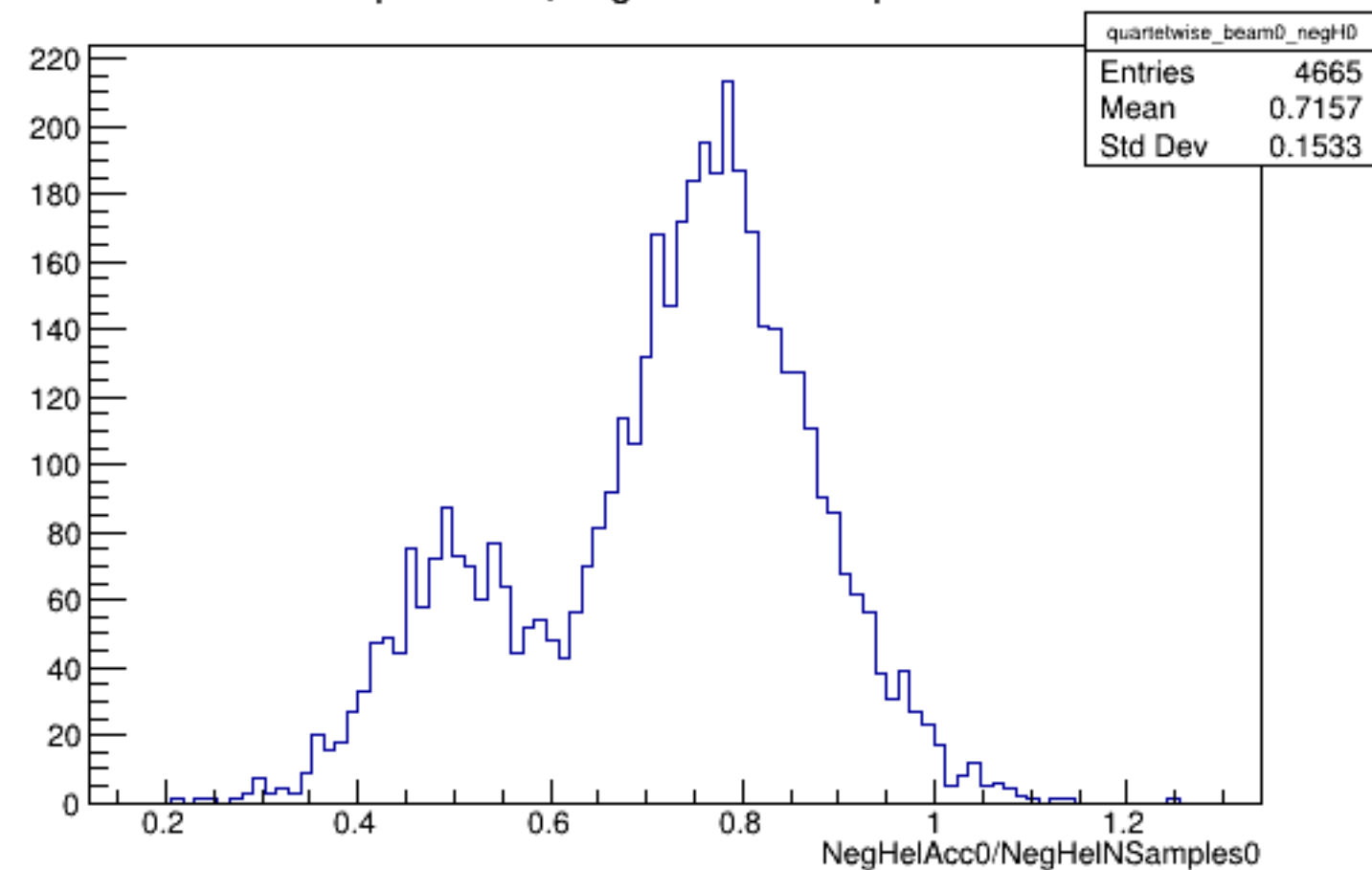
Run 4578 quartetwise, NegHelAcc0/NSamples0: Beam OFF
