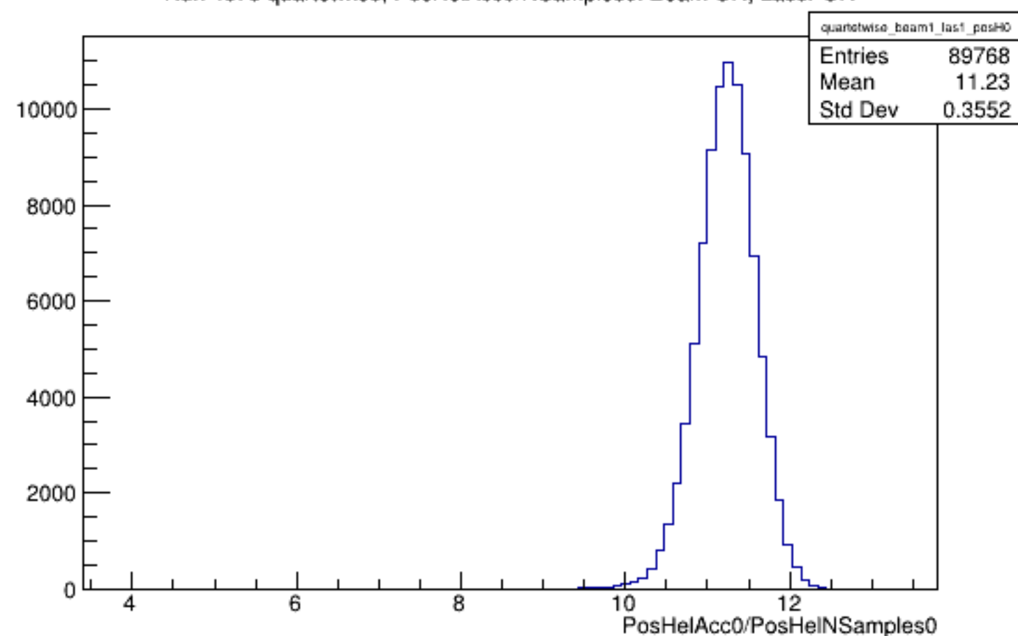
Run 4578 quartetwise, PosHelAcc0/NSamples0: Beam ON, Laser ON
