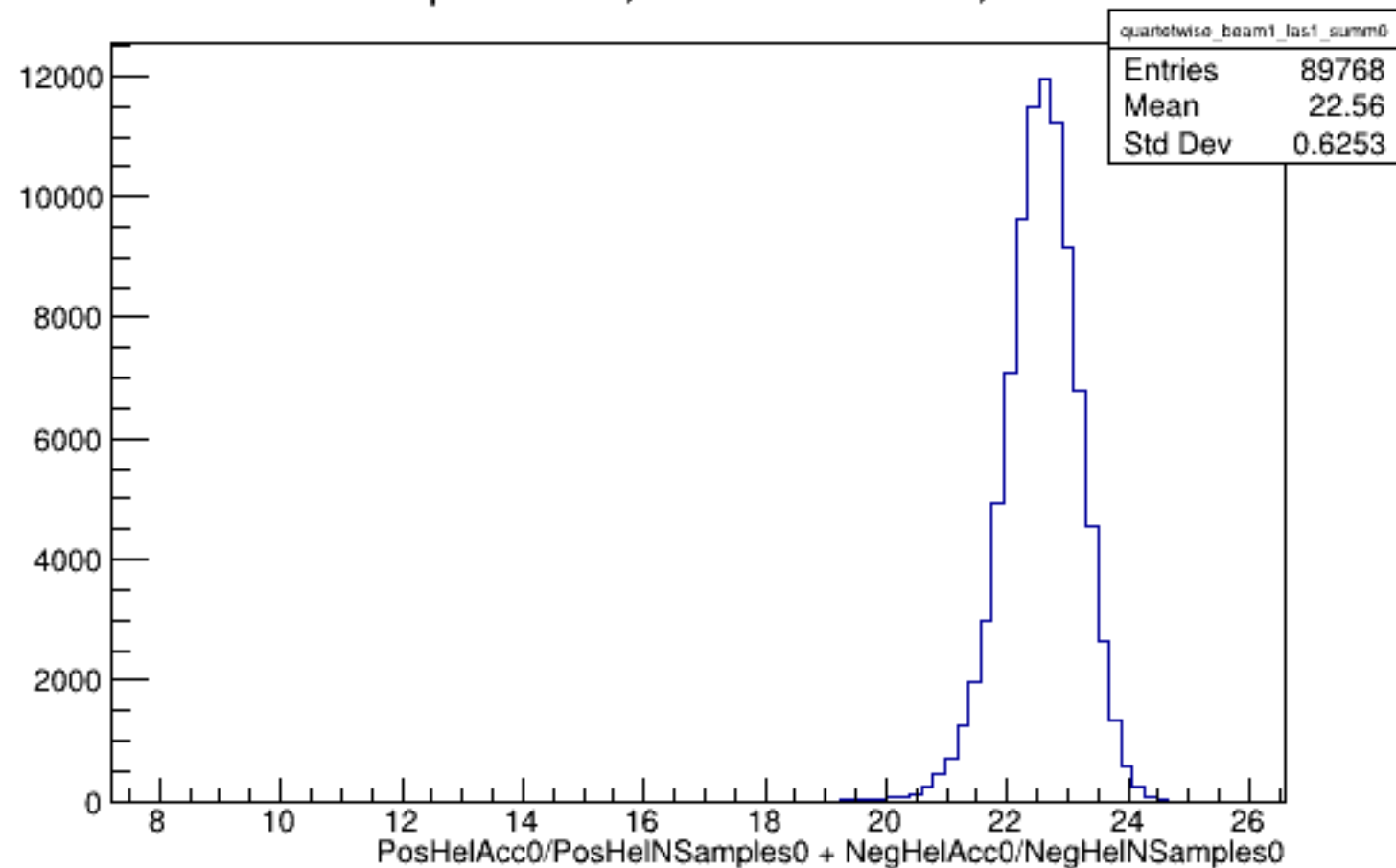
Run 4578 quartetwise, Sums0: Beam ON, Laser ON
