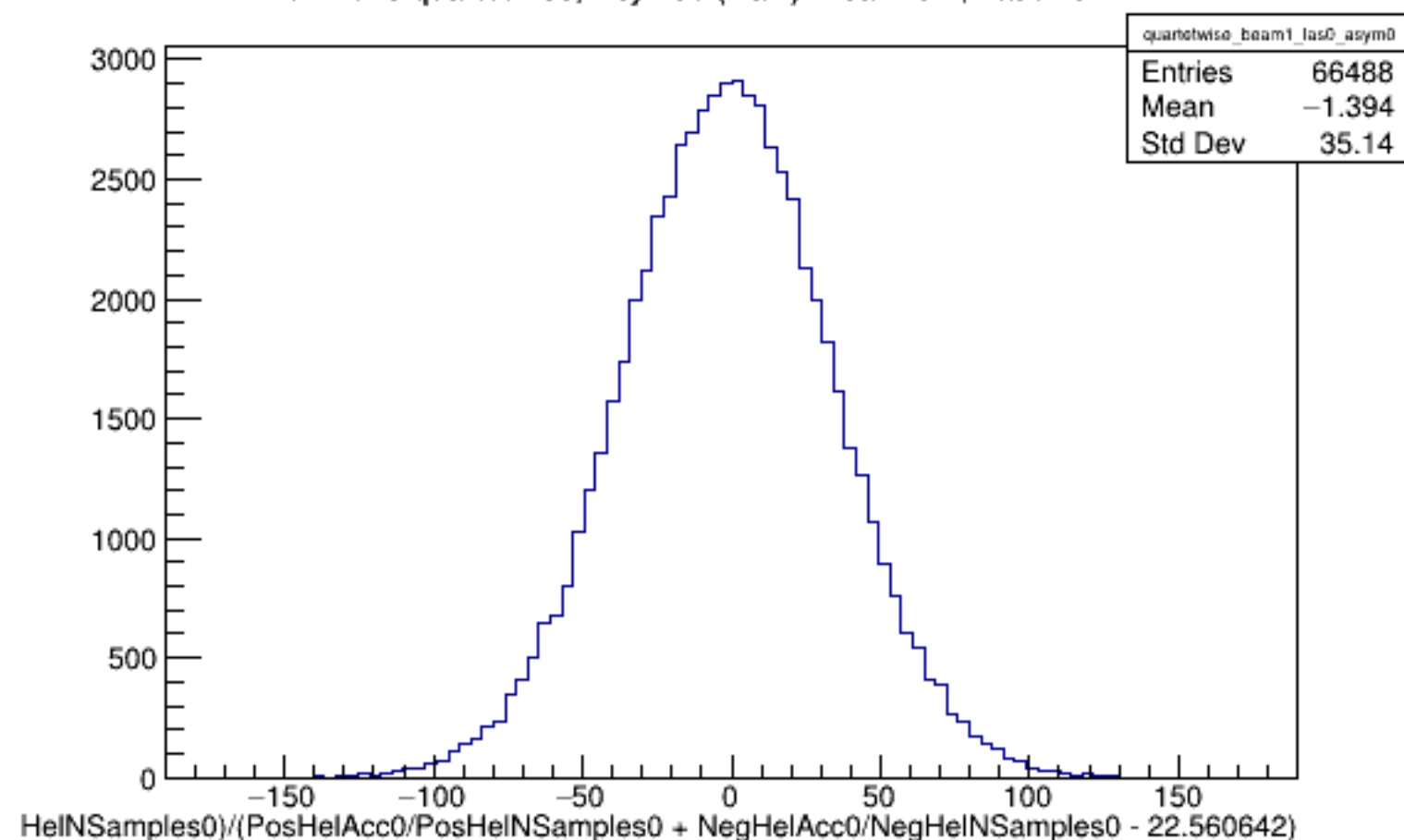
Run 4578 quartetwise, Asyms0 (Raw): Beam ON, Laser OFF
