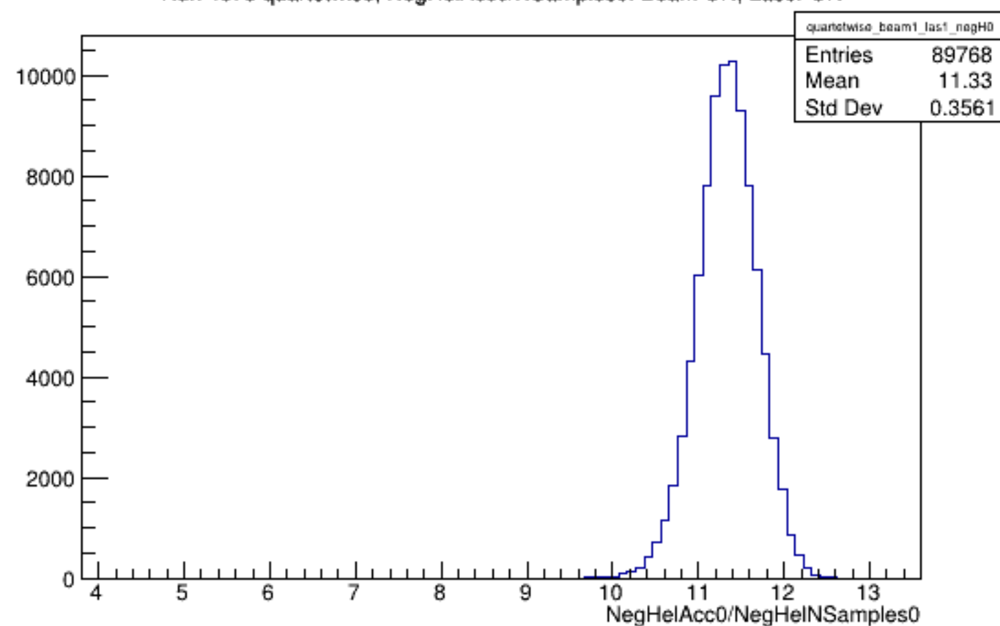
Run 4578 quartetwise, NegHelAcc0/NSamples0: Beam ON, Laser ON
