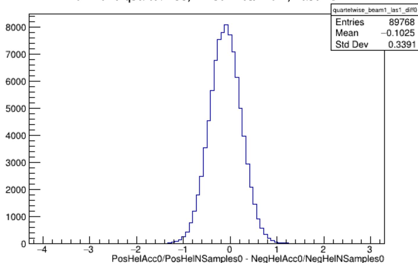
Run 4578 quartetwise, Diffs0: Beam ON, Laser ON
