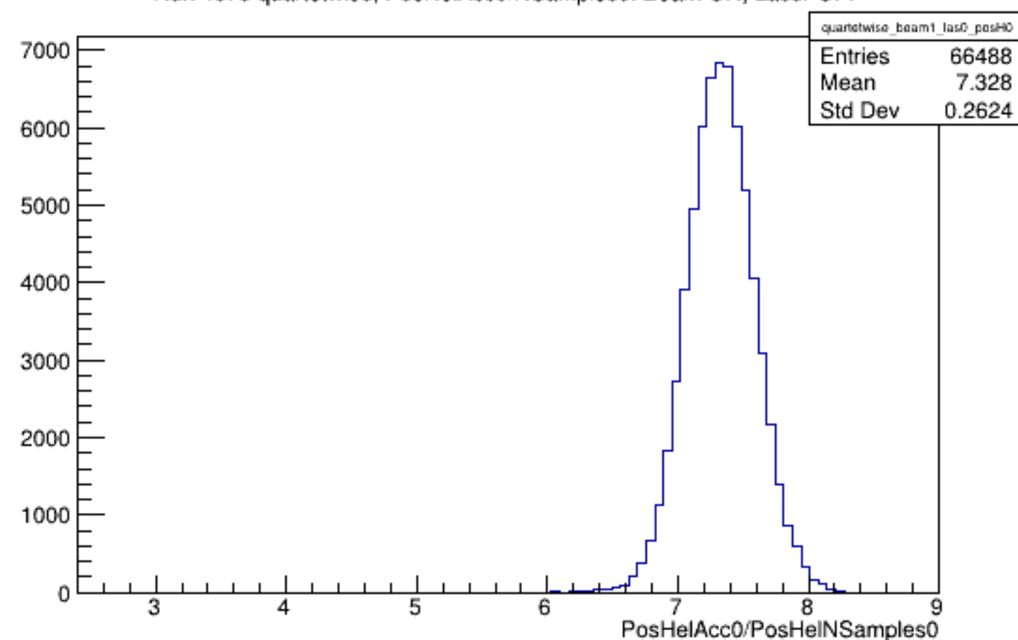
Run 4578 quartetwise, PosHelAcc0/NSamples0: Beam ON, Laser OFF
