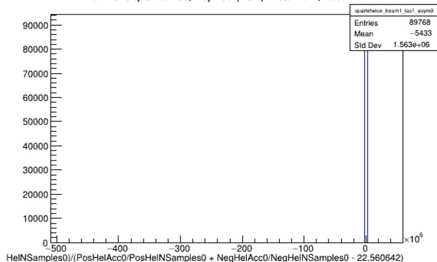
Run 4578 quartetwise, Asyms0 (Raw): Beam ON, Laser ON
