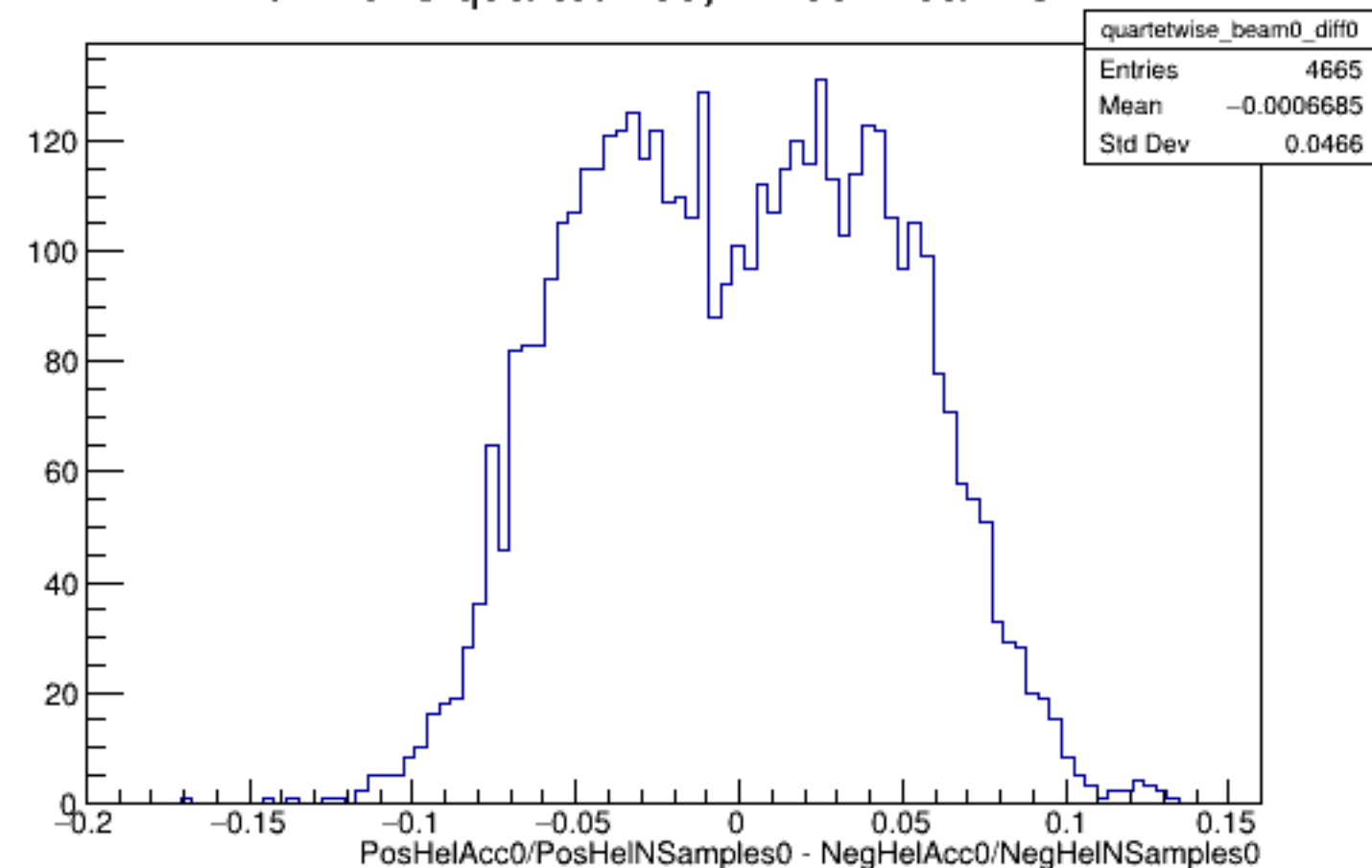
Run 4578 quartetwise, Diffs0: Beam OFF
