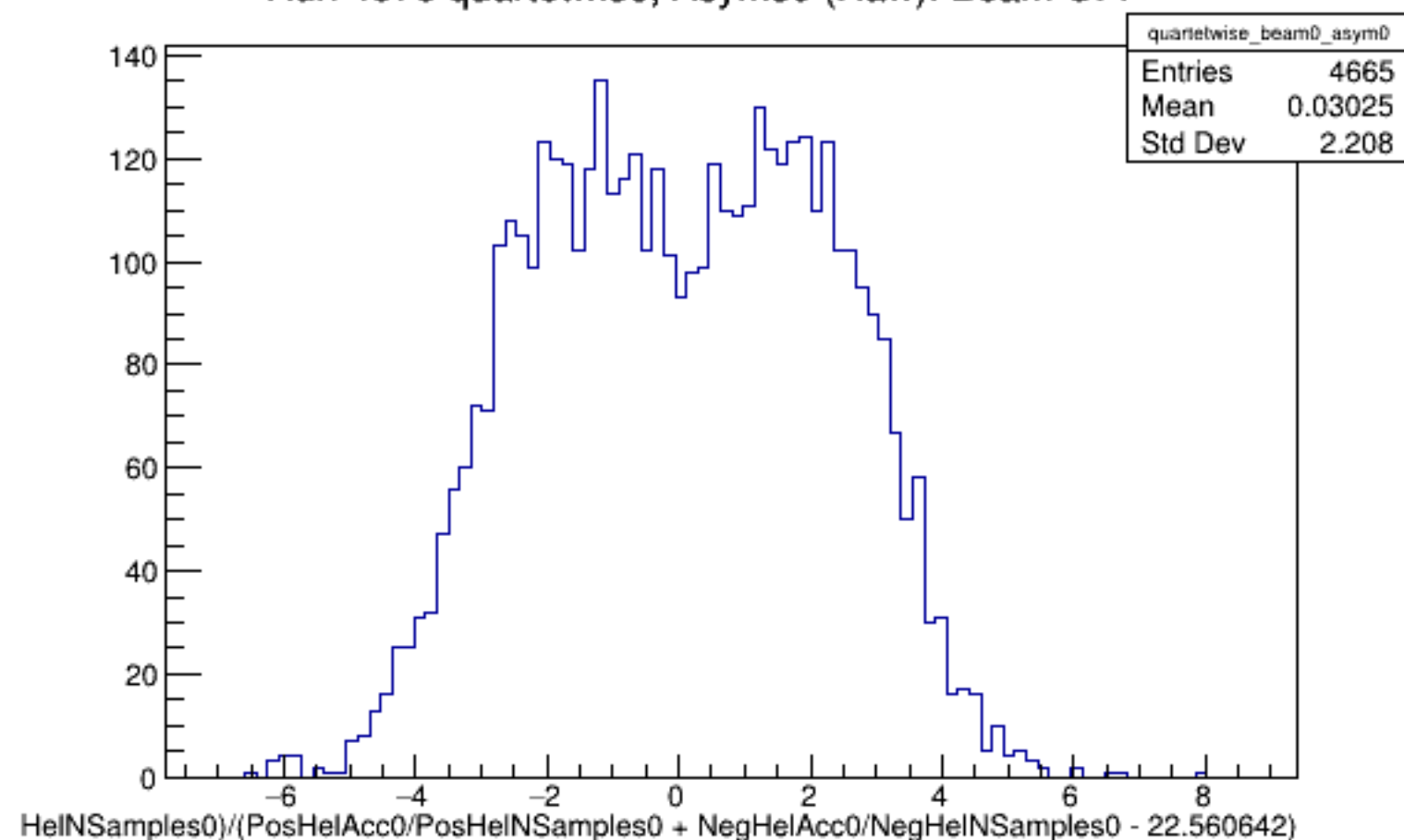
Run 4578 quartetwise, Asyms0 (Raw): Beam OFF
