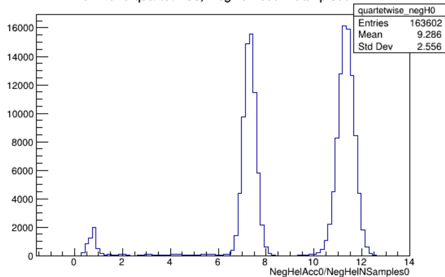
Run 4578 quartetwise, NegHelAcc0/NSamples0: All
